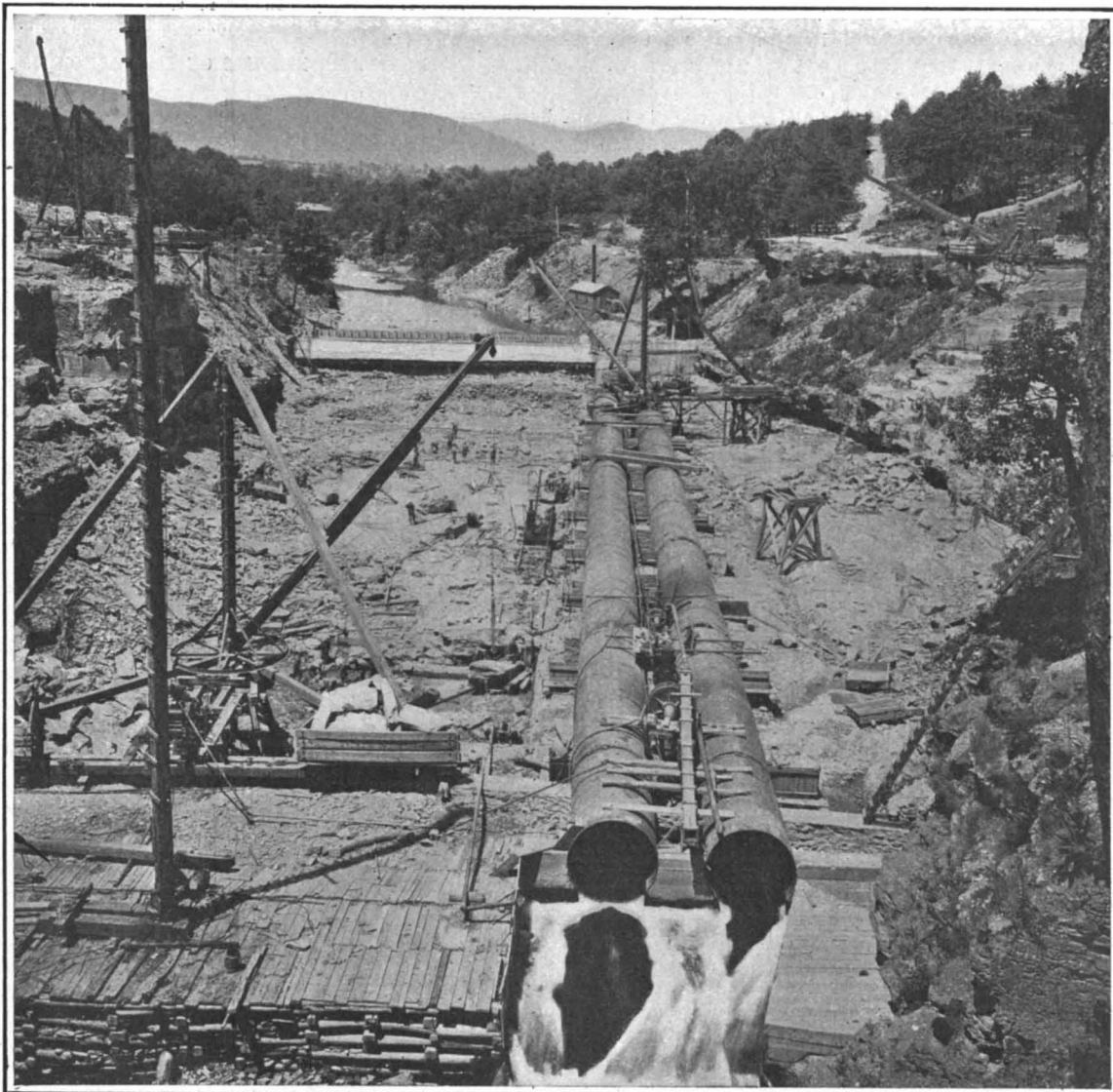
During construction the flow of the river is conducted across the site of the dam in two 8-foot steel pipes. PREPARING THE FOUNDATIONS FOR THE ASHOKAN DAM, WHICH WILL IMPOUND 170,000,000 GALLONS OF WATER.
