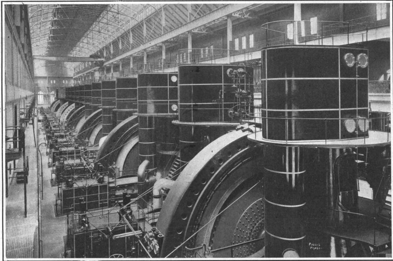
This power station, the largest for traction purposes in the world, is 200 feet wide by 790 feet long. It contains nine reciprocating Allis-Chalmers engines of 12,000 overload horse-power and three steam turbines of 1,800 horse-power.
