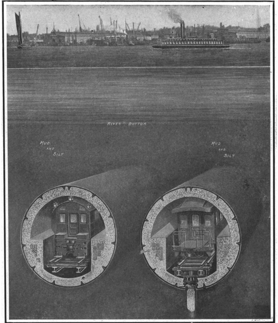
External diameter, 23 feet; internal diameter, 19 feet. Driven by the shield method. Maximum rate of advance through mud and silt, 37 1/4 feet per day.
