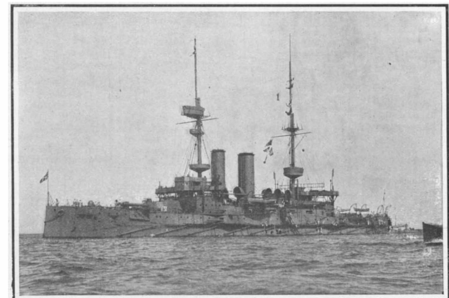
Displacement, 15,000 tons. Speed, 18.5 knots. Coal, 2,100 tons. Armor: belt, 9-inch; side, 9-inch; deck, 3-inch; barbette turrets 10-inch to 12-inch; casemates, 6-inch. Guns: four 40-caliber 12-inch; twelve 45-caliber 6-inch; sixteen 12-pounders. Torpedo tubes, four. Date, 1898-1902. Battleship "Bulwark." Eight Ships.
