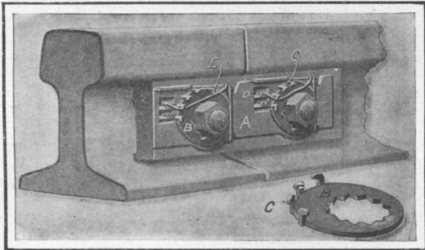
IMPROVED NUT LOCK.
