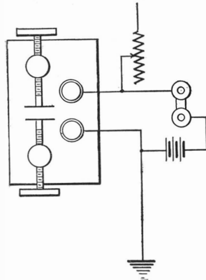
Fig. 2.—Electrical Connections of the Wireless Telegraph Detector.
