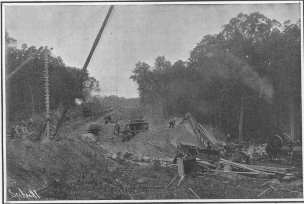
Mixing Concrete for Culvert Under the Aqueduct. Trench for Aqueduct is Seen in the Background.
