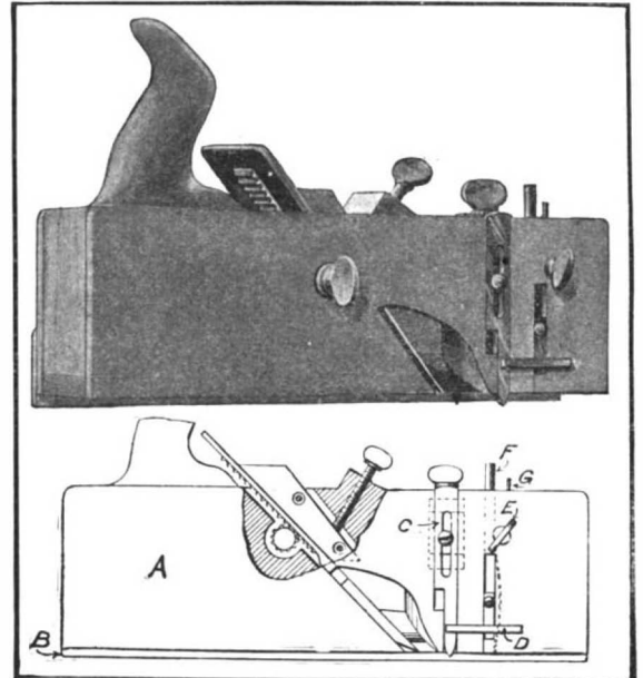
IMPROVED PLANE PROVIDED WITH ADJUSTABLE GUIDES.
