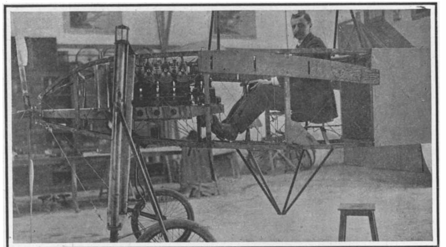
Front End of Body of the New Bleriot Aeroplane.
