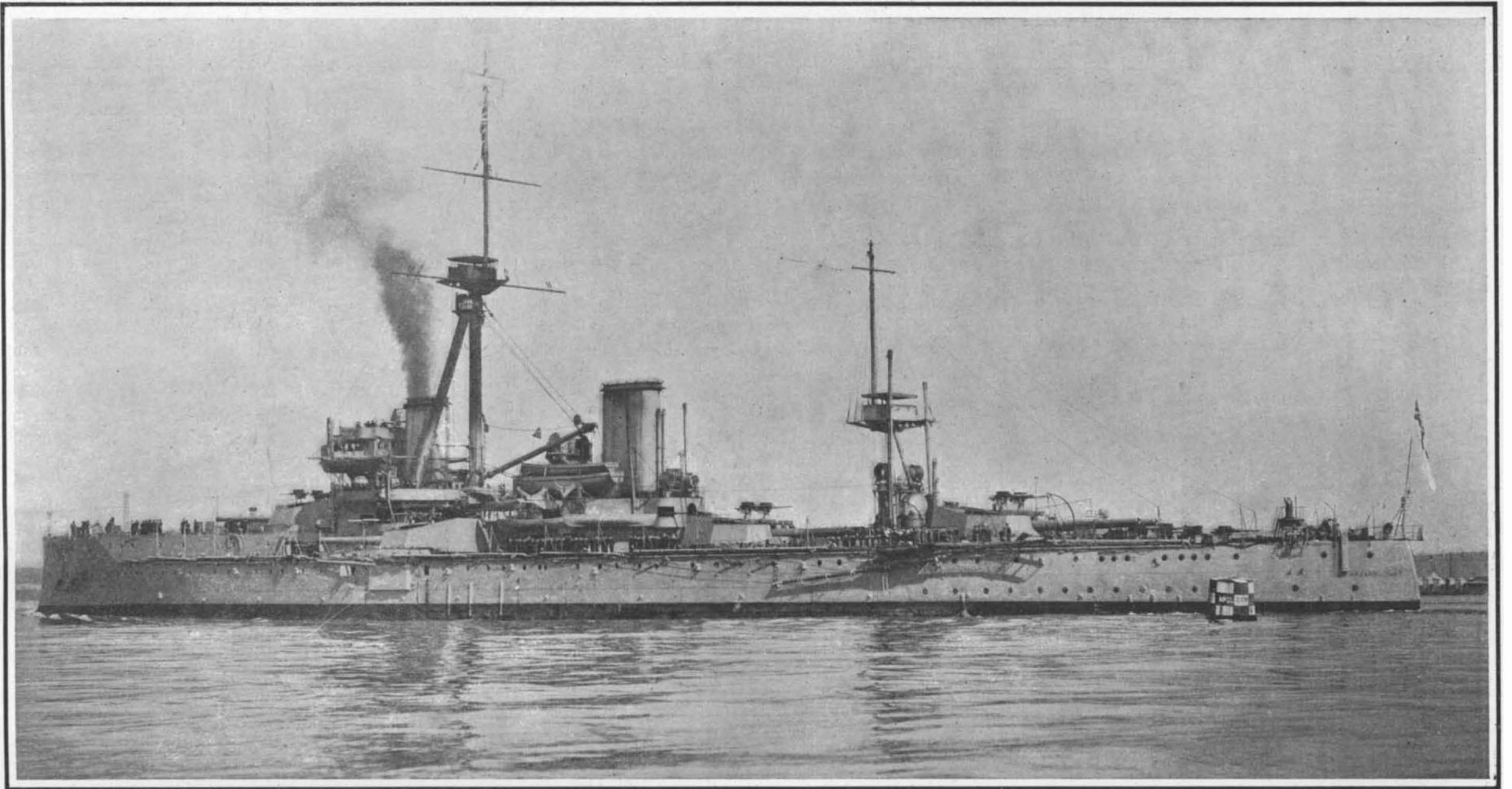
Displacement , 17,900 tons. Speed , 21 knots. Coal supply , 2,000 tons. Fuel oil , 400 tons. Armor : Belt, 11 inches; turrets, 11 inches; deck, 2\frac{3}{4} inches; side armor, 11 inches to 8 inches. Guns : Ten 45-caliber 12-inch; twenty-seven 12-pounders. Torpedo tubes , 5 submerged. Date , 1906.
