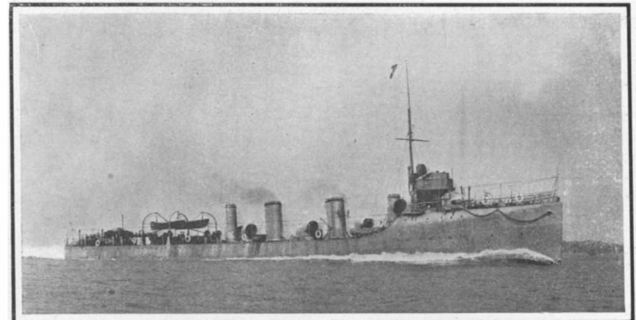
Displacement, 765 tons. Speed, 34 to 36 knots. Oil, 95 tons. Guns, three 12-pounders. Torpedo tubes, two. Date, 1907. Destroyer "Mohawk." Five Boats.
