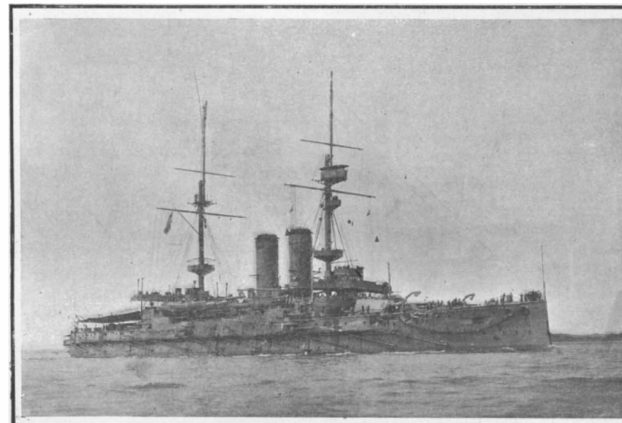
Displacement, 14,000 tons. Speed, 19.5 knots. Coal, 2,000 tons. Armor: belt, 7-inch; side, 7-inch; deck, 2 1/2-inch; barbette turrets, 6-inch to 11-inch; casemates, 6-inch. Guns: four 40-caliber 12-inch; twelve 45-caliber 6-inch; sixteen 12-pounders. Torpedo tubes, four. Date, 1901. Battleship "Russell." Five Ships.
