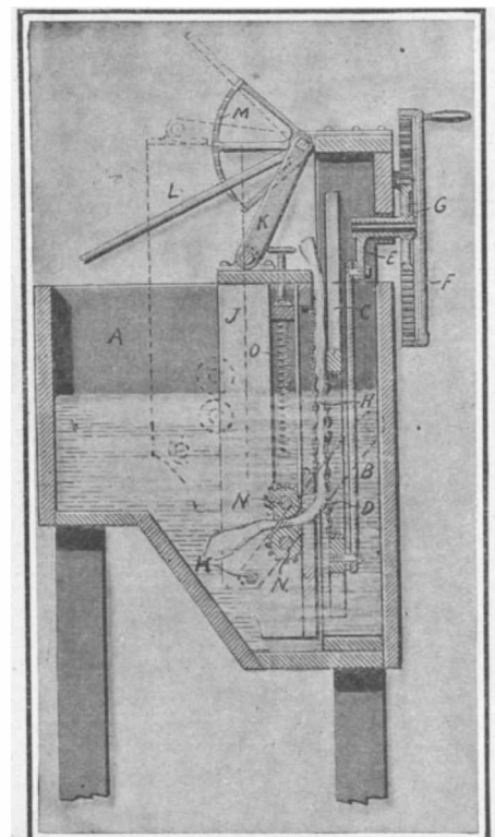
AN IMPROVED WASHING MACHINE.
