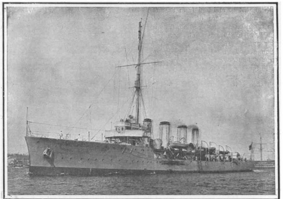
Displacement, 2,670 tons. Speed, 25.6 knots. Coal, 380 tons. Armor, 2-inch deck. Guns: ten 12-pounders; eight 3-pounders. Torpedo tubes, two. Date, 1904. Scout "Attentive." Six Ships.
