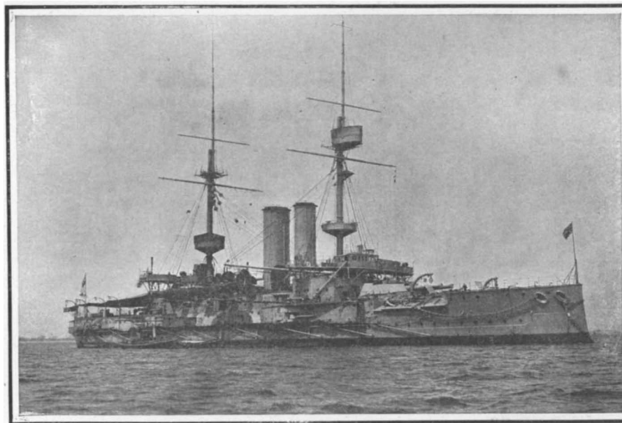
Displacement, 12,950 tons. Speed, 18.5 knots. Coal, 2,300 tons. Armor: belt, 6-inch; side, 6-inch; deck, 2 1/2-inch; barbette turrets, 8-inch to 12-inch; casemates, 5-inch. Guns: four 35-caliber 12-inch; twelve 40-caliber 6-inch; ten 12-pounders. Torpedo tubes, four. Date, 1898. Battleship "Ocean." Six Ships.
