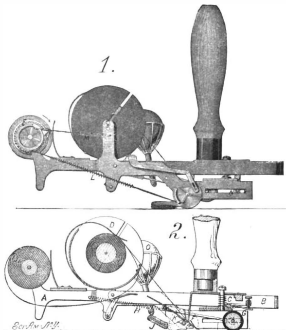
STAMP-AFFIXING MACHINE.
