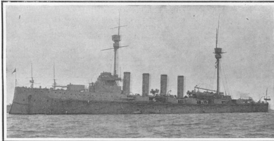
Displacement, 13,550 tons. Speed, 22.5 knots. Coal, 2,000 tons. Oil, 400 tons. Armor: belt, 6-inch; side, 6-inch; deck, 1-inch; barbette turrets, 6-inch to 7-inch; casemates, 6-inch. Guns: six 50-caliber 9.2-inch; four 50-caliber 7.5-inch; twenty-five 3-pounders. Torpedo tubes, three. Date, 1905. Armored Cruiser "Achilles." Four Ships.
