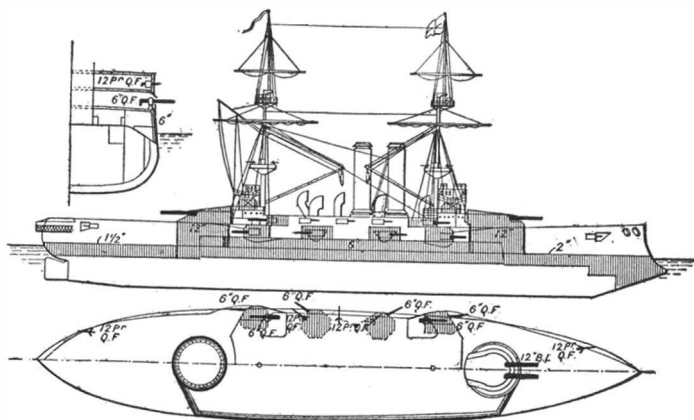
Displacement, 12,950 tons. Speed, 18.5 knots. Coal, 2,900 tons. Armor: belt, 6-inch; side, 6-inch; deck, 2 1/2-inch; barbettes turrets, 8-inch to 12-inch; casemates, 5-inch. Guns: four 35-caliber 12-inch; twelve 40-caliber 6-inch; ten 12-pounders. Torpedo tubes, four. Date, 1898.
