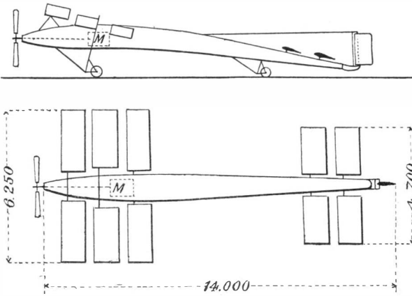
Side and Plan Diagrams of New Farman Aeroplane.
