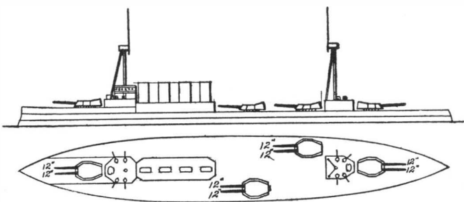
Displacement, 17,250 tons. Speed, 25 knots. Coal, 2,500 tons. Armor: belt, 7-inch; side, 6-inch; turrets, 9-inch. Guns, eight, 45-caliber, 12-inch. Date, 1907.
