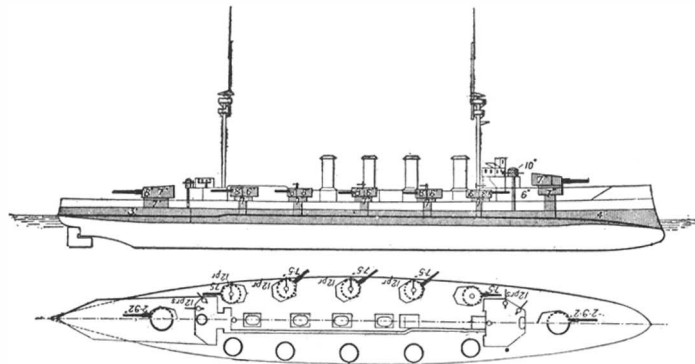
Displacement, 14,600 tons. Speed, 23 knots. Coal, 2,000 tons. Oil, 400 tons. Armor: belt, 6-inch; side, 6-inch; deck, 1-inch; turrets, 6-inch to 7-inch; Guns: four 50-caliber 9.2-inch; ten 50-caliber 7.5-inch; sixteen 3-pounders. Torpedo tubes, five. Date, 1906.
