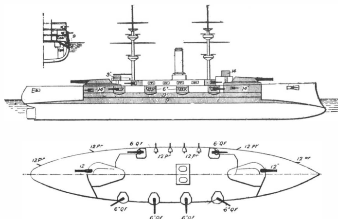
Displacement, 14,900 tons. Speed, 17.5 knots. Coal, 2,000 tons. Oil 400 tons. Armor: belt, 9-inch; barbettes turrets, 10-inch to 14-inch; deck, 4-inch; casemates, 6-inch. Guns: four 35-caliber 12-inch; twelve 40-caliber 6-inch; sixteen 12-pounders. Torpedo tubes, five. Date, 1895.
