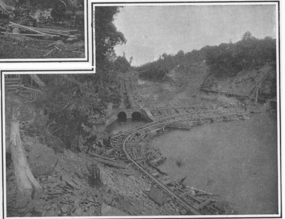
Site of Olive Bridge Dam, Which will be 220 Feet High and 5,650 Feet Long. The Two 8-Foot Pipes Are for By-passing the Esopus Creek During Construction.
