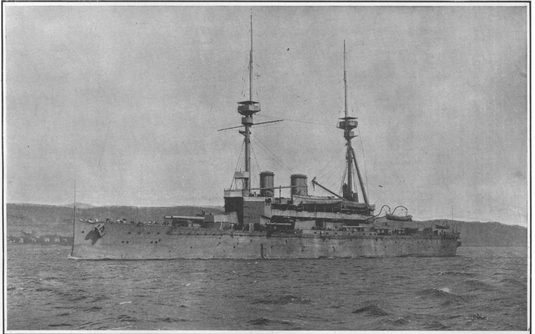
Displacement , 16,600 tons. Speed , 18.8 knots. Coal supply , 2,000 tons. Fuel oil , 400 tons. Armor : Belt, 12 inches; side armor, 7 inches; 12-inch turrets, 8 inches to 14 inches; 9.2-inch turrets, 7 inches; deck, 2 inches. Guns : Four 12-inch; ten 9.2-inch; fifteen 12-pounders. Torpedo tubes , 5. Date , 1906.
