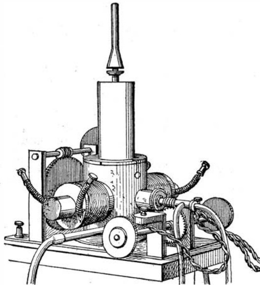
Fig. 1.—Poulsen Hydrogenic Arc Emitter.
