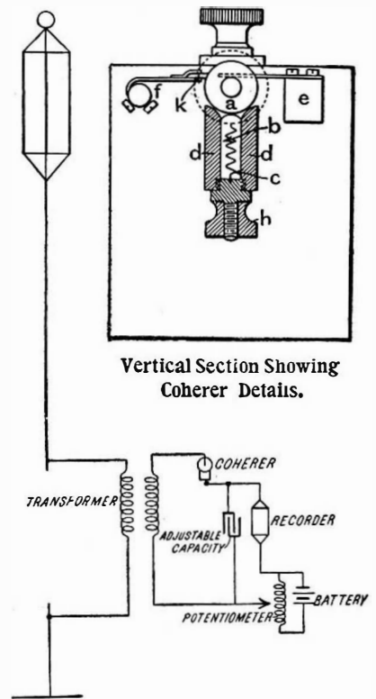
Diagram of the Sending Station.
