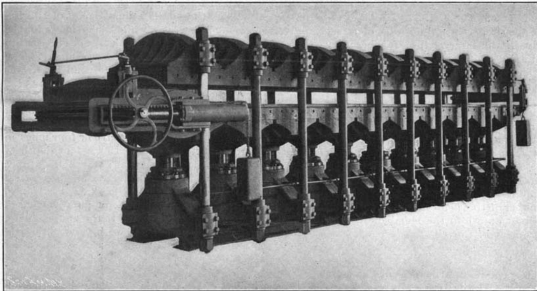
Hydraulic Belt-Press, in which Rubber Belting and Packing are Vulcanized Under Heavy Pressure.
