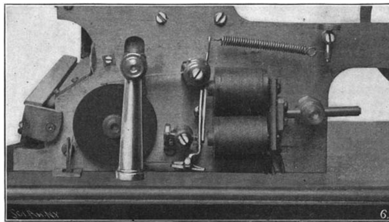
The Recorder.—Showing the manner of detaching a section of paper. A Portion of the Driving Mechanism.
