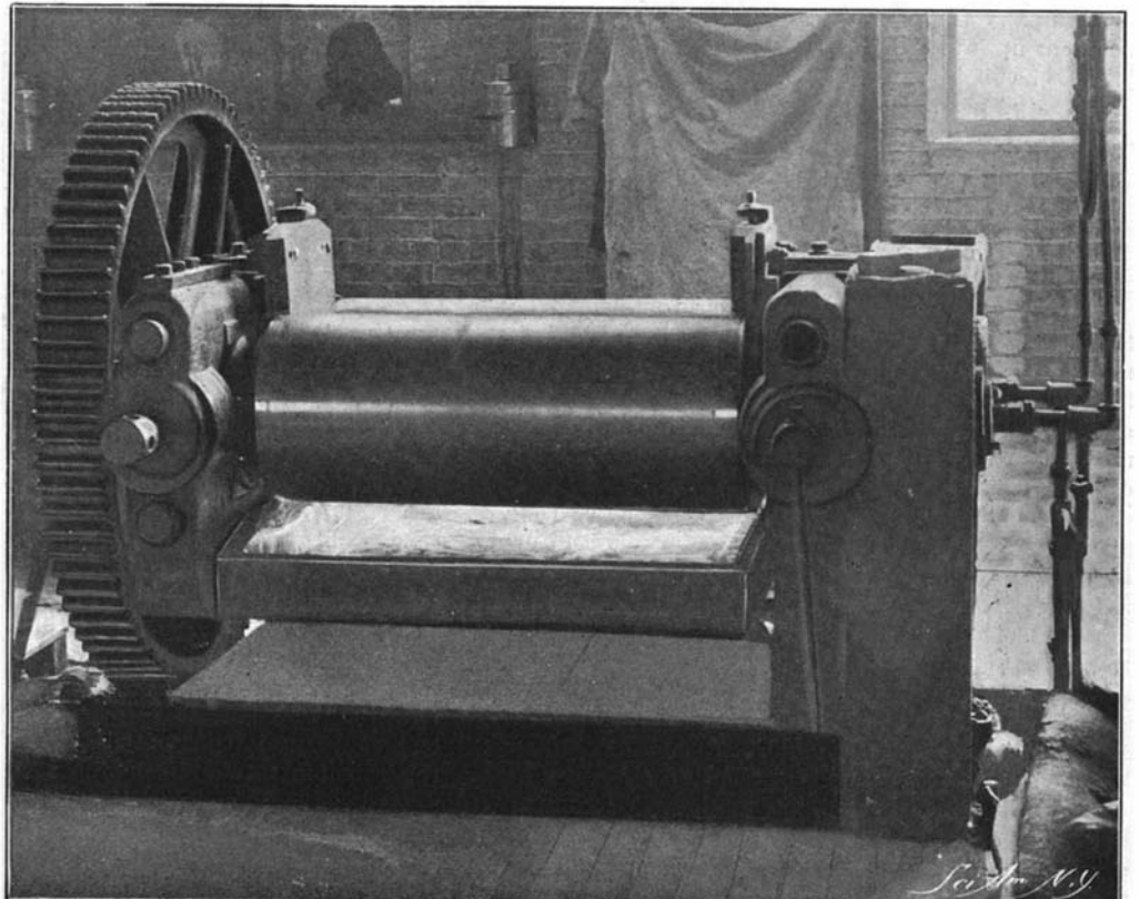
The "Mixer," in which the Rubber is Formed into a Homogenous Mass, and "Compounded" with Various Ingredients.
