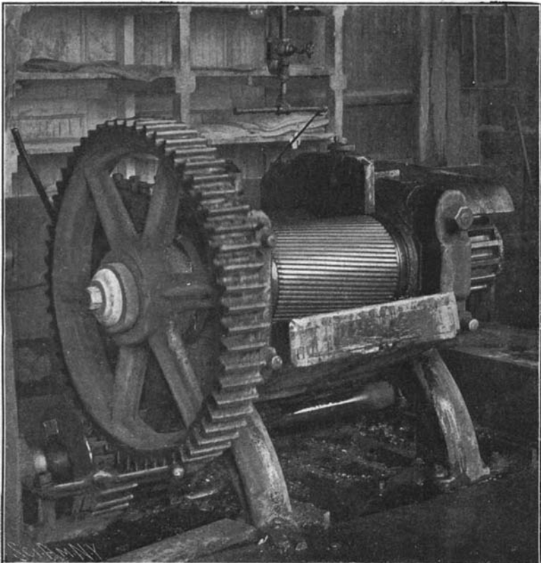
The "Washer," for Extracting the Sand and Other Impurities in the Crude Rubber.
