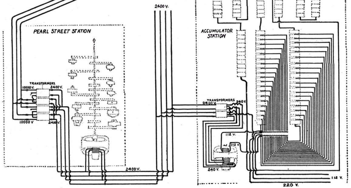
DIAGRAM OF THE HARTFORD ELECTRIC LIGHT AND POWER PLANT.
