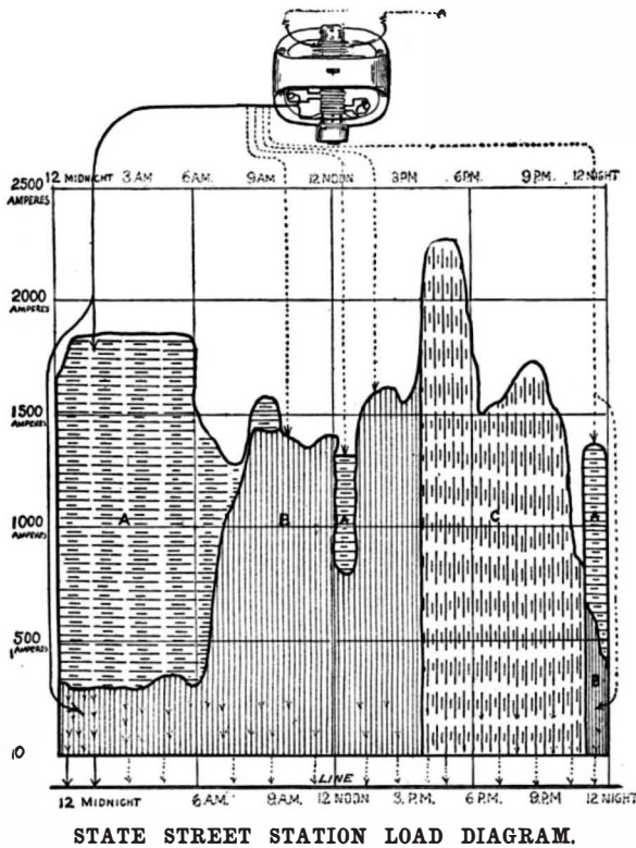
STATE STREET STATION LOAD DIAGRAM.
