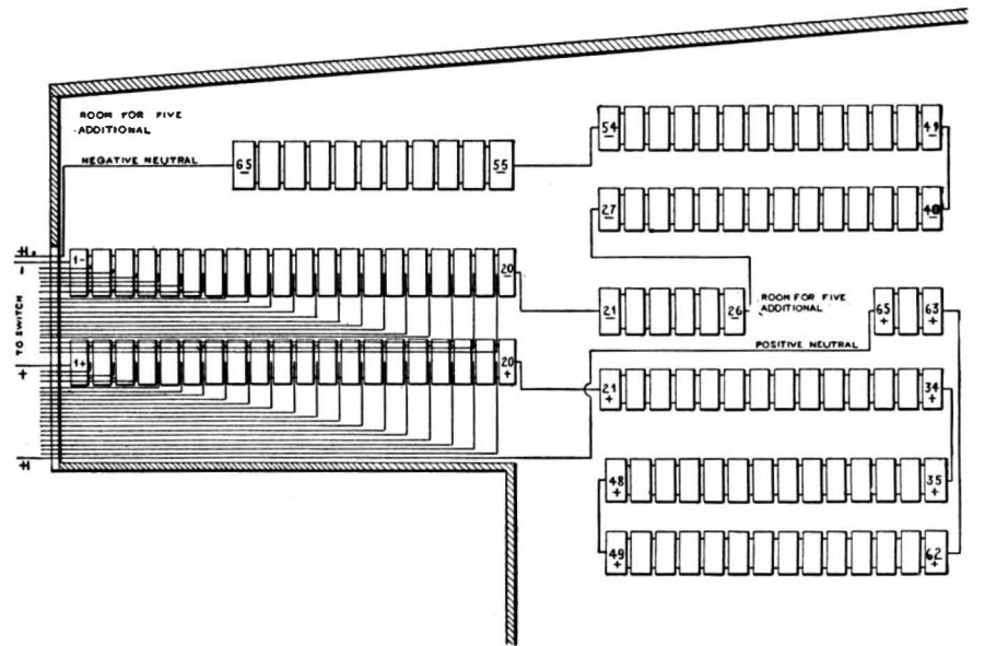
DIAGRAM OF STATE STREET BATTERIES.
