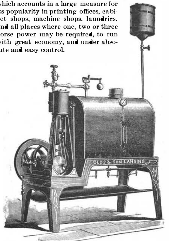
THE OLDS GASOLINE ENGINE.
