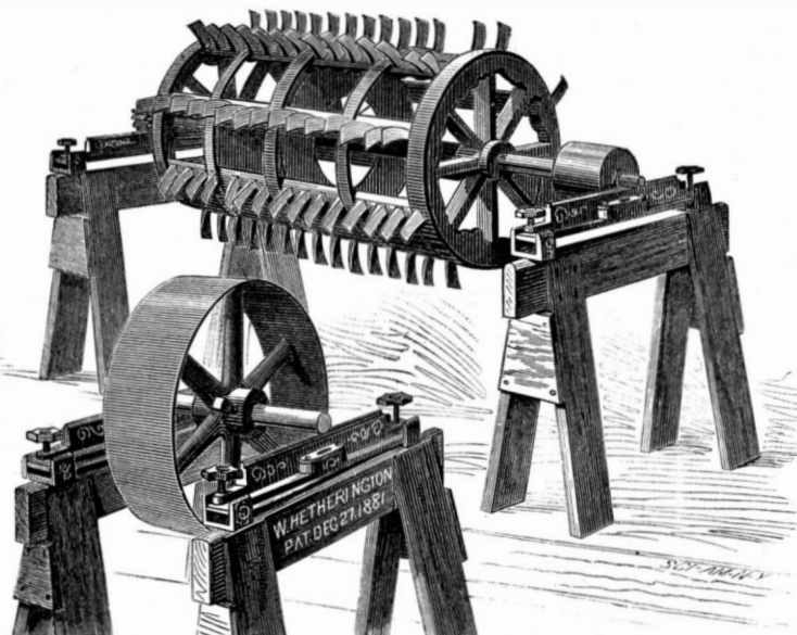
IMPROVED PARALLELS FOR BALANCING PULLEYS, ETC.
