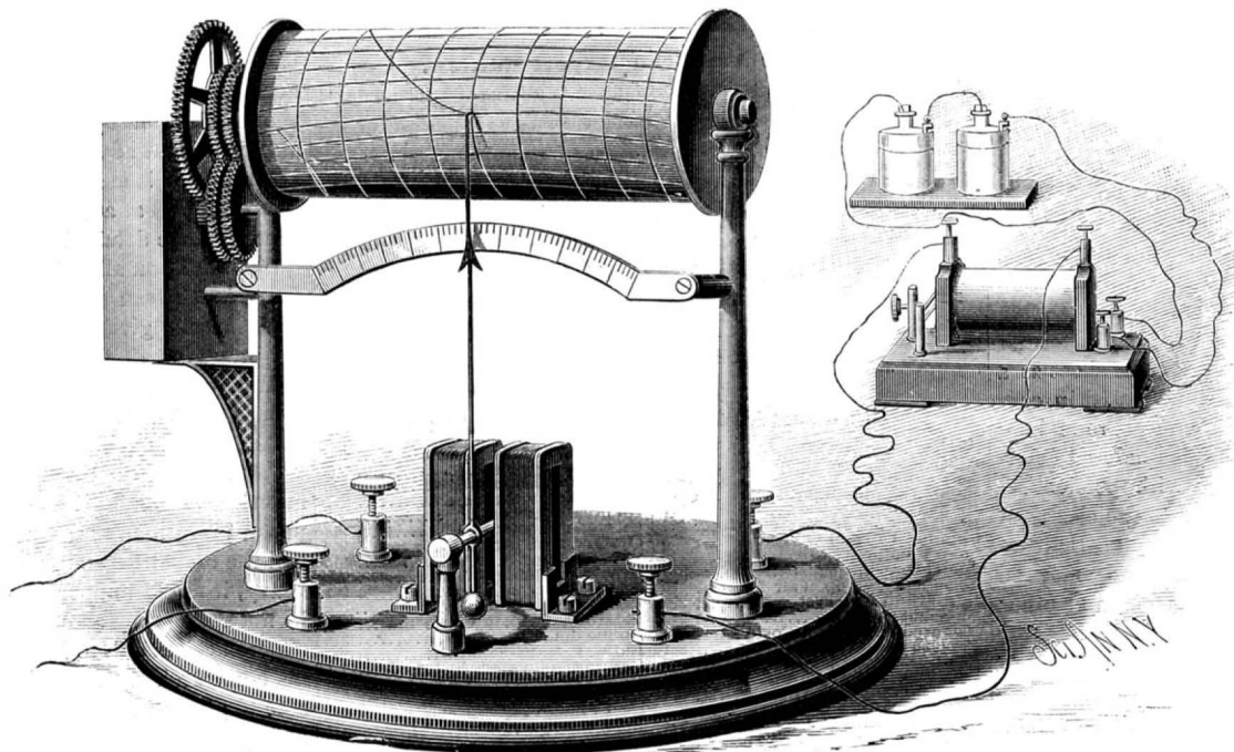
RECORDING GALVANOMETER.
