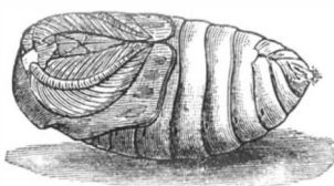
CHRYALIS COVERING OF THE POLYPHEMUS SILKWORM.
