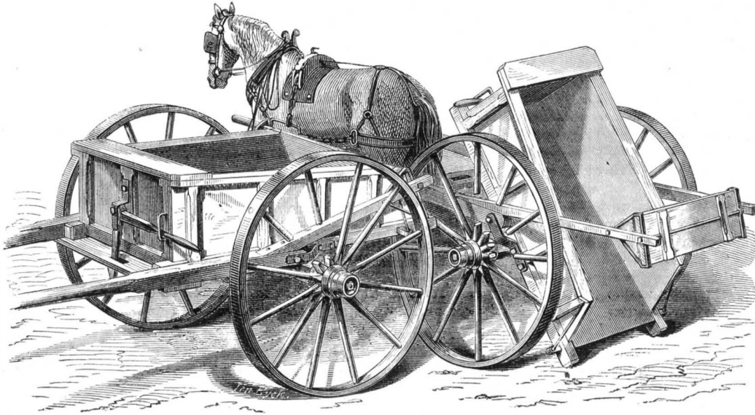
HAND'S IMPROVED DUMPING CART.
