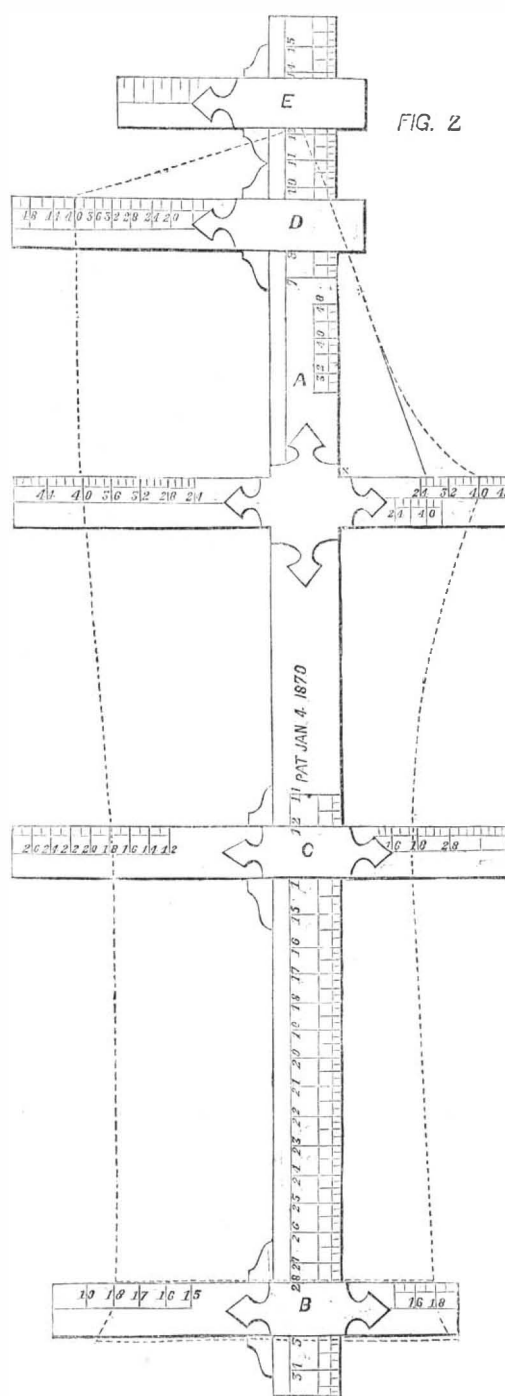
ORDWAY'S APPARATUS FOR DRAFTING CLOTHES.
