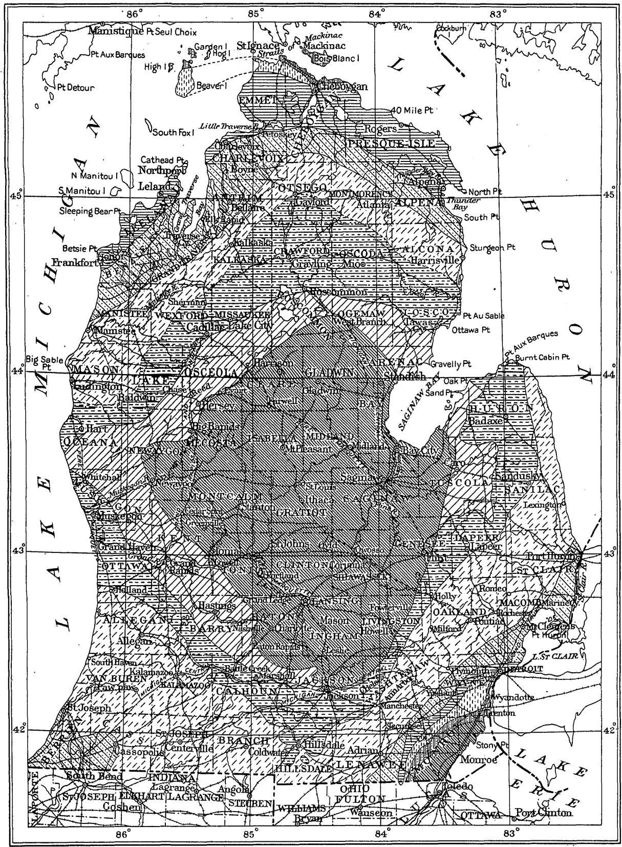
GEOLOGIC MAP OF THE LOWER PENINSULA OF MICHIGAN
