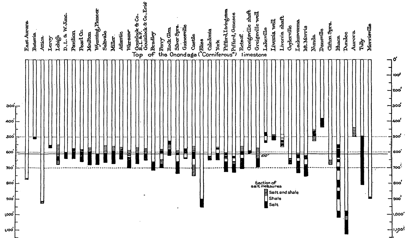
DIAGRAMMATIC SECTIONS SHOWING DEPTHS OF ROCK SALT BELOW THE TOP OF THE ONONDAGA ("CORNI-FEROUS") LIMESTONE IN NEW YORK. After F. J. H. Merrill.
