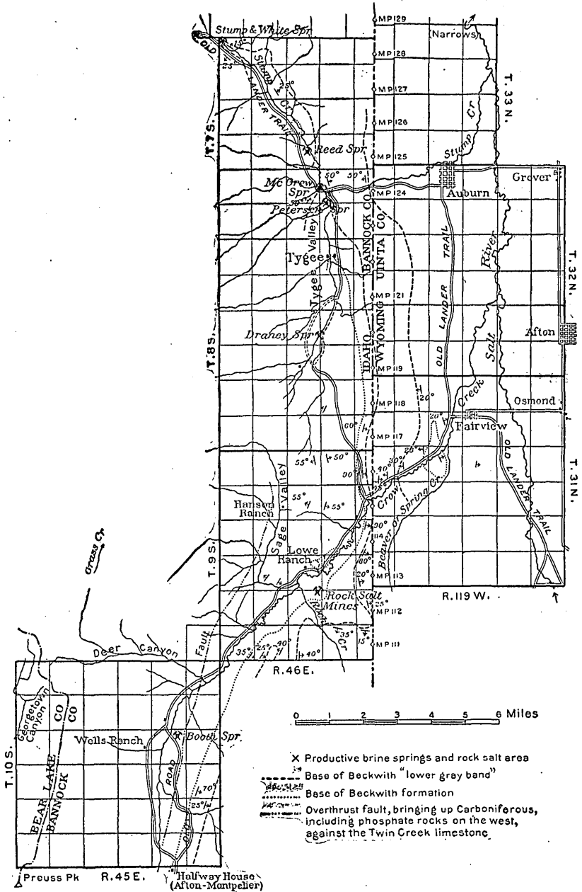
FIGURE 8.—Sketch geologic map of part of Idaho-Wyoming border country. (After C. L. Bregor, U. S. Geol. Survey Bull. 430, 1910.)
