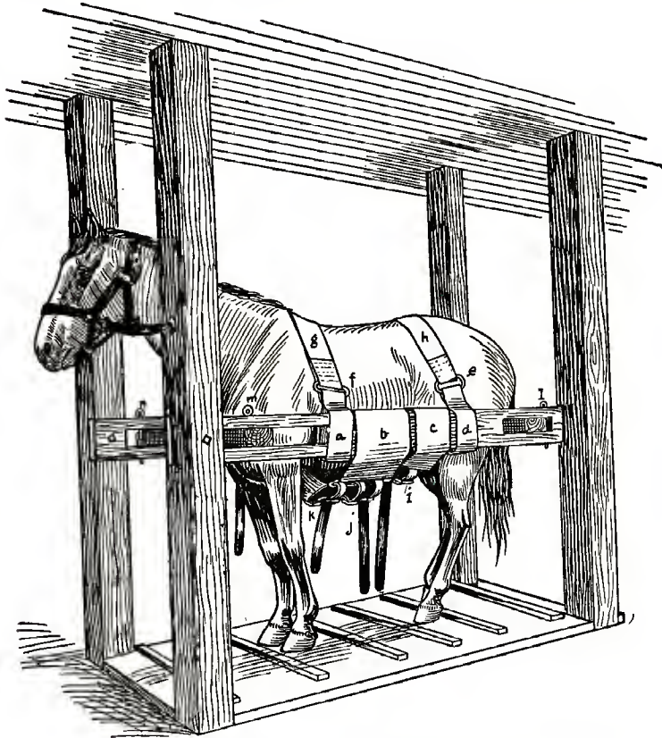
Fig. 63. McKillip Veterinary College Stocks with Horse Secured—Side View.
