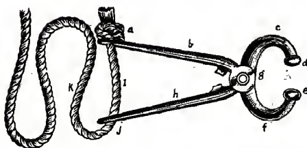
Fig. 234. American Nose Clamp With Rope.
