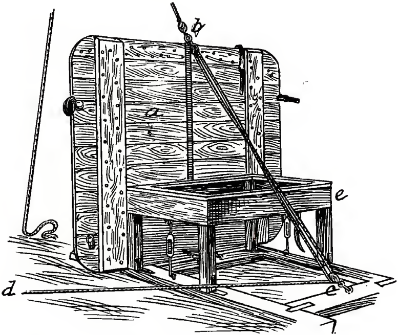
Fig. 194. Hodgson & Magee's Table, Upright Position, Back View.
