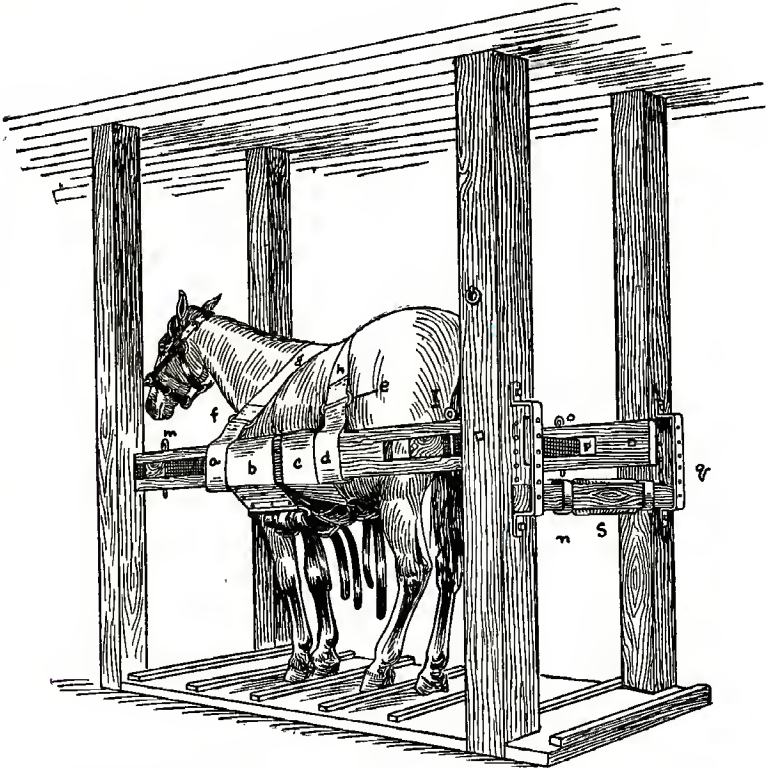
Fig. 64. McKillip Veterinary College Stocks—Side and Rear View.
