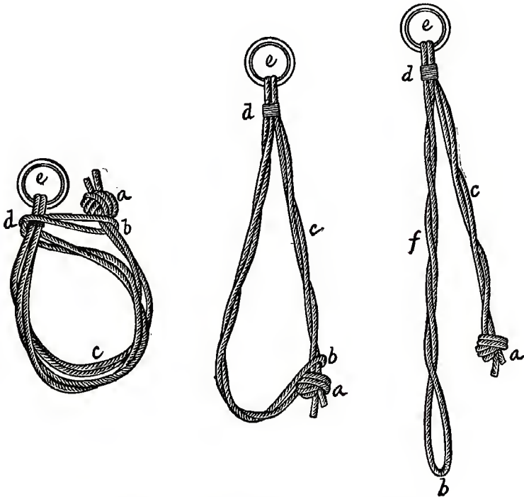
Fig. 85. Suykerbuyck's Rope Hobbles.
