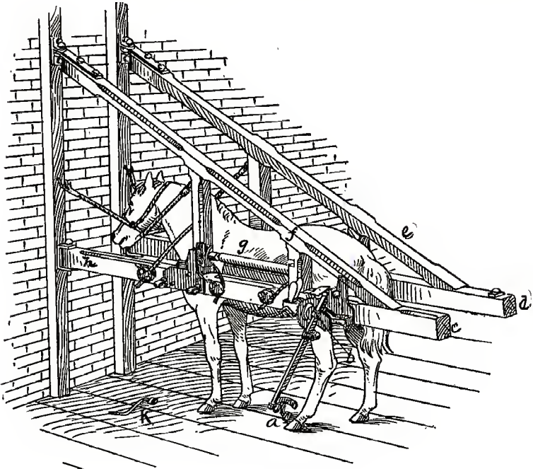
Fig. 61. Barcus Stocks.
