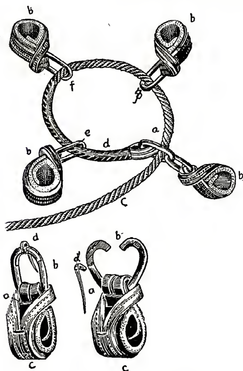
Fig. 92. Barnick's Hobbles.
