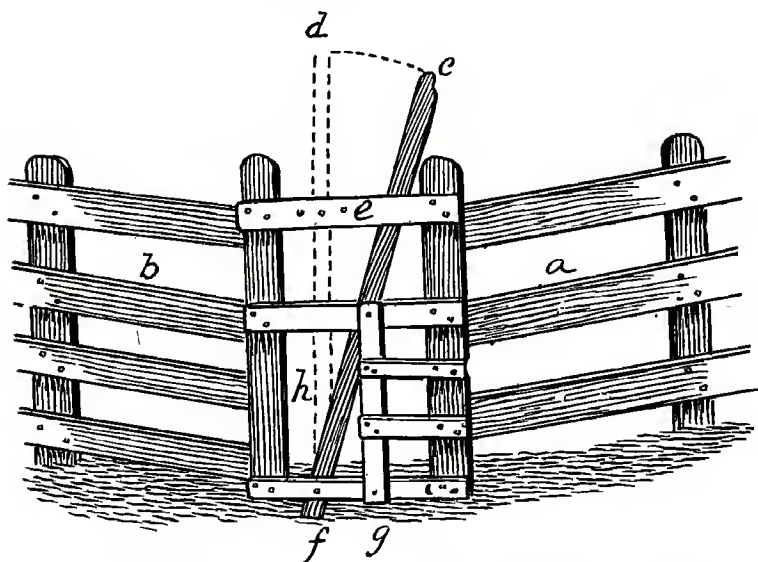
Fig. 316. Hog Catcher Open Ready for Reception of Animal.
