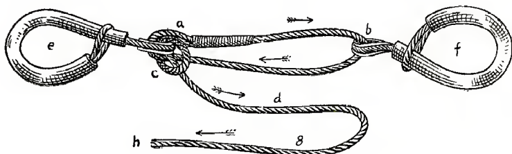
Fig. 82. James' Cross Hobbles.
