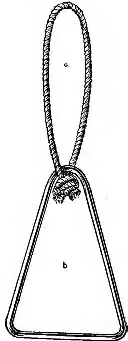
Fig. 4. Triangle Twitch.
