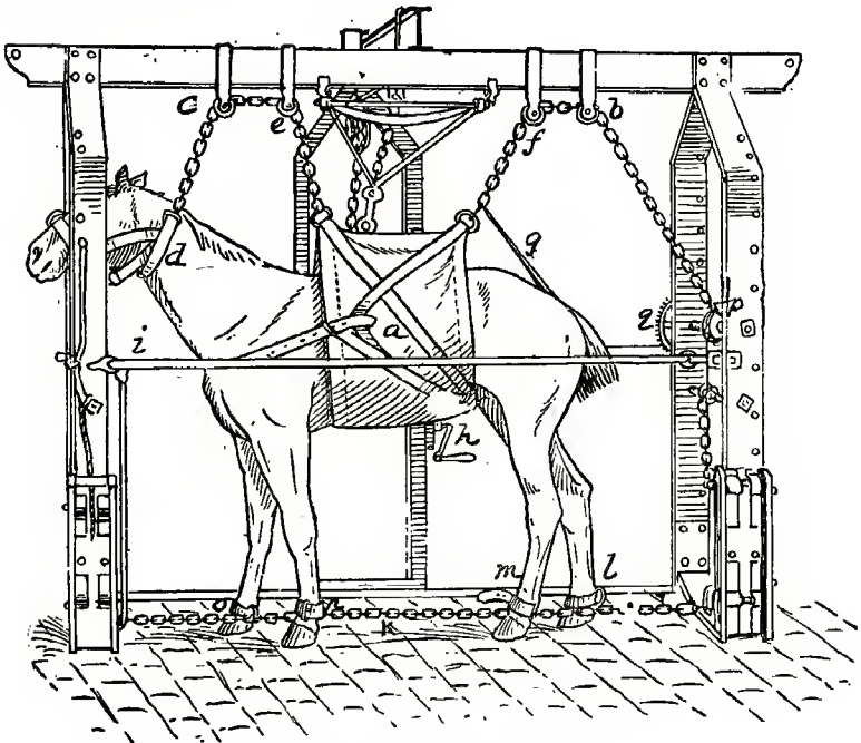
Fig. 67. Vinsot's Stocks.
