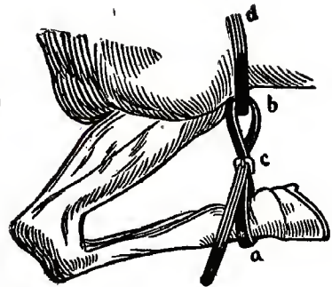
Fig. 137. Magner's Surcingle and Strap.
