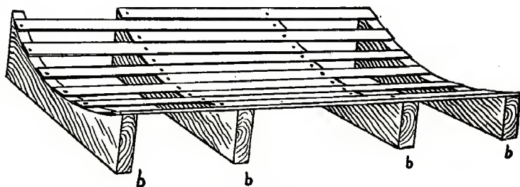
Fig. 285. Extension Grate.
