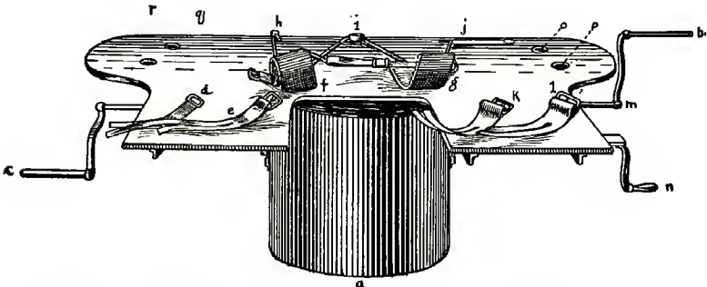
Fig. 209. Conkey's Equine Operating Table, Horizontal Position.
