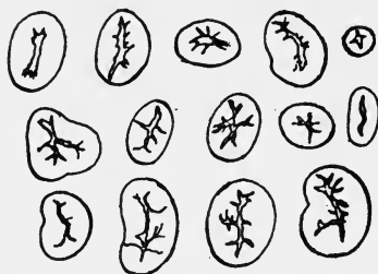
FIG. 37.—G, corn starch; H, rice starch; I, corn dextrin; J, pea starch; K, cassava starch; L, bean starch. Explanation in text.
