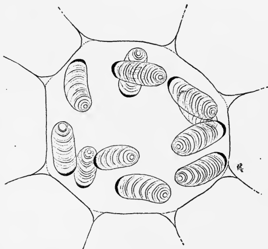
FIG. 35.—Cell of Pellionia Daveauana , showing starch-grains. The black, crescent-shaped body on the end of each grain is the leucoplast . Greatly enlarged. (Gager.)
