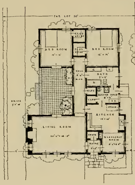
FLOOR PLAN SCALE \frac{1}{8} " = 1'-0"
