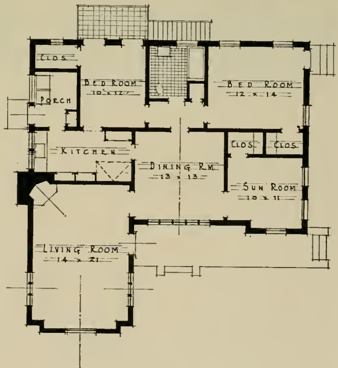
RESIDENCE LOS ANGELES, CALIFORNIA M. P. WILKINSON ARCHITECT
