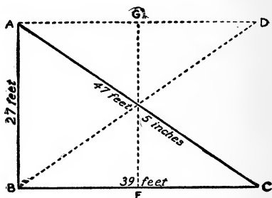
How to mark out a tennis court
