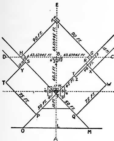
How to lay out a baseball field
