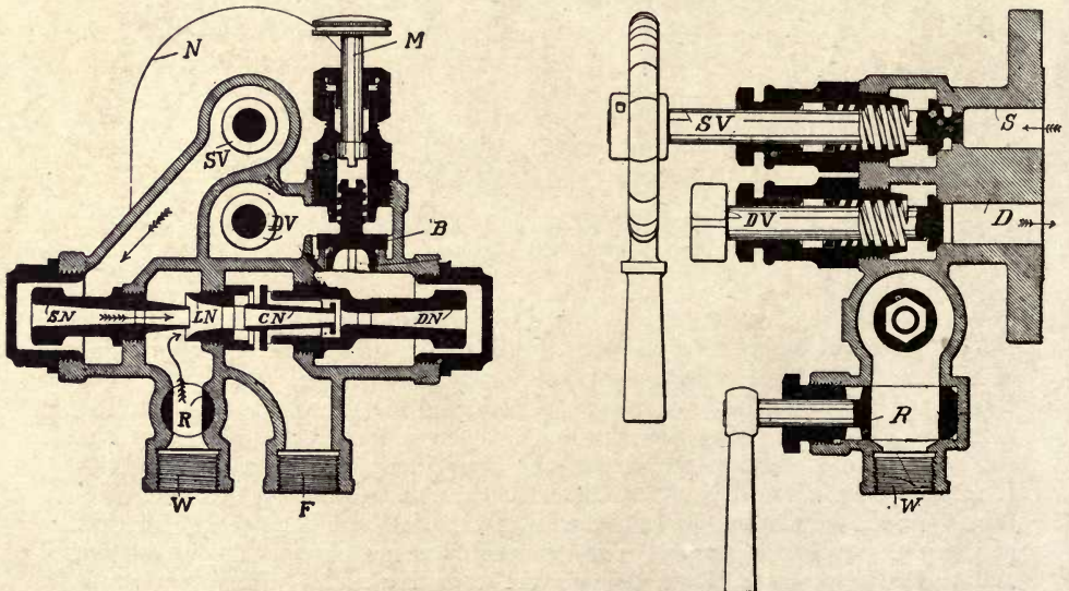
Fig. 135.—White's Injector for Traction Engines.
