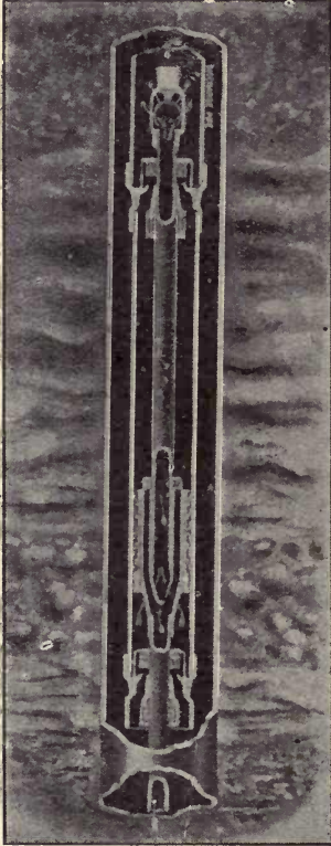
Fig. 72.—Double-acting Single Plunger Borehole Pump
