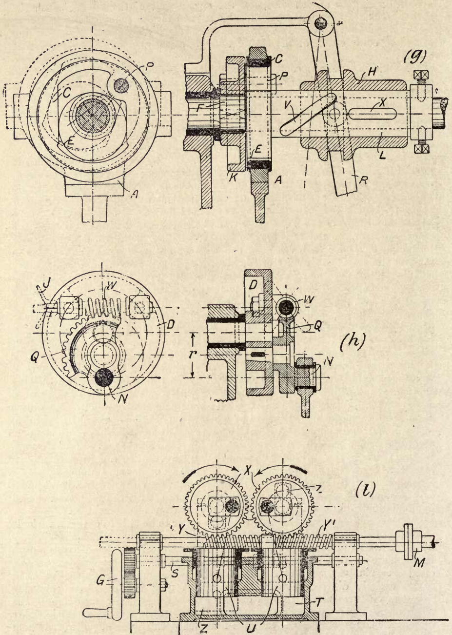
Fig. 223.—Examples of Compound Eccentric, Crank, and Plunger Mechanisms for obtaining Variable Delivery at Constant Speeds.
