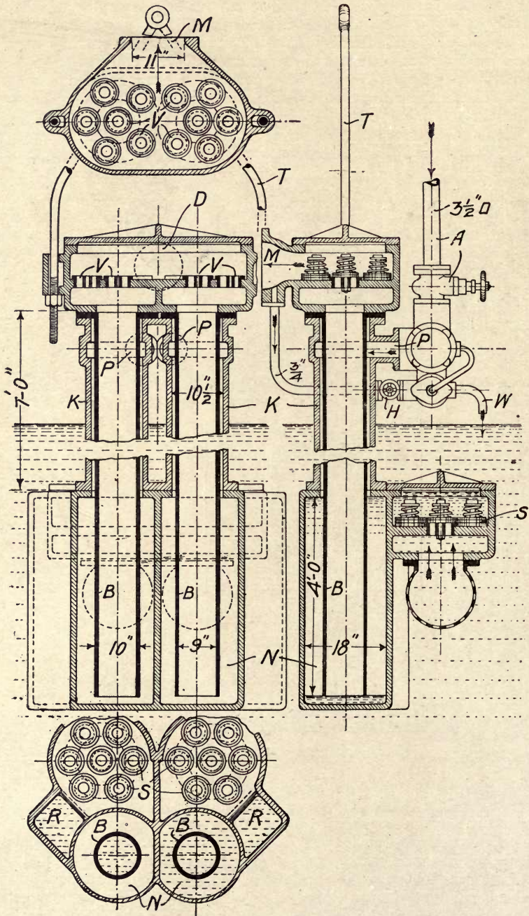
Fig. 189.—Twin Air-displacement Pump. Capacity, 30,000 Gallons per Hour.
