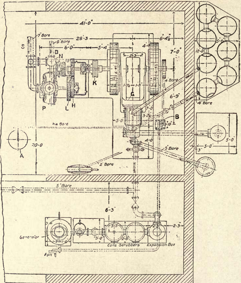
Fig. 220.—Half-plan Arrangement of Gas-power Pumping Plant.
