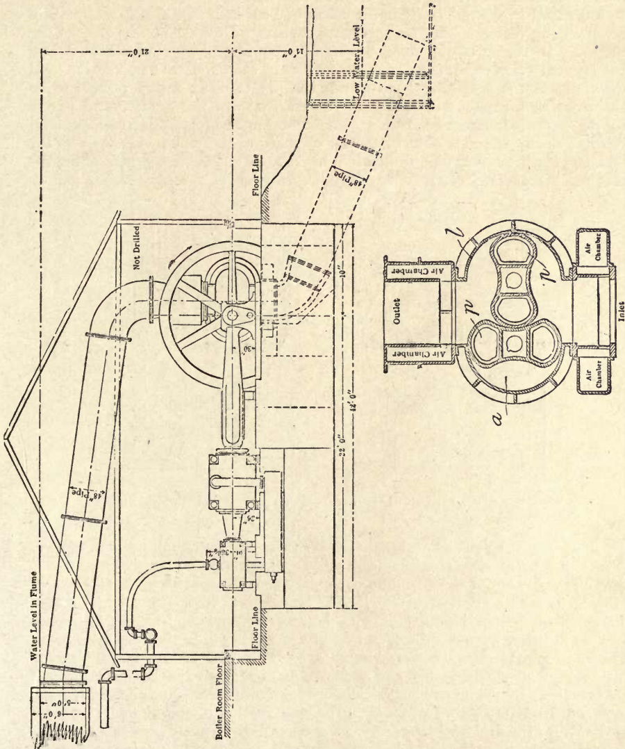
Fig. 243.—Cross-sections of Connersville Cycloidal Rotary Pump, and Irrigation Pumping Plant of 108,000 gallons per minute capacity
