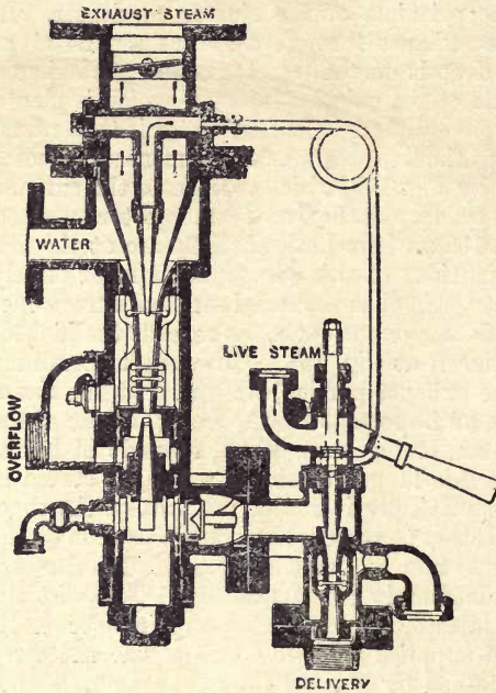
Fig. 140.—Section showing Arrangement of Holden and Brooke's Compound Non-lifting Exhaust Injector.
