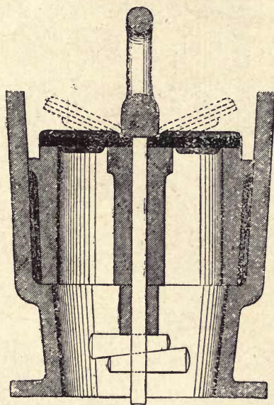
Fig. 52.—Butterfly Leather Flap Foot Valve.
