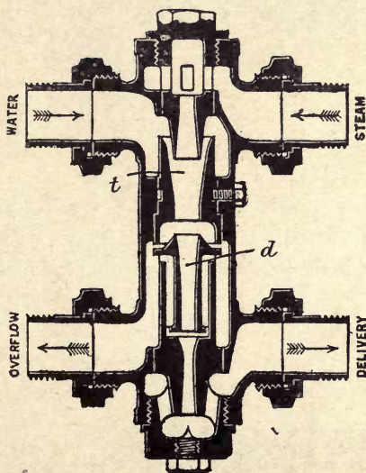
Fig. 136.—Gresham Injector (Re-starting).
