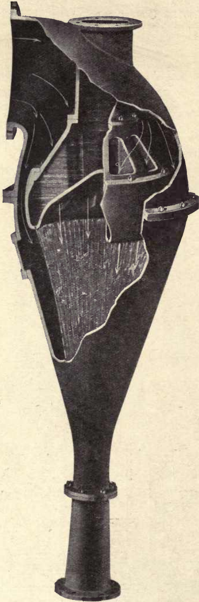
Fig. 151.—Worthington Barometrical Condenser Ejector.
