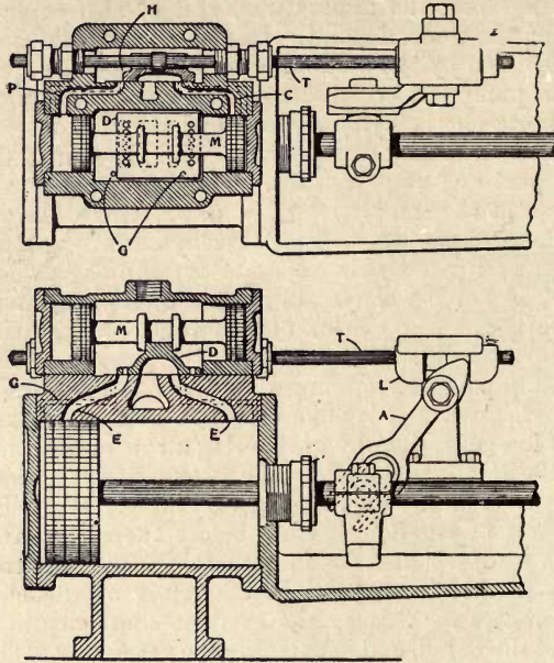
Fig. 90.—Section of Steam Cylinder, showing Distribution used in the Burnham Simplex Direct-acting Pump.
