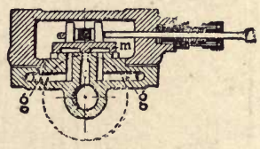
Fig. 105.—Simplex Pump with Gland-packed Plunger
