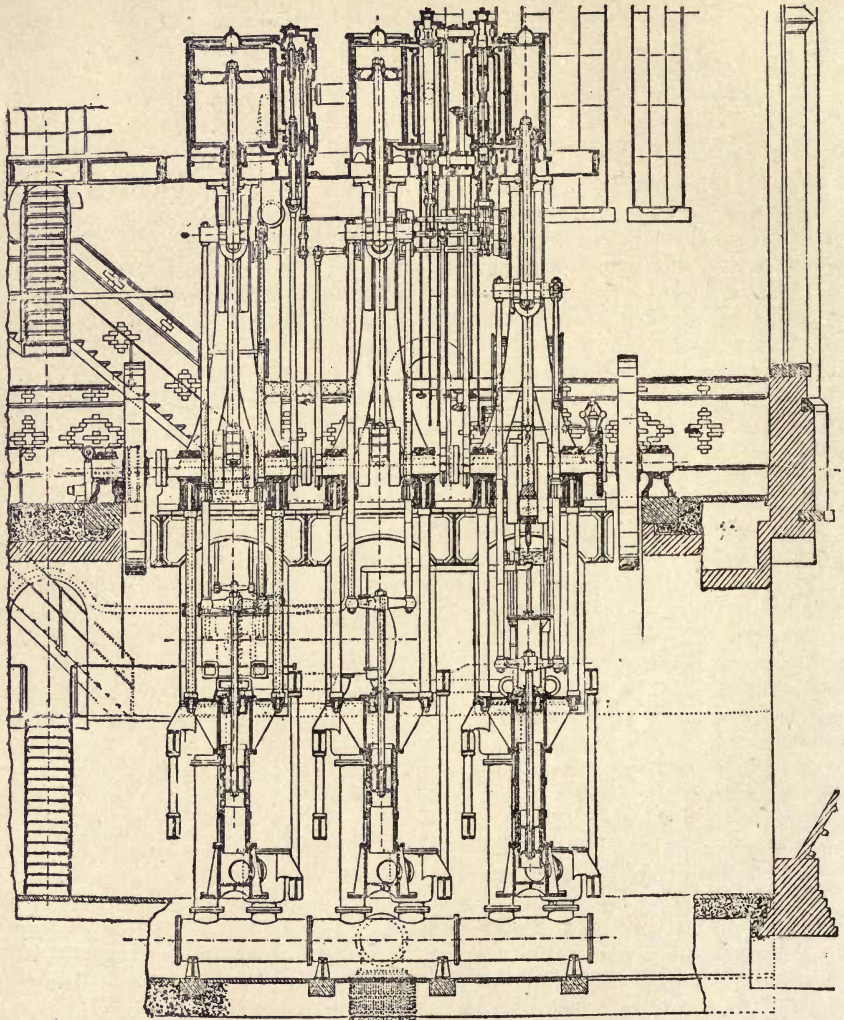
Fig. 16.—Sectional Elevation of Triple-expansion Three-crank Pumping Engine, with Double-acting High-lift Pumps, at the Riverdale Station, Hampton-on-Thames.
