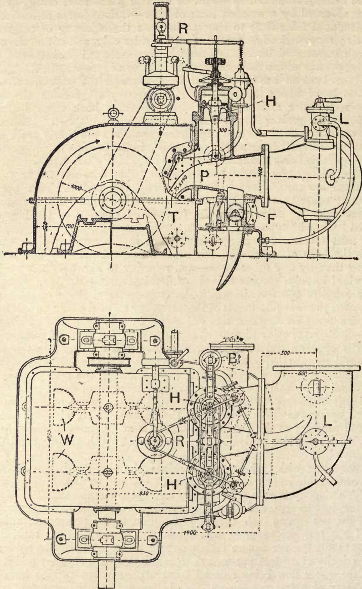
Fig. 335.—Double Wheel Impulse Turbine. Supplied by Escher-Wyss & Co., to develop 500 H.P. on a pressure head of 260 feet at St. Gall, Switzerland.
