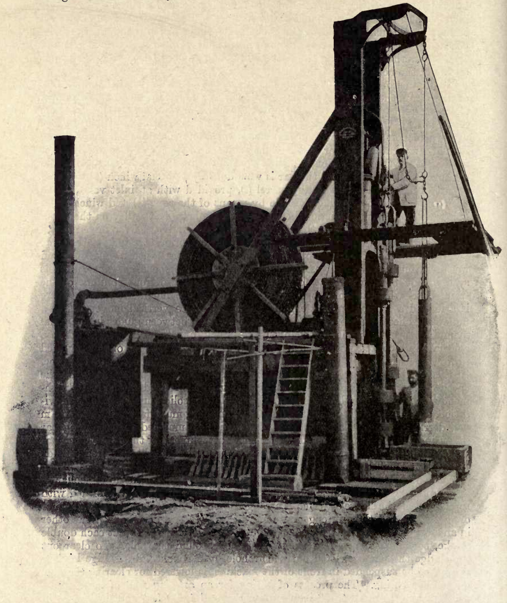
Fig. 60.—Flat Rope Boring Machine, showing Steam-driven Jumping Action.
