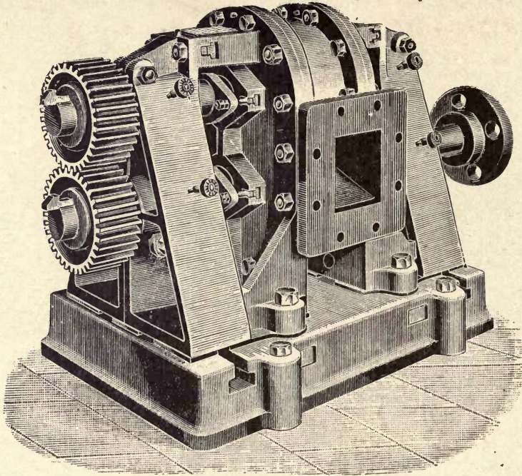
Fig. 239.—“Drum” Pump for delivering 30 Tons or Masse-cuite per Hour against a Head of 90 Feet.
