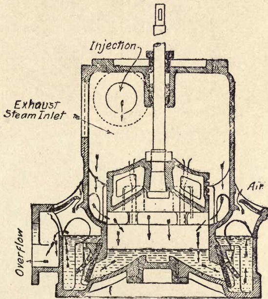
Fig. 160.—Stott Valveless Plunger Air Pump (Benn's Patent).
