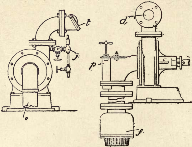
Fig. 282.—Starting Arrangements for Centrifugal Pumps.
