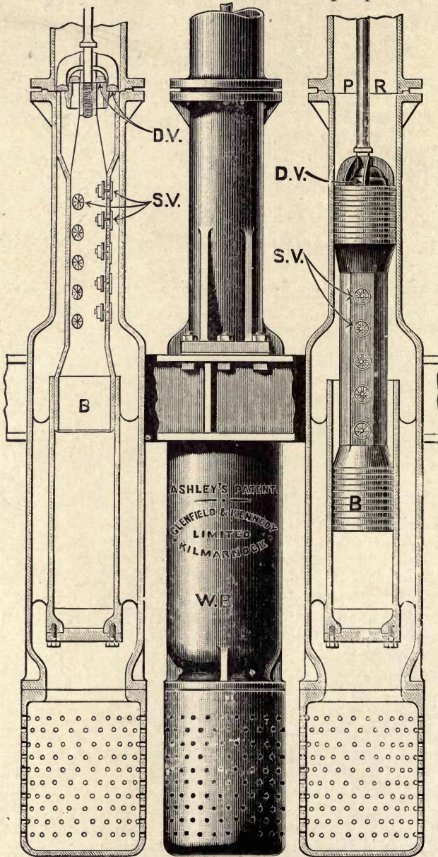
Fig. 36.—Ashley Deep-level Pump.
