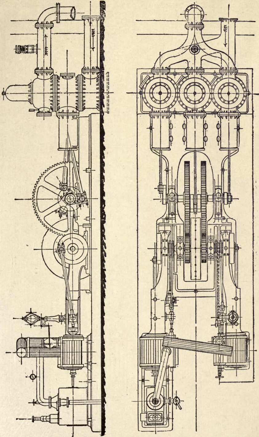
Fig. 12.—Three-throw Force Pumps for Shoreham.
