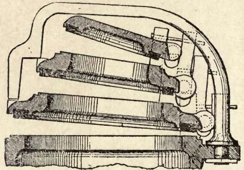
Fig. 50.—Pyramidal Arrangement of Rubber-faced Hinged Valves.
