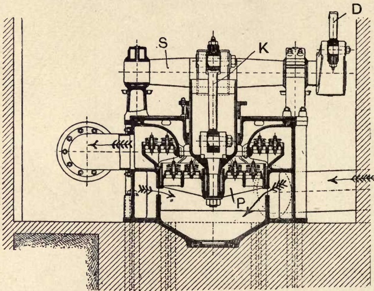
Fig. 155.—Bucket Piston Air Pump without Foot Valves, for Triple-expansion Borsig Engine and Jet Condenser.
