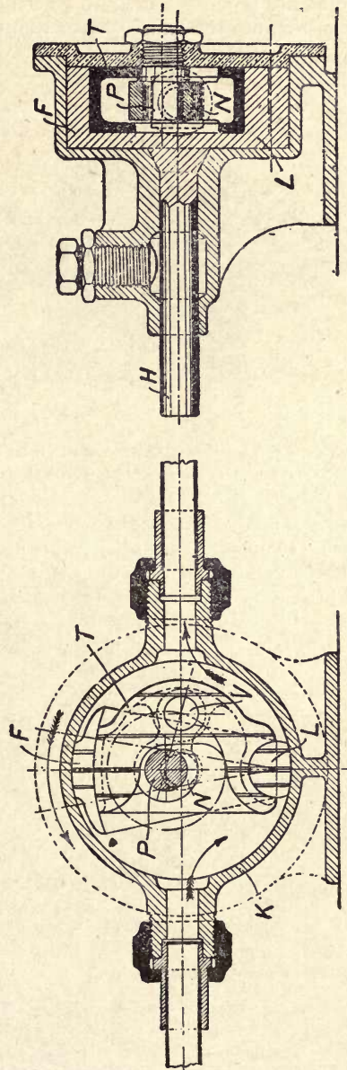
Fig. 250.—Sectional Elevations of Albany Positive Rotary Pump. Lamplough's Patent.
