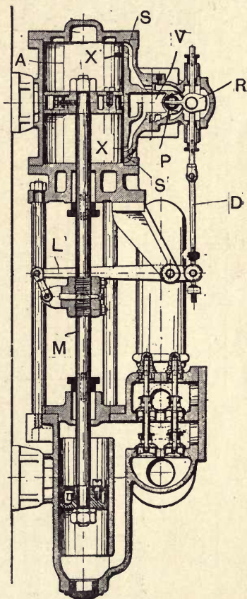
Fig. 85.—Sectional Elevation of Simplex Feed Pump.
