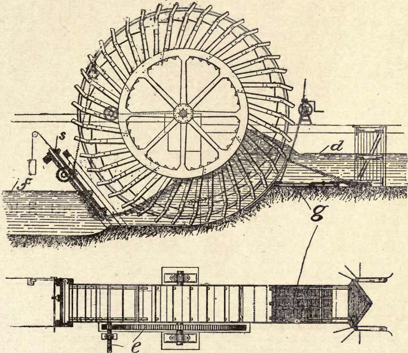
Fig. 261.—30 by 5 Feet Scoop-wheel Pump. Capacity, 5 tons per Second against head of 5 to 6 feet.
