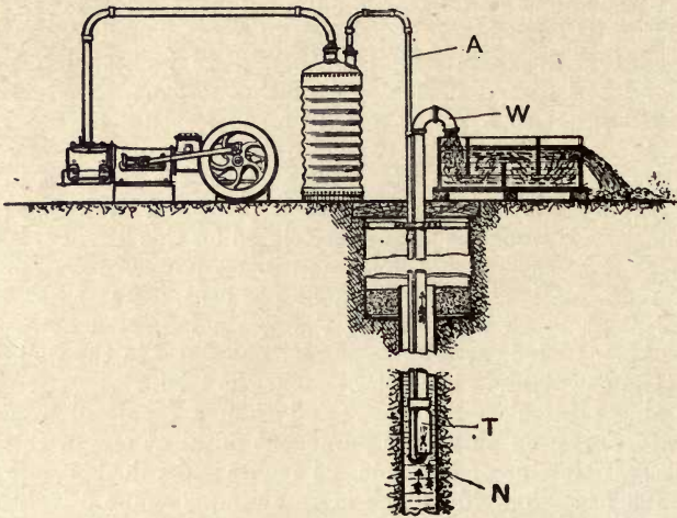
Fig. 76.—Air-lift Pump at the Kent Waterworks.
