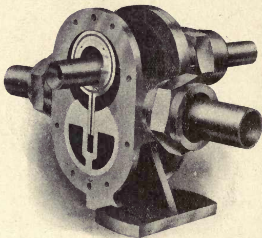
Fig. 254.—Lamplough-Albany Rotary Pump, with Eccentric Action Displacer.
