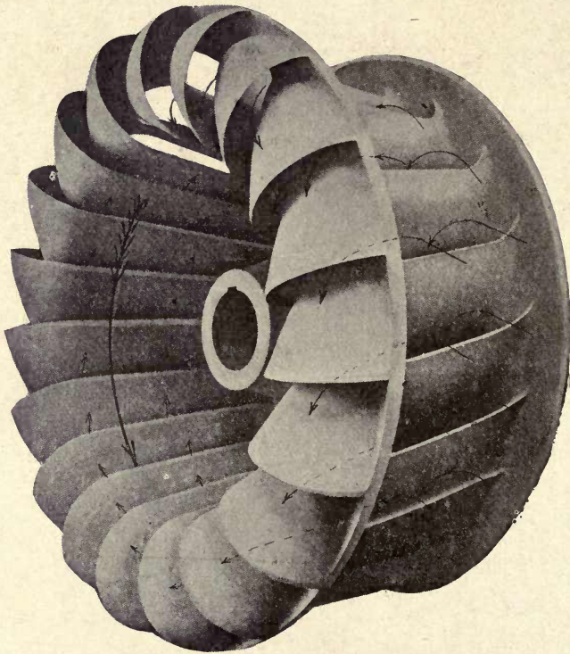
Fig. 305.—Theodore Bell Radial-axial-flow Impeller Wheel for Pressure Heads, 5 to 50 feet.
