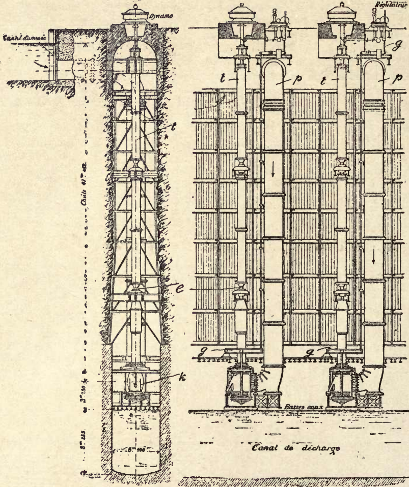
Fig. 327.—General Arrangement of Installation of Ten Piccard Outward-flow Turbines. At the No. 1 Power house of the Niagara Falls Power Company, each to develop 5,000 H.P. at 250 revolutions, under a pressure head of 136 feet.
