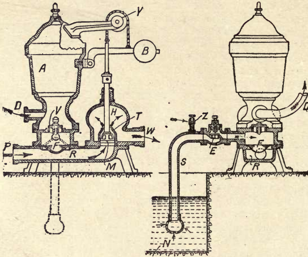
Fig. 183.—Belien-Durozoi Hydraulic Ram, with Diaphragm Pump.
