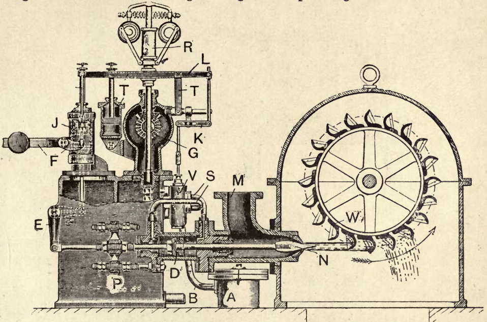
Fig. 338.—Sectional Elevation of "Gilbert Gilkes" Hydraulic Compensating Governor for Jet Action High-pressure Turbines.
