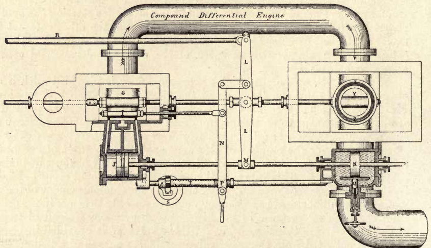
Fig. 29.—Sectional Elevation and Plan of Davey Compound Differential Engine, showing the Action of the Valve Gear.
