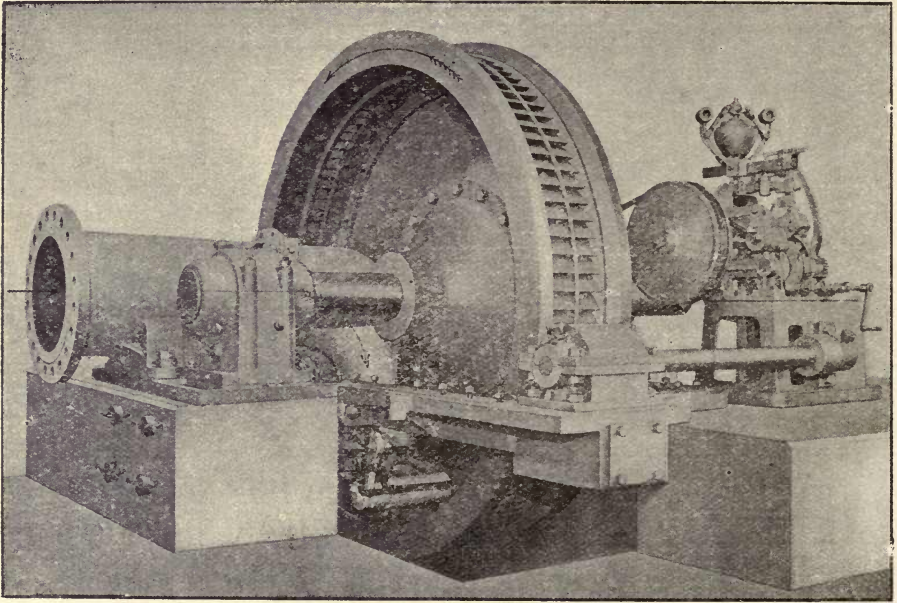
Fig. 332.—Piccard Double Jet Outflow Turbine. To develop 1,580 H.P. at 500 revolutions and fall of 1,340 feet, showing ratchet relay governor and impeller with hood removed.
