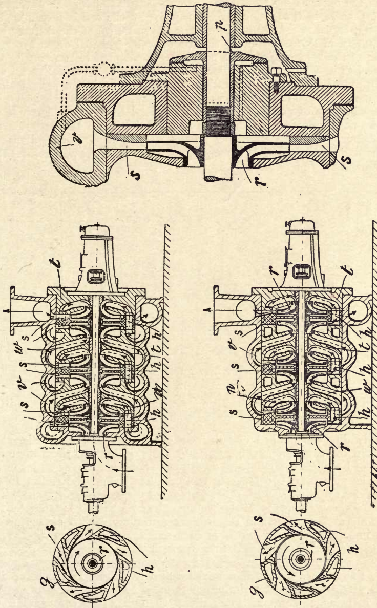
Fig. 285.—Sectional Elevations of Six-stage Sulzer High-lift Centrifugal Pump.
