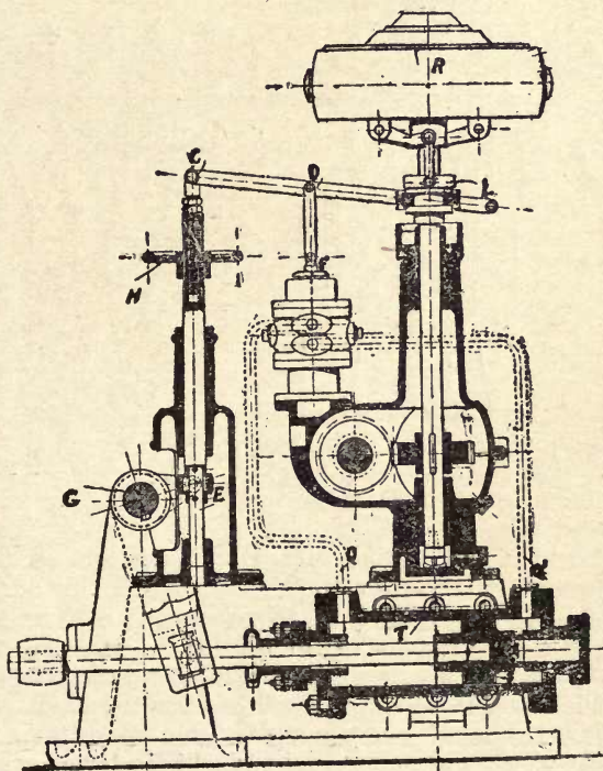
Fig. 318.—Ganz Hydraulic Relay Governor for Reaction Turbines.
