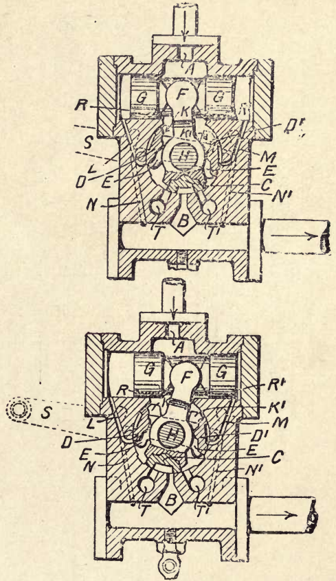
Fig. 95.—Detail of Woodeson Distributing Valve.
