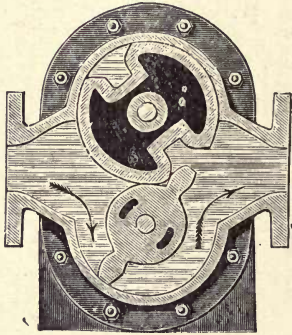
Fig. 240.—Section of the “Drum” Pump
