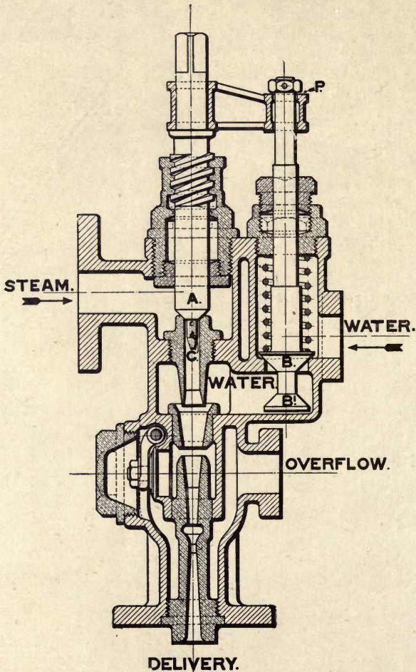
Fig. 128.—Single Movement Brooke Injector, with Fixed Steam Nozzle and Synchronous Action Regulating Valves.
