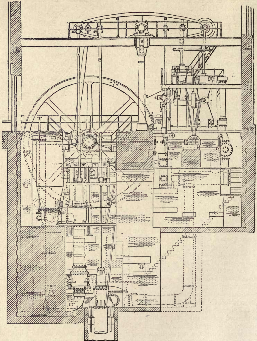
Fig. 10.—Compound Rotative Beam Pumping Engine, with Bucket and Plunger, High and Low-lift Pumps, for Chatham Waterworks.
