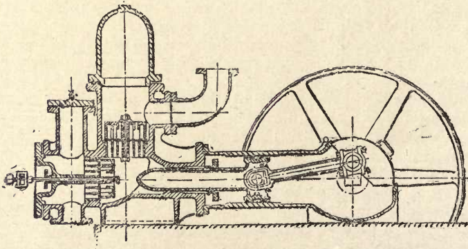
Fig. 210.—Sectional Elevation of One of a Pair of 8\frac{1}{2} \times 12 inch Oddie-Barclay Mine Pumps. Capacity, 600 Gallons per Minute.
