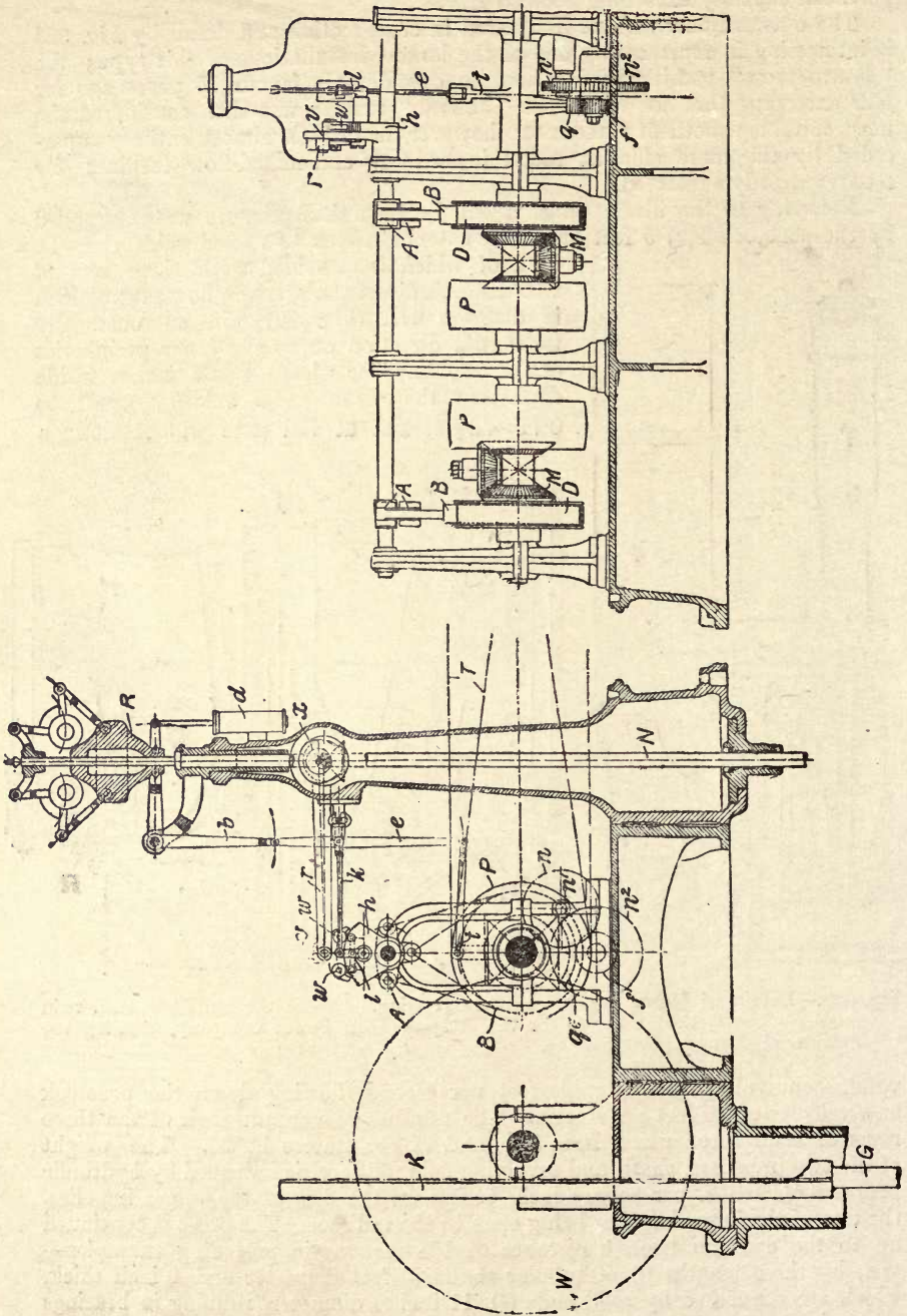
Fig 329.—Sectional Elevations of Relay Governor for the 5,500 H.P. Outward-flow Turbines at Niagara Falls.
