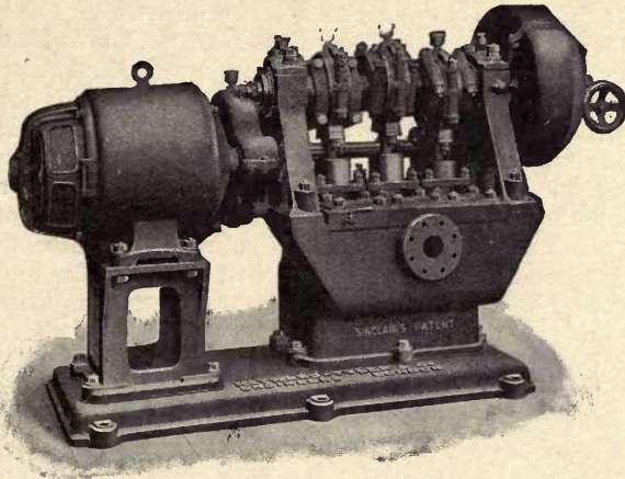
Fig. 227A.—Hayward-Tyler 5-inch by 4-inch Variable Delivery Pump, feeding Boilers at 200 Lbs. Pressure with Water 190°.
