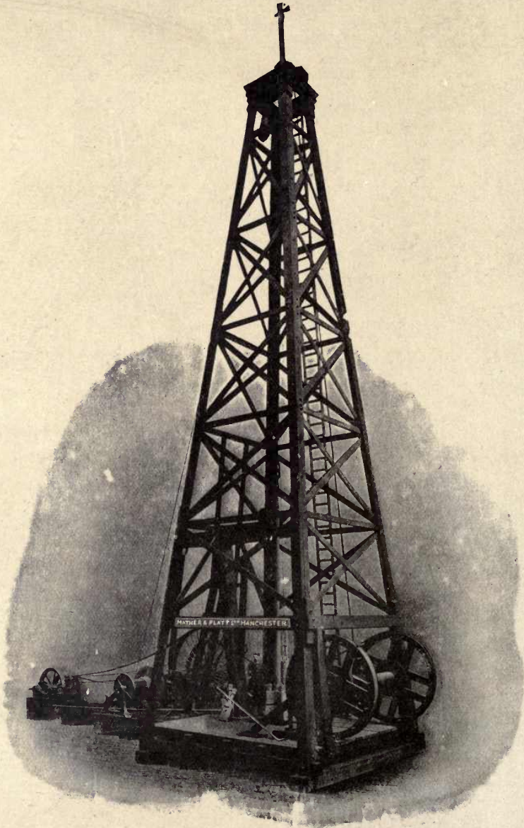
Fig. 59.—General View of Round Rope Well Boring Plant.
