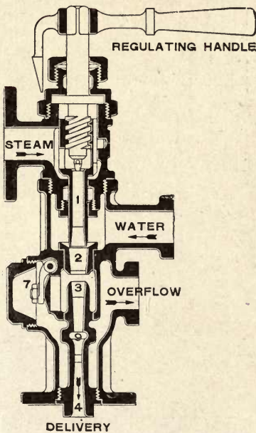
Fig. 126.—Brooke One-movement Injector, with Sliding Steam Nozzle.
