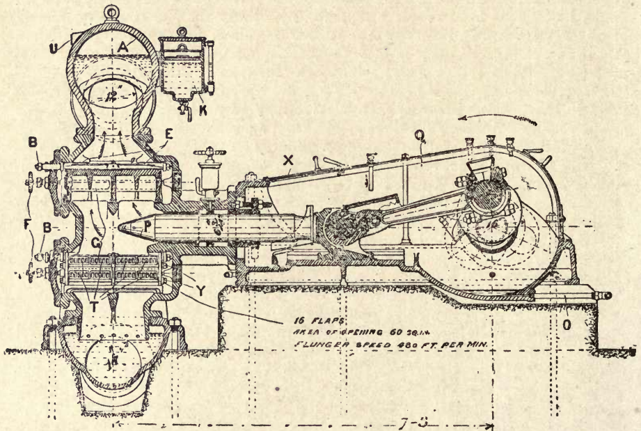
Fig. 215.—Sectional Elevation of Fraser and Chalmers' 3-throw Pump with Gutermuth Valves.
