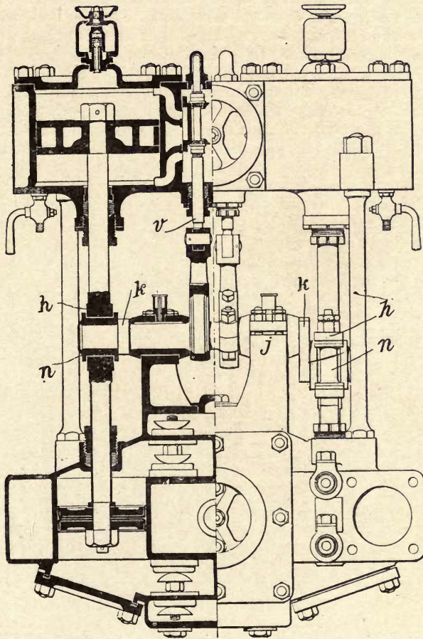
Fig. 197.—Merryweather Fire Pump (without Flywheel).
