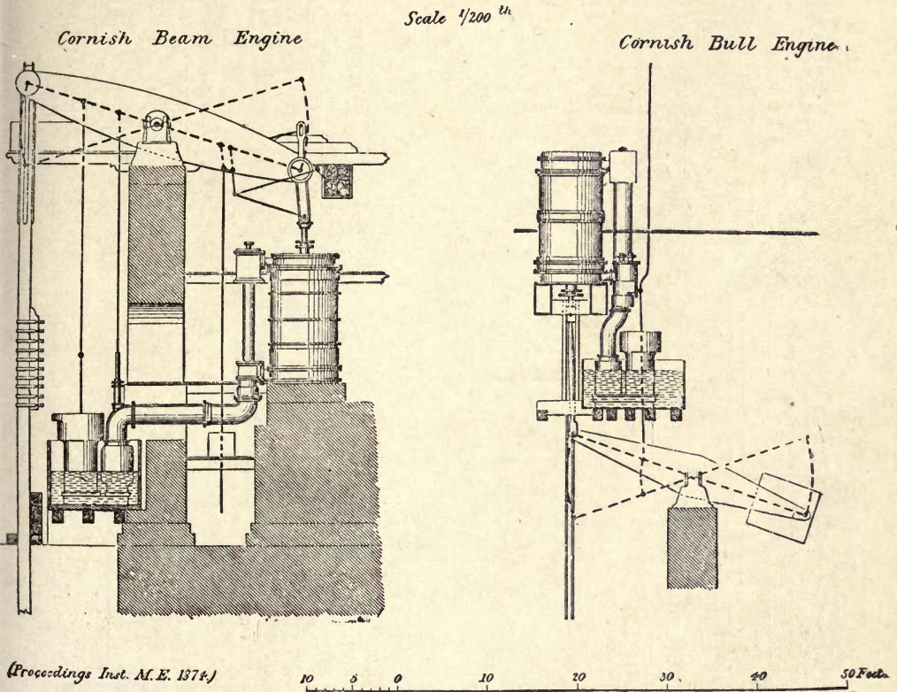
Fig. 7.—Sections showing Comparative Space occupied by Cornish and Bull Direct-acting Pumping Engines.
