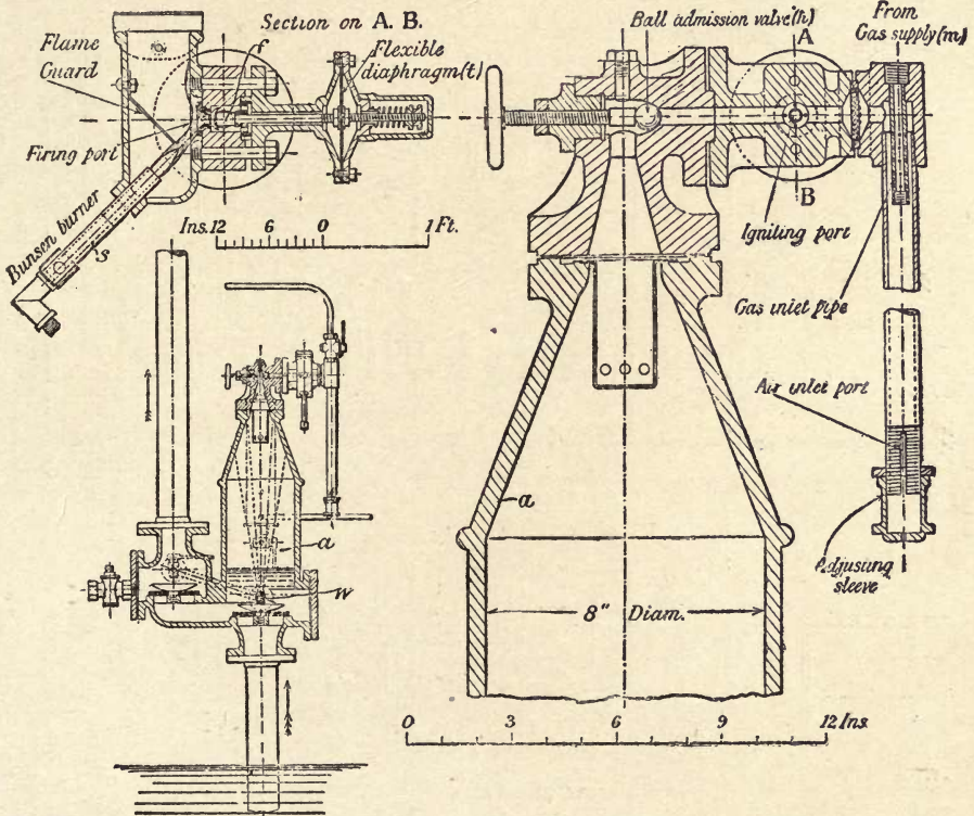
Fig. 192.—Joy's Domestic Gas Displacement Pump. Capacity, 1,000 gallons per hour against 20 feet head.
