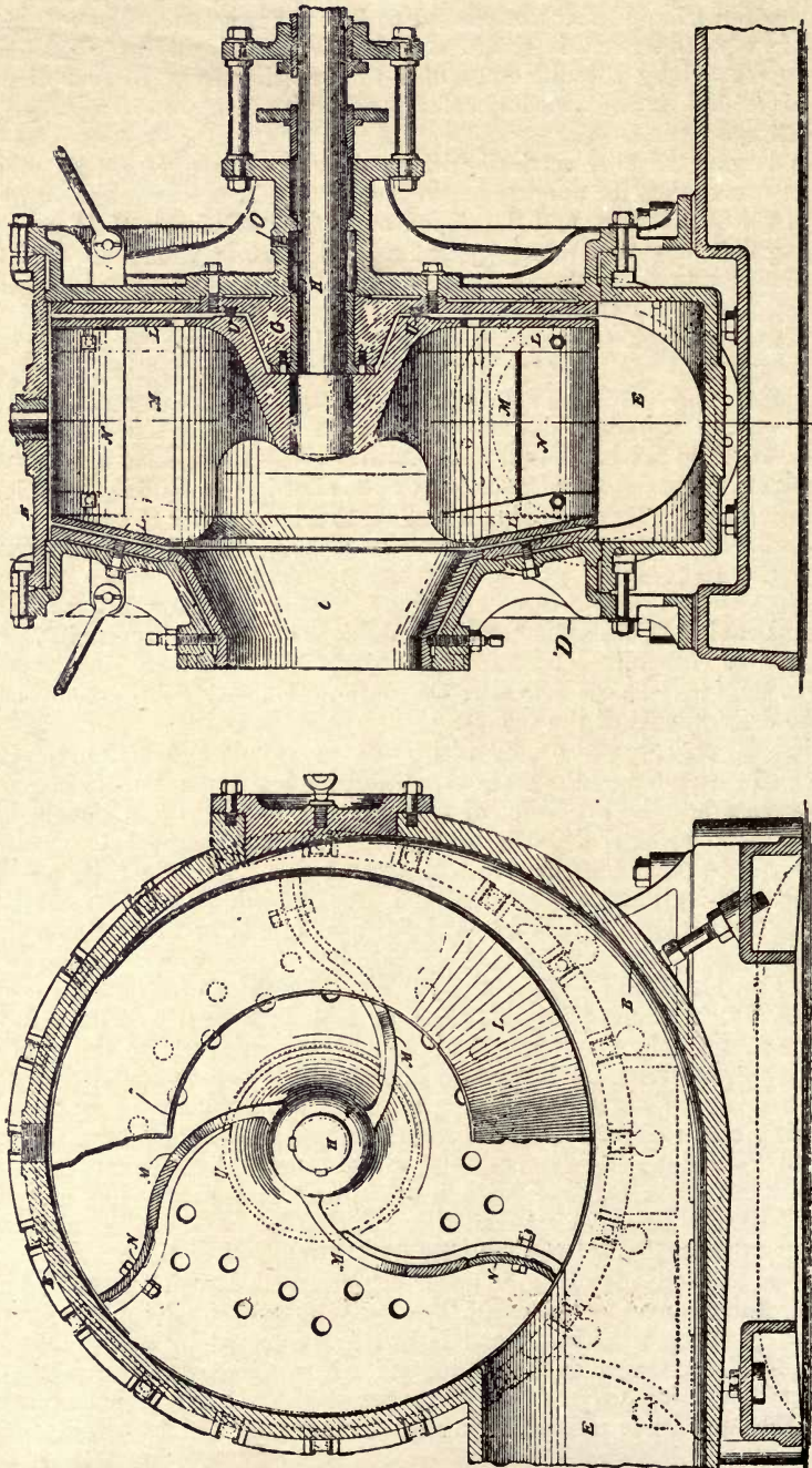
Fig. 270.—Sectional Elevations of Edwards "Cataract" Dredging Pump, showing Arrangement of Renewable Vanes.
