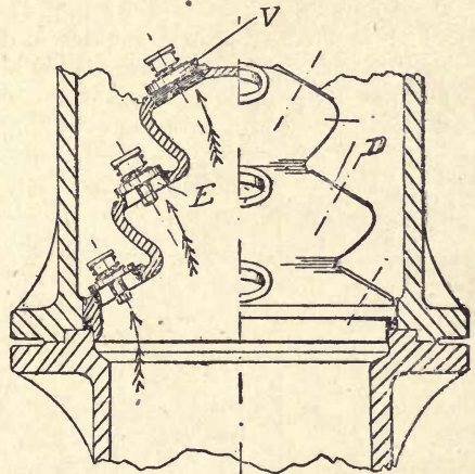
Fig. 44.—Triple Tier Beehive Multiple Valve Box.
