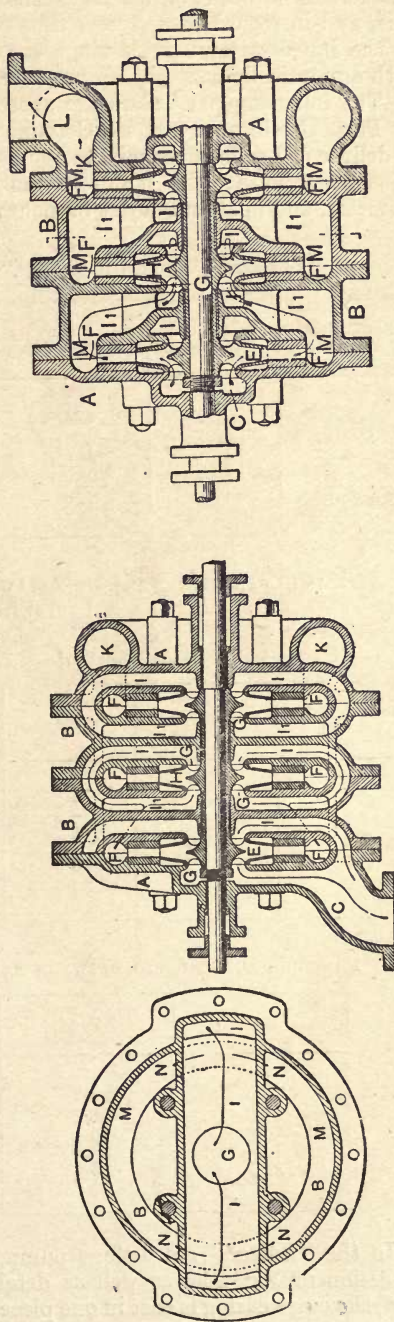
Fig. 284.—Sectional Elevations of Three-stage High-lift "Invincible" Centrifugal Pump.
