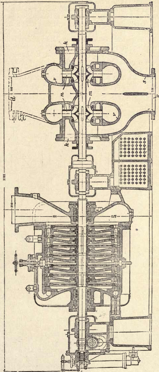
Fig. 281.—Twin Wheel Single-stage Turbine Pump. Capacity, 1,800 Gallons per minute, raised 120 feet; speed, 3,300 revolutions per minute.
