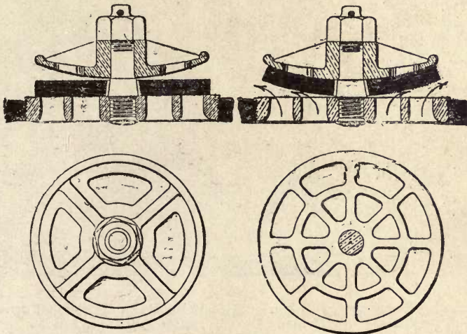
Fig. 201.—Sectional Elevations and Plans of Suction and Discharge Valves used in High-speed Fire Pumps.
