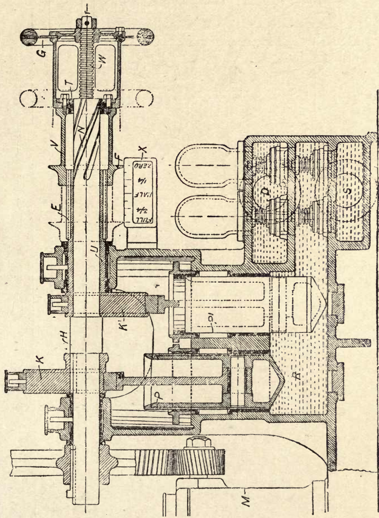
Fig. 230.—Clarke-Chapman 2-throw Variable-delivery Pump, with Compound Plunger Control. (See p. 316.)
