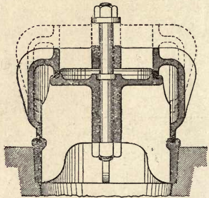
Fig. 54.—Double-seated Ring Valve.
