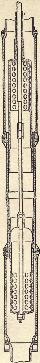
Fig. 67. — Double Plunger Balanced Deep - well Pump with Ashley Valves.
