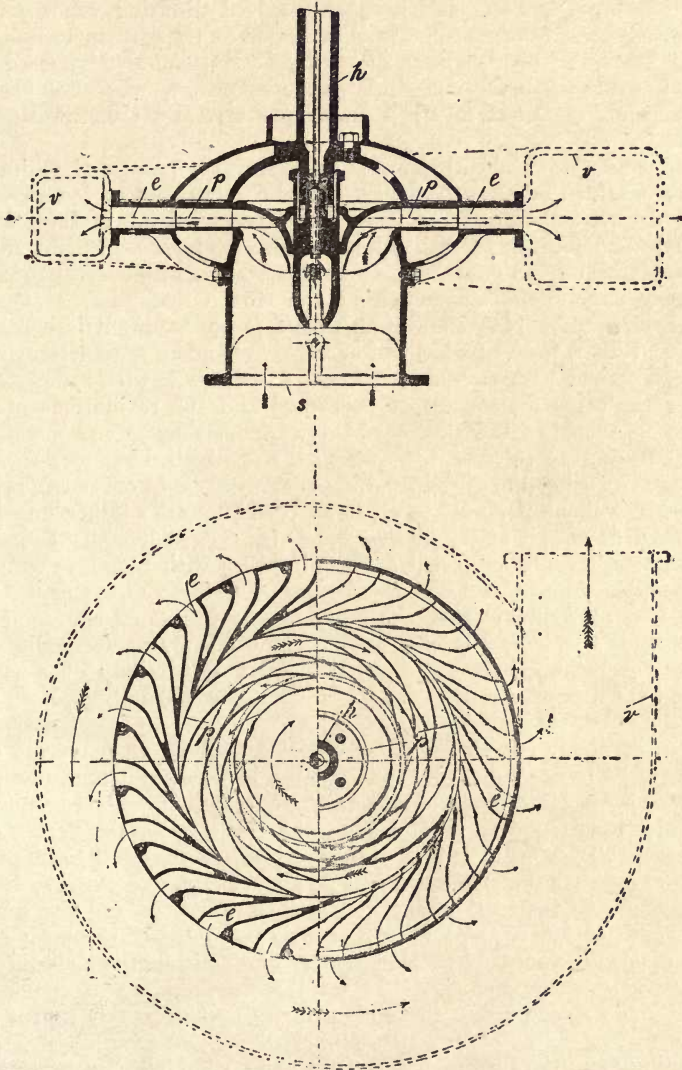
Fig. 275.—Nagel and Kaempe's Centrifugal Pump, with Ring containing Diverging Guide Passages between the Impeller and Vortex Chamber.
