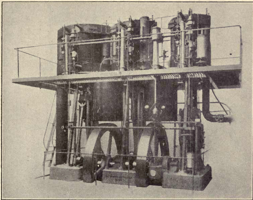
Fig. 14.—Three crank Triple-expansion Pumping Engine for Argentina.
