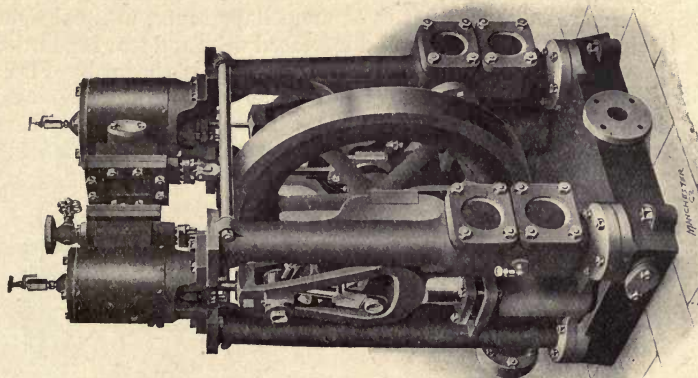
Fig. 119.—Compound Cameron Pump.
