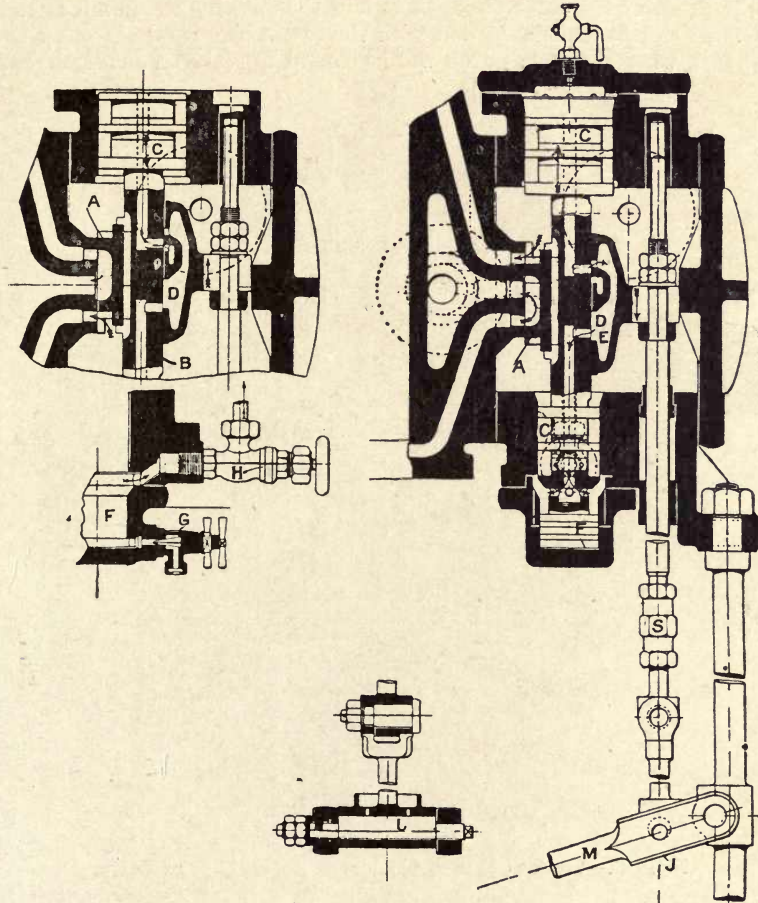
Fig. 103.—Differential Valve Gear used in the Storey Direct-acting Simplex Pump.
