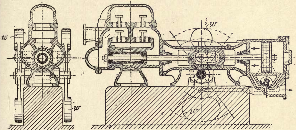
Fig. 98a.—Michael's Simplex Direct-acting Pump, with Compensating Balance Weights.
