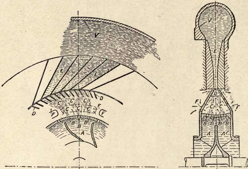
Fig. 172.—Rees Centrifugal Ejector Vacuum Pump.
