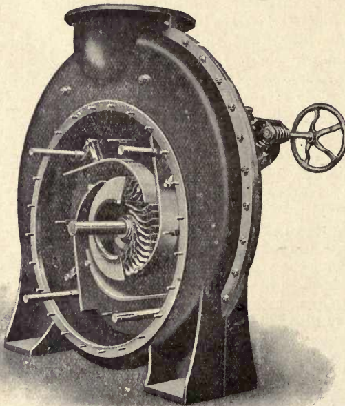
Fig. 300.—View of "Gilbert Gilkes'" Vortex Turbine, with Cover removed showing Swivel-action Guide Blades.
