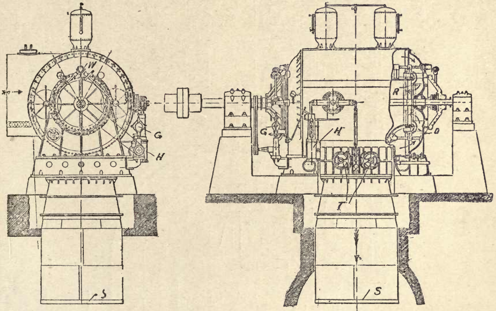
Fig. 321.—Part Sectional Elevations of One of Three Mixed-flow Central Discharge Horizontal Turbines. (Supplied by the I. P. Morris Company to develop 6,000 H.P. on a pressure head of 125 feet, and speed of 180 revolutions per minute, at Shawinigan Falls Quebec. Speed control by throttle in draft tube.)
