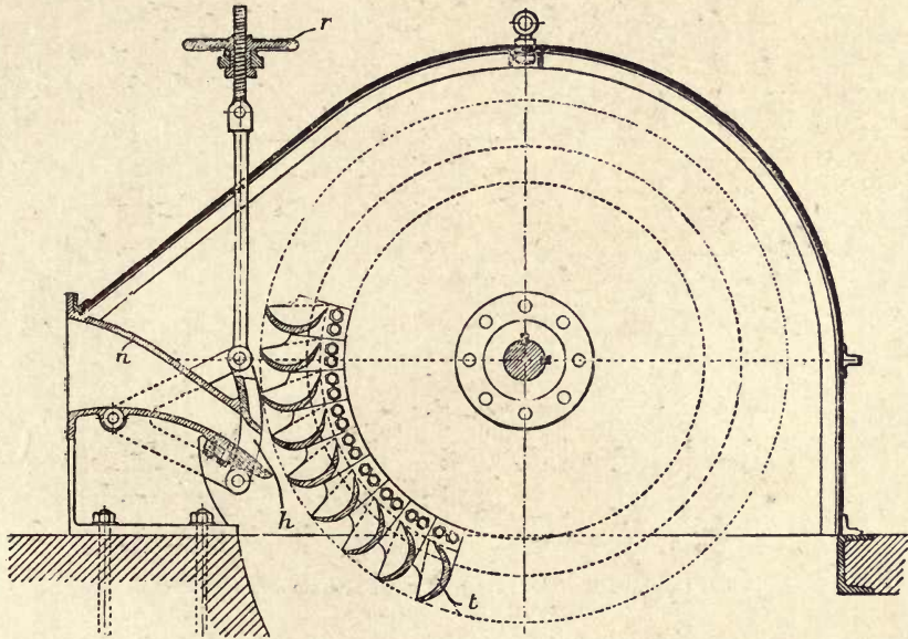
Fig. 340.—Hood Regulator used in Pitman Single-jet Impulse Turbines.
