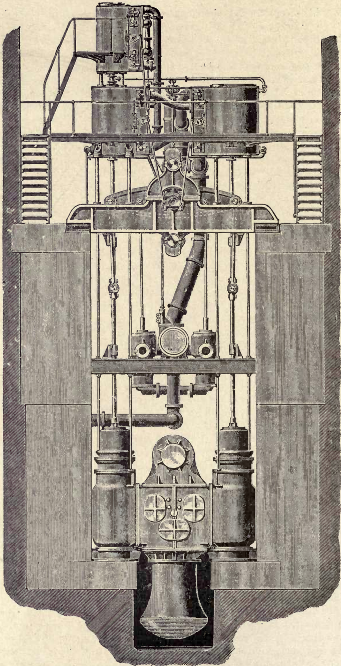
Fig. 22.—Sectional Elevation of Vertical Triple-expansion Worthington Pumping Engine, with Four Single-acting High-lift Pumps,
