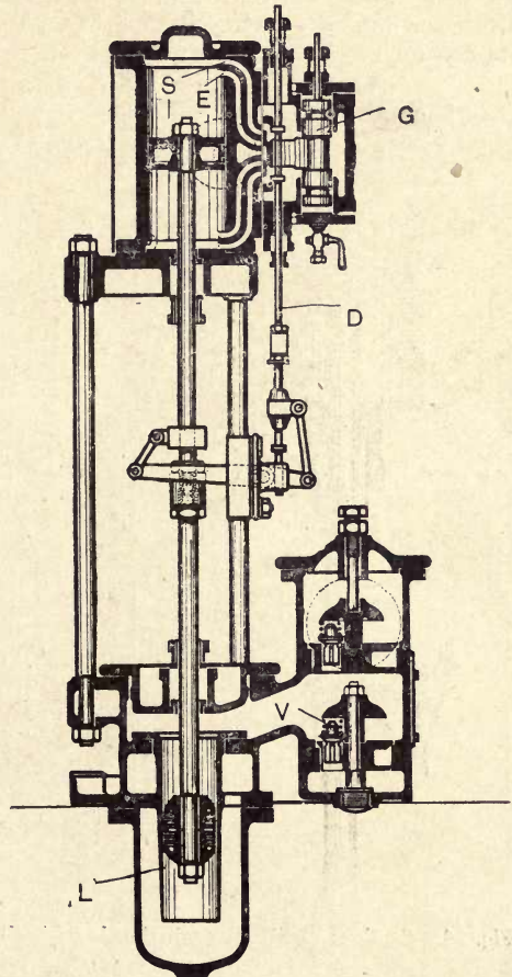
Fig. 97.—Sectional Elevation of Karoome Feed Pump.
