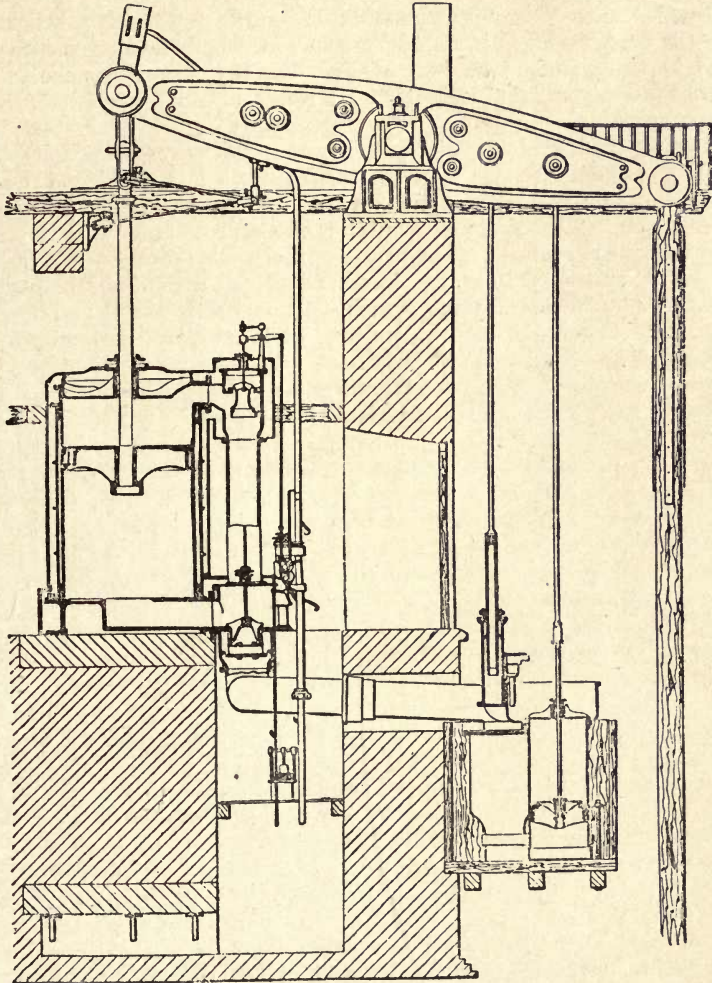
Fig. 6.—Cornish Pumping Engine, with Single-acting Steam-jacketed Cylinder.
