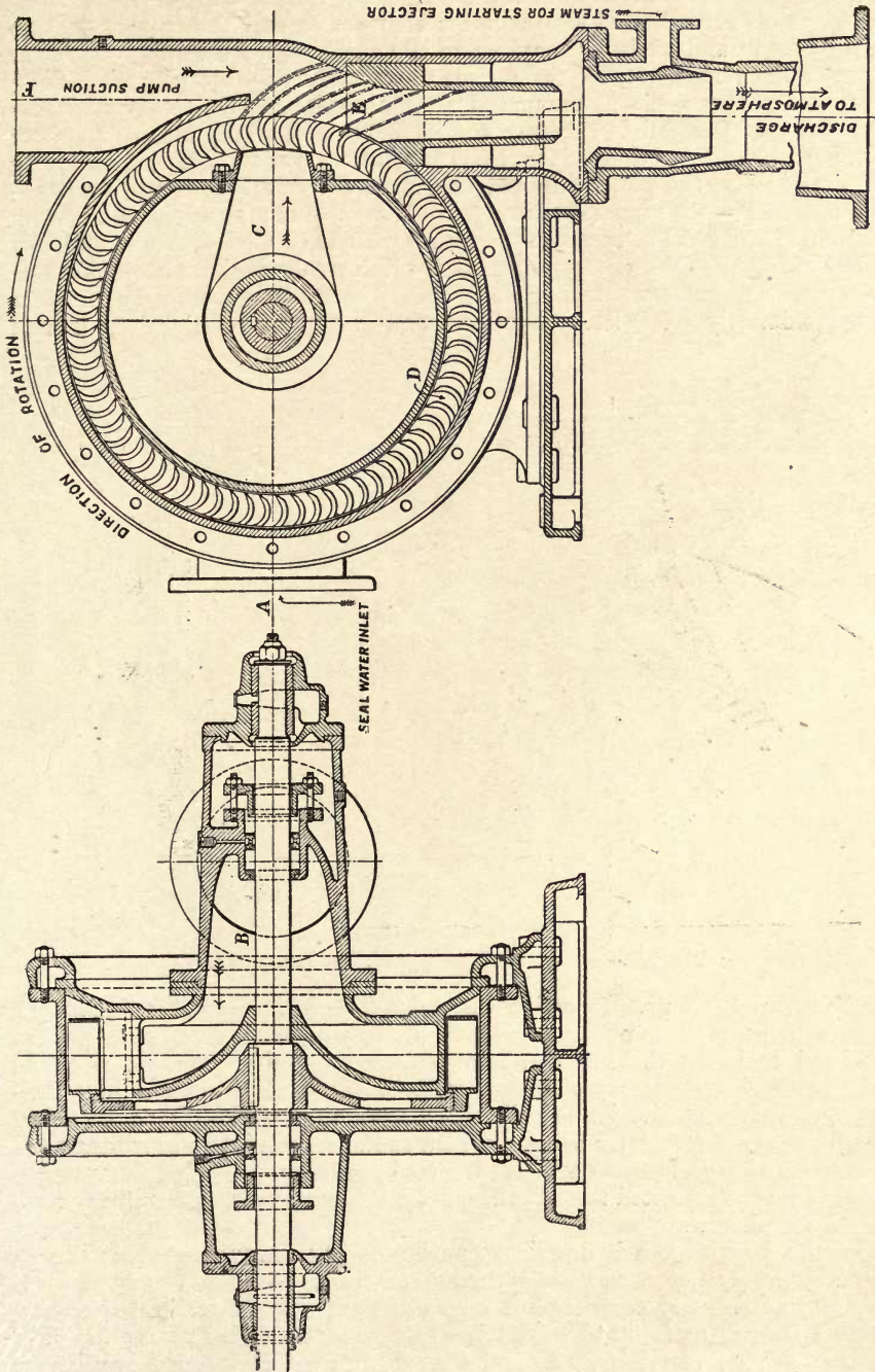
Fig. 171.—Leblanc-Westinghouse Rotary Hydraulic Vacuum Pump.
