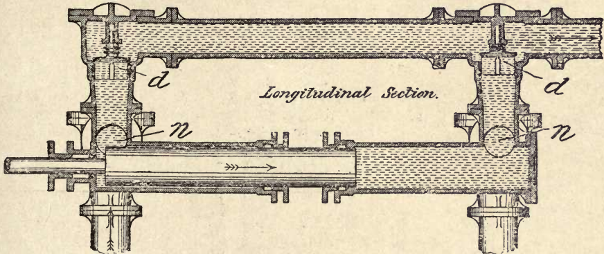
Fig. 35.—Double-acting Ram Force Pump.
