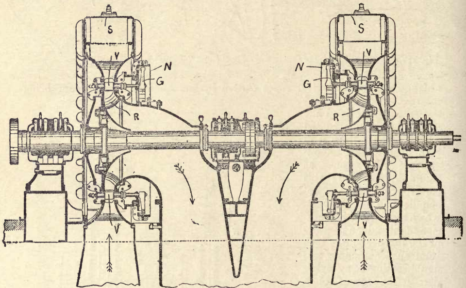
Fig. 319.—Cross-section of a 12,000 H.P. Twin Inward-flow Horizontal Turbine, for the Ontario Power Company. Pressure head of 175 feet, revolutions 187 per minute, speed control by movable guide vanes
