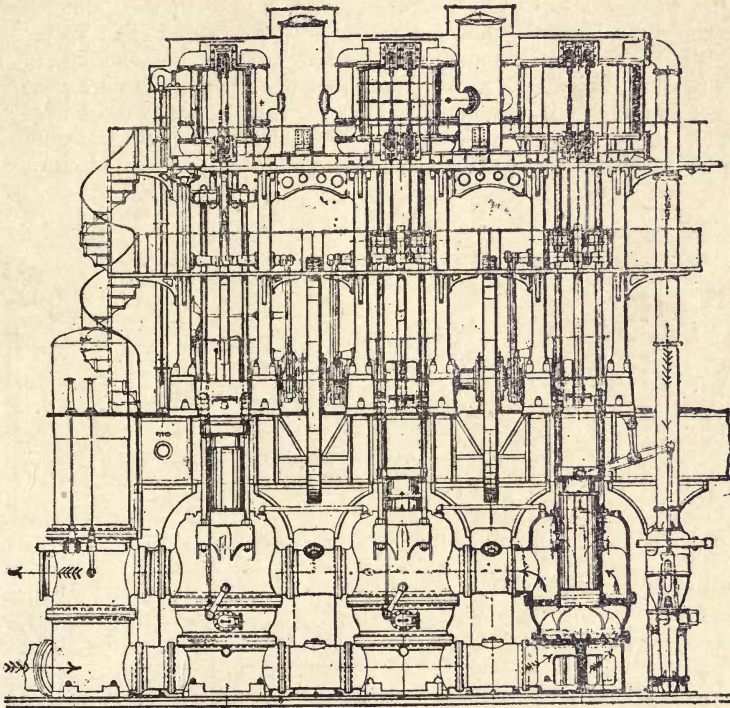
Fig. 18.—Triple-expansion High-duty Pumping Engine.
