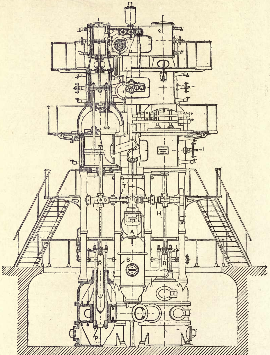
Fig. 24.—Section showing Arrangement of Steam Cylinders, Double-acting Air Pumps, and Hydraulic Balancing Plungers of Worthington Vertical Pumping Engine.
