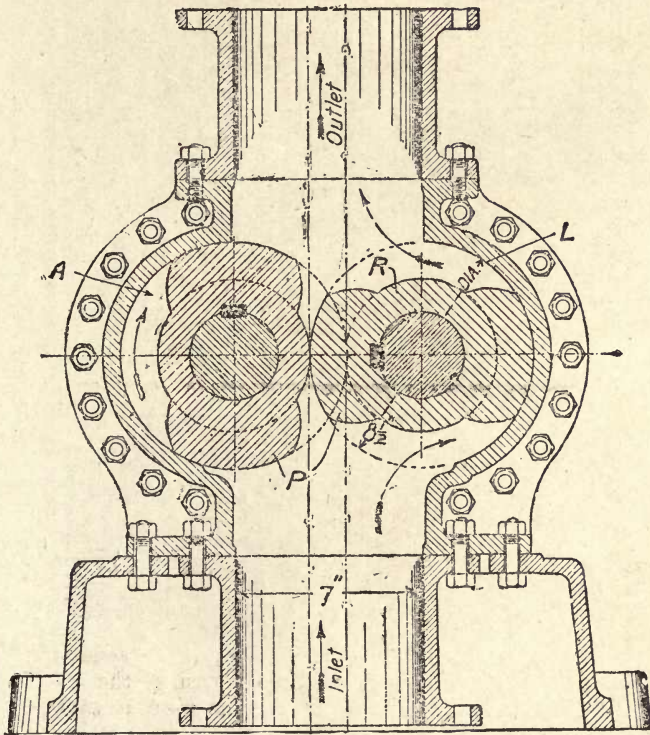
Fig. 241.—A-cme Rotary Pump. Capacity, 42,000 gallons per hour.
