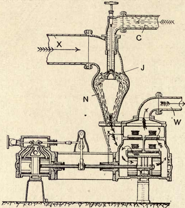
Fig. 153.—Worthington Independent Jet Condenser
