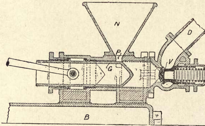
Fig. 234.—Section of Horizontal Ram-plunger Force Pump for Green Sugar.
