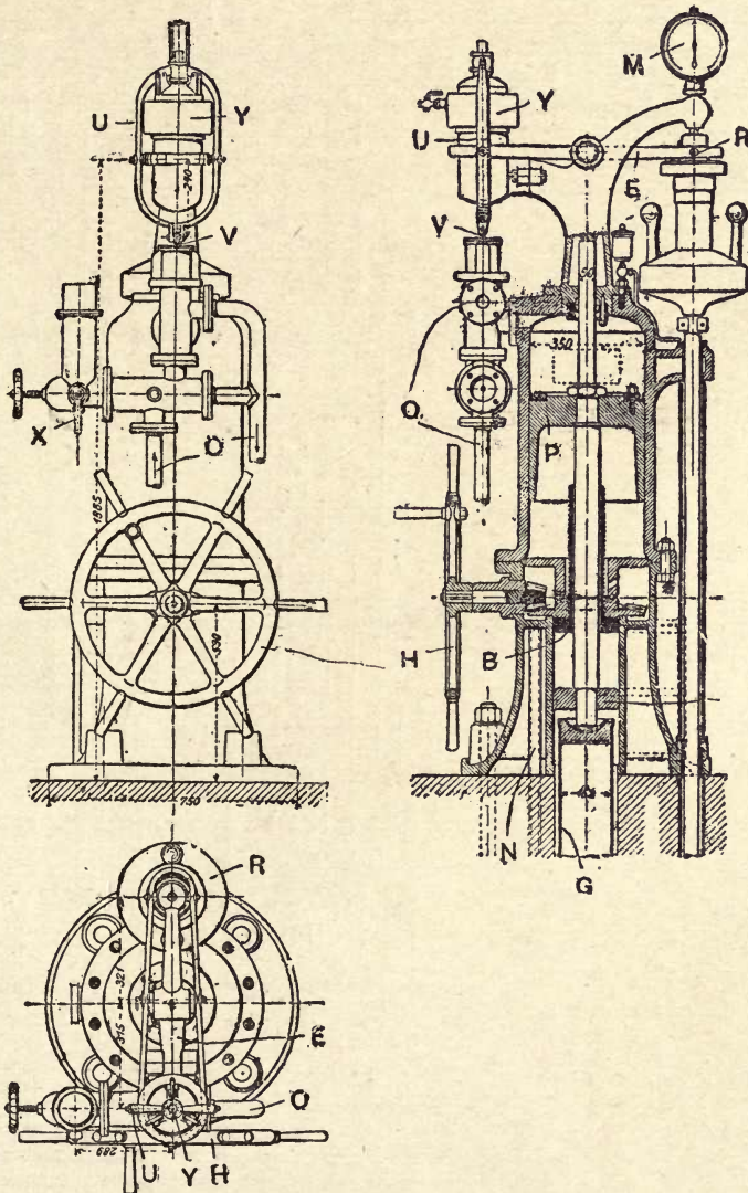
Fig. 325.—Elevation, Cross-section, and Plan of "Escher-Wyss" Oil Pressure Governor As used for the 5,500 H.P. turbines at Niagara Falls.
