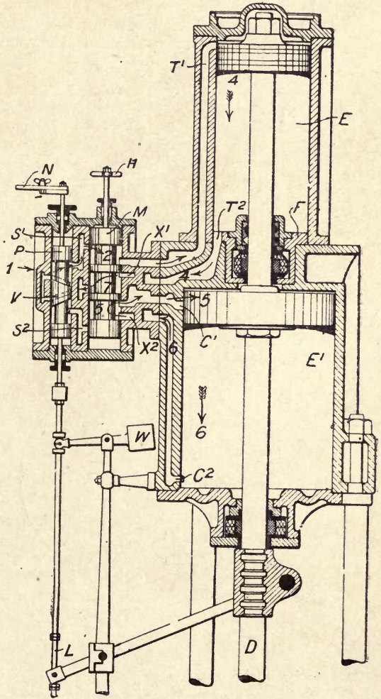
Fig. 100.—Nichols' Distribution applied to a Compound Direct-acting Pump.
