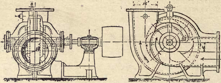
Fig. 264 —Ruston-Proctor Belt-driven Irrigation Pump, showing Special Form of Suction Branch.
