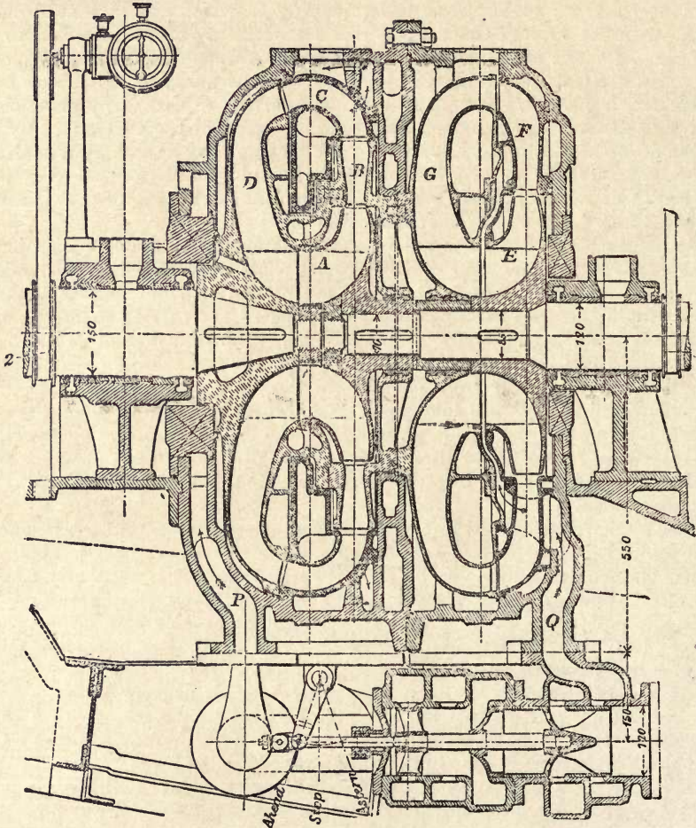
Fig. 233.—Föttinger Hydraulic Turbine Action Variable Transmitter.
