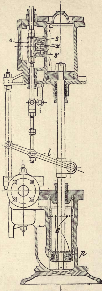
Fig. 89.—Sectional Elevation of the Bradford Patent Boiler Feed Pump (Slide Valve Type).
