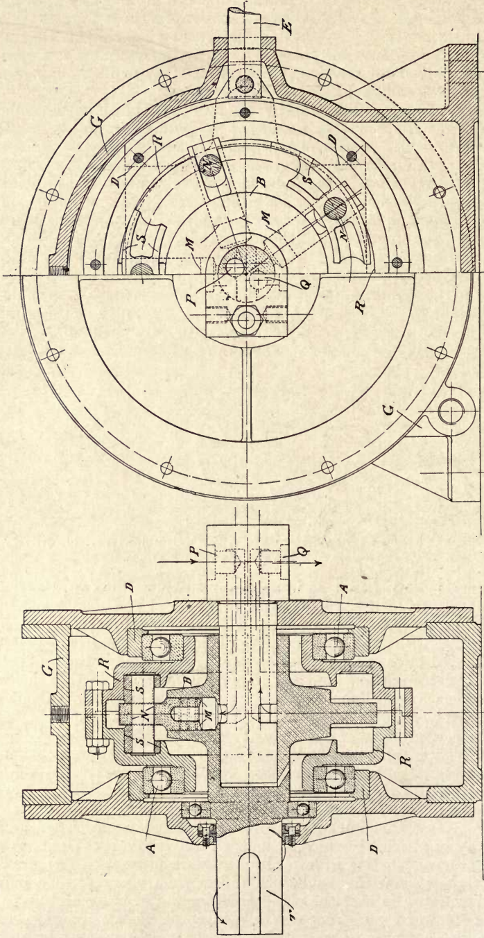
Fig. 232a.—Cross-sections of Hele-Shaw variable and Reversible Flow Radial Pump or Motor.
