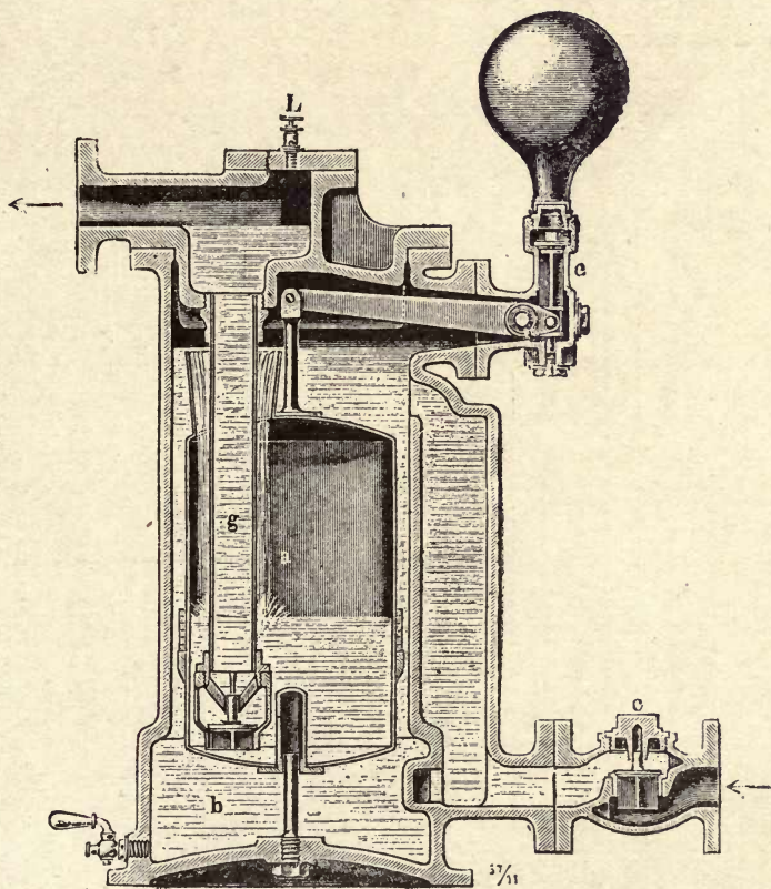
Fig. 188.—Körtzing's Float-action Feed Pump.
