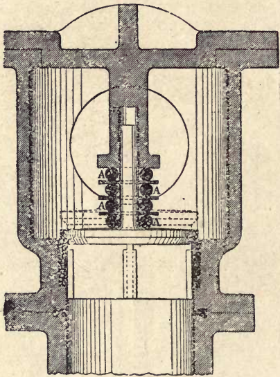
Fig. 53.—Common Form of Single Mitre Valve.
