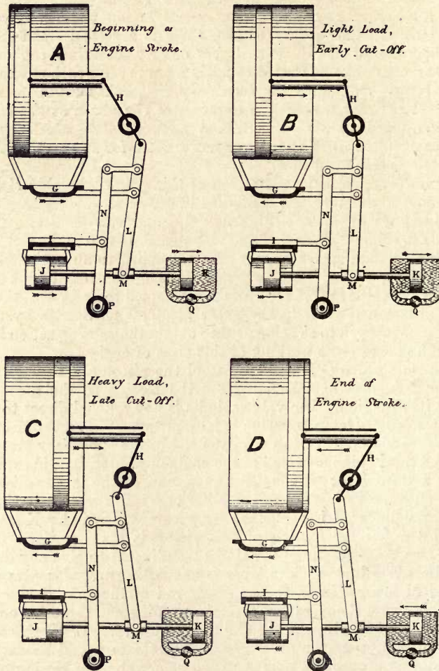
Fig. 28.—Davey Differential Valve Gear.
