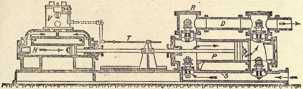
Fig. 176.—Davey Hydraulic Mine Pump.
