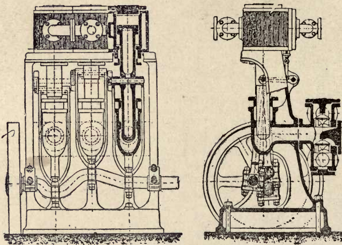
Fig. 118.—Yates and Thom Feed Pump.
