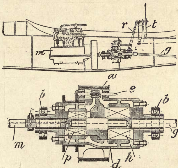
Fig. 249.—Pittler Hydraulic Reversing Gear applied to a Motor-launch.
