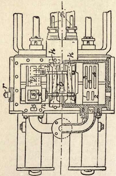
Fig. 113.—Sectional Elevations, showing Steam Cylinders of "Odessa" Compound Duplex Pump.
