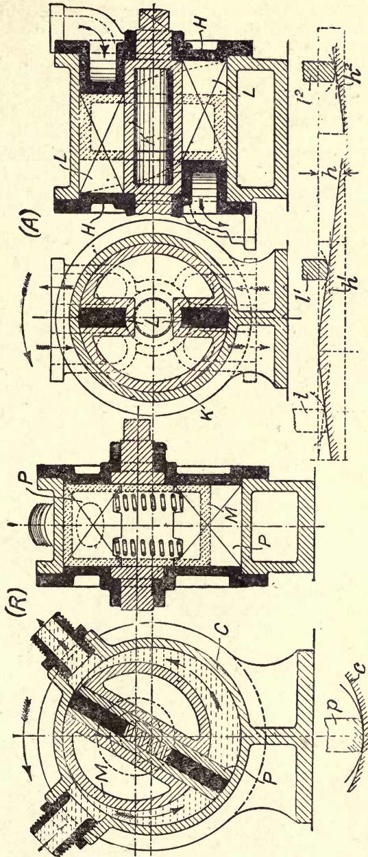
Fig. 247.—Rotary Pumps with Radial and Axial Sliding Pistons
