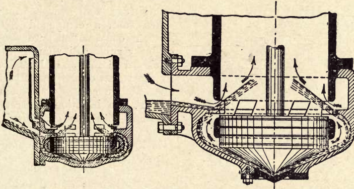
Fig. 157.—Sections showing the Difference in the Working of the Bodmer and Edwards Air Pumps.
