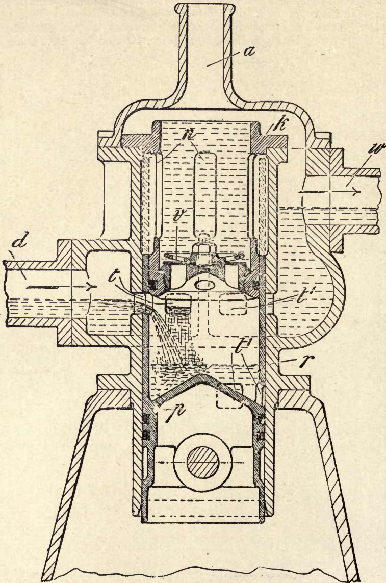
Fig. 166.—Inverted Design of Valveless Condenser Pump.
