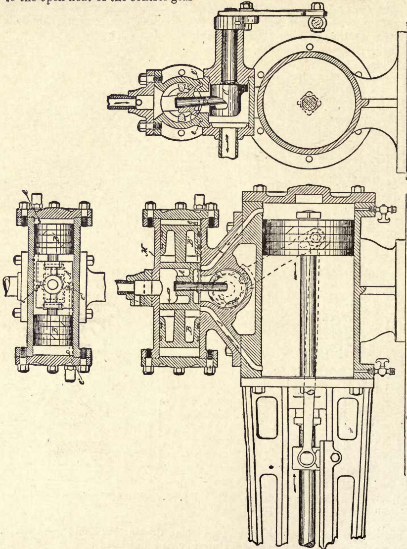
Fig. 36.— Valve Gear used in Davidson Simplex Pump.
