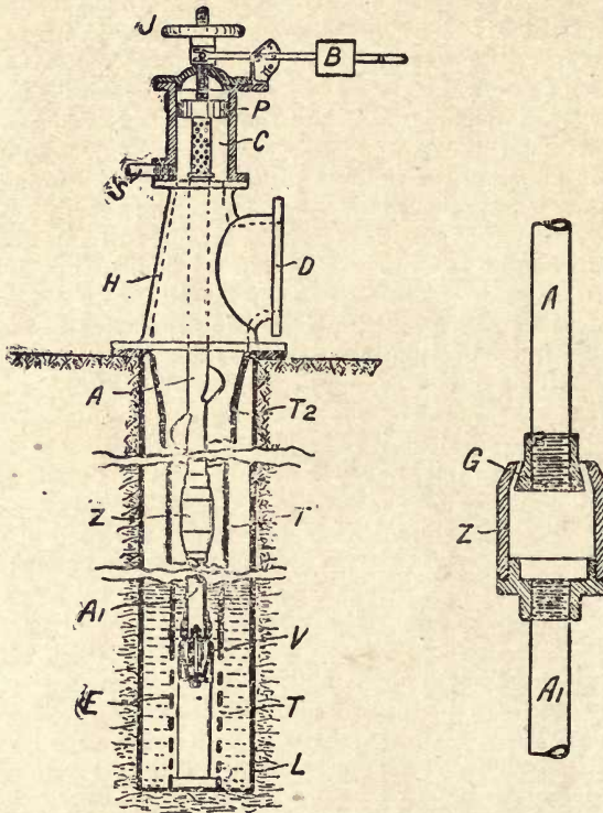
Fig. 77.—Price's Taper Tube Air-lift Pump.
