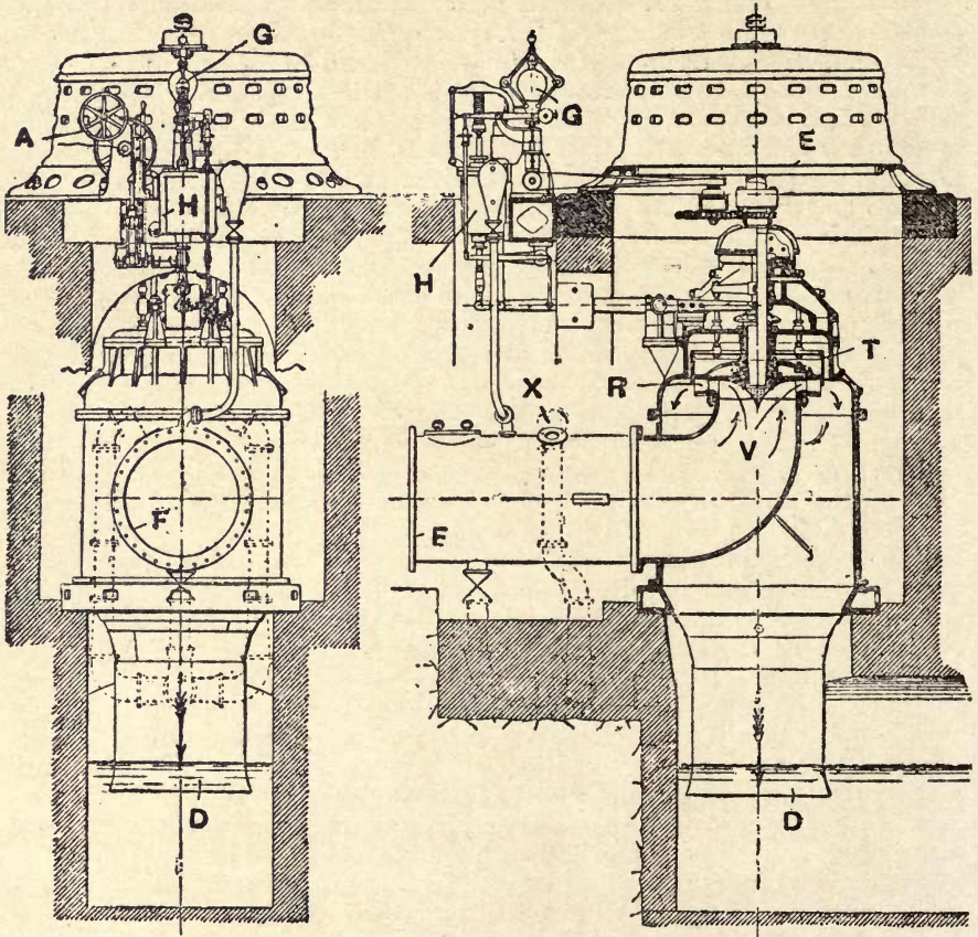
Fig. 330.—2,000 H.P. Single-wheel Outward-flow Vertical Turbine at Trenton Falls, N.Y. Pressure head, 266 feet; revolutions, 360 per minute. Speed control by cylindrical sluice gate.
