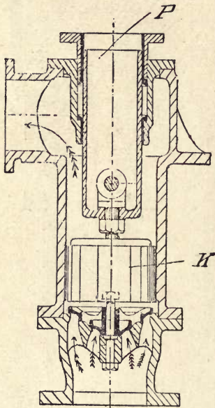
Fig. 34.—Typical Plunger and Bucket Force Pump, with Triple-seated Ring Valves.
