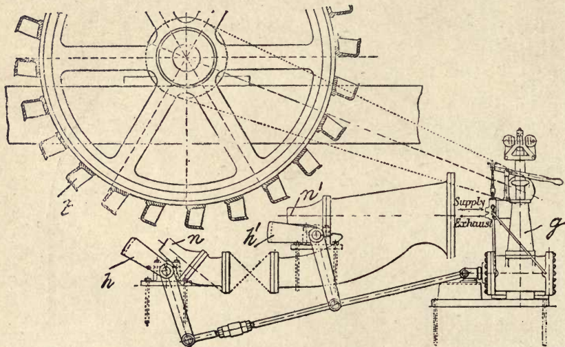
Fig. 341.—Pitman Impulse Turbine arranged with Double Jet Action controlled by Hydraulic Governor
