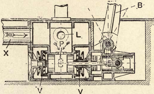
Fig. 158.—Double-acting Valveless Piston Air Pump for Compound Corliss Engine with Jet Condenser.
