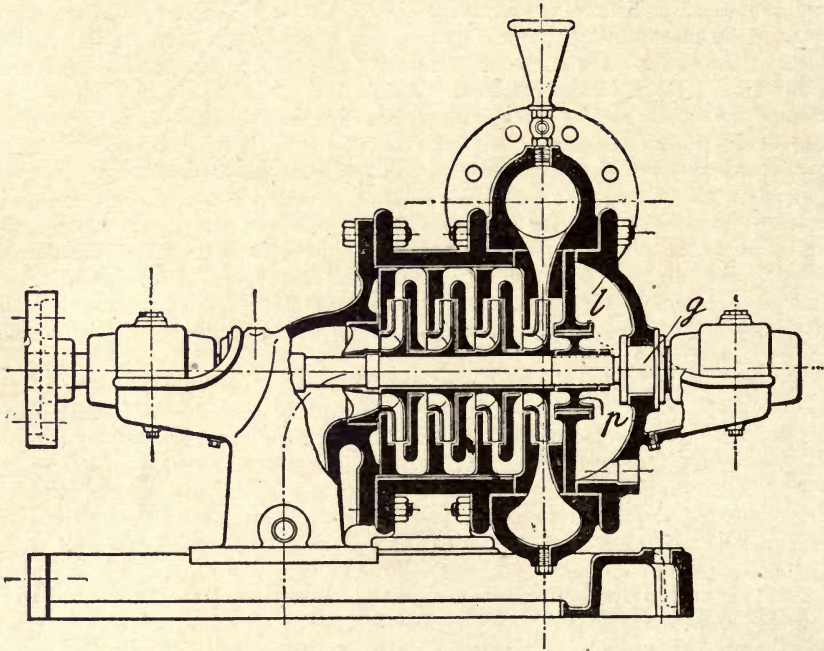
Fig. 295.—Sectional Elevation of Four-stage Victoria Turbo Pump.
