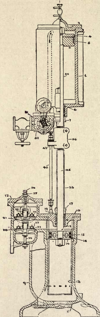
Fig. 89a.—Sectional Elevation of a later form of Bradford Boiler Feed Pump, with "Corliss" Valve Steam Distribution?
