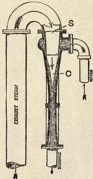
Fig. 149.—Exhaust Ejector for Barometrical Condenser.
