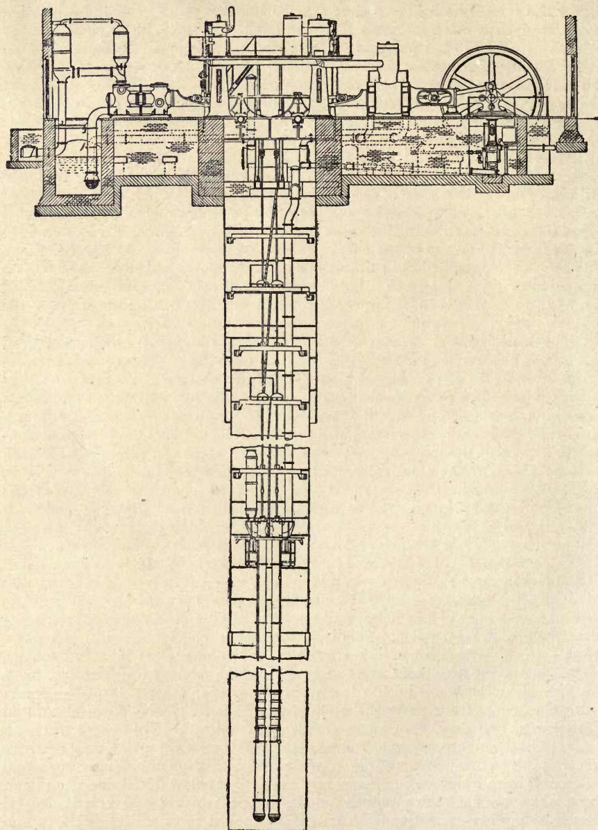
Fig. 9.—Sectional Elevation of Simpson Triple-Expansion Rotatory Deep-level Balanced Action Pumping Engine for the Barnet Gas and Water Company.
