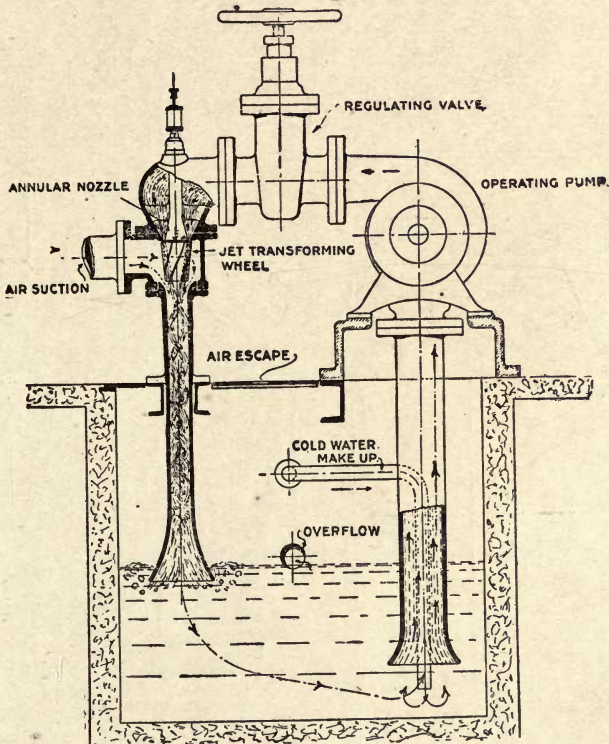
Fig. 173.—Worthington Hydraulic Ejector Vacuum Pump.
