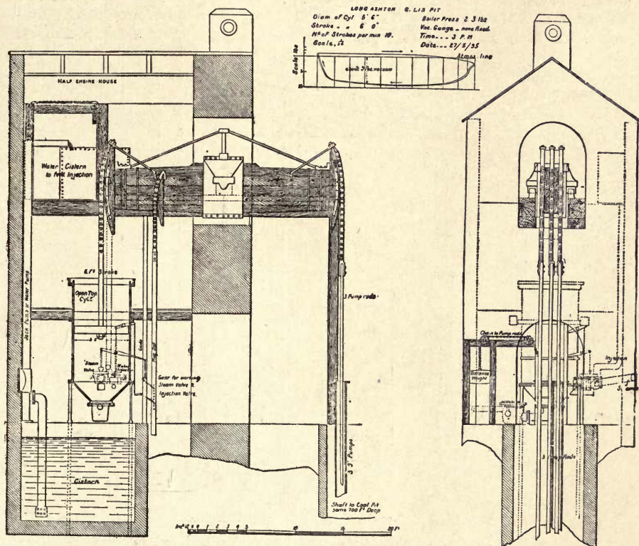
Fig. 2.—Section of Newcomen Pumping Engine, showing Details of Steam and Injection Valve Gear.
