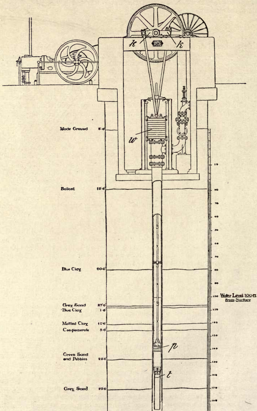
Fig. 63.—Gas-driven Artesian-well Pump, with Counterpoise Balancing Action.
