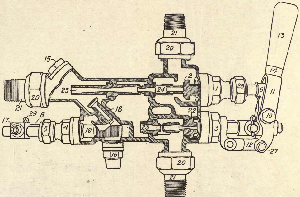
Fig. 133 —Buffalo Combined Lifter and Forcer, Double-tube Single-movement Boiler-feed Injector.
