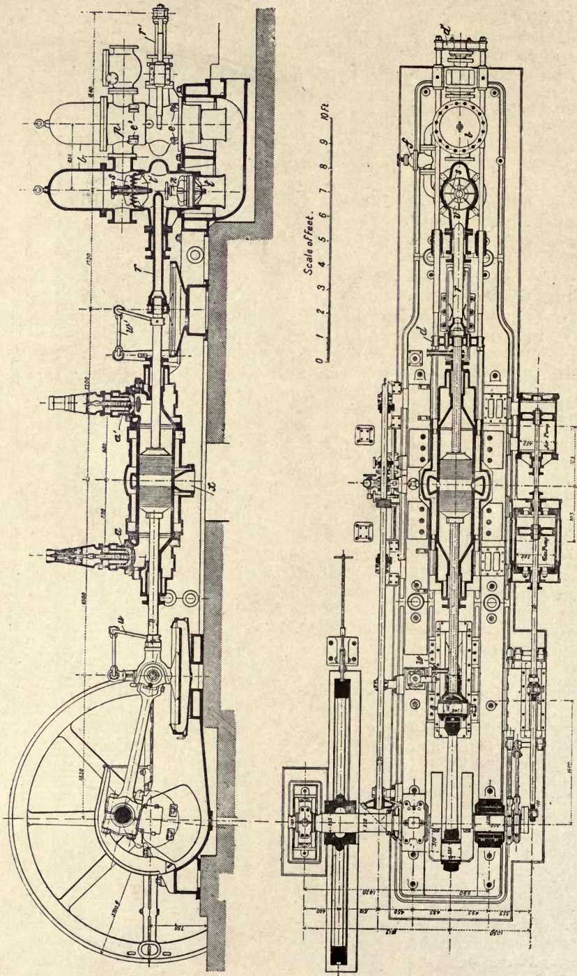
Fig. 219.—Gas-Engine Driven Direct-Connected Accumulator Pumps. (Capacity, 25 to 90 cubic feet per minute against a pressure of 375 lbs. per square inch.)
