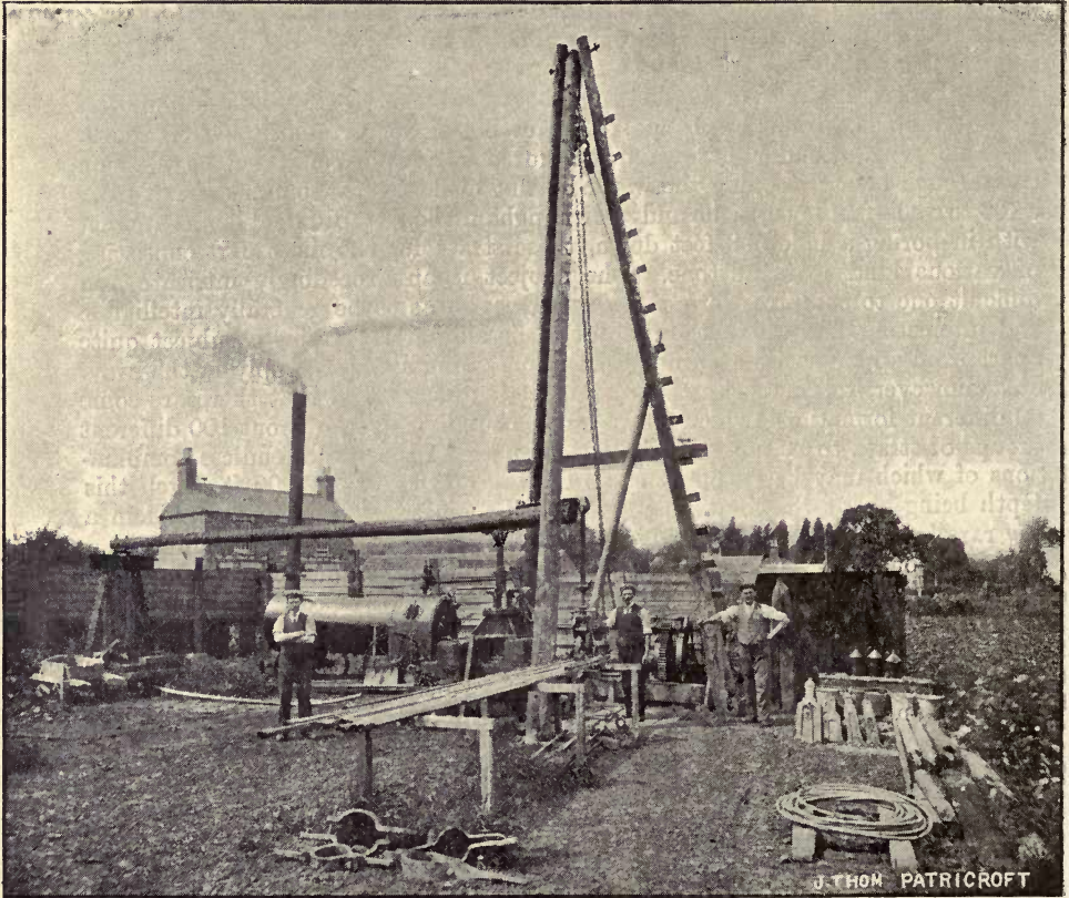
Fig. 57.—Steam Percussion Boring Rig, with Pole and Trestle Action.
