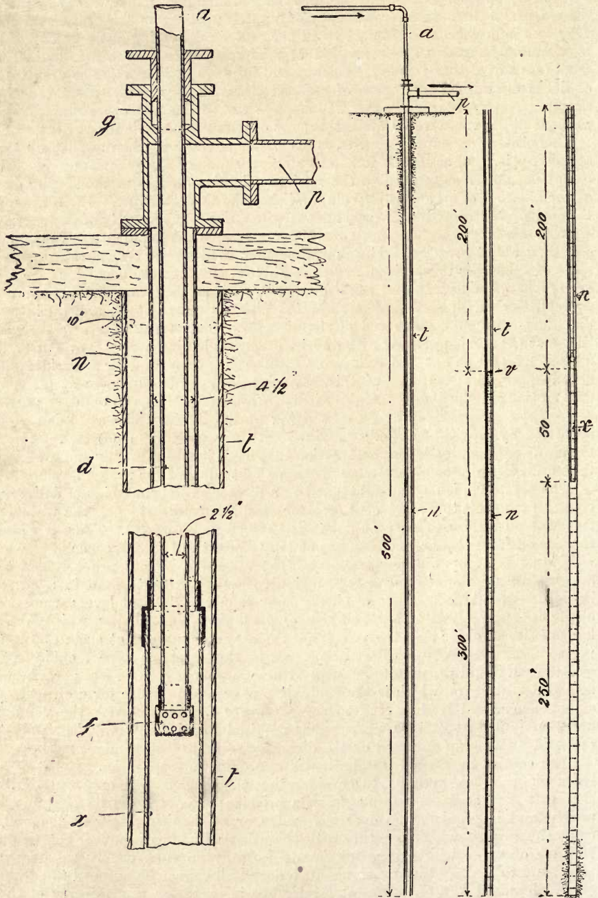
Fig. 83.—Arrangement of Air-lift Pump for 1,500 Feet Well with Oil at the 700 Feet Level.
