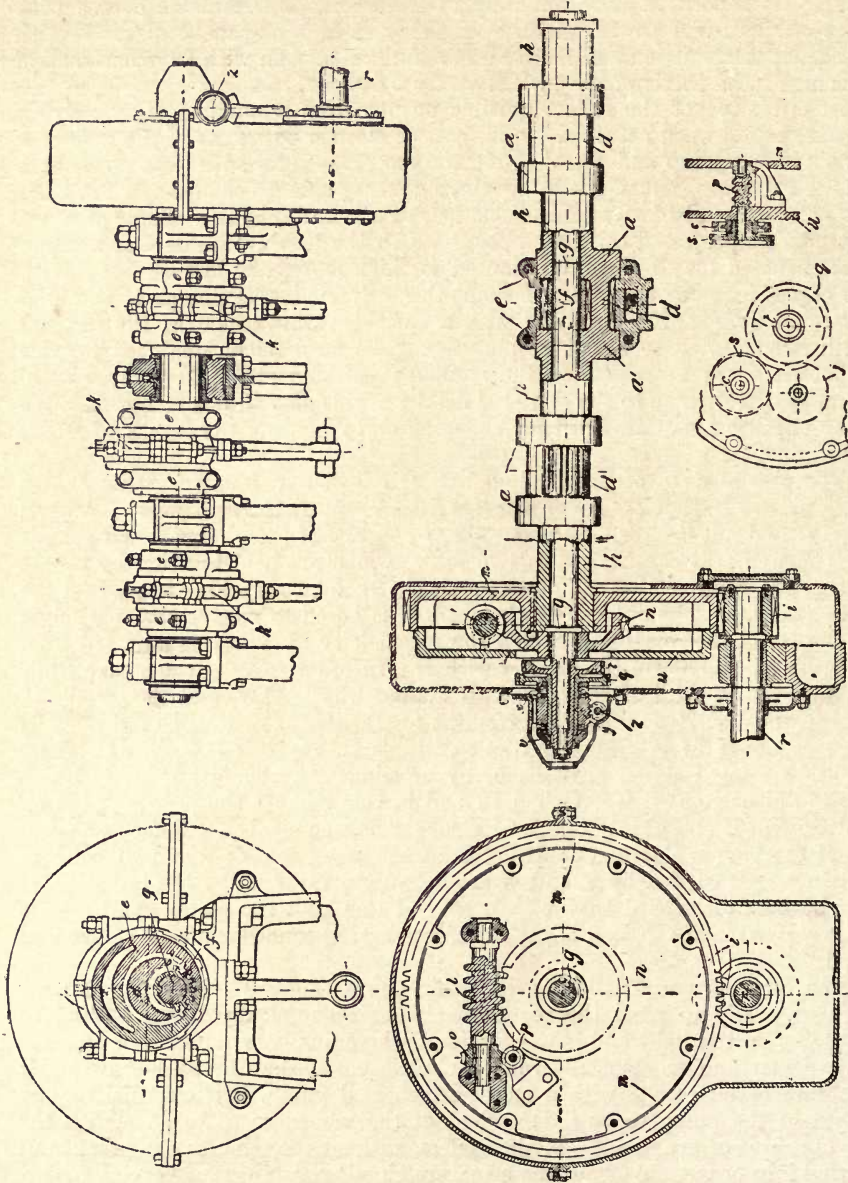
Fig. 227.—Sinclair Stroke controlling Mechanism used in Hayward-Tyler Variable Delivery Pump.
