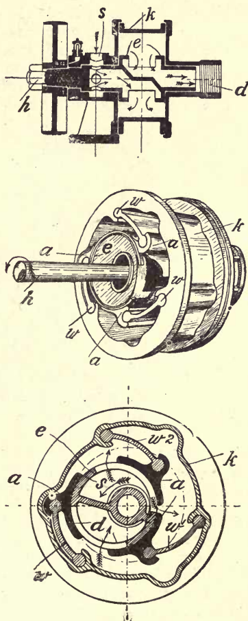
Fig. 253.—Sectional and Perspective Views of Lane-Eland Rotary Pump.
