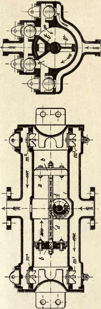
Fig. 257.—Sectional Elevations of the Arma and Delta Double-acting Oscillating Pumps.
