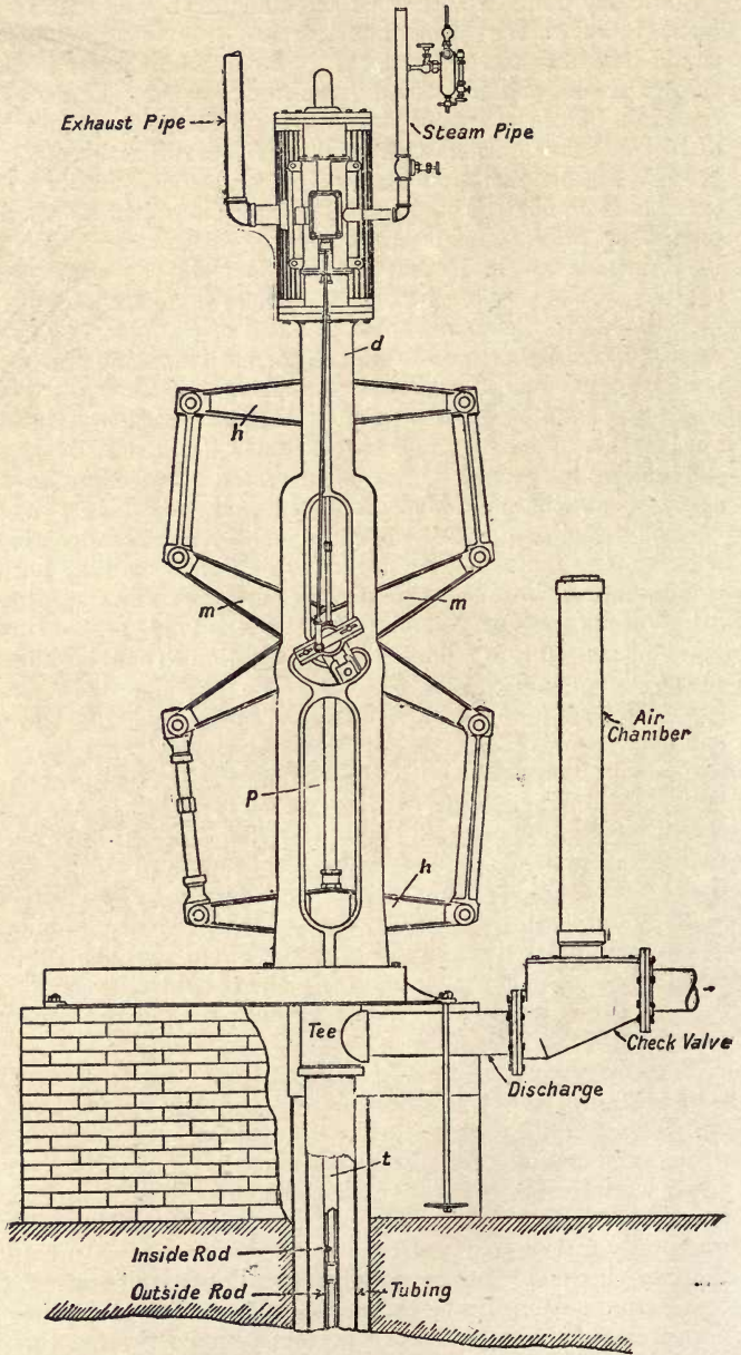
Fig. 68. — Downie Double-acting Direct-connected Steam Borehole Pump.
