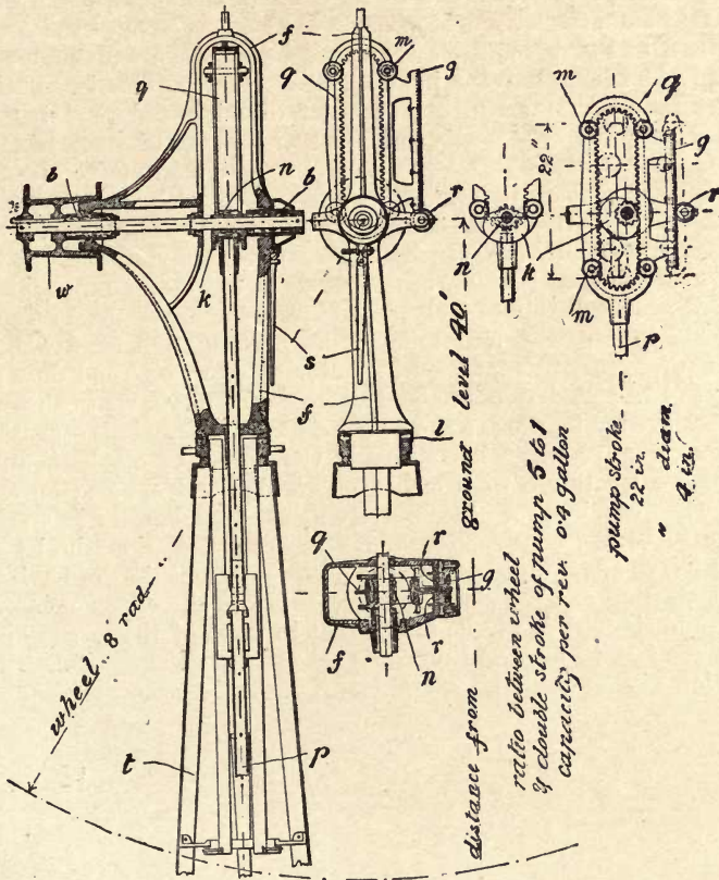
Fig. 260.—Details of Driving Gear of Canadian Imperial, 22 × 4 Inches, Double-acting Wind Pump.
