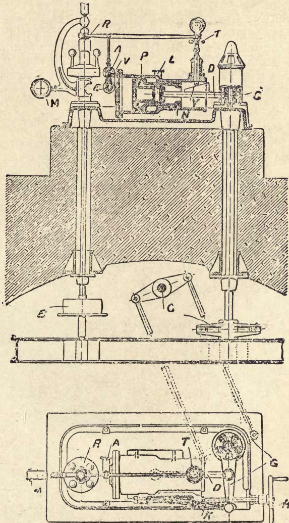
Fig. 304.—Cross-section and Plan of Oil Pressure Governor as used for the 1,250 H.P Conical Turbines at Lyons.
