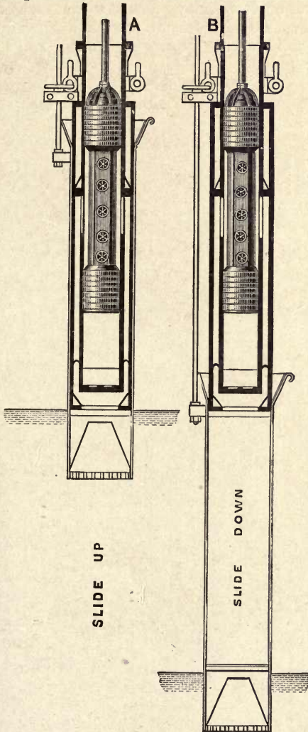
Fig. 39.—Ashley Sinking Pump
