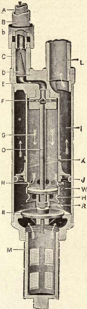
Fig. 185.—Erwin Steam Ram.
