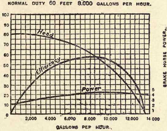
Fig. 278.—Diagram of Rees-Roturbo Self-regulating Pump.
