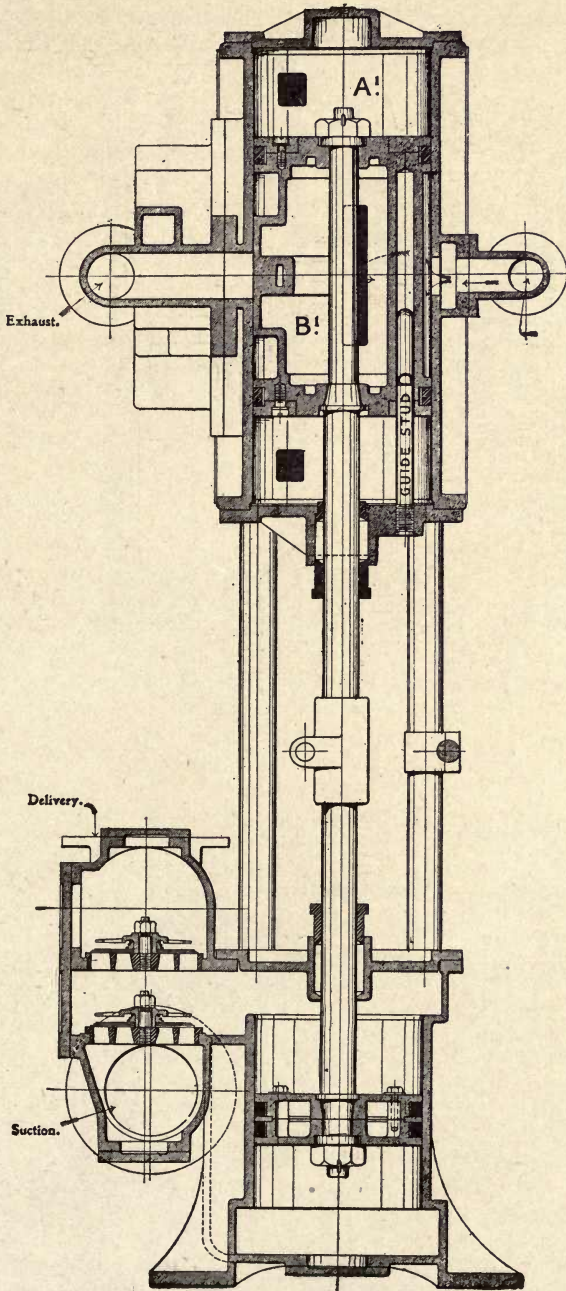
Fig. 110.—Cross-section of Mumford Valveless Duplex Feed Pumps.
