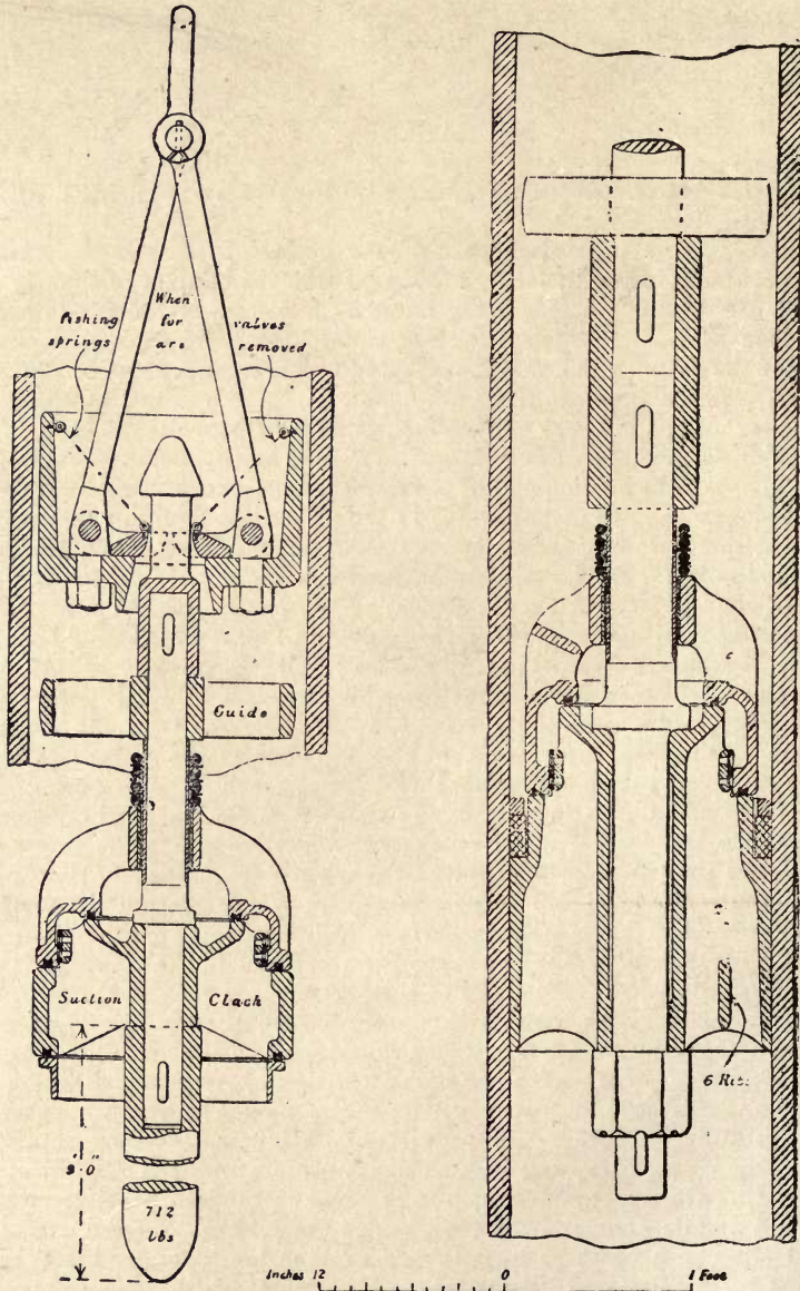
Fig. 62.—Artesian-well Pump with Double-seated Valves.
