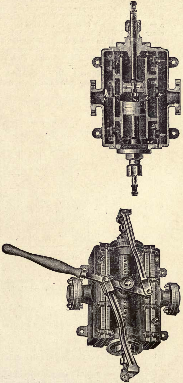
Fig. 258.—Turner-Wilcox Triple-action Plunger Pump.
