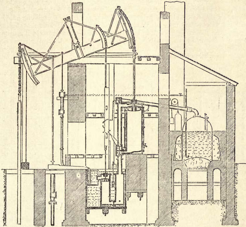
Fig. 4.—Early "Watt" Pumping Engine, with Enclosed Cylinder and Separate Condenser.
