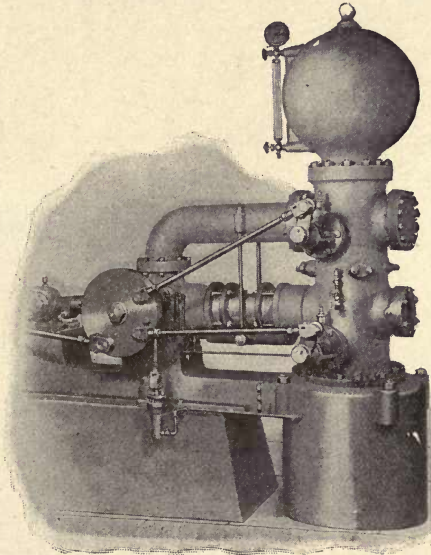
Fig. 207.—Elevation of Riedler Differential Pump, showing Actuating Gear.
