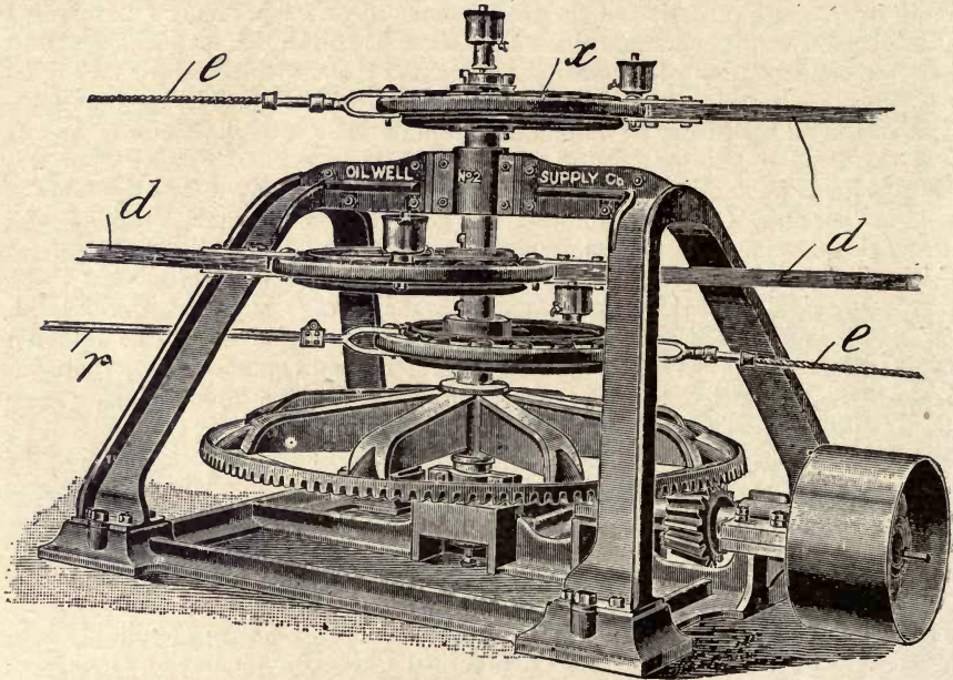
Fig. 78.—Multiple Plunger Pump actuating Gear for Oil Wells.
