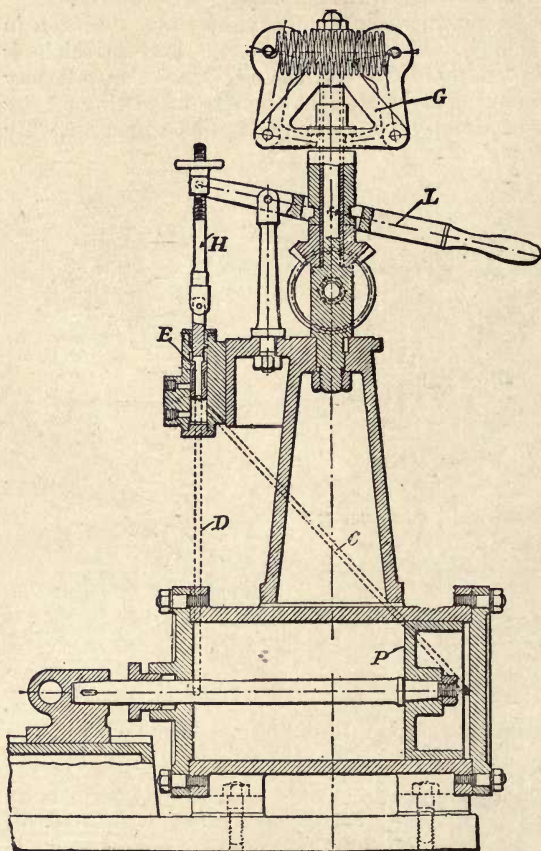
Fig. 337.—Pitman Hydraulic Turbine Governor.
