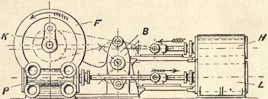
Fig. 19.—Rotative Duplex Pumping Engine.
