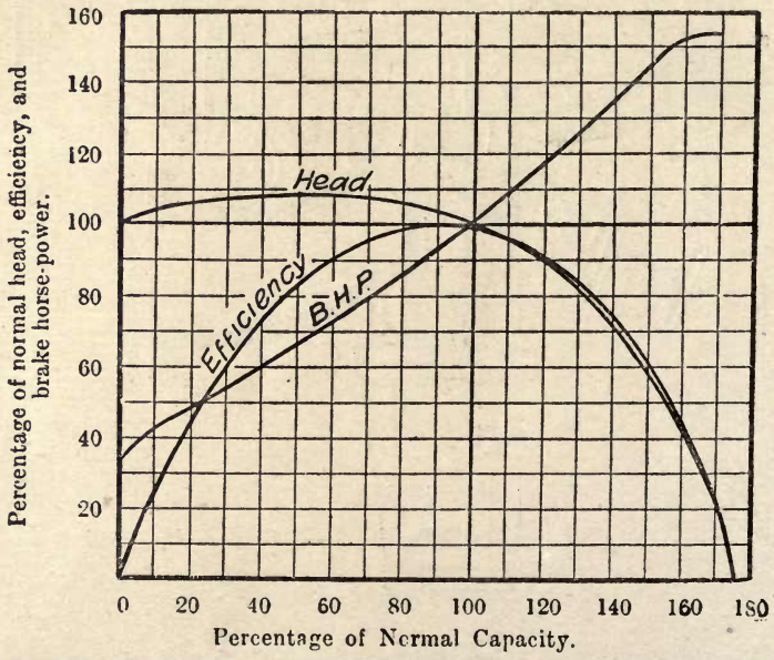
Fig. 290.—Characteristic Curves of High-lift Worthington Turbine Pumps.
