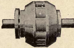
REES ROTURBO IMPELLER OR REVOLVING PRESSURE DRUM.
