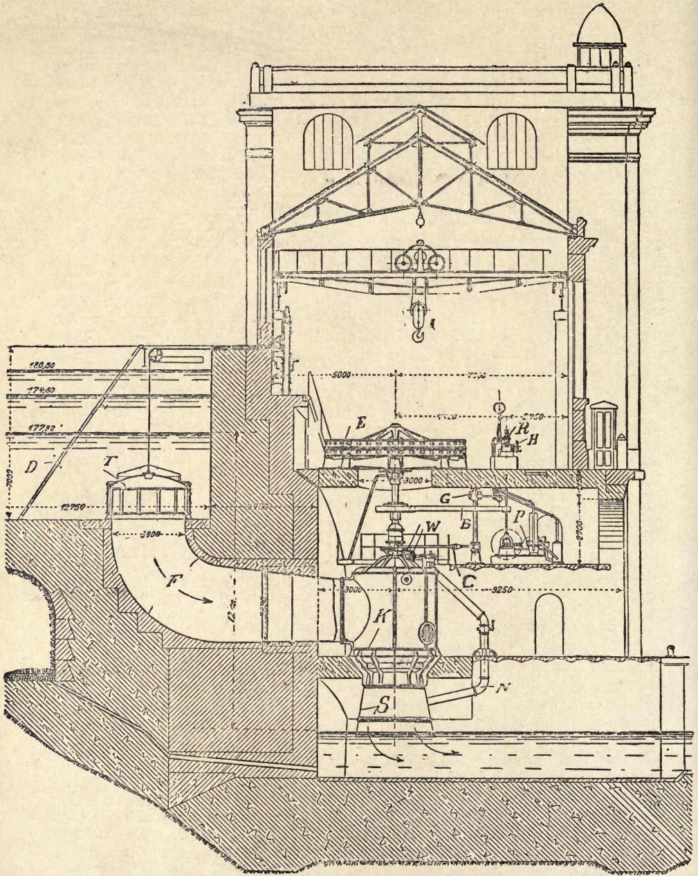
Fig. 303.—Cross-section showing General Arrangement of One of Eight Diagonal Flow Conical-wheel Turbines. (Supplied by the Escher-Wyss Company for the Cusset Electric Power Plant, Lyons, each capable of developing 1,250 H.P., at a speed of 120 revolutions per minute, with a pressure head of 39 feet.)
