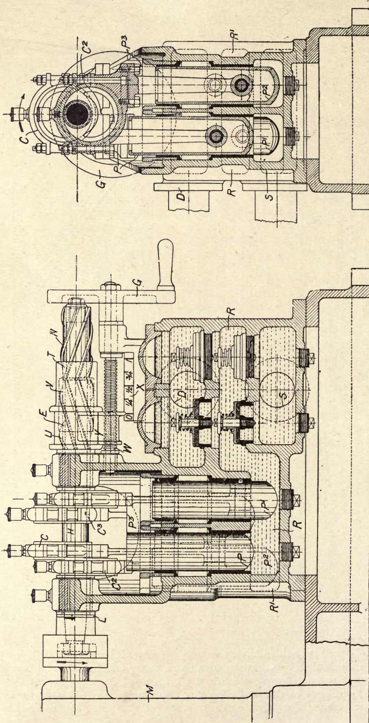
Fig. 231.—4-throw Direct-coupled Plunger-controlled Clarke-Chapman Variable-delivery Pump.
