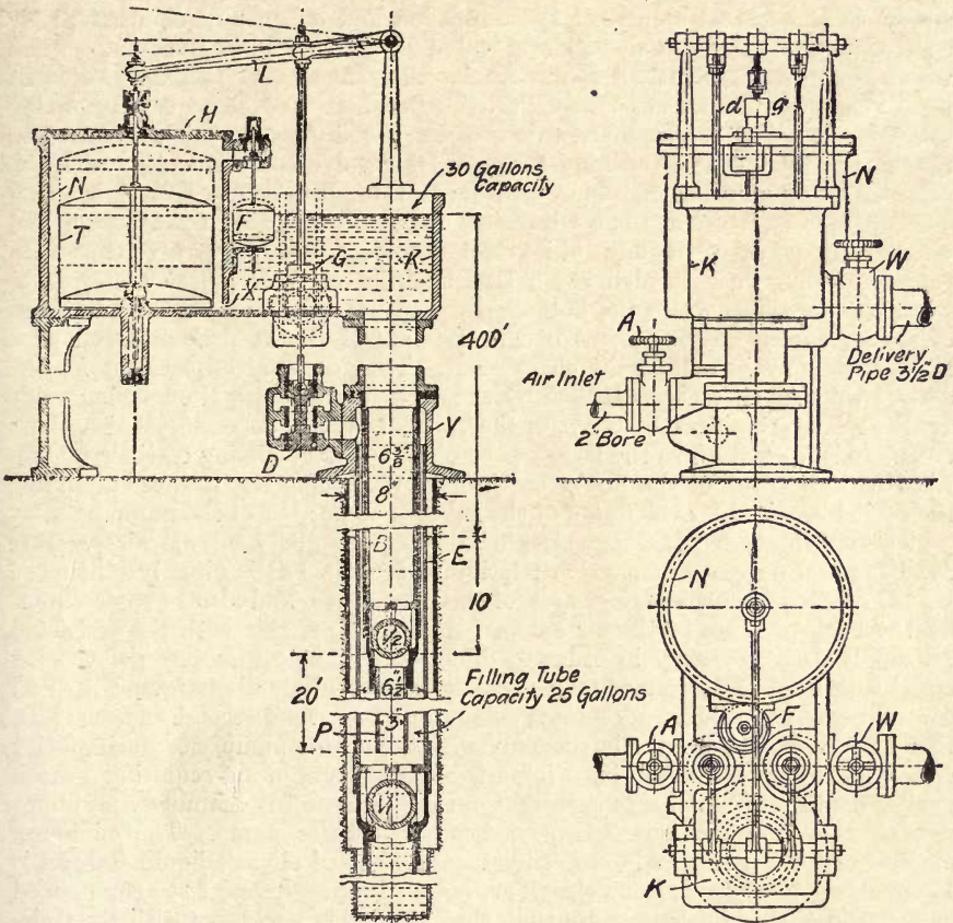
Fig. 82.—Air-displacement Borehole Pump with Automatic Float Distributor.
