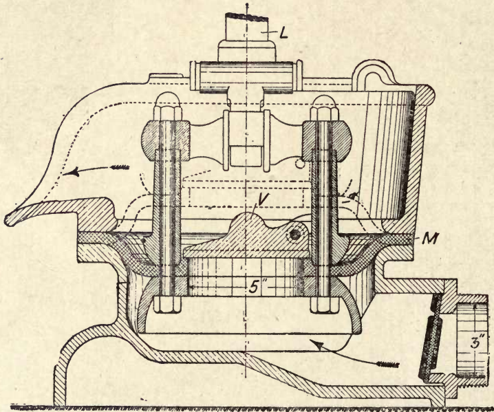
Fig. 259.—Paragon Diaphragm Pump.
