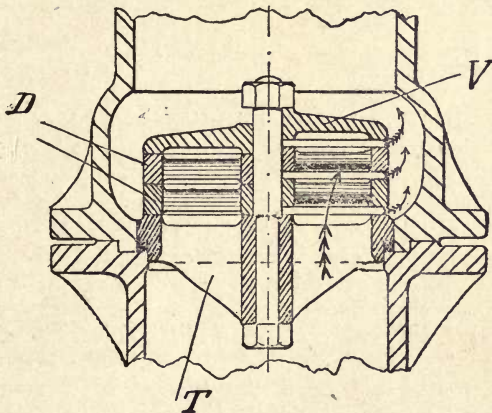
Fig. 48.—Half-sections, showing Multiple Disc Flat-seated Valves, Open and Closed.
