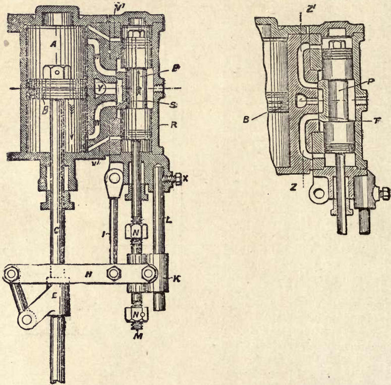
Fig. 98.—Sections of Steam End, showing Distribution in Lamont's Simplex Direct-acting Pump.
