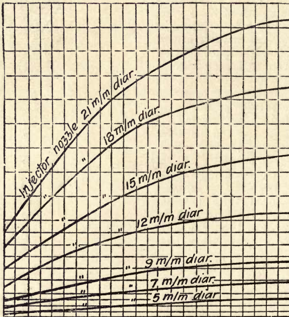
Fig. 125.—Diagram showing the Working of Boiler-feed Injectors.
