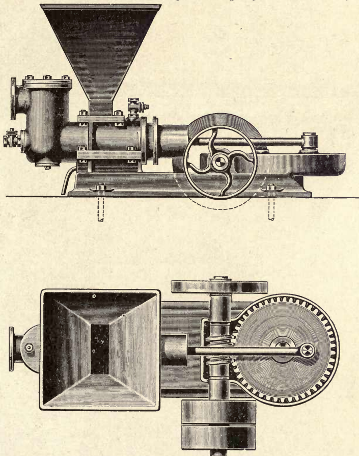
Fig. 235.—Elevation and Plan of Watson and Laidlaw's Plunger Masse-cuite Pump.
