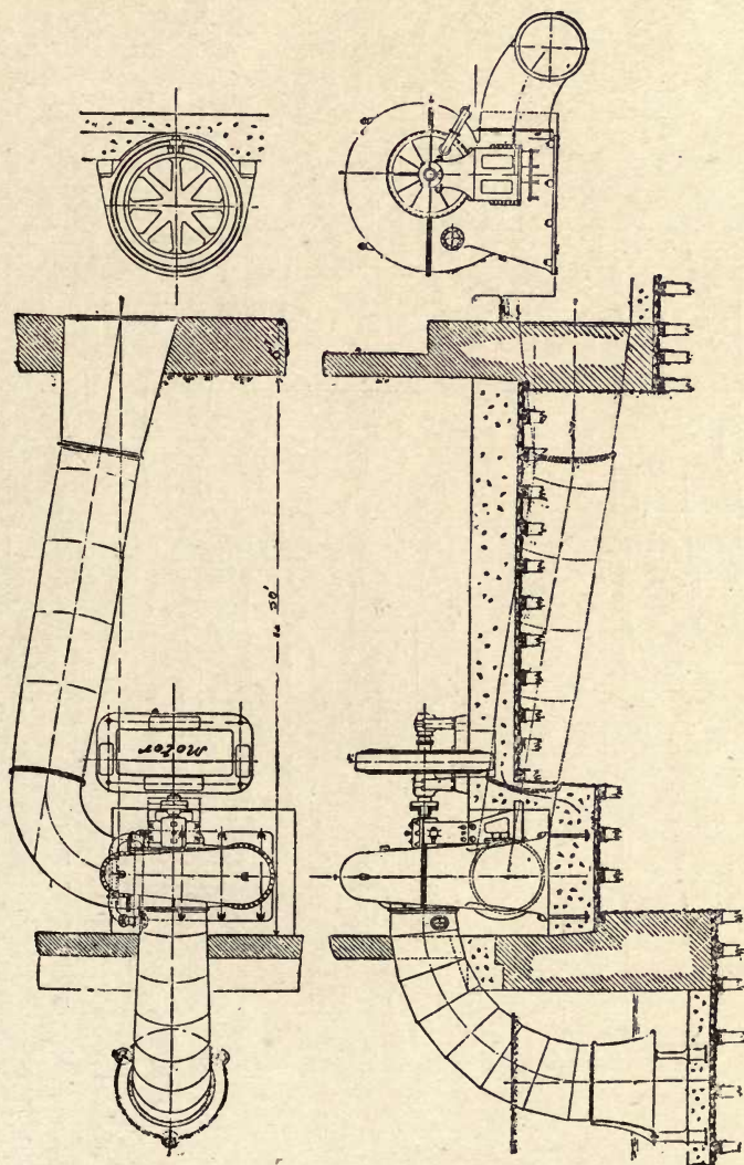
Fig. 268.—Arrangement of Electrically-driven Horizontal Drainage Pump. Capacity, 400 tons per minute.
