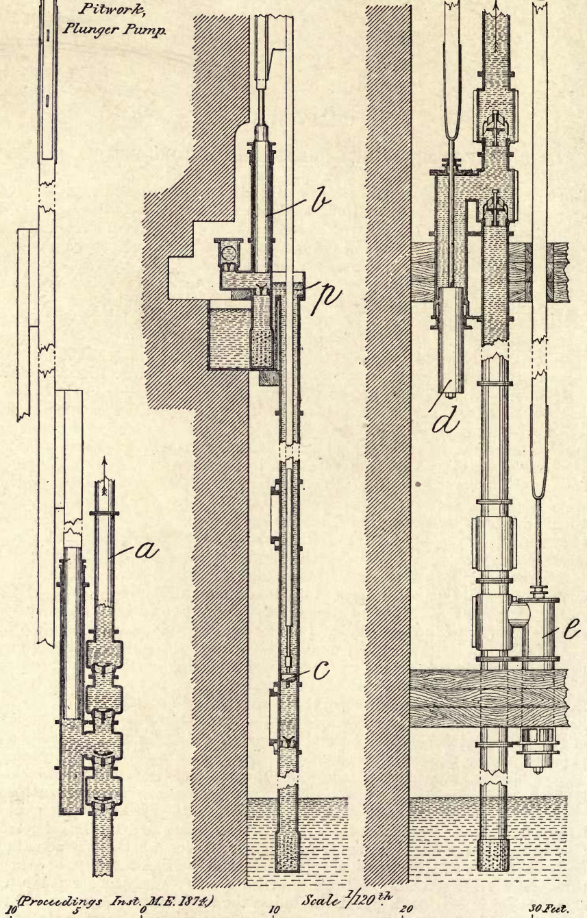
Fig. 32.—Typical Deep-level Mine Pumps.
