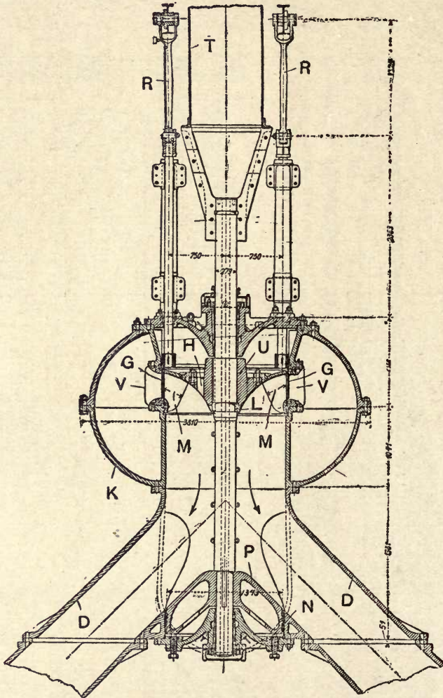
Fig. 324.—Vertical Section of "Escher-Wyss" Diagonal-flow Turbine. One of ten supplied by the I. P. Morris Company for the Niagara Falls Power Company, each capable of developing 5,500 H.P. at a speed of 250 revolutions per minute, with a pressure head of 146 feet.
