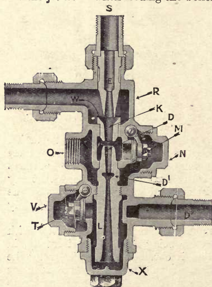
Fig. 138.—Section of Brooke Simplex Injector for use with ordinary Steam and Water Regulating Valves.
