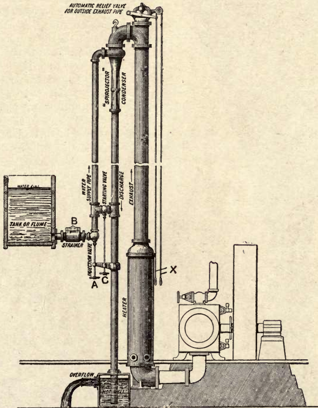
Fig. 150.—General Arrangement of Barometrical Ejector Condenser.
