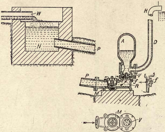
Fig. 182.—Arrangement of Drive Pipe on Glenfield Hydraulic Ram.
