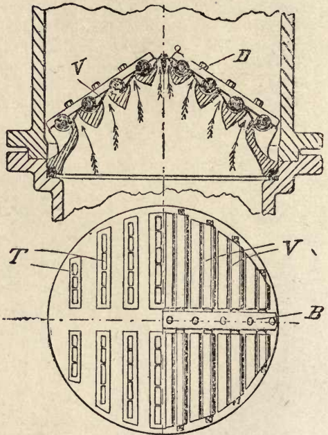
Fig. 46.—Arrangement of Spring-seated Copper Flap Gutermuth Valves.
