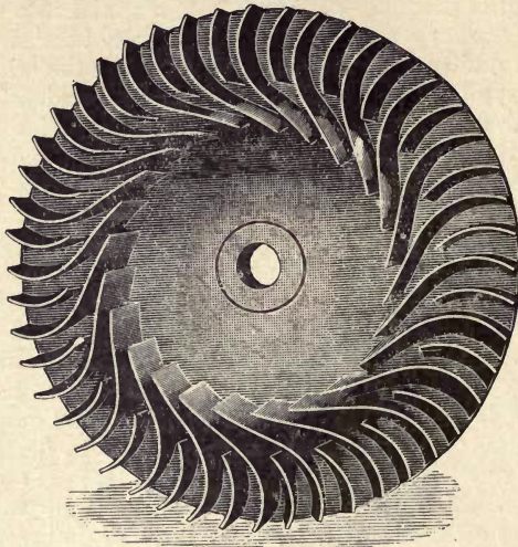
Fig. 299.—Impeller Wheel of Gilkes' Vortex Turbine.
