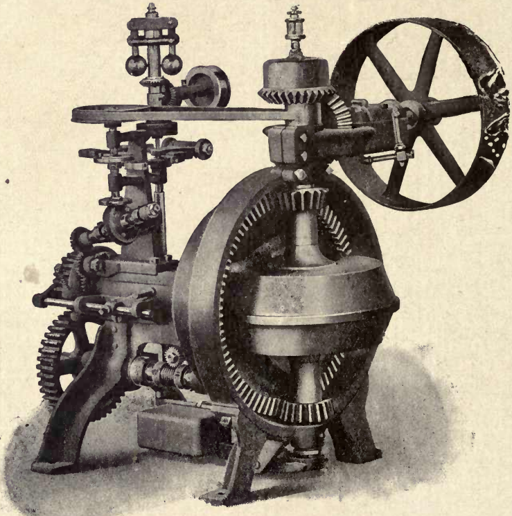
Fig. 343.—Friction-disc Quick-action Relay Turbine Governor fitted with Compensating Gear.
