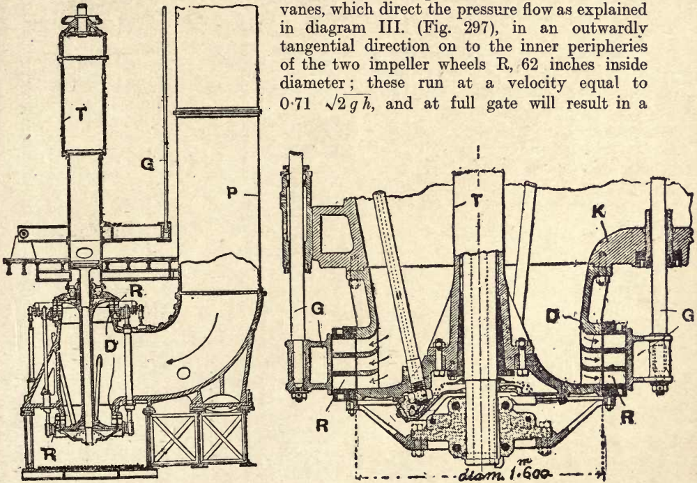
Fig. 328.—Details of Lower Impeller and Guide Ring. One of the ten 5,000 H.P. twin outward-flow vertical turbines for the Niagara Falls Power Company, showing the cylindrical sliding regulator sluice.
