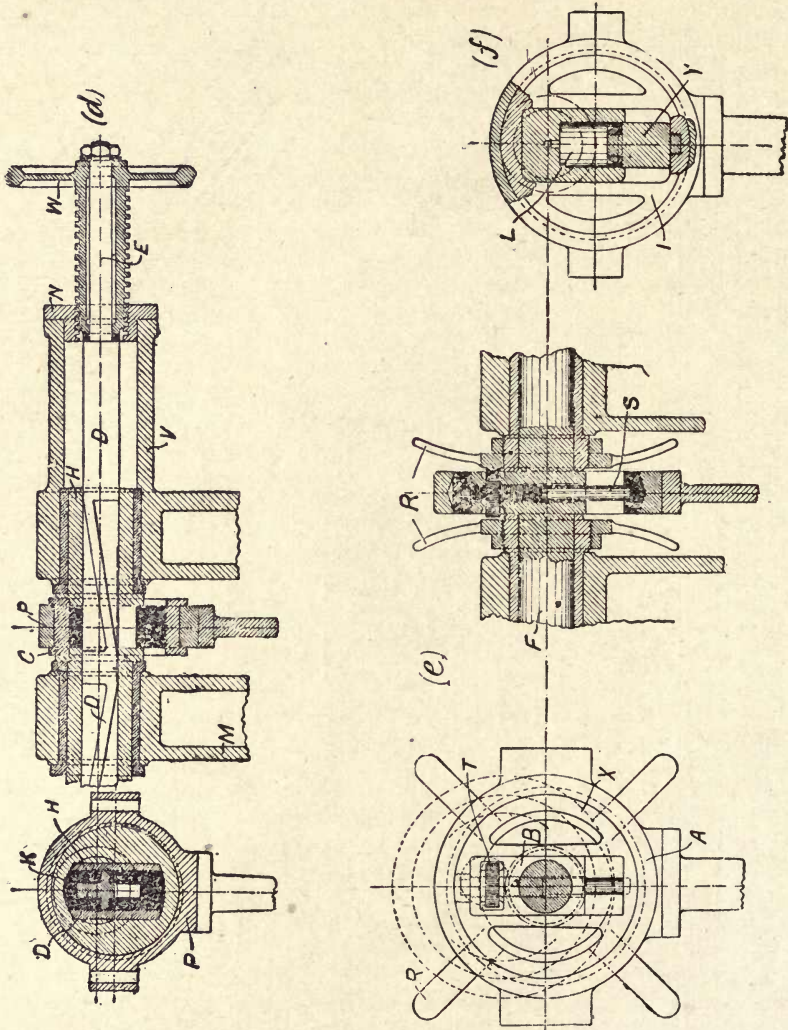
Fig. 222.—Examples of Variable-throw Eccentrics.
