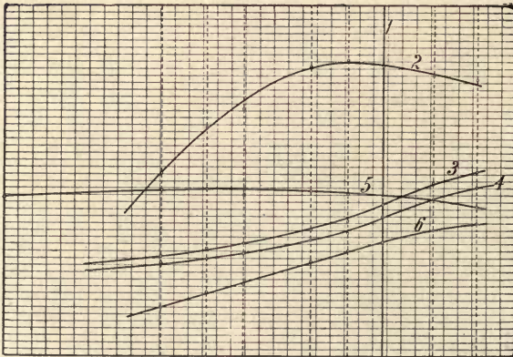
Fig. 286.—Diagrams showing Output, Power, and Efficiency of Sulzer Electrically-driven Sinking Pump.
