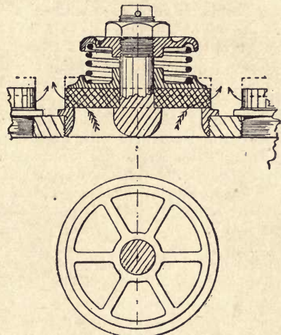
Fig. 56.—Modern Form of Suction or Delivery Composite Disc Valve, arranged in Multiple Series.
