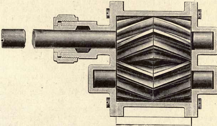
Fig. 246.—Willesten-Albany Double Helical Pump.
