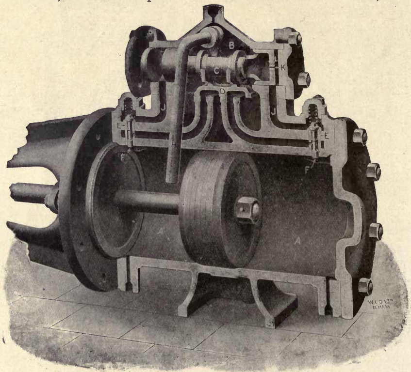
Fig. 104.—Section of Steam Cylinder of Tangye Simplex Pump.
