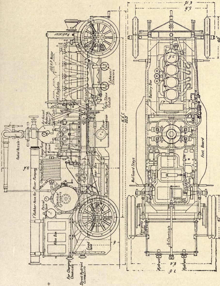
Fig. 203.—Petrol Motor Fire Engine with 2-throw Double-acting Force Pump for Tottenham.
