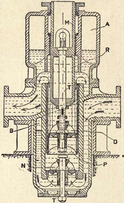
Fig. 204.—Ram and Plunger Fire Pump (Rigg).
