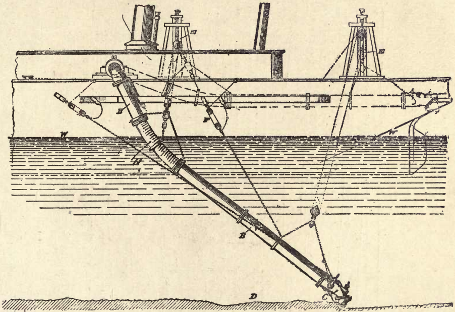
Fig. 271.—Arrangement of Suction Pipe on Dredging Steamer, showing Flexible Connection.
