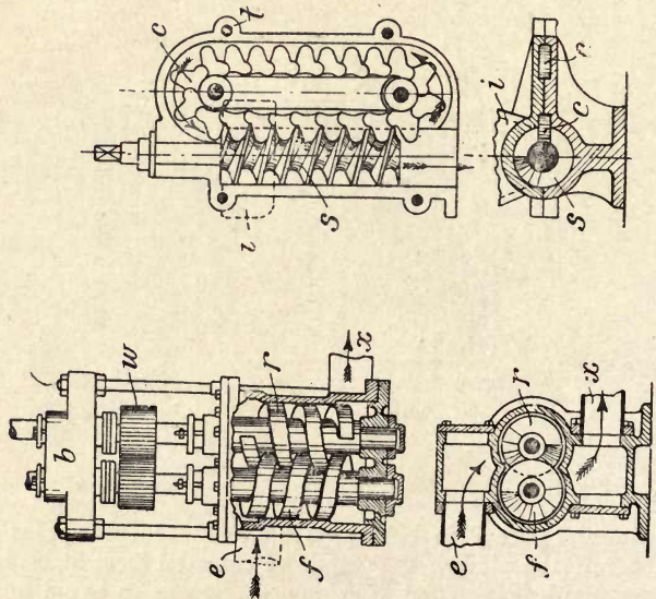
Fig. 237.—Sectional Views of the Quinton and Triben Archimedean Pumps for Semi-fluids.
