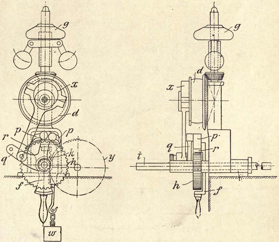
Fig. 344.—Turbine Governor with Ratchet Relay Movement.
