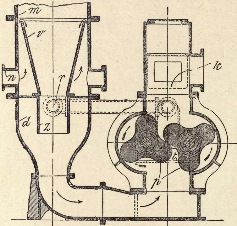
Fig. 170.—Cylindrical Rotary Vacuum Pump.
