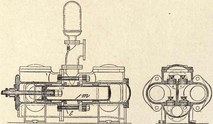
Fig. 115.—Water End of Epping-Carpenter Duplex Pump, with Inside-packed Ram Plungers.
