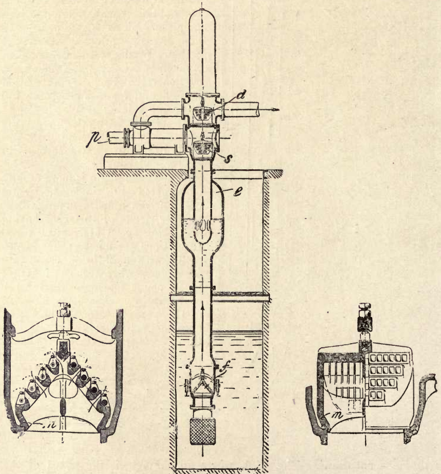
Fig. 214.—Details of a Differential Pump at the Woodford Pumping Station fitted with Gutermuth Valves.
