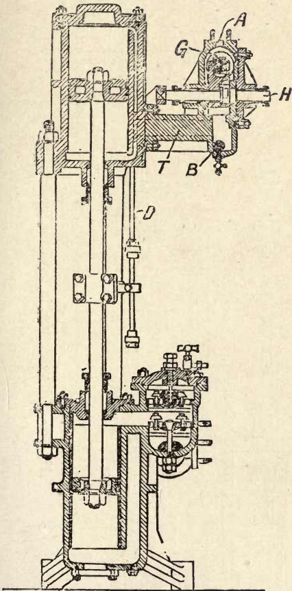
Fig. 94.—Sectional Elevation of Clarke-Chapman Direct-acting Feed Pump.
