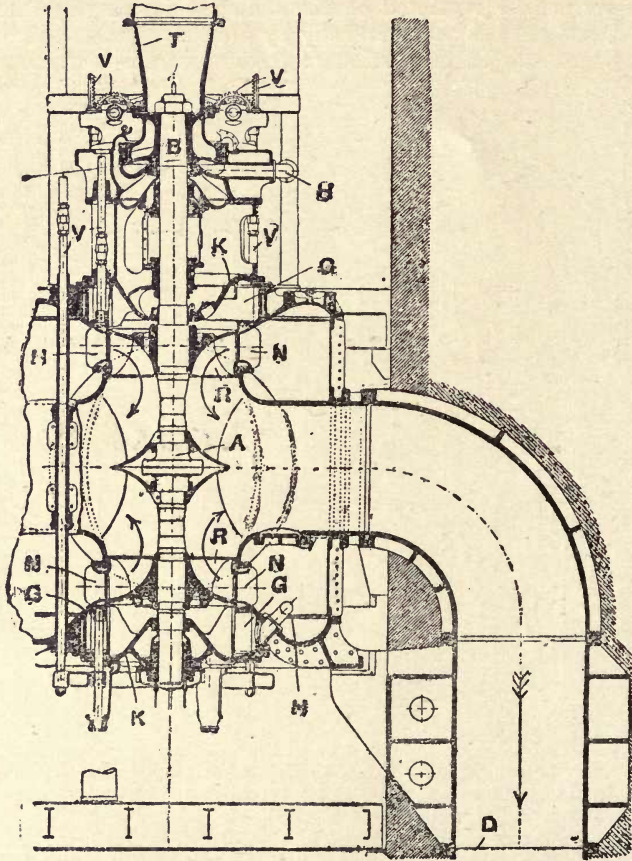
Fig. 322.—Cross-section of a 10,000 H.P. Twin Inward-flow Vertical Turbine for the Canadian Niagara Power Company. Pressure head, 133 feet; revolutions, 250 per minute; speed control by cylindrical gates.
