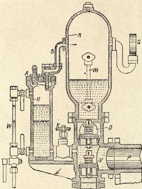
Fig. 178.—Wipperman Air Chamber Charger for Hydraulic Engines and Pumps.
