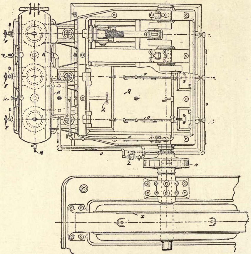
Fig. 217.—Plan of Fraser and Chalmers' Electrically-driven Dirt-tet-coupled High-speed Pump
