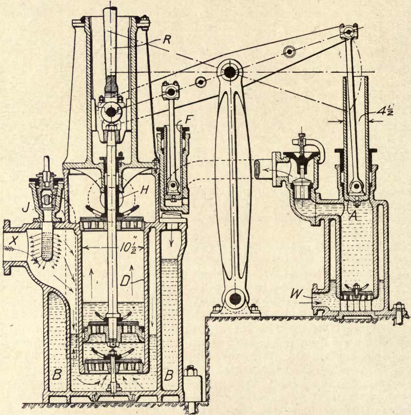
Fig. 152.—Jet Condenser Air Pump combined with Circulating and Feed Pumps.
