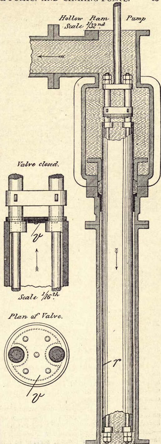
Fig. 33.—Hollow-ram Mine Pump.
