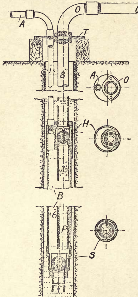
Fig. 81.—Air-displacement Artesian Oil-Well Pump.
