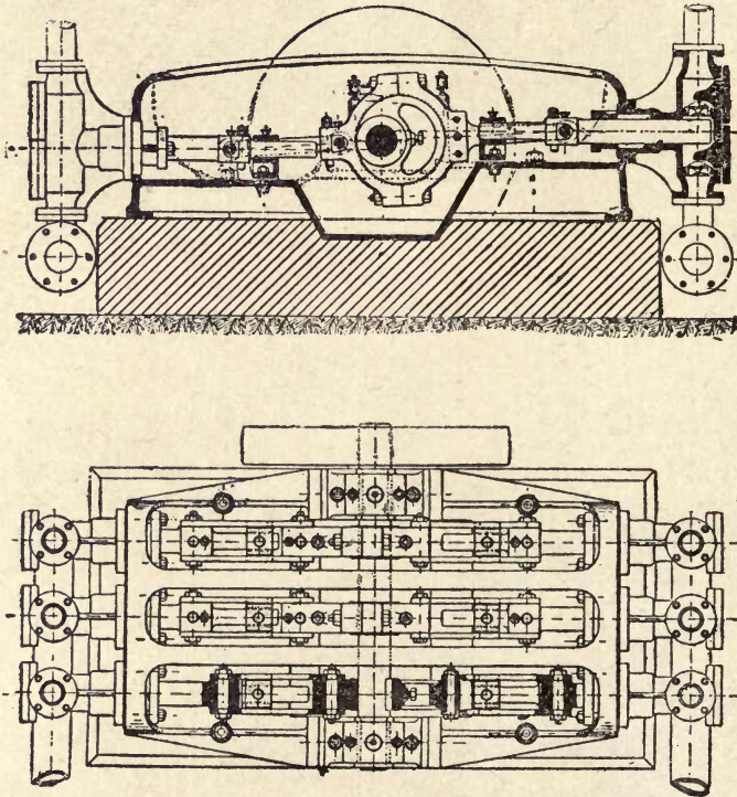
Figs. 121 and 121a.—Three-throw Belt-driven Feed Pump.
