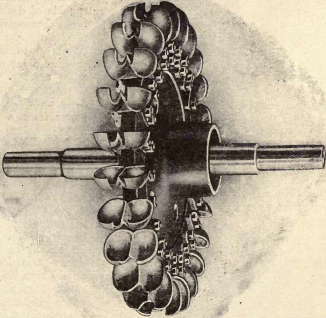
Fig. 333.—Victoria Impulse or Jet-action Turbine Wheel.
