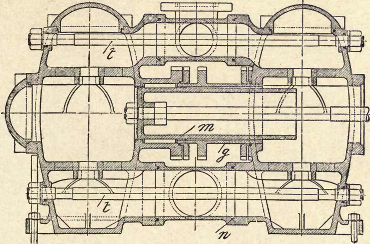
Fig. 116.—Section of Heisler Duplex Pressure Pump, with Water-sealed Inside-packed Plunger.
