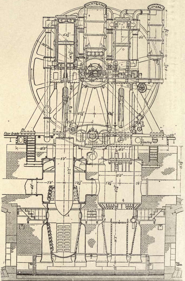
Fig. 20.—Sectional Elevations of Three-cylinder Rotative Beam Engine with T...
