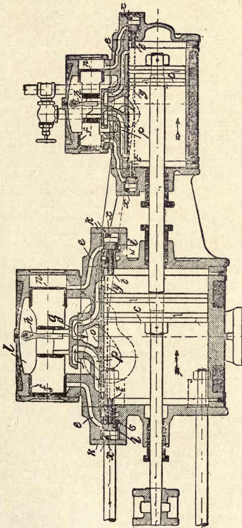
Fig. 93—Section of Steam Cylinders of "Cameron" Compound Direct-acting Pump, showing Method of actuating the Steam-thrown Valves
