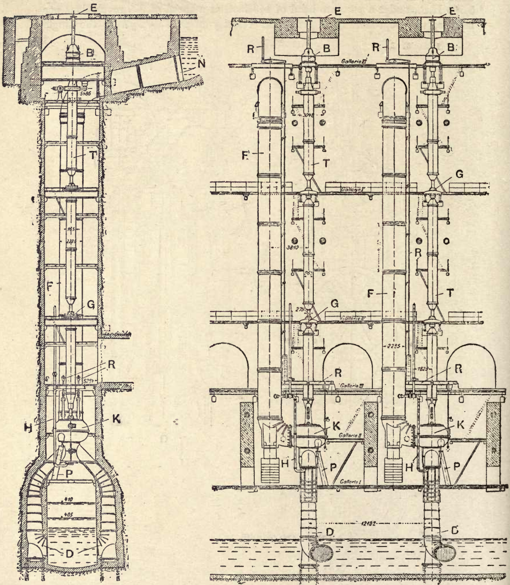
Fig. 326.—Sectional Views showing General Arrangement of "Escher-Wyss" 5,500 H.P. Diagonal-flow Single-wheel Turbines in Power House No. 2 of the Niagara Falls Power Company.
