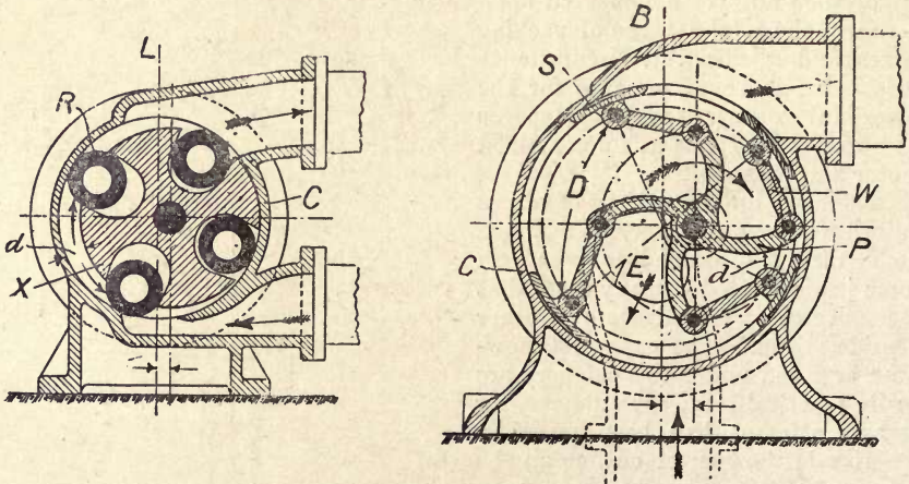
Fig. 252.—Cross-sectional Elevations of the Colebrook and Oddie Rotary Pumps.
