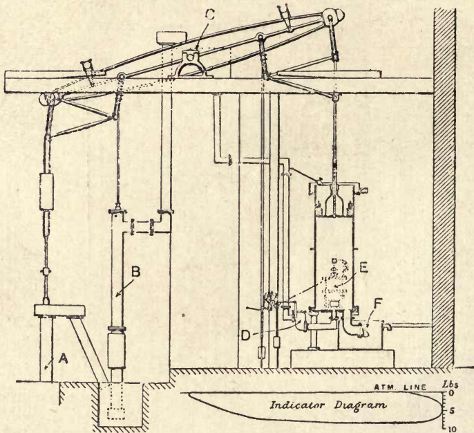
Fig. 3.—Improved Newcomen Engine.
