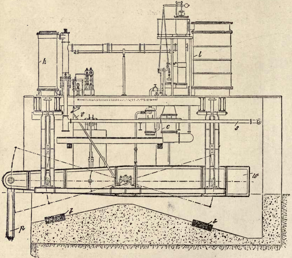
Fig. 8.—Davey Compound Beam Pumping Engine (Cornish Type).
