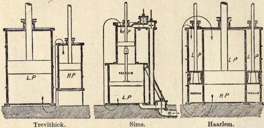
Fig. 5.—Early Types of Compound Cylinders used in Pumping Engines.
