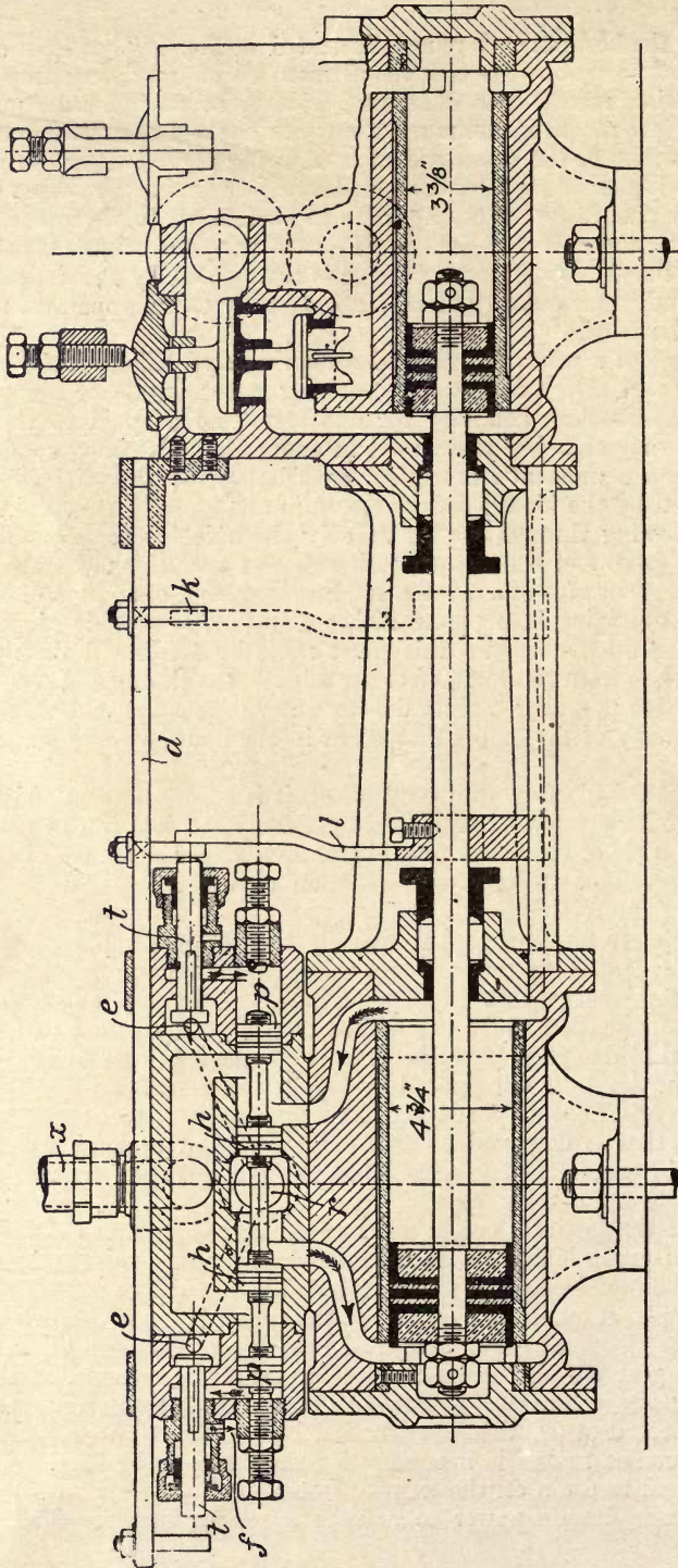
Fig. 179.—Hydraulic Relay Direct-acting Pump.
