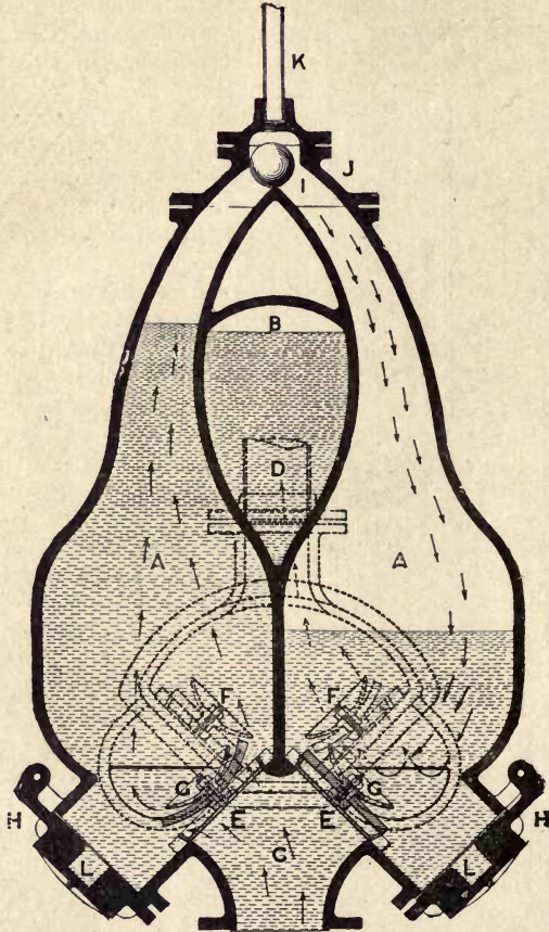
Fig. 41.—Pulsometer Sinking Pump.
