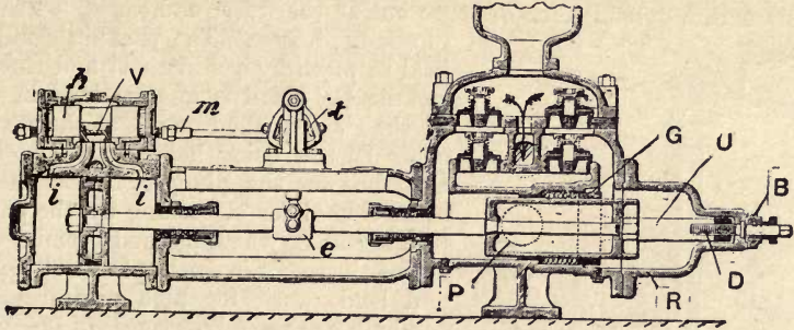
Fig. 105.—Simplex Pump with Gland-packed Plunger
