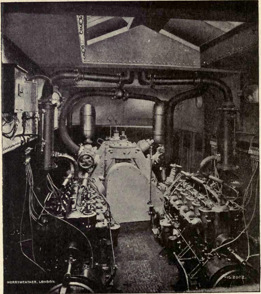
Fig. 202.—Engine Room, showing a Pair of Hatfield Pumps on a Fire Float driven by Two 6-cylinder Petrol Motors. Capacity, 1,200 Gallons per Minute.
