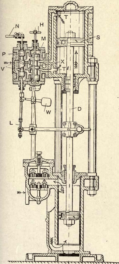
Fig. 99.—Nichols' Patent Simplex Pump.
