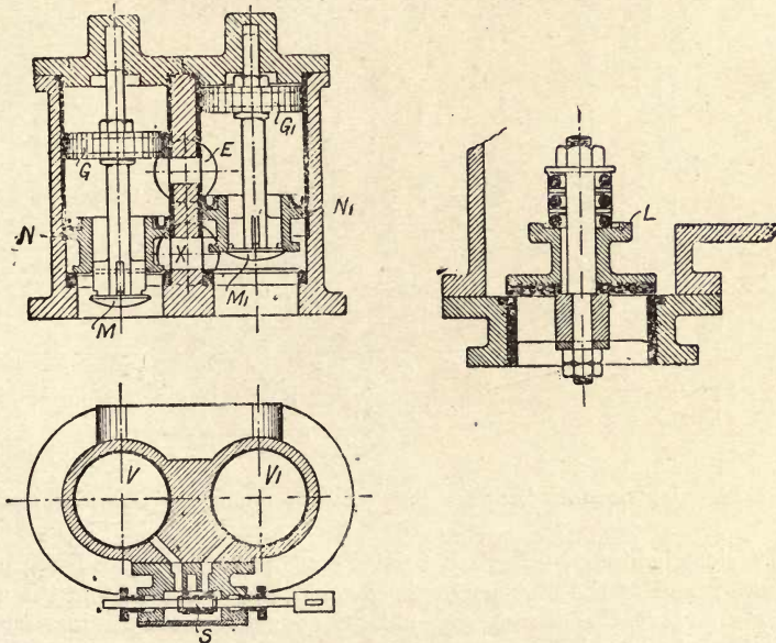
Fig. 177.—Details of Engine and Pump Valves for Hydraulic Mine Pump.
