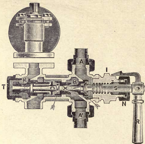
Fig. 137.—White's Re-starting Injector.
