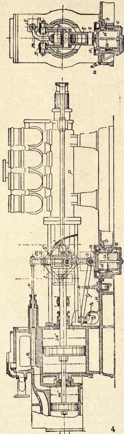
Fig. 26.—“Oddesse Compound,” 14 × 24 × 8 × 18 inches, Mine Pumping Engine, fitted with Air-spring Compensator.
