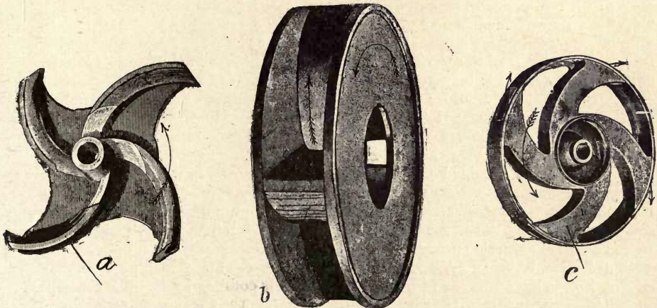
Fig. 274.—Impellers used in the Morriss Centrifugal Pumps.
