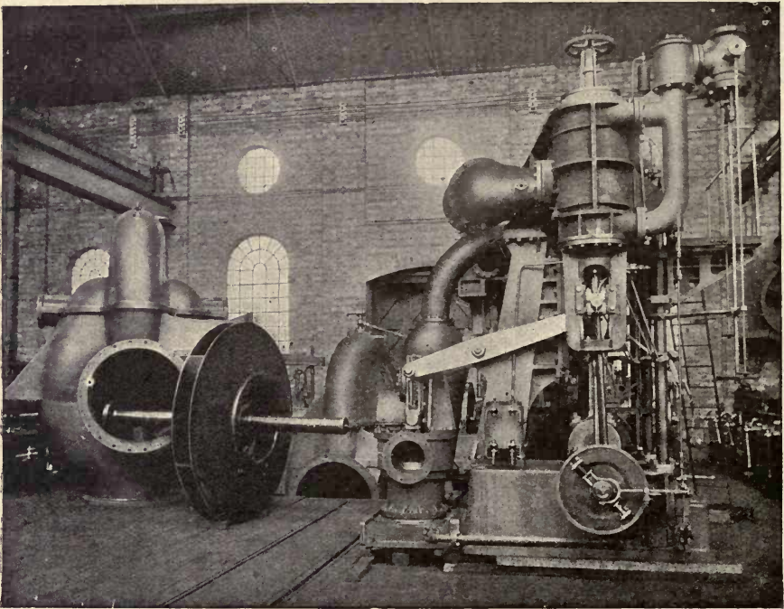
Fig. 267.—Two 45-inch “Conqueror” Centrifugal Pumps, each driven by a 500 B.H.P. Engine with Jet Condensing Plant. Supplied to the Mersey Docks and Harbour Board for Herculaneum Dock, Liverpool. Capacity of each pump, 140 tons per minute.
