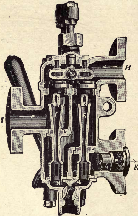
Fig. 134.—Körting Double Tube Injector
