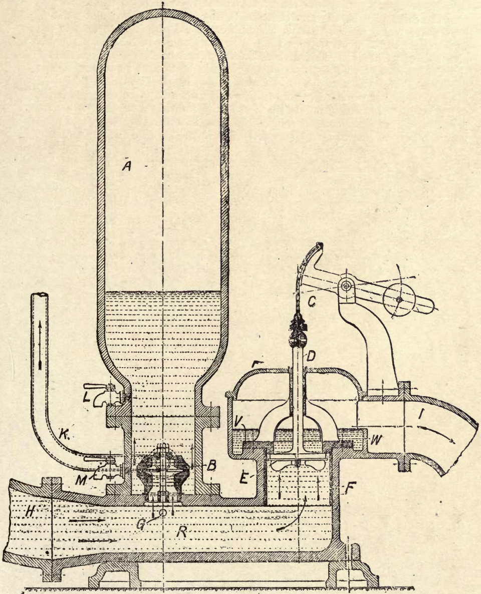
Fig. 181.—Keith's Hydraulic Ram.
