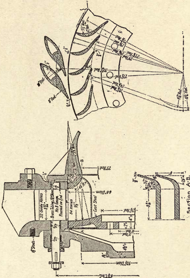
Fig. 313.—Details of Swivel Guide Vanes and Impeller for 10,000 H.P. Single-wheel Turbine.
