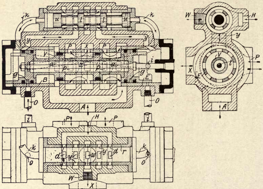
Fig. 190.—Hydraulic Distributor for Twin Air-displacement Pump ( Butler ).
