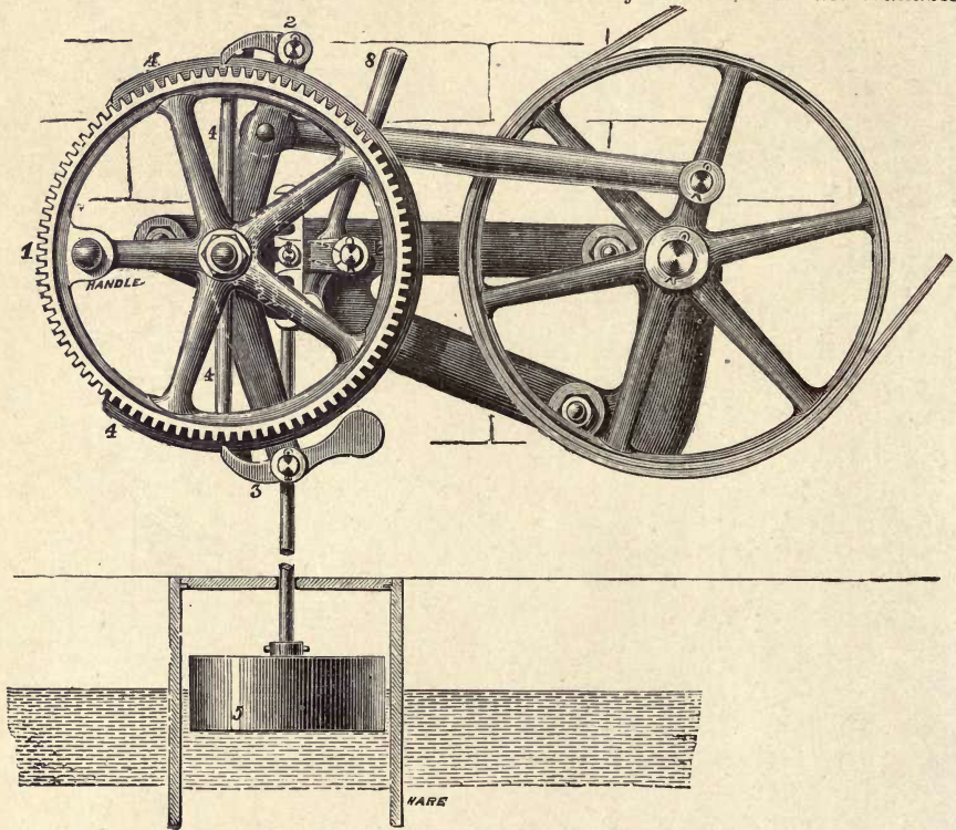
Fig. 345.—"King" Float-controlled Turbine Governor.
