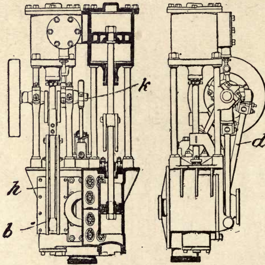
Fig. 196.—Merryweather Fire Pump (Flywheel Type).
