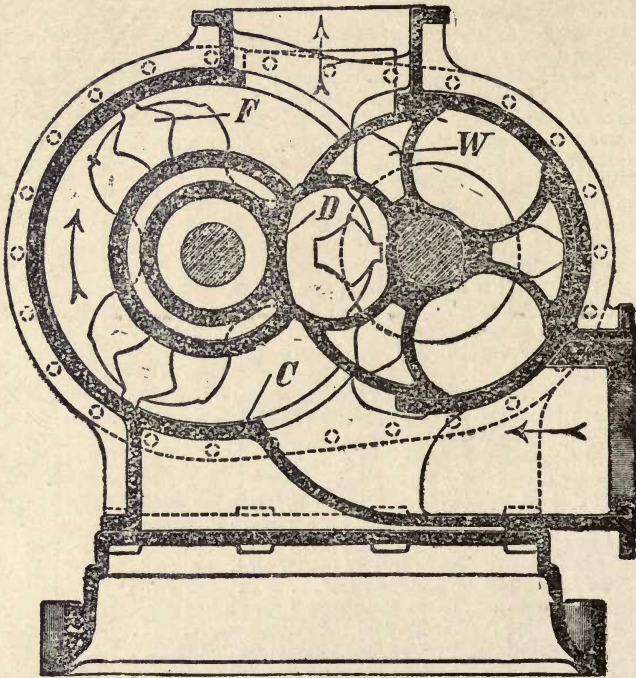
Fig. 244a.—Sectional Elevation of Enke Pump, with a capacity of 200,000 gallons per hour at 60 revolutions per minute, against a head of 75 feet.
