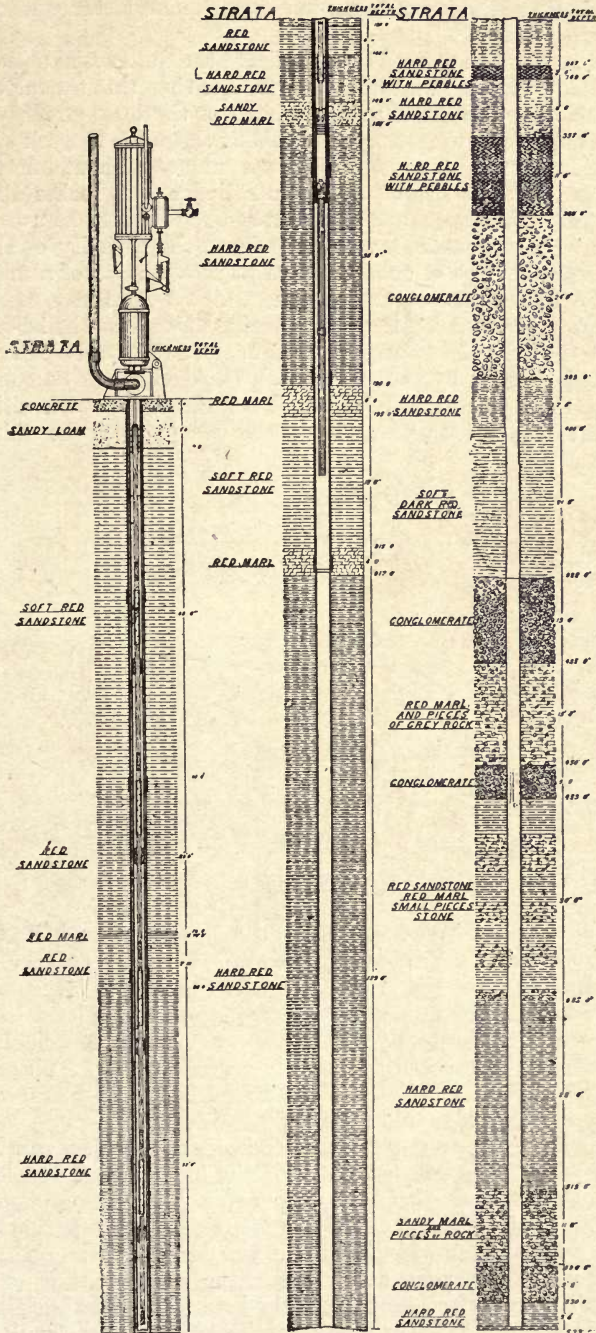
Fig. 70.—Section of Artesian Well, showing Direct-acting Steam Pump.
