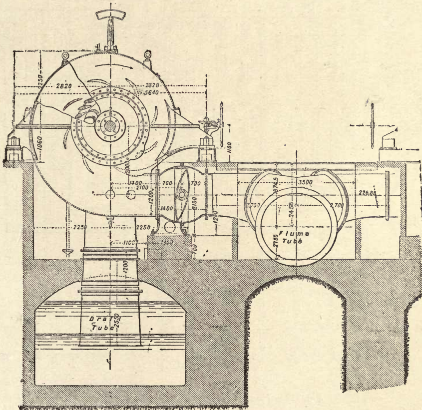
Fig. 315.—Elevation of One of a Pair of Single-wheel Radial axial-inflow Horizontal Turbines, supplied by Ganz & Co., to develop 2,000 H.P. on a pressure head of 90 feet, at Valtellina, Italy.
