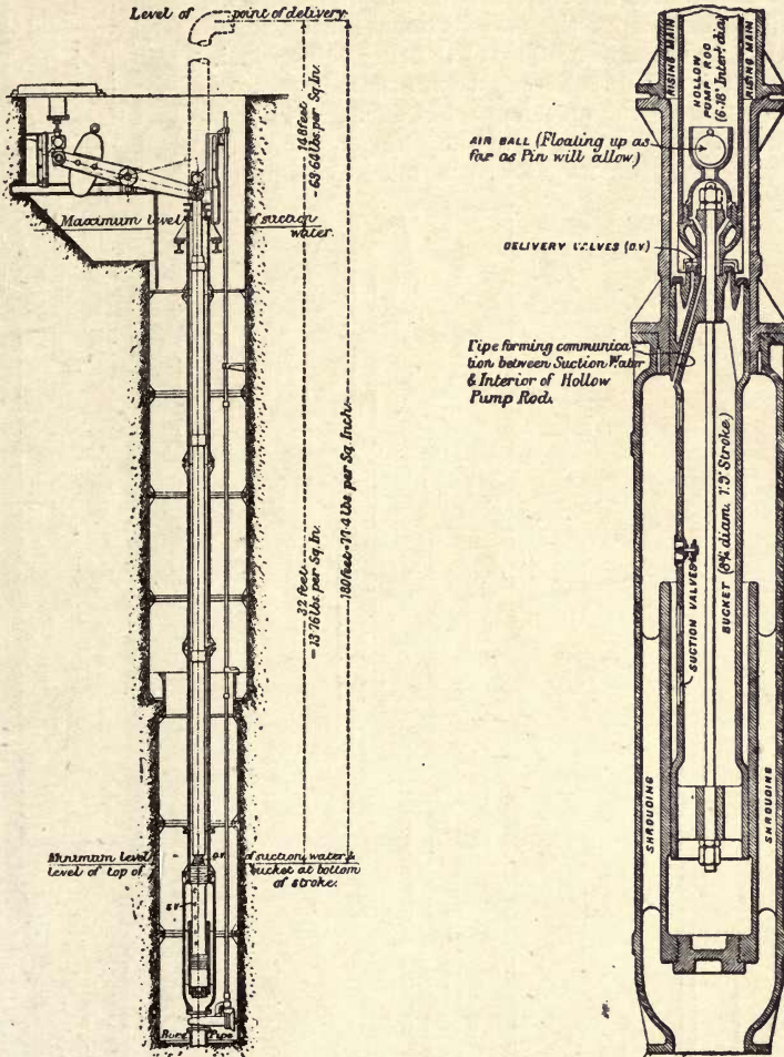
Fig. 64.—Ashley Balanced Deep Well Pump.
