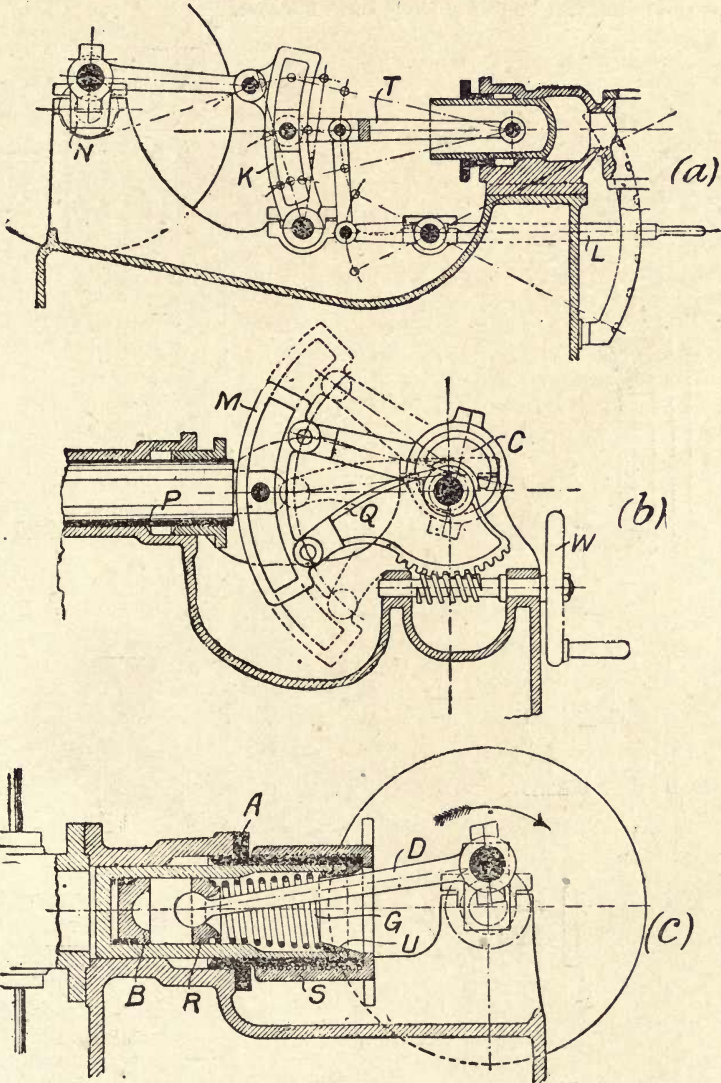
Fig. 221.—Pump Arrangements, showing Link and Lost Motion Methods for obtaining Variable Delivery at Constant Speeds
