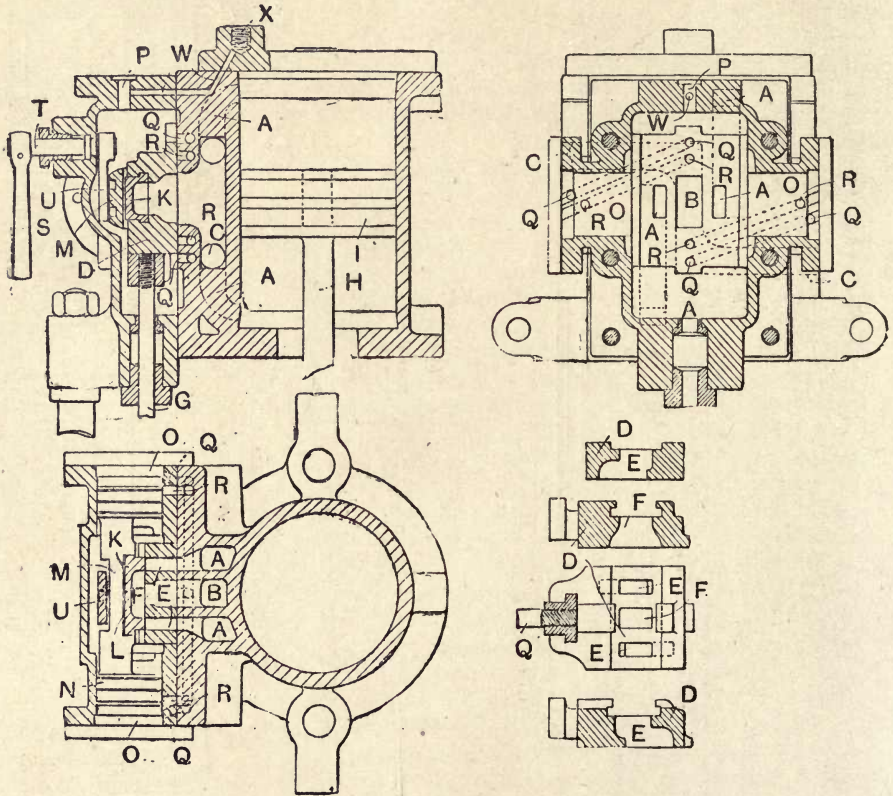
Fig. 101.—Pearn's Simplex Valve Gear.
