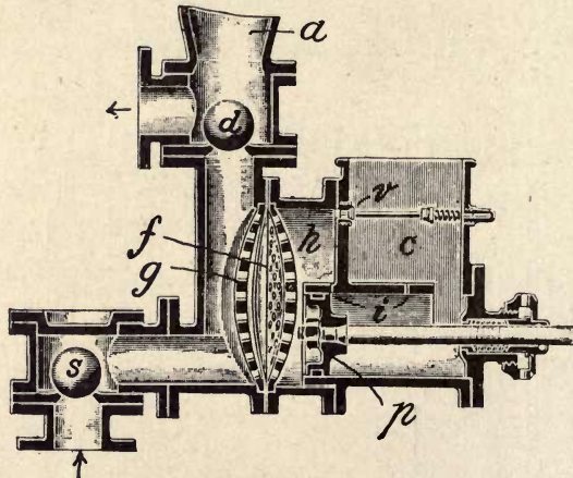
Fig. 123a.—Belt-driven Diaphragm Pump for Corrosive Liquids.
