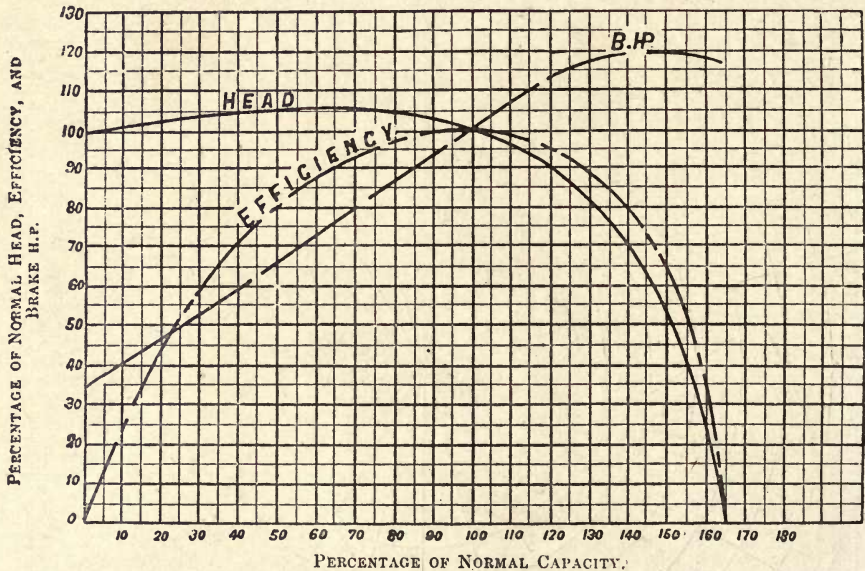
Fig. 277.—Diagram showing Variable Delivery of Low-lift Centrifugal Pump under throttled Discharge Control.
