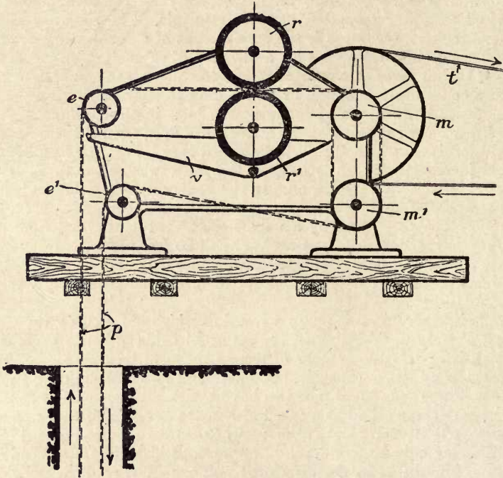
Fig. 84.—Leinweber Endless Band Pump for Raising Oil.
