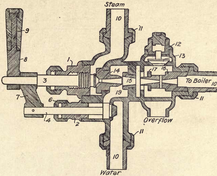
Fig. 129.—Buffalo One-movement Injector.
