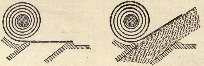
Fig. 213.—Section of 16-coiled Spring Flaps used in Gutermuth Suction and Delivery Valves for Fraser Chalmers' High speed 3-throw Pump.
