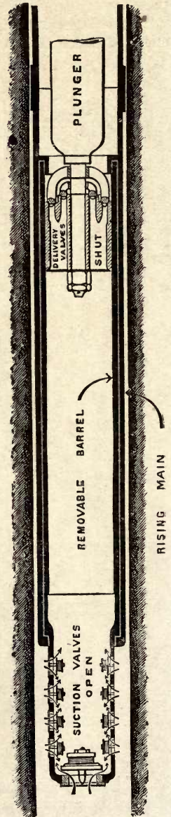
Fig. 66.—Modified Form of Ashley Deep-level Pump with Removable Barrel.
