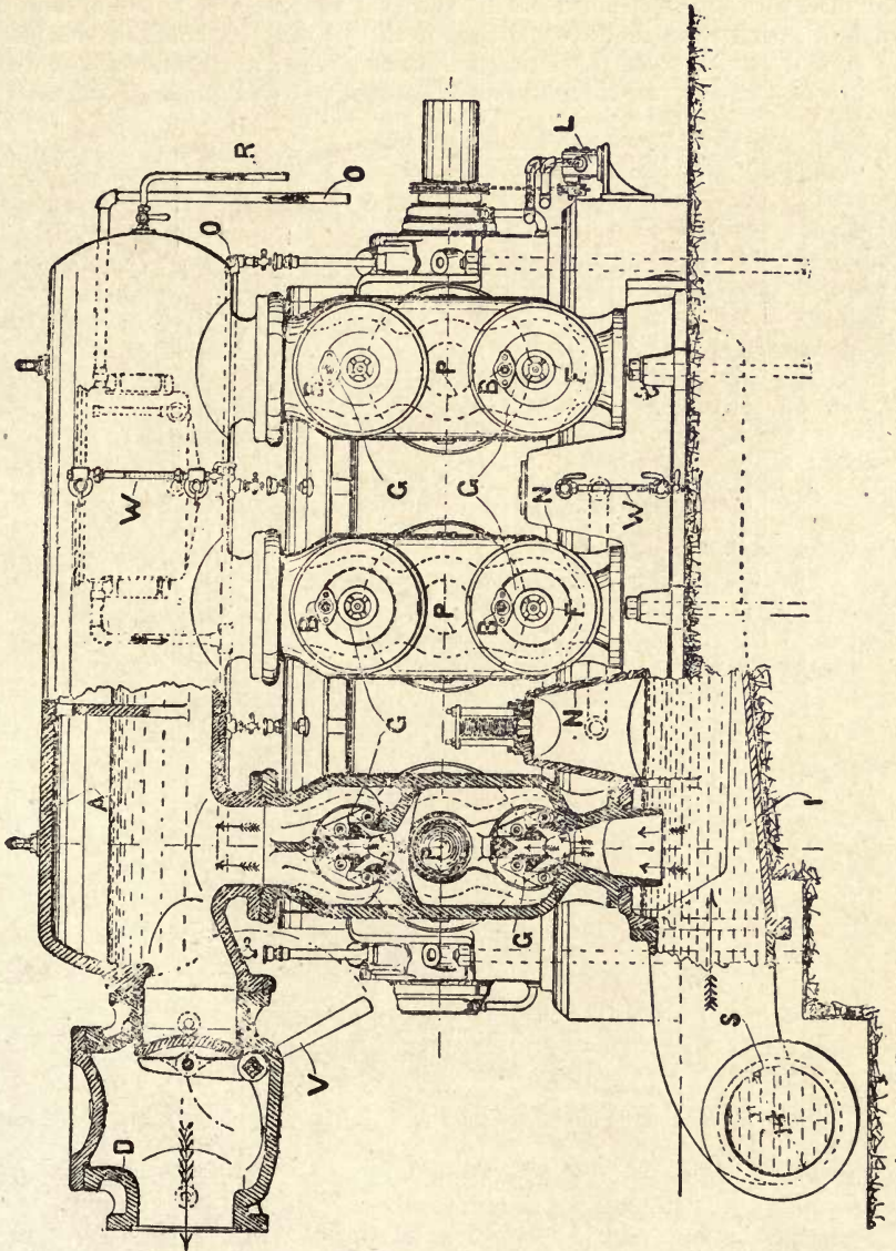
Fig. 216.—End Elevation of Fraser and Chalmers' 3-throw High-speed Pump.
