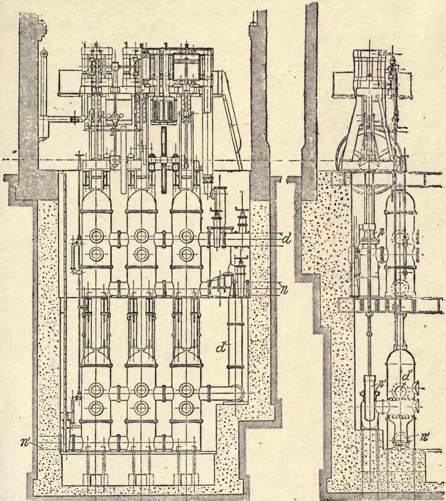
Fig. 15a.—Sectional Elevations of Three-crank Pumping Engines fitted with separate Sets of High- and Low-service Ram Plungers, for Rosario Waterworks, Argentina.
