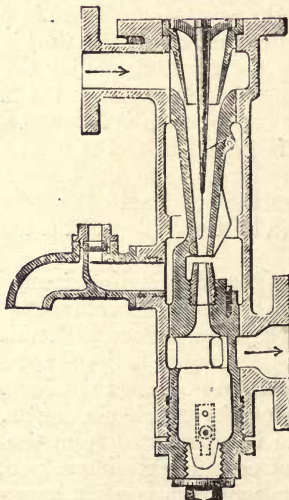
Fig. 141.—Schäffer and Budenberg Exhaust Injector.
