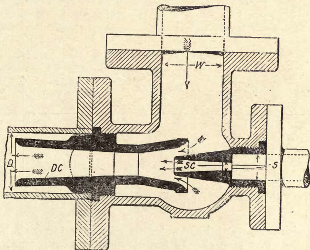
Fig. 143.—White's Jet Pump.
