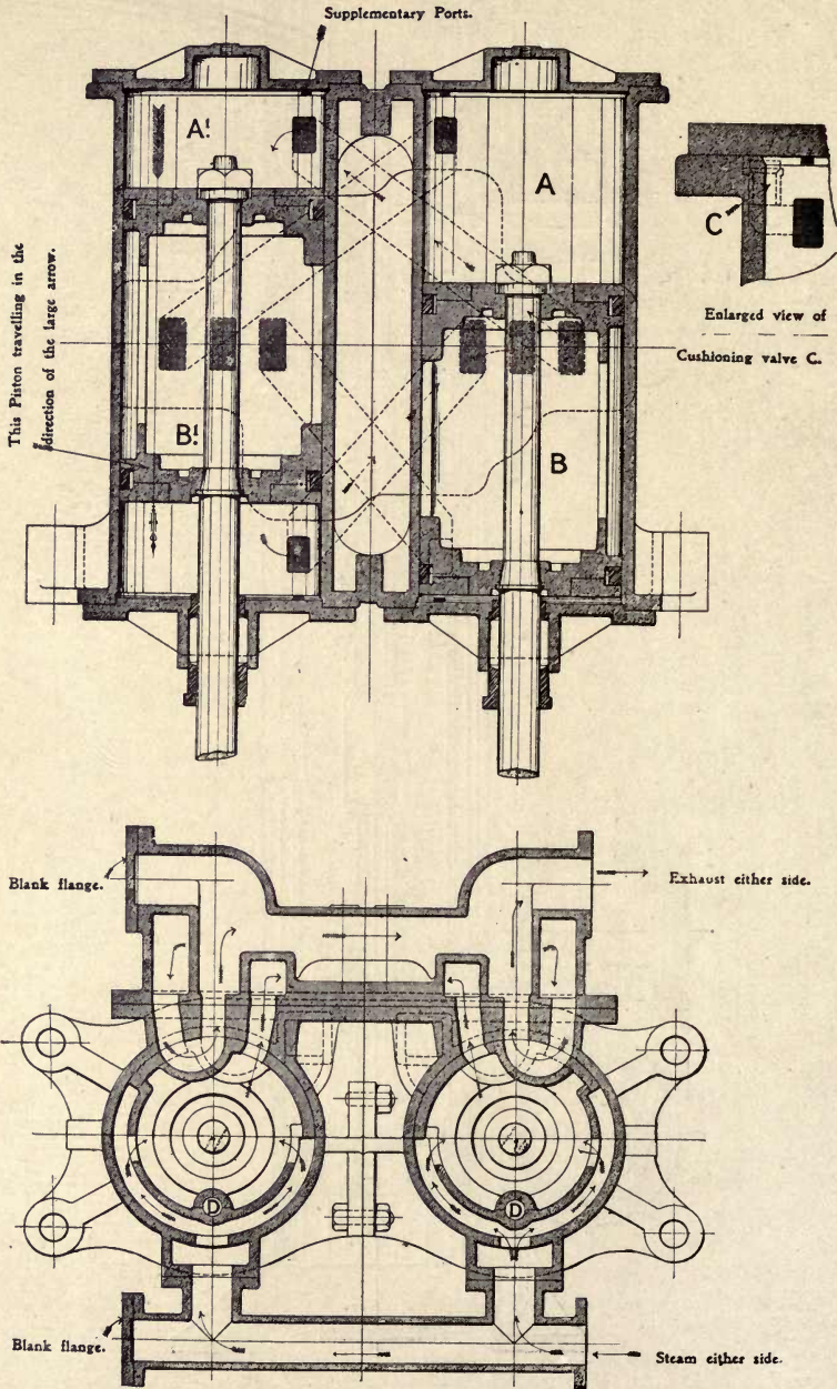
Fig. 110a.—Sectional Elevation and Plan of Steam Cylinders of Mumford Valveless Feed Pump.
