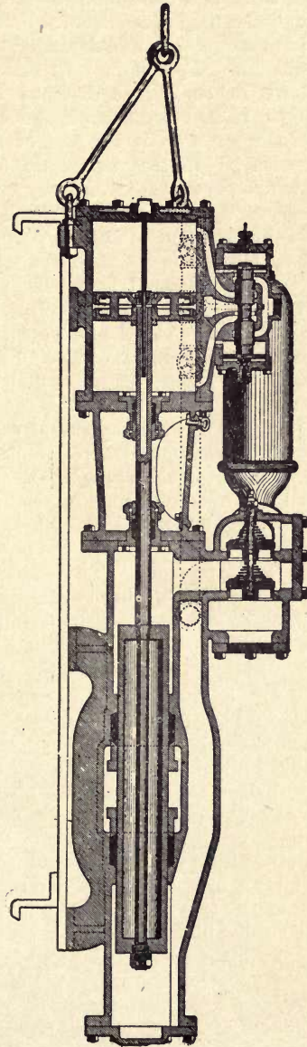
Fig. 38.—Marsh Sinking Pump.
