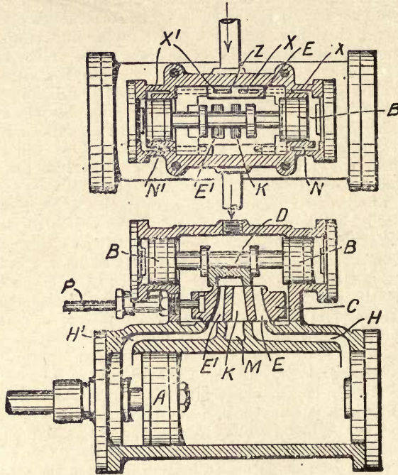
Fig. 86.—Sectional Views of Cylinder, showing Steam Distribution in Blake Direct-acting Pump.
