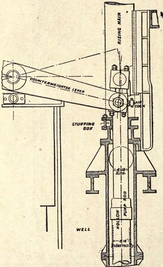
Fig. 65.—Details of Ram Plunger used in Ashley Double-acting Balanced-action Deep-well Pump.
