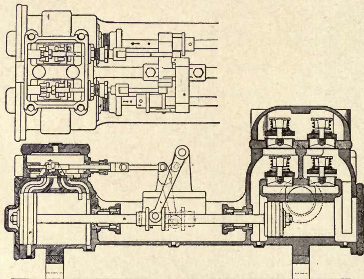
Fig. 109.—Deane General Service Pump, showing Worthington Duplex Valve Traversing Action.
