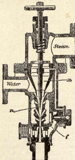
Fig. 142.—Mansfield Exhaust Steam Injector.
