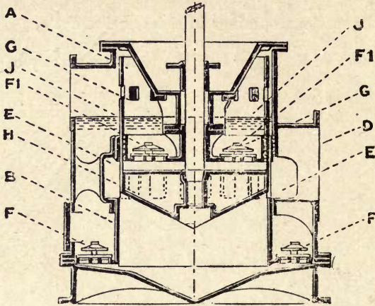
Fig. 161.—Caird and Rayner's Double-acting Air Pumps constructed without Foot or Bucket Valves on the Zylinderlast System.
