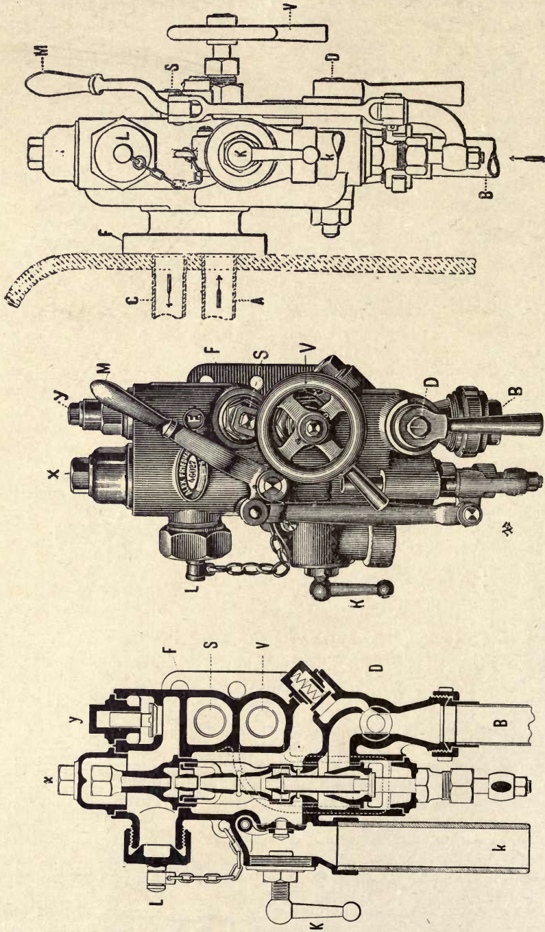
Fig. 131.—Friedmann Re-starting Boiler-fed Injector (Locomotive Type).
