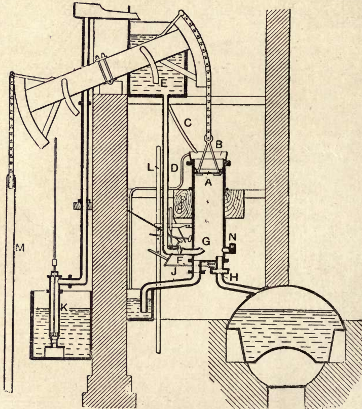
Fig. 1.—Early Type of "Newcomen" Pumping Engine.
