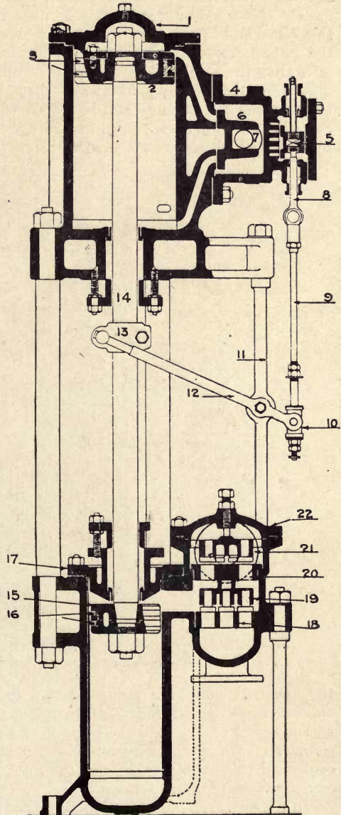
Fig. 91.—Caird & Rayner Feed Pump.
