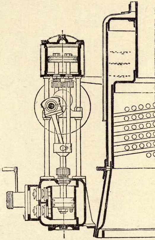
Fig. 195.—Sectional Elevation of Shand-Mason Fire Engine and Boiler
