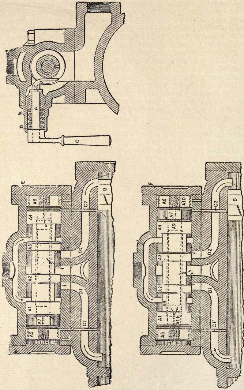
Fig. 108.—Sections showing details of "Wilson-Snyder" Automatic Steam Valve for Horizontal Simplex General Service Pumps,
