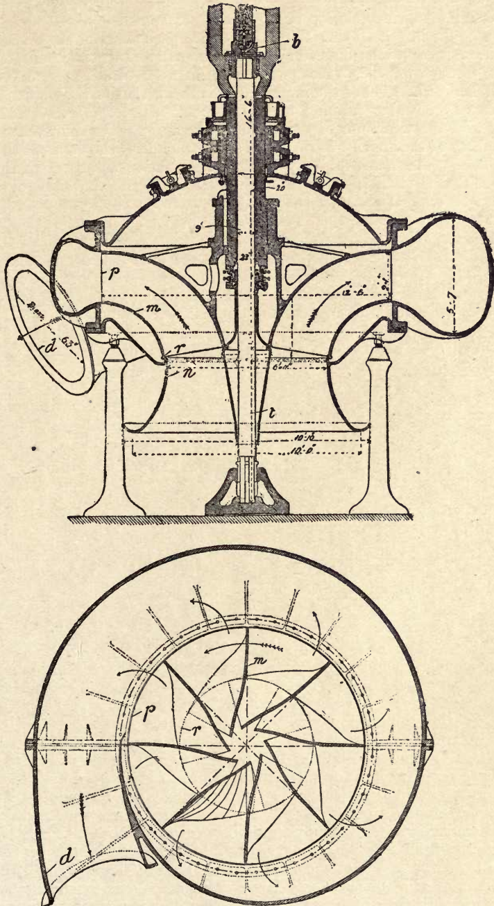
Fig. 262.—Farcot Vertical Centrifugal Irrigation Pump. Capacity, 6 tons per second, raised 10 feet.
