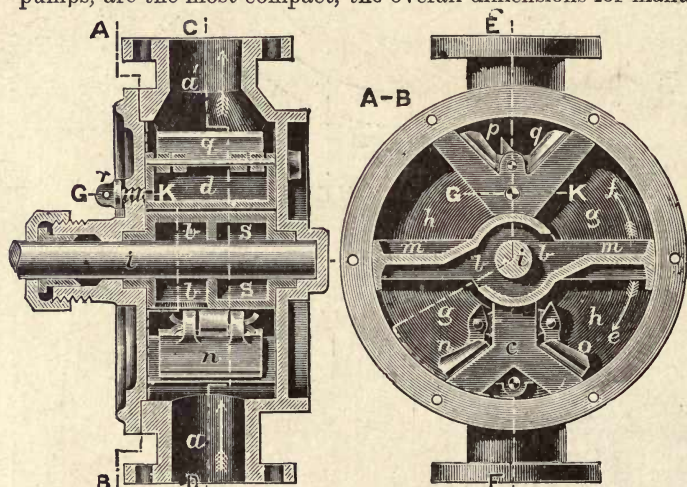
Fig. 256.—Wilcox Quadruple Action Wing Pump (Abrahamson's Patent).
