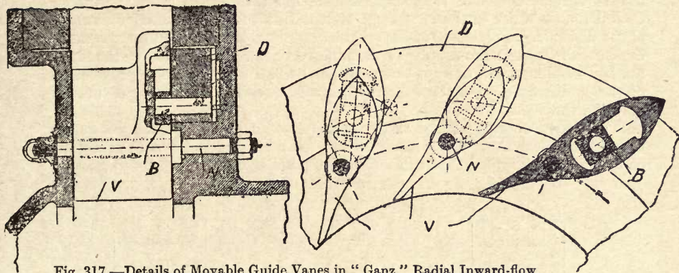
Fig. 317.—Details of Movable Guide Vanes in "Ganz" Radial Inward-flow Turbine.
