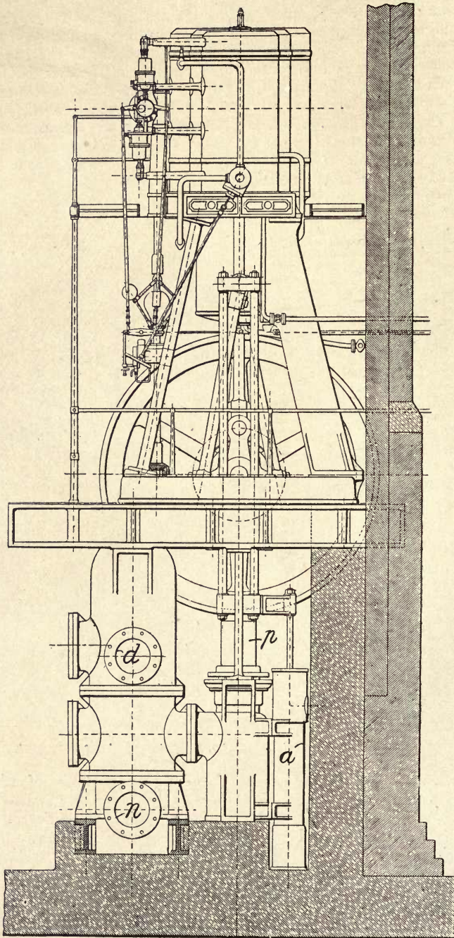
Fig. 15.—Cross Sectional Elevation of Three-crank Pumping Engine for Leeds Waterworks.
