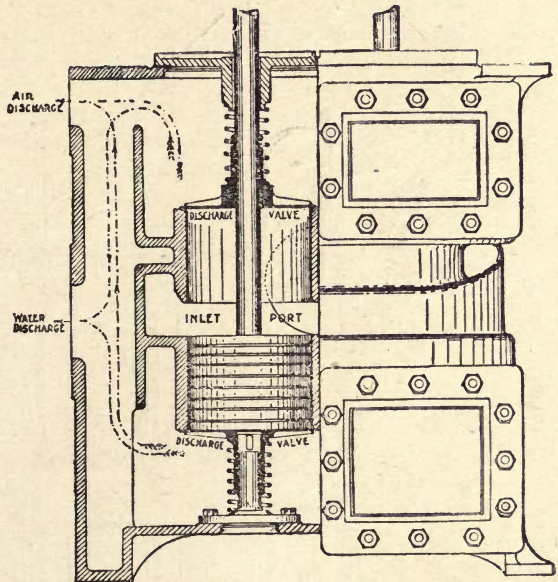
Fig. 168.—Fraser Combined Dry and Wet Air Pump.
