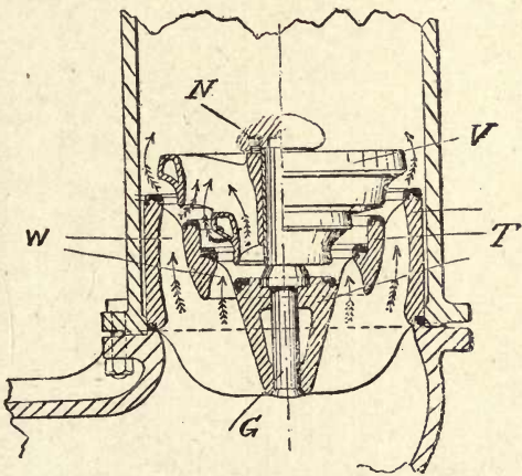
Fig. 43.—Quadruple-seated Suction Ring Valve.
