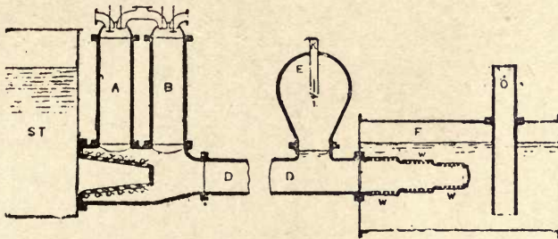
Fig. 194b.—Sectional Diagram of Double-barrel Humphrey Gas Pump adapted for high lifts.
