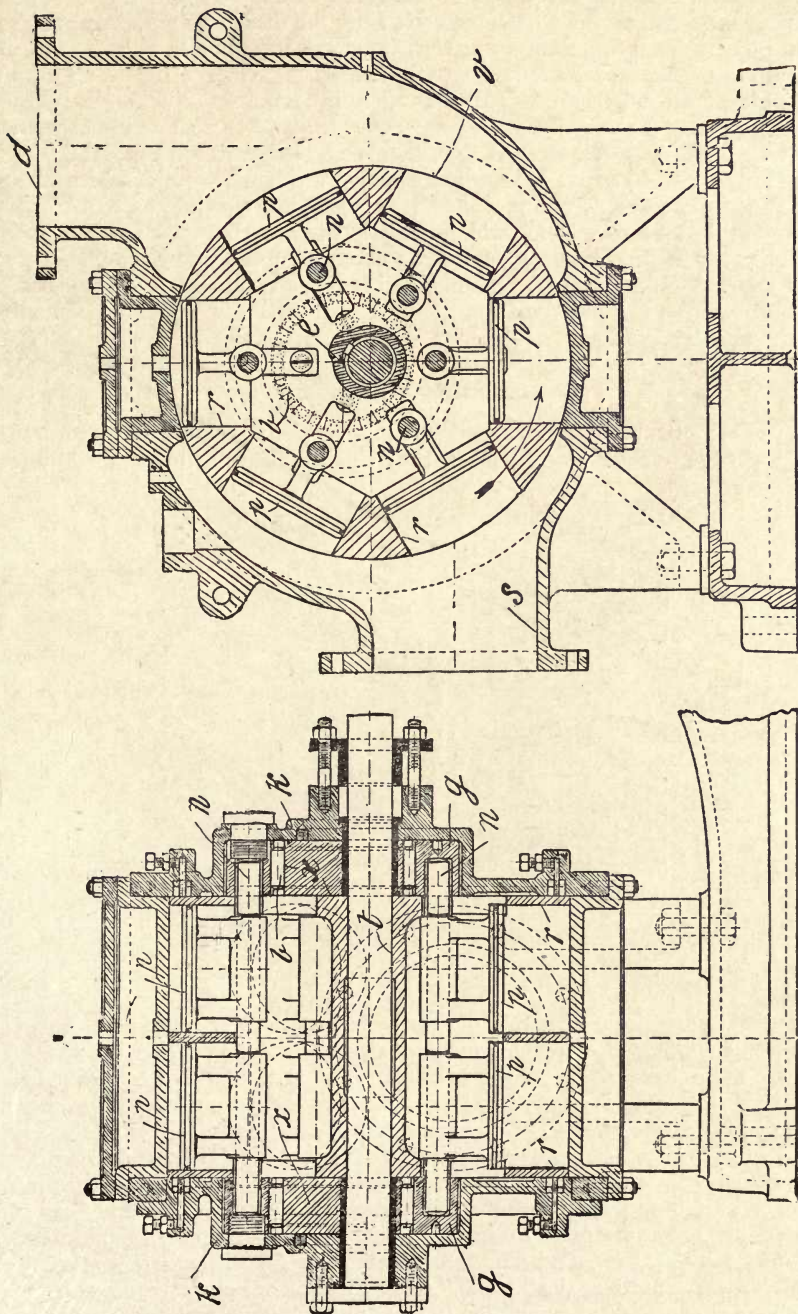
Fig. 255.—Sectional Elevations of the Vincent Rotoplunge Pump.
