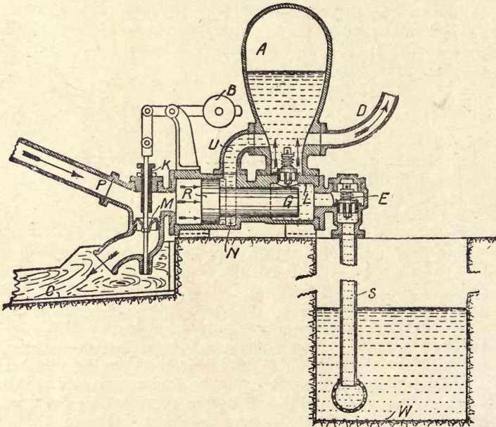
Fig. 184.—Hydraulic Ram in Combination with Plunger Force Pump.
