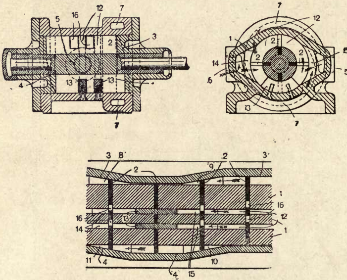
Fig. 248.—Pittler's Reversible Rotary Motor or Pump.
