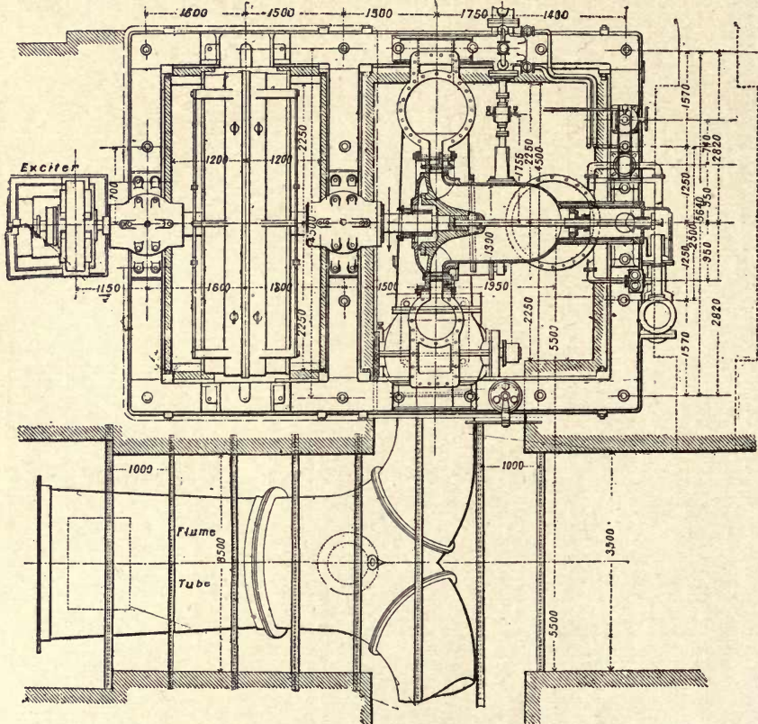
Fig. 316.—Plan of Turbines shown in Fig. 315.
