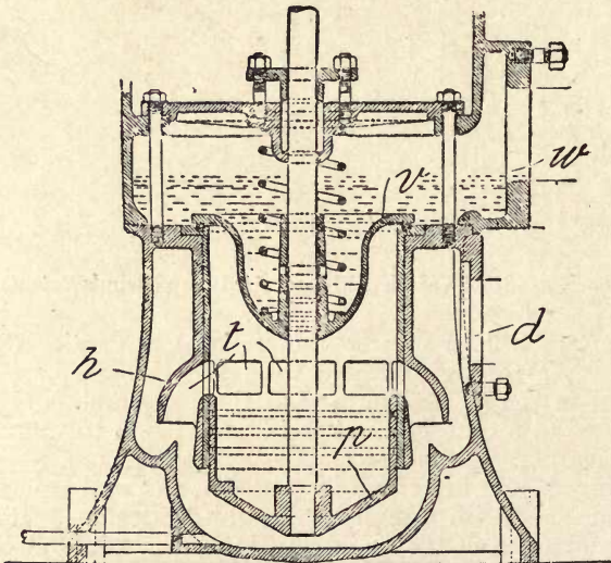
Fig. 162.—Heisler Vacuum Pump.
