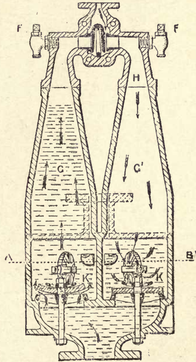
Fig. 186.—Brooke Expulsor Steam Pump.
