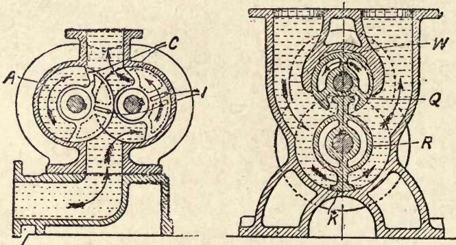
Fig. 244.—Cross-sections of Goldsmidt-Hahlo and Greindl Rotary Pumps.
