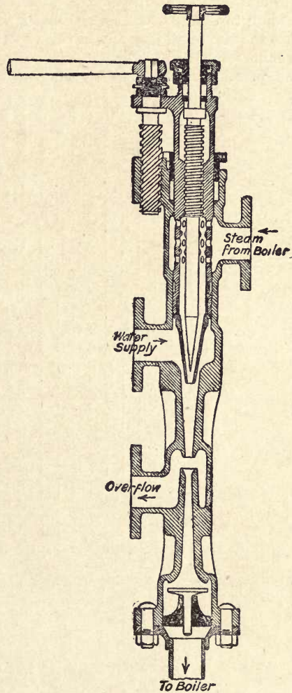
Fig. 124.—Early Form of Giffard Boiler-feed Injector with Plug-controlled Sliding Steam Nozzle.
