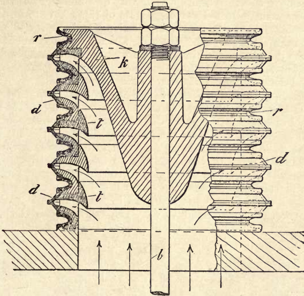
Fig. 47.—Witting Multiple Gill Suction or Delivery Valve.
