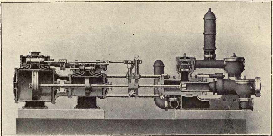
Fig. 117.—Sectional Elevation of "Wilson-Snyder" Compound Duplex 25" x 42" x 9½" x 30" Oil Pump to deliver one million gallons per 24 hours against an average pressure of 1000 lbs.
