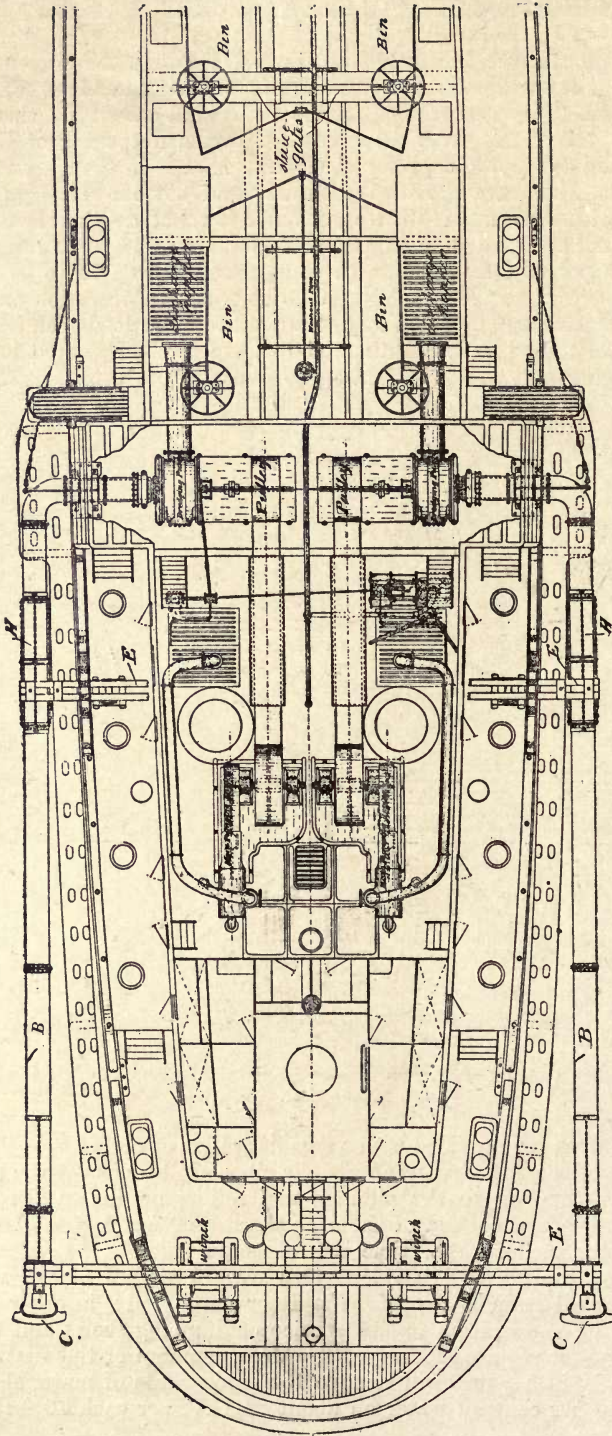
Fig. 272.—Plan Arrangement of Dredging Steamer with Two 15-inch Pumping Sets. Capacity, 12 cubic yards per minute.
