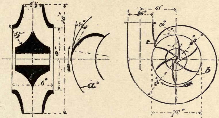
Fig. 266.—Impellers used in Ruston-Proctor Irrigation Pumps.
