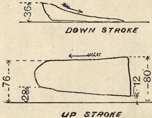
Fig. 71.—Diagrams from Direct-acting Artesian Well Pump.
