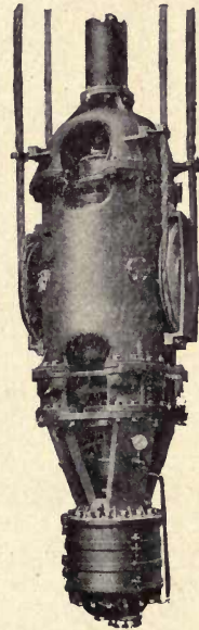
Fig. 40.—Electrically-driven Turbine Sinking Pump.
