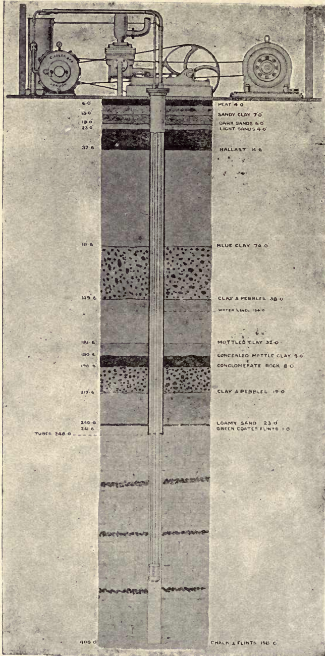
Fig. 75.—Artesian Well at Caxton House, Westminster, showing Electrically-driven Air-lift Pump.
