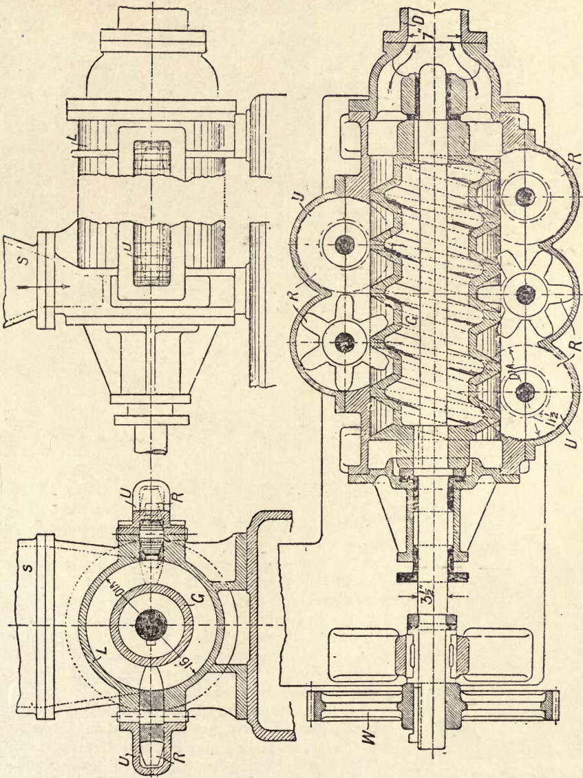
Fig. 238.—Cross section, Elevation, and Sectional Plan Views of Maxwell Archimedean Force-pump for Viscous Fluids and Semi-solids, such as Masse-cuite. (Capacity, 20 tons per hour.)
