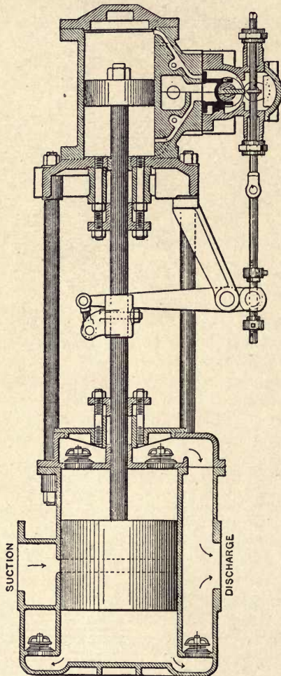
Fig. 159.—Double-acting Valveless Piston Independent Air Pump (Worthington Feather-weight Type).
