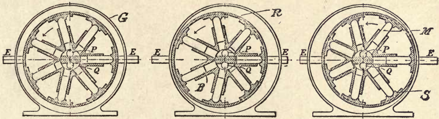
Fig. 232.—Diagrams showing the Action of Hele-Shaw's Combined Variable-delivery and Reversible Action Valveless Rotary Pump.
