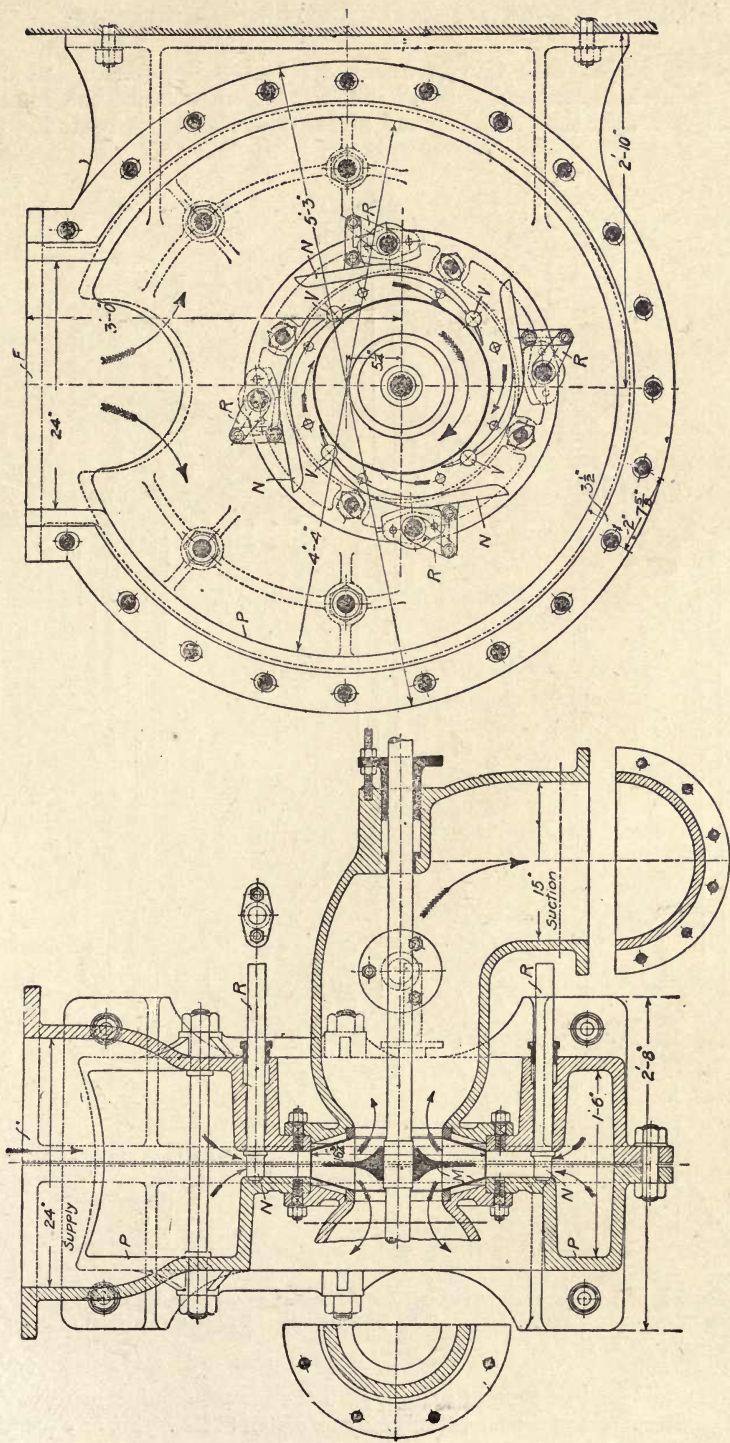
Fig. 301.—Sectional Plan and Elevation of Gilbert Gilkes' Standard Type of Vortex Turbine. Capable of developing 102 H.P. at a speed of 480 revolutions per minute, under a fall of 100 feet, and velocity of 12 cubic feet per second.
