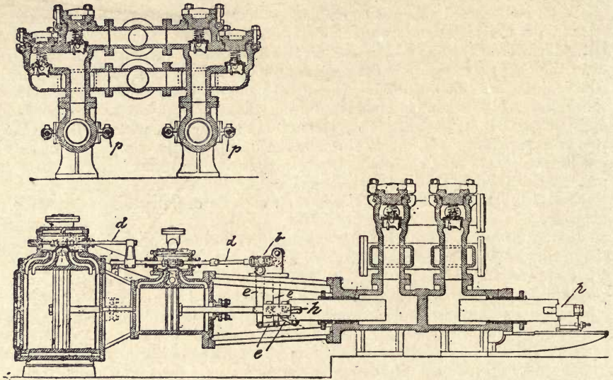
Fig. 114.—Sectional Elevations of "Prescott" Direct-acting Compound-pressure Pump.
