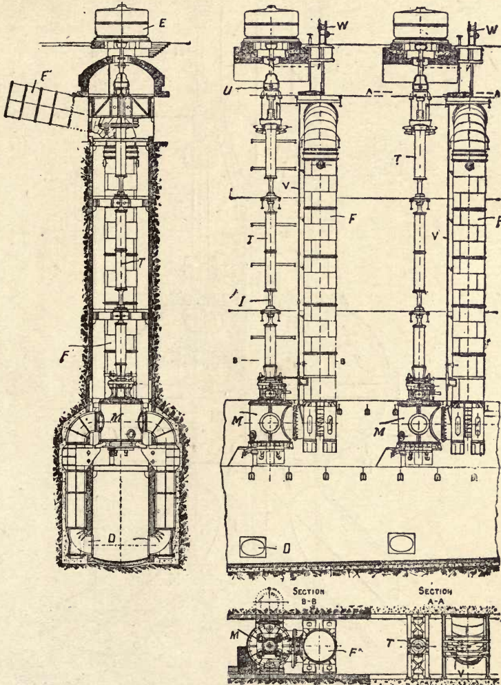
Fig. 323.—General Arrangement of Pair of 10,000 H.P. Inward-flow Vertical Turbines for the Canadian Niagara Power Company.
