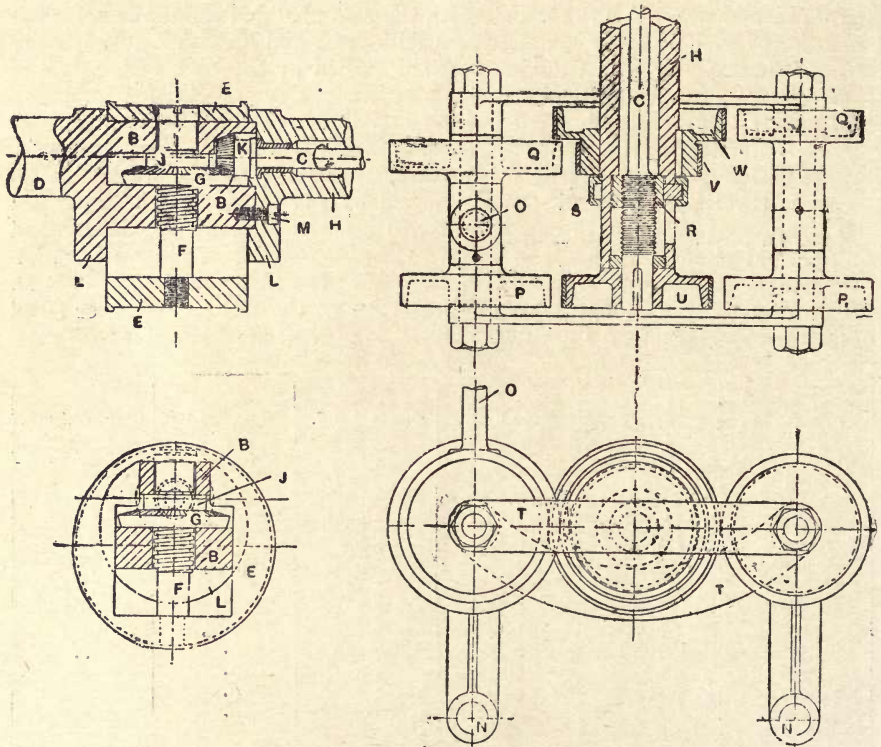
Fig. 226.—Variable Stroke Mechanism for Merryweather Fire Pump.
