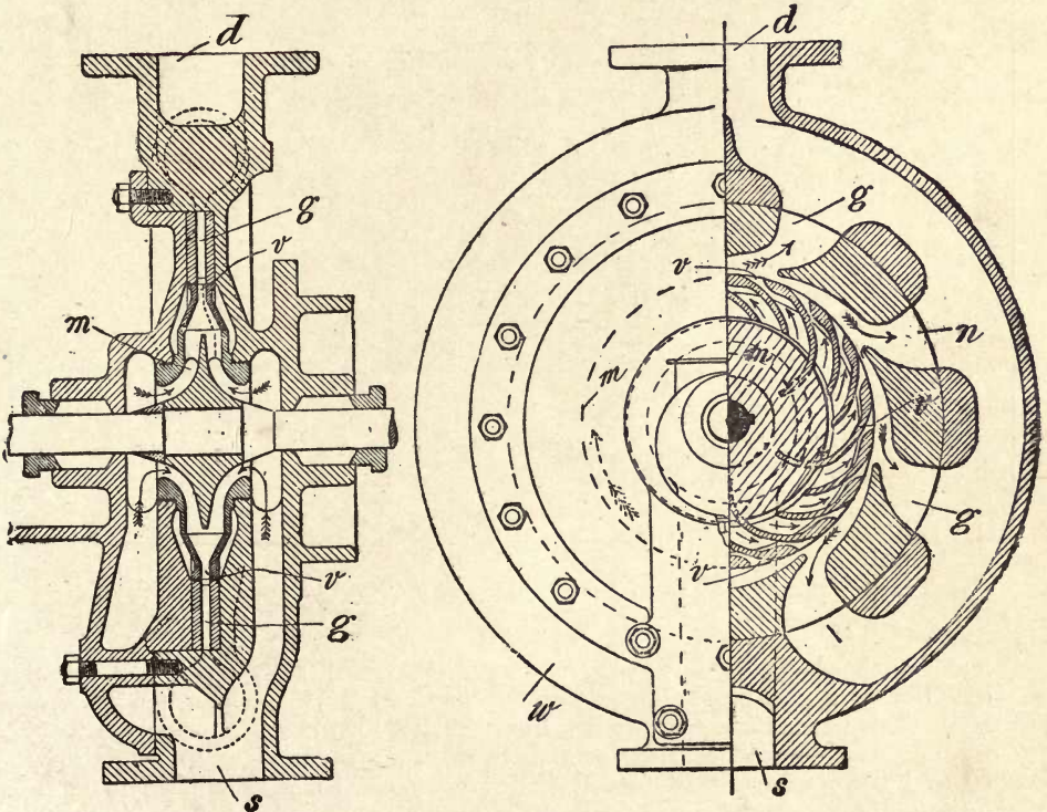
Fig. 279.—Sectional Elevations of the Rees-Roturbo Self-regulating Centrifugal Pump.
