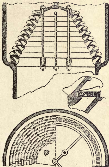
Fig. 51.—Pyramidal Arrangement of Rubber Ring or Gill Valves in Multiple Series.
