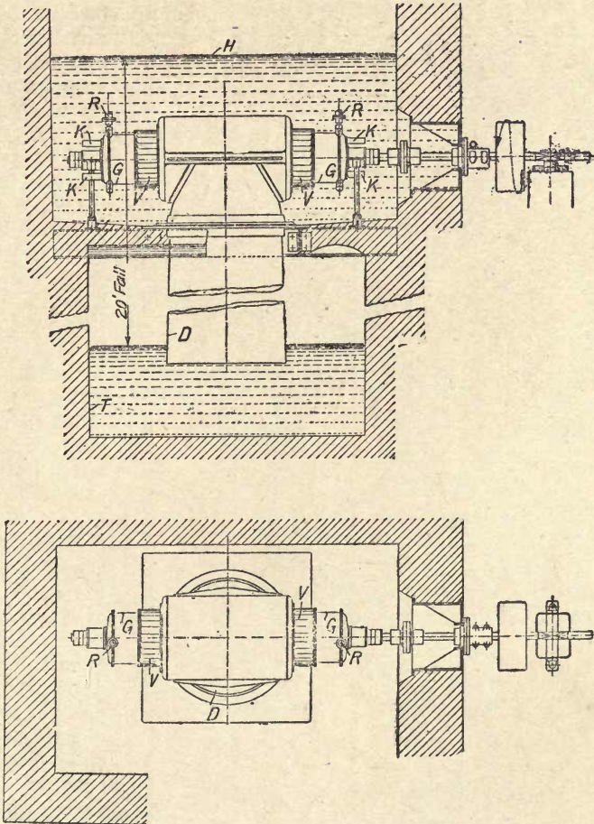
Fig. 309.—Elevation and Plan of 24-inch Twin Diagonal Flow "Victor" Turbine, with cylindrical gate control to develop 120 H.P. at 225 revolutions per minute under a fall of 20 feet. Volume of discharge at 80 per cent. efficiency = 66 cubic feet per second.
