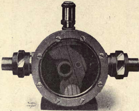
Fig. 251.—Lamplough-Albany Positive Rotary Pump, with Cover removed, showing Revolving Shuttle Action Displacer.
