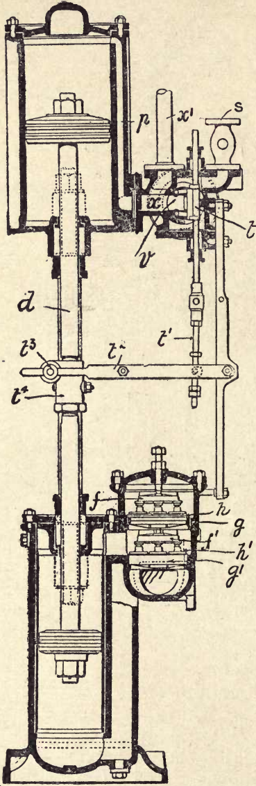
Fig. 107.—Sectional Elevation of "Weir" Feed Pump.
