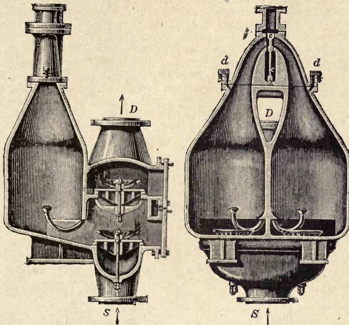
Fig. 42.—Sectional Views of Korting Pulsator Sinking Pump.
