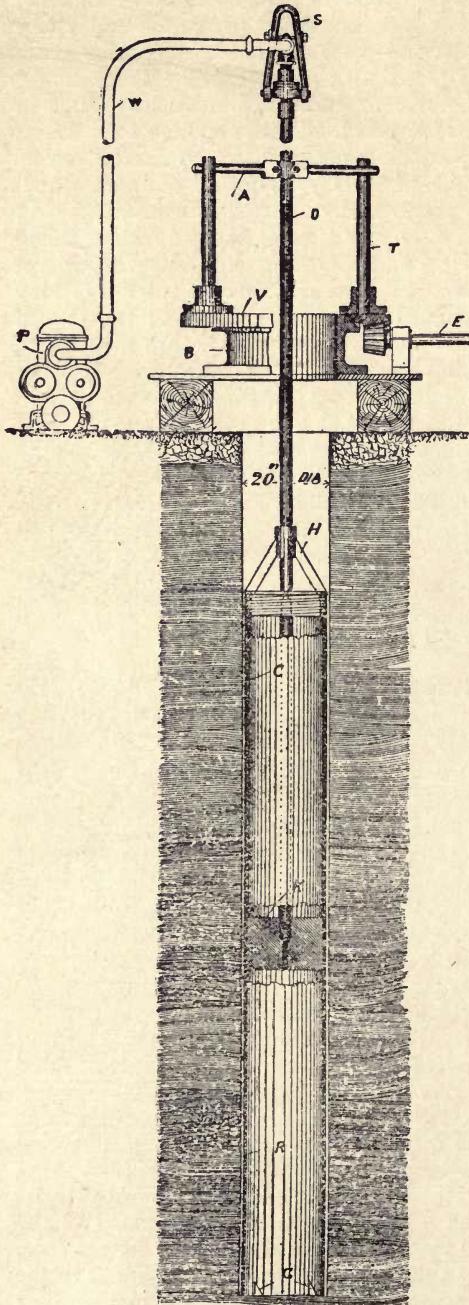
Fig. 61.—Rotary Abrasive-action Boring Machine.
