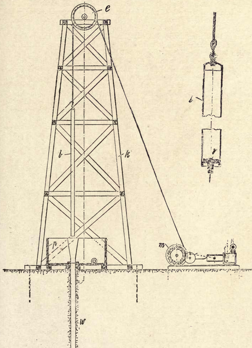
Fig. 79.—Derrick and Winding Gear for Baler Pump.
