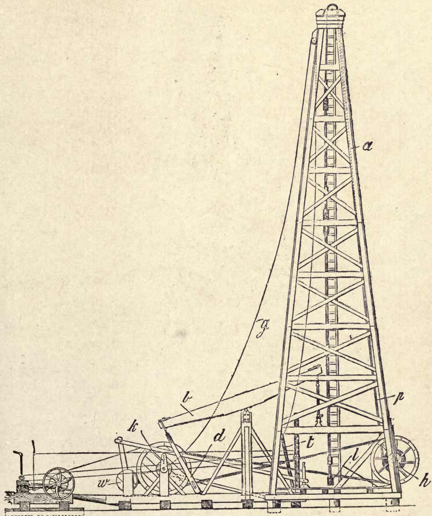
Fig. 58.—Elevation of Percussion Boring Rig, showing Action of Walking Beam.
