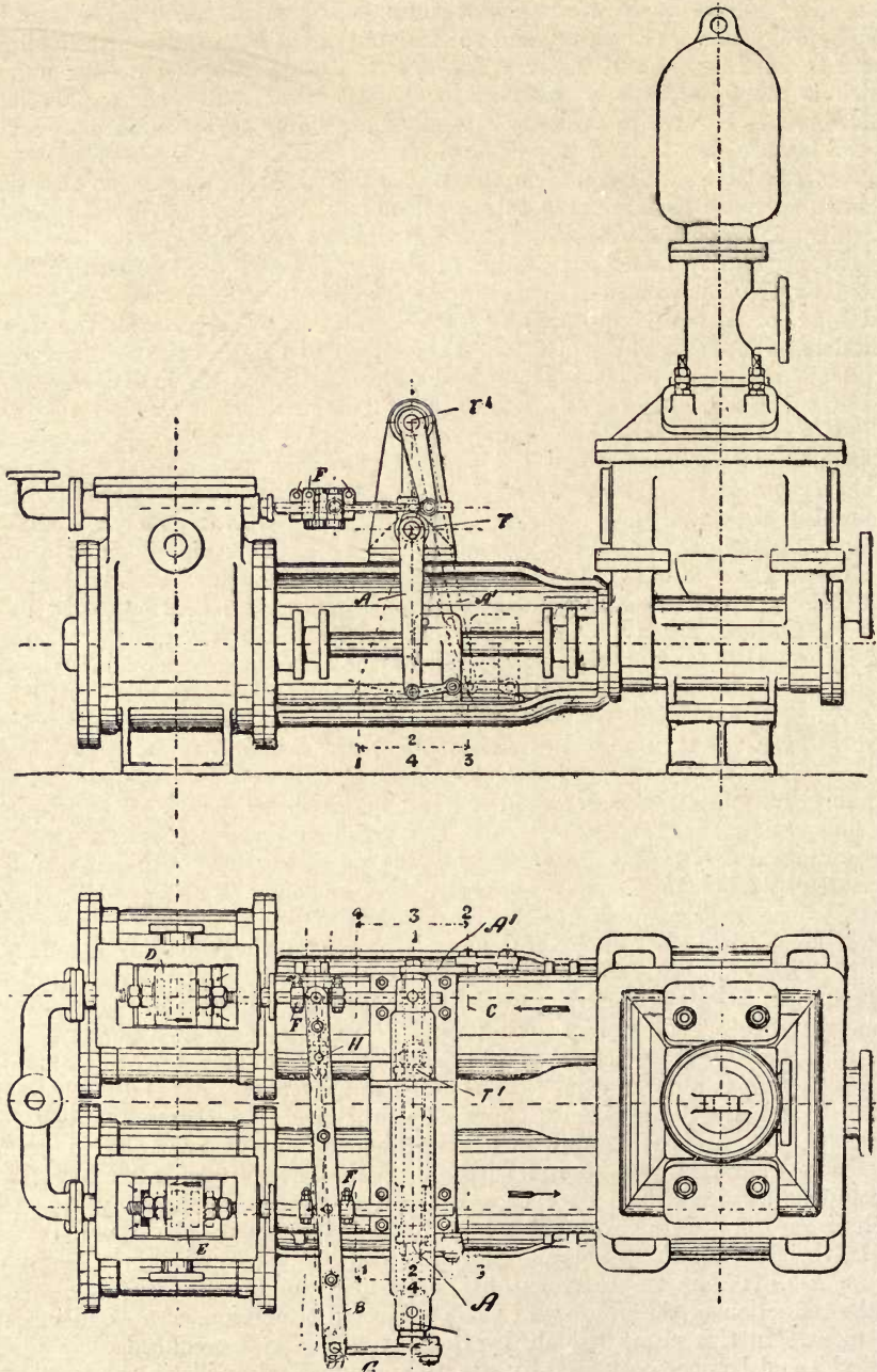
Fig. 111.—Duplex Pump, with Beaver Differential Steam Control.
