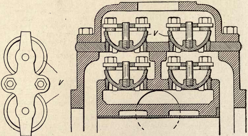
Fig. 90a.—Section showing Spherical Valves used in Burnham Double-acting Pump for Thick Fluids.
