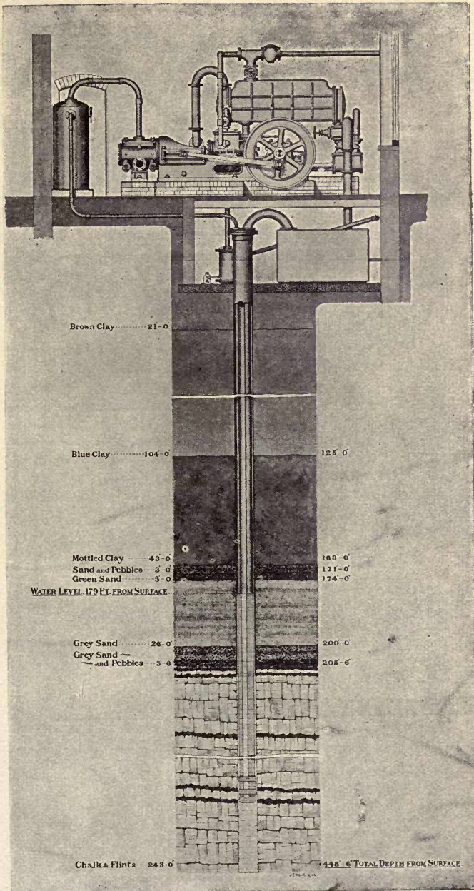
Fig. 74.—Artesian Well at the Prince of Wales Road Public Baths, London, N.W., showing Steam-driven Air-lift Pump.
