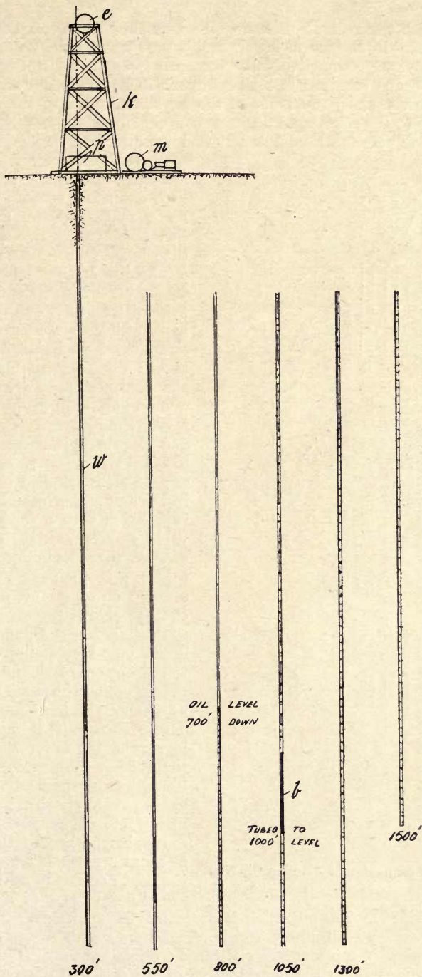
Fig. 80.—Section of Oil Well with Baler Pump.
