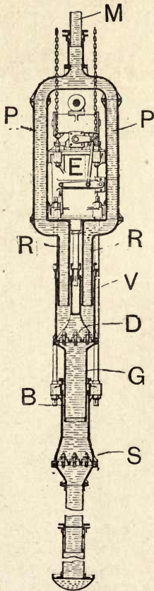
Fig. 37.—Denaby Sinking Pump.
