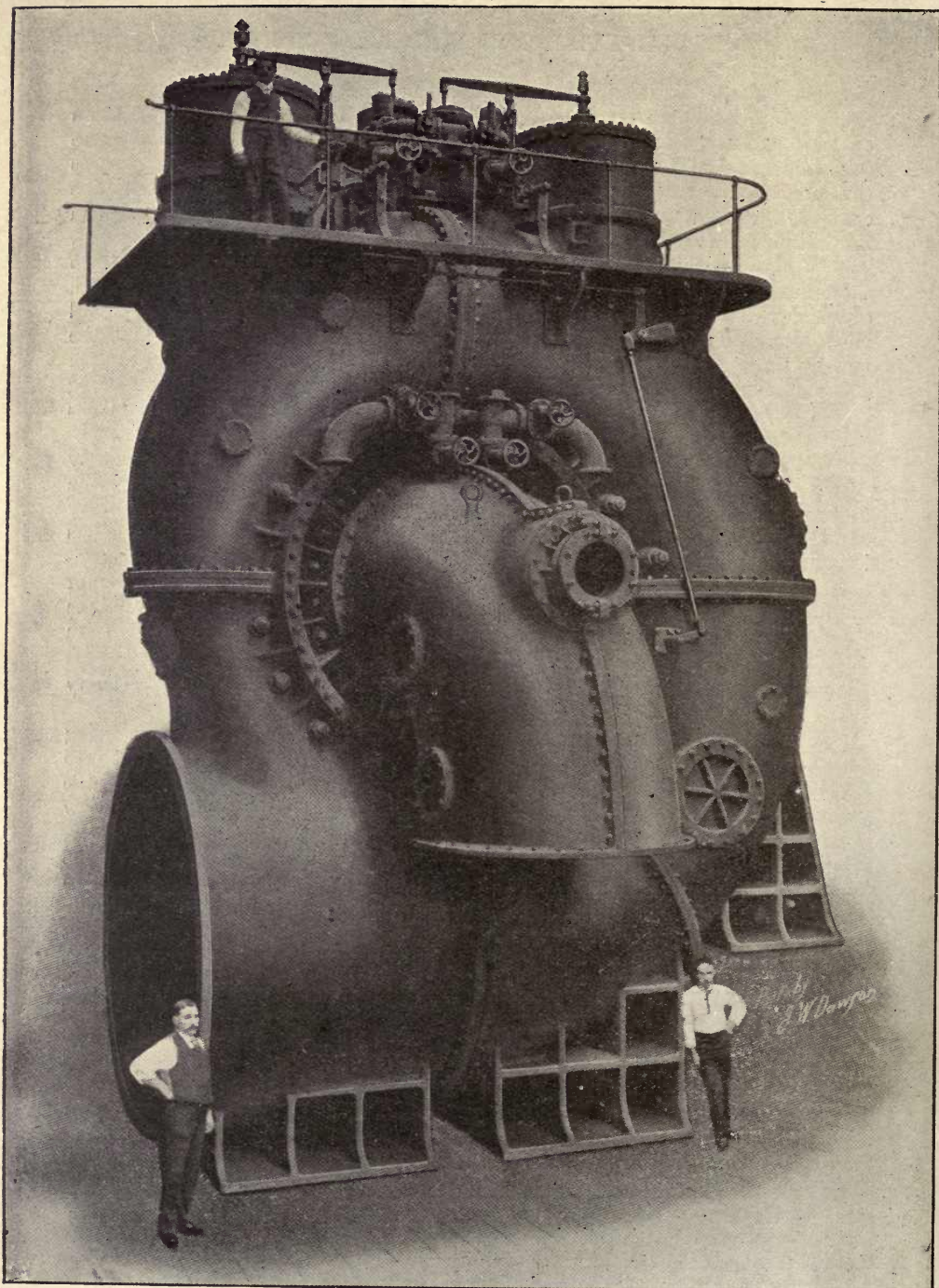
Fig. 320.—Photo-view of Double-wheel Radial-axial-inflow Horizontal Turbine. (Supplied by the I. P. Morris Company to develop 10,500 H.P. on a pressure head of 135 feet at Shawinigan Falls.)
