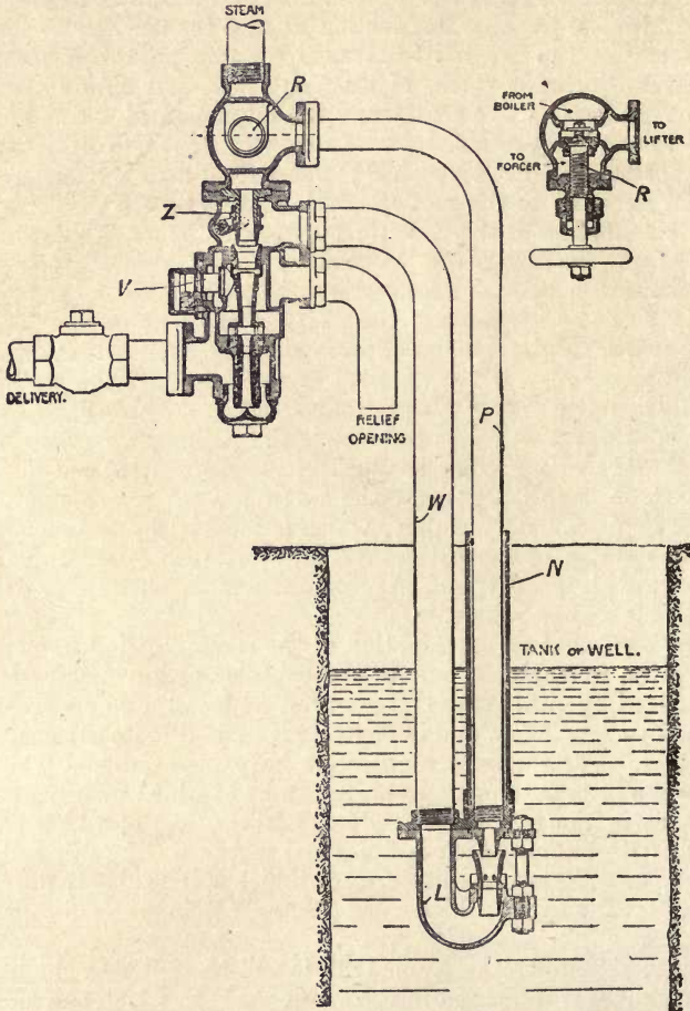
Fig. 132.—Albion Combined Lifter and Forcer Injector.
