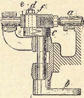
Fig. 209.—Details of Valve Gear of Oddie-Barclay Pump.
