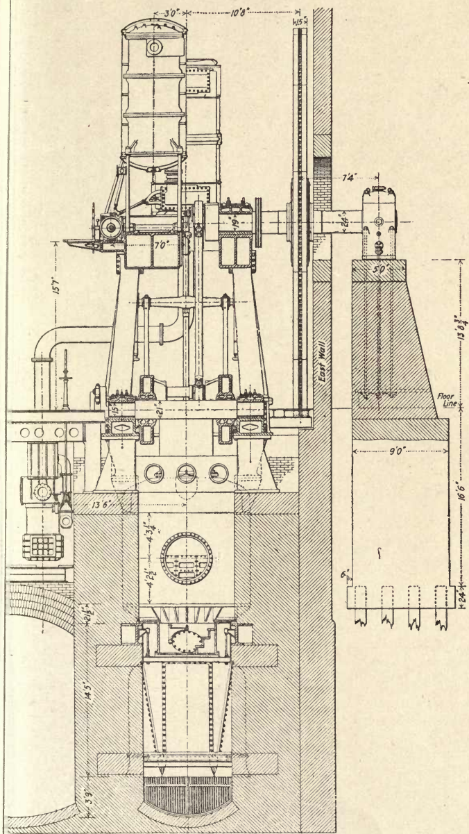
Single-acting Plunger Pumps for the Boston Main Drainage Works.
