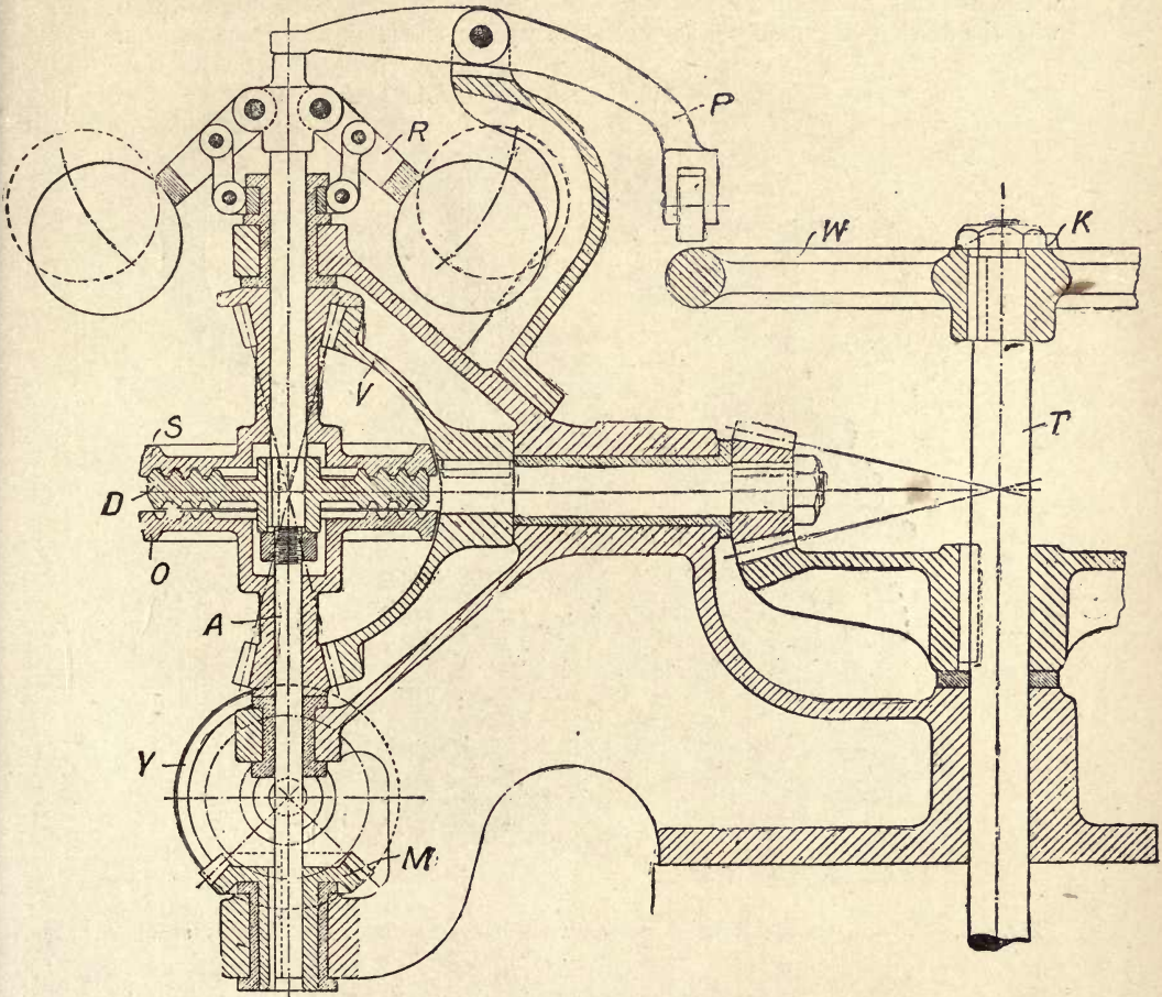
Fig. 342.—Turbine Relay Governor with Frictional Drive.
