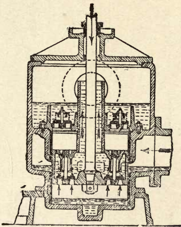
Fig. 167.—Paxman Combined Dry and Wet Air Pump.
