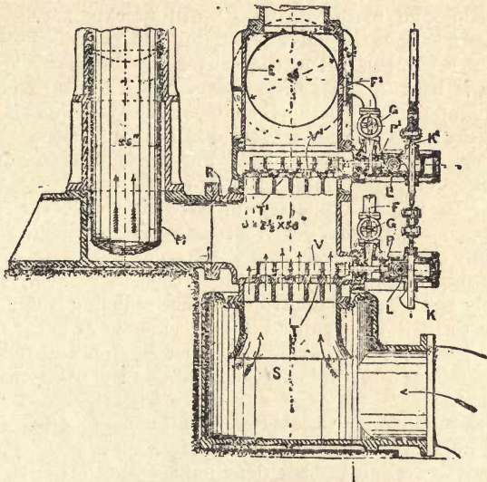
Fig. 205.—Sectional View of Waterworks Pumping Engine, showing Southwark Suction and Discharge Valves.
