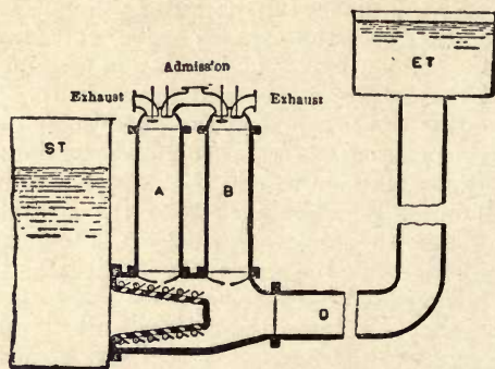
Fig. 194a.—Sectional Diagram of Two-cycle Humphrey Gas Pump.
