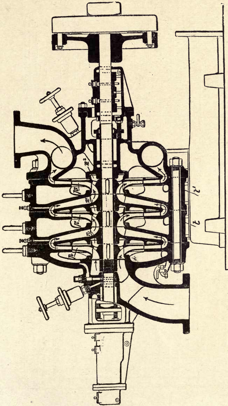
Fig. 289.—Sectional Elevation of Worthington Three-stage Turbine Pump.
