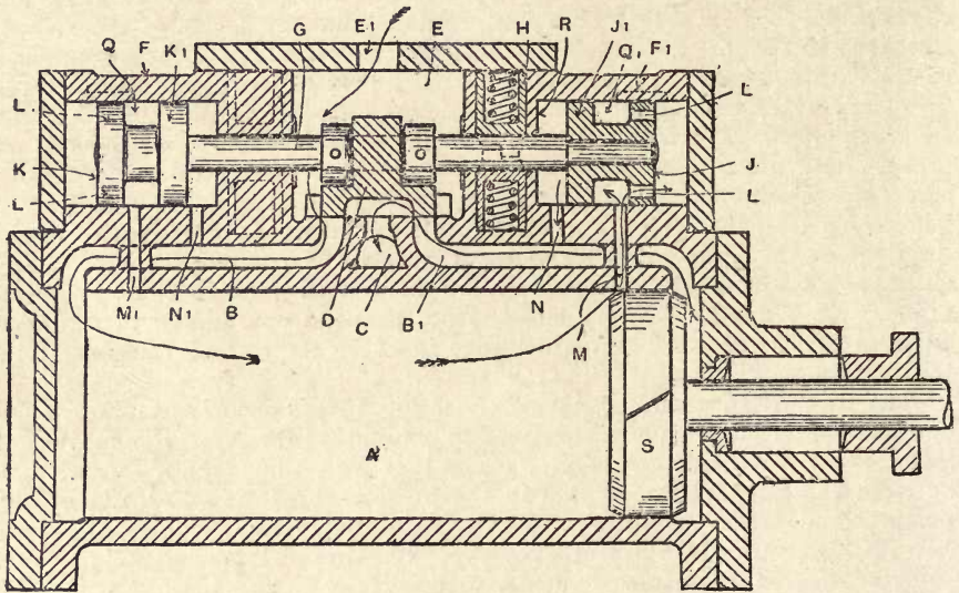
Fig. 102.—Richardson's Simplex Valve Gear.
