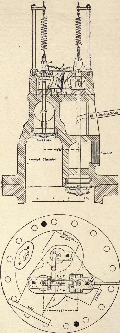
Fig. 194.—Details of Valves and Controlling Mechanism for Humphrey Gas Pump.
