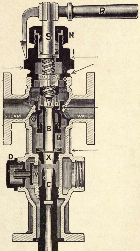
Fig. 127.—White One-movement Injector (Vertical Locomotive Type).
