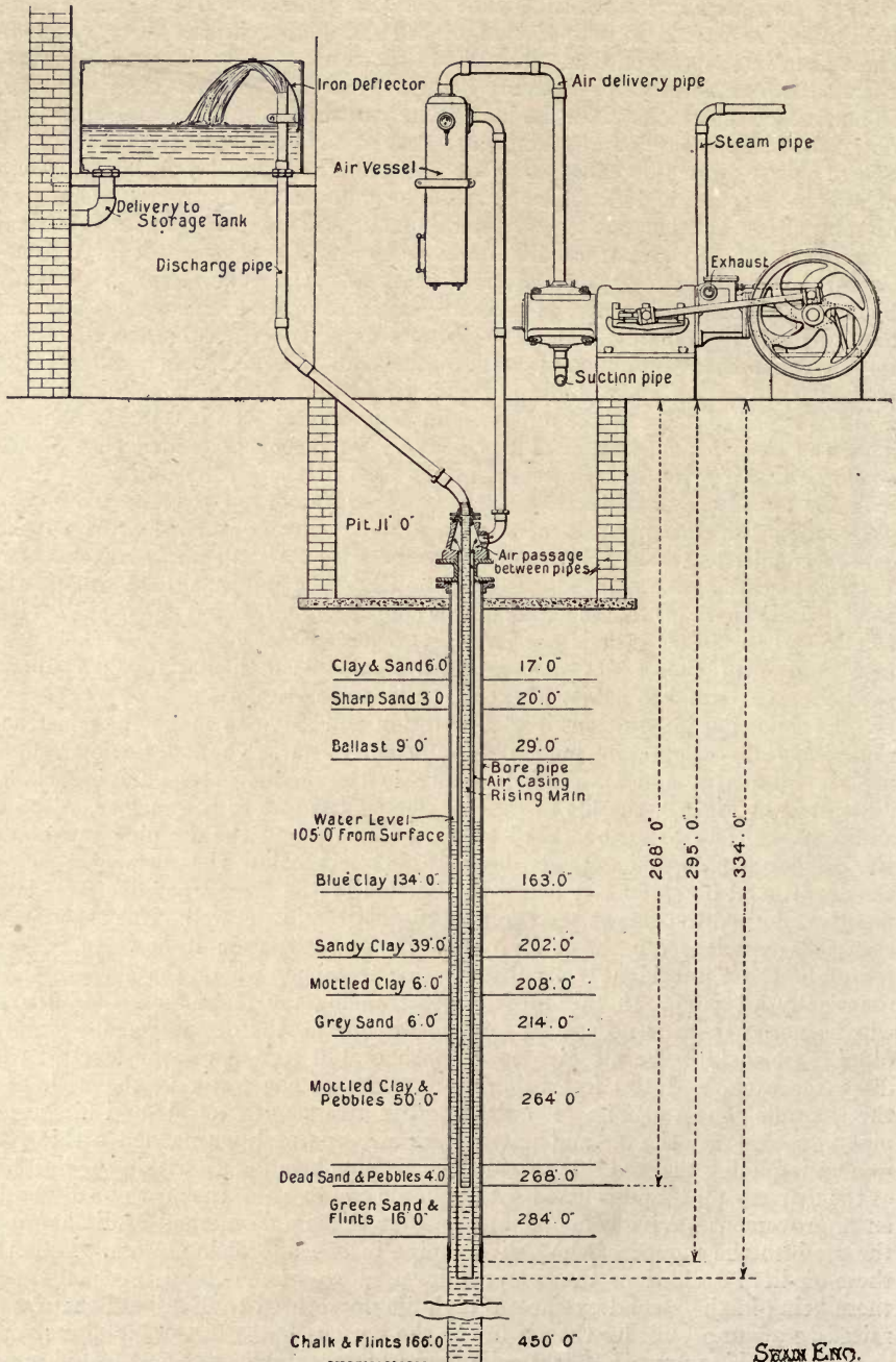
Fig. 73.—Artesian Well Air-lift Pump.
