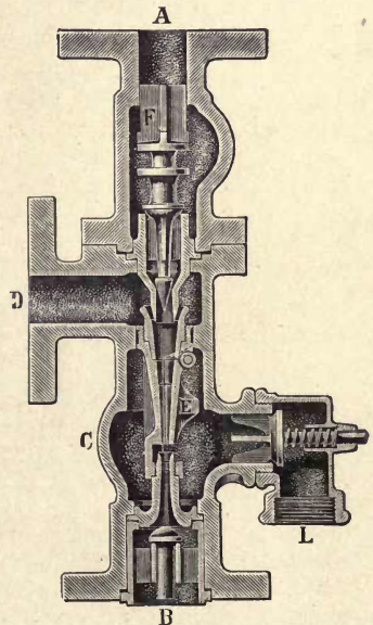
Fig. 130.—Schaffer & Budenberg Injector, with Split Combining Cone.
