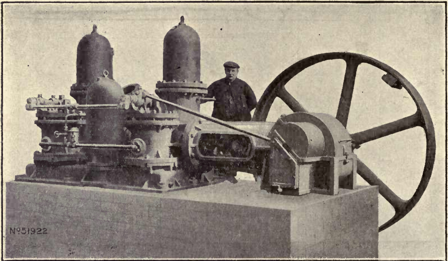
Fig. 211.—Double-acting Belt-driven Oddie-Barclay Pump. (Rams, 8 × 15 Inches Stroke.)
