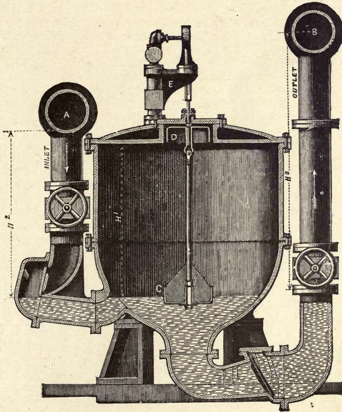
Fig. 187.—Shone's Pneumatic Ejector.
