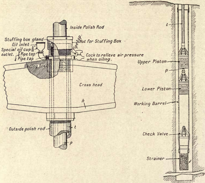
Fig. 69.—Details of Crosshead and Plunger Connections of Downie Double-acting Borehole Pump.
