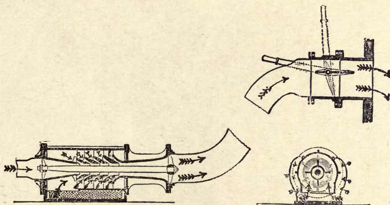
Fig. 144.—Friedmann Bilge Water Ejector.
