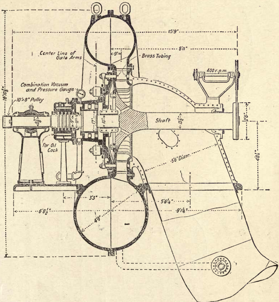
Fig. 311.—Sectional Elevation of Single-wheel Radial-axial-inflow Horizontal Turbine. (Supplied by the Platt Iron Works Company to develop 10,000 H.P. on a pressure head of 260 feet at Snoqualmie Falls.
