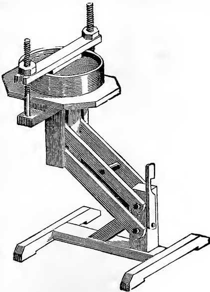
Fig. 82. Cheese-press.
