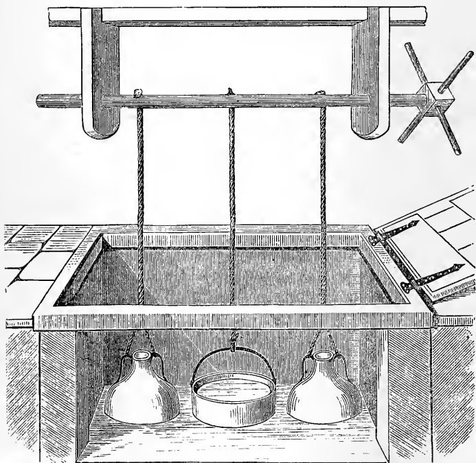
Fig. 97. Cool-bath
