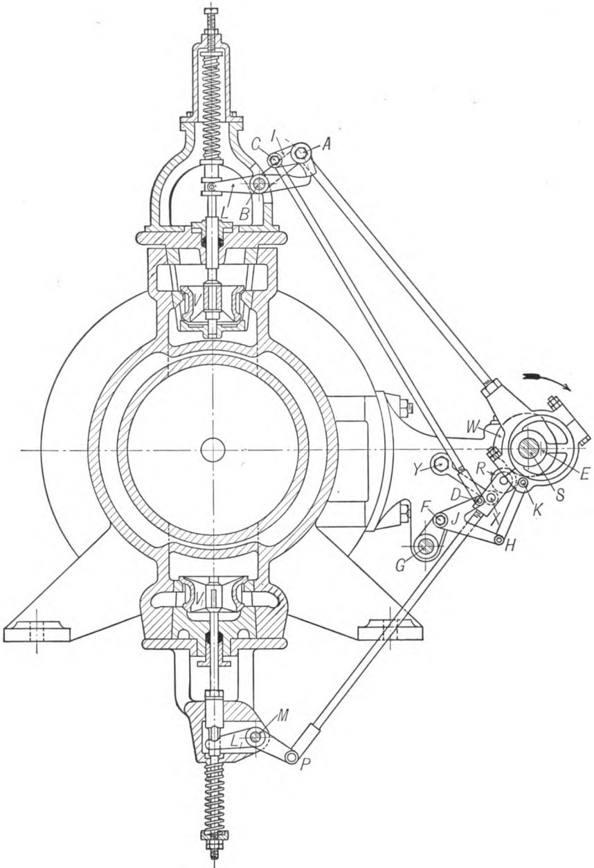
FIG. 129. Sulzer Valve Mechanism.
