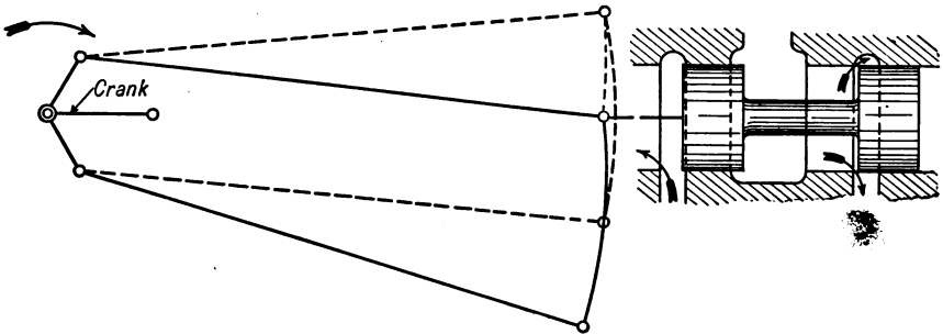
FIG. 140. Increasing Lead.
