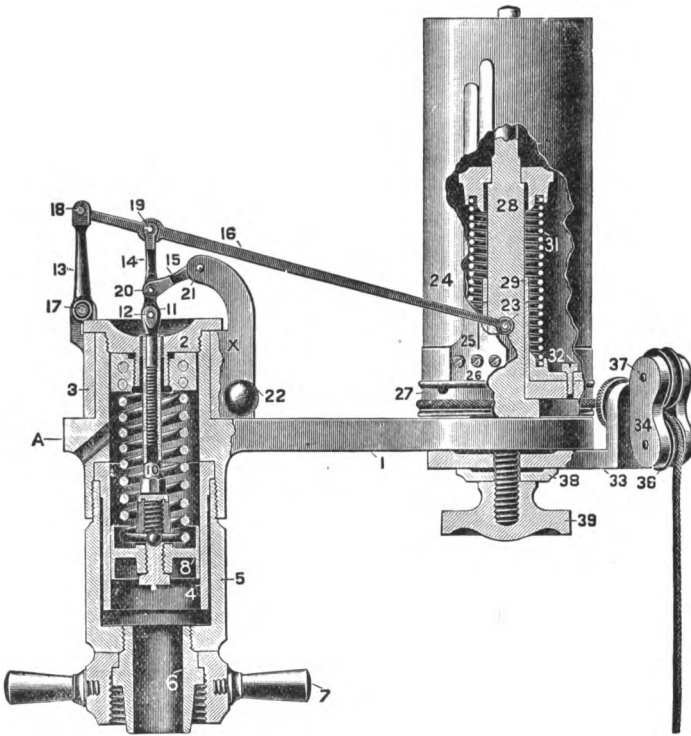
FIG. 14. Section of Crosby Indicator.
