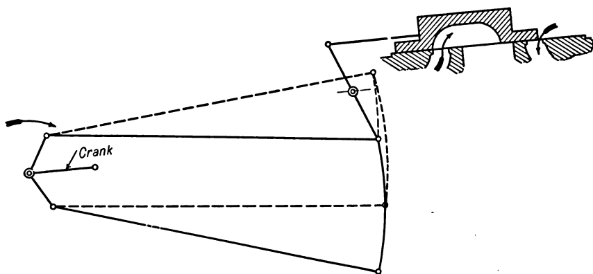
FIG. 142. Increasing Lead.
