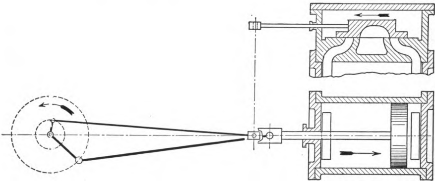
FIG. 32. Head-end Compression.
