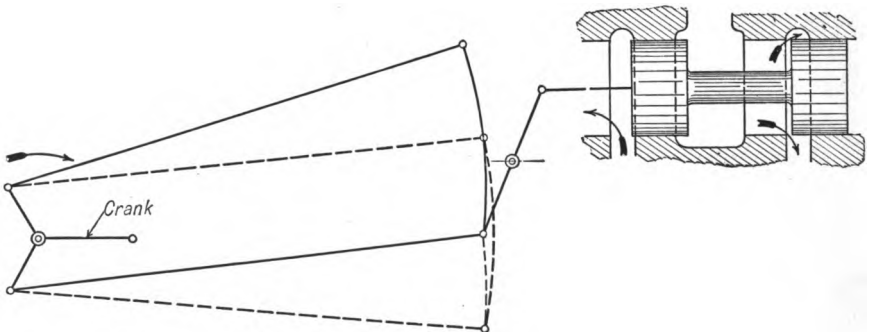
FIG. 145. Decreasing Lead.
