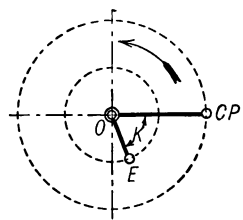
FIG. 46. D Valve with Reversing Rocker.
