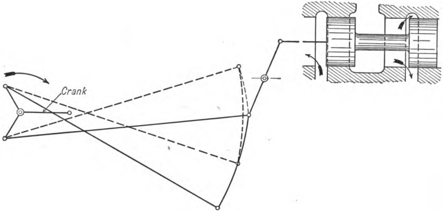
FIG. 144. Increasing Lead.
