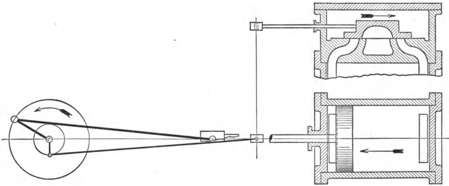
FIG. 30. Mid-position.
