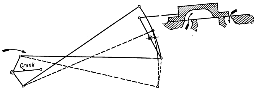
FIG. 143. Decreasing Lead.
