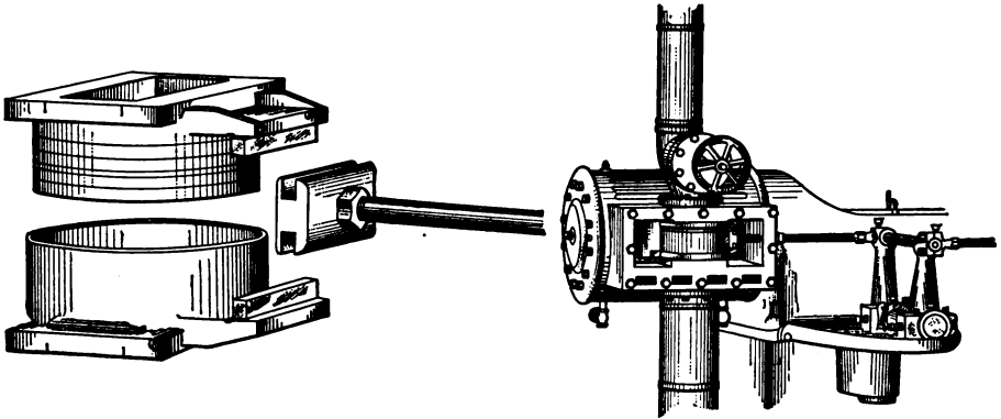
FIG. 38. American-Ball Engine Valve.
