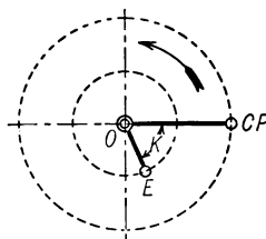
FIG. 45a. Piston Valve Direct.
