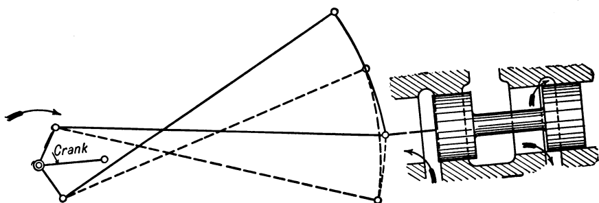
FIG. 141. Decreasing Lead.
