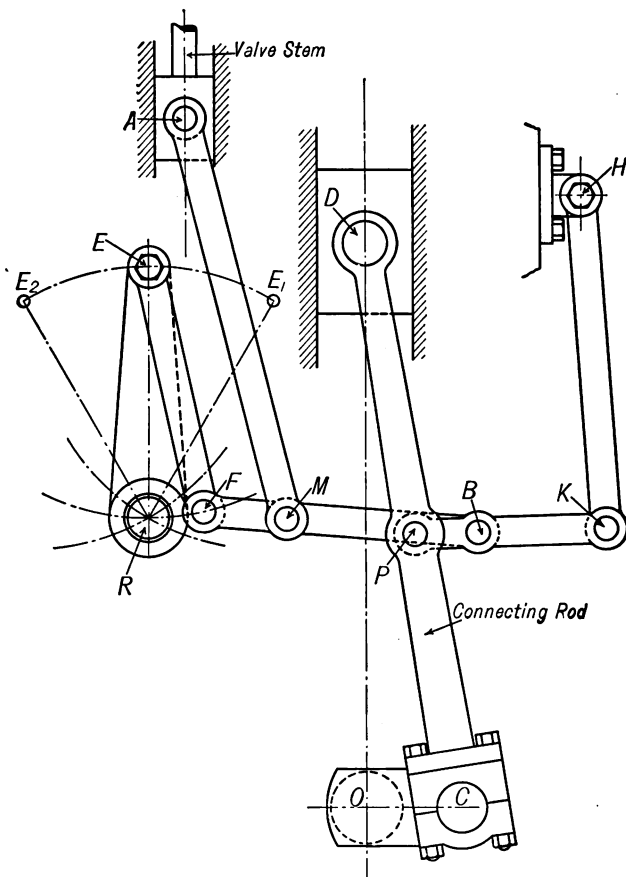
FIG. 156. Joy Valve Gear.
