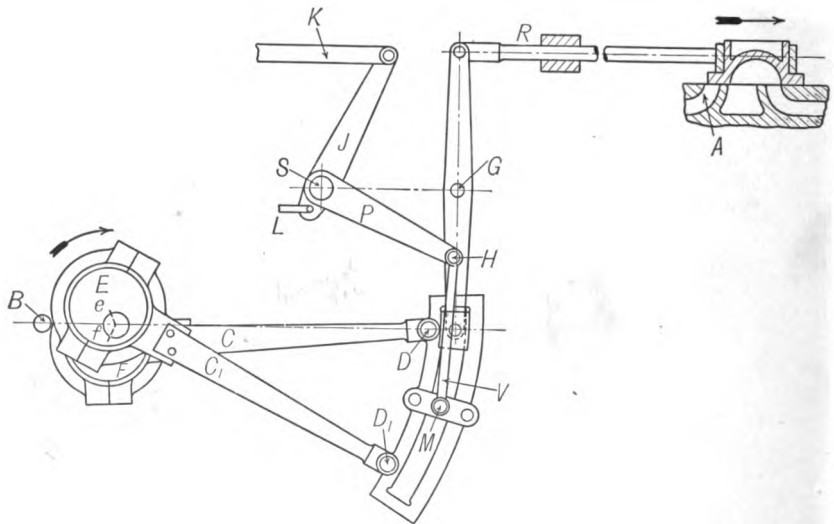
FIG. 137. Stephenson Link with Rocker, Full Gear Forward.
