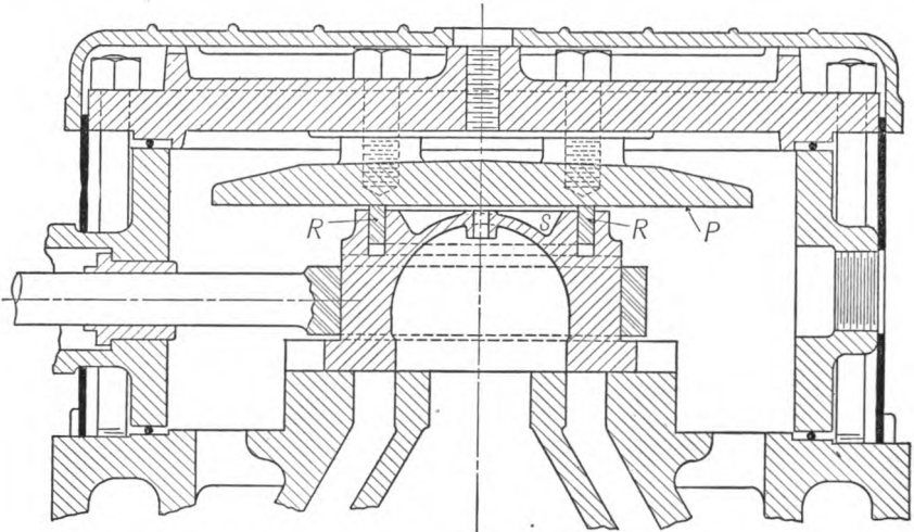
FIG. 36. Locomotive Balanced Valve.
