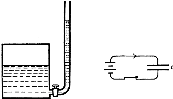
FIG. 8.— Model illustrating the flow of a displacement current in a dielectric C . The pressure in the vessel represents the voltage of the battery; the height of the column, the displacement in the dielectric; the flow of water, the charging current. The energy expended may be recovered.
