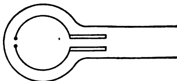
FIG. 35.—Blondlot's method. The wire which connects the plates of the oscillator is bent into a circle, and acts inductively upon another loop concentric with it, to which the wires are attached.
