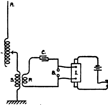
FIG. 130.—Marconi coherer system—transmitter. I is the induction coil, with battery and key, B the spark-gap. C an adjustable condenser, P, S the oscillation transformer, and L a variable inductance in series with the antenna A.
