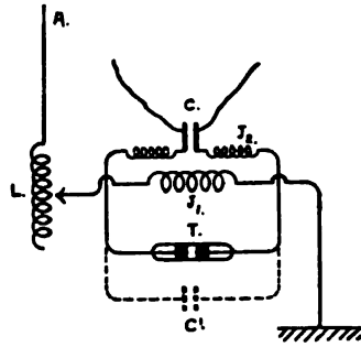
FIG. 131.—Marconi coherer system—receiver. A is the antenna, with variable inductance L, J, J, the jigger, T the coherer and C a condenser, to which the relay and recording apparatus are connected. C' is an additional condenser sometimes used to improve the resonance.
