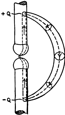
FIG. 86.—A portion of the oscillator, FIG. 85, enlarged, showing a single Faraday tube. The tube terminates in opposite charges, +Q and -Q, on the surface, equal to the integral value of the current which supplied these charges, and also to the induction, or "electric flux" across any section of the tube.*
