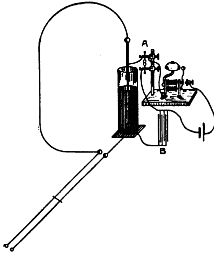
FIG. 94.—Lodge's knob coherer, applied to Syntonie jar experiment (see p. 209). The knobs are shown at A, mounted on the same base as the bell that gives the signal. The vibration of the bell is sufficient to decohere the knobs.
