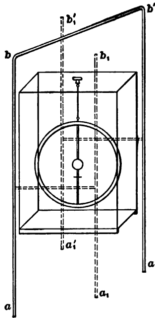
FIG. 99.— Hertz's inductive detector. The hoop of aluminum wire is shown with mirror attached, suspended within the box. The wire abb'a'' carries the oscillations, which repel the currents that they induce in the hoop.
