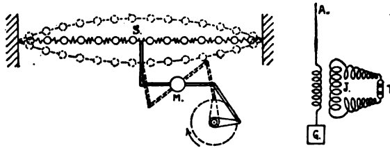
FIG. 137.— Model illustrating the operation of Marconi's "jigger," whose distributed capacity and inductance (elasticity and mass) are so proportioned to the frequency that the current (velocity) imparted through the mutual induction (mass M ) to the secondary (weighted spring) is transformed into potential (tension) at the free terminals of the coil (ends of spring).
