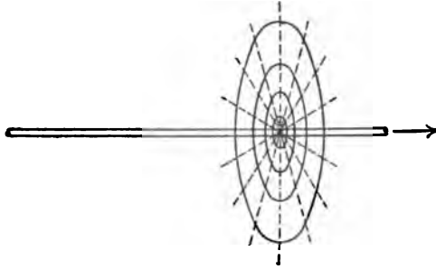
FIG. 46.— A portion of the wave-front surrounding a perfectly conducting wire transmitting oscillations. The magnetic force forms closed circles concentric with the wire, which slide along without expanding; hence the intensity of the wave remains constant. The electric force, and hence the displacement currents, are radial, and so are strongest close to the wire.
