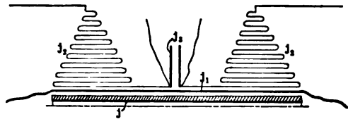
FIG. 109.—Marconi's jigger—improved arrangement. The secondary winding j_2 is divided in the middle and the ends are connected to a condenser, j_1 . For connections, see Fig. 110.
