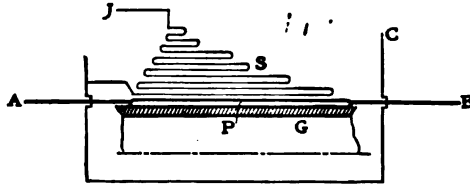
FIG. 108.—Marconi's jigger 1 —half section. G is a glass tube on which are wound the primary P and secondary S. Each of the zigzag lines represents a layer of winding. The terminals A E of the primary are connected to the antenna and to earth, and the terminals C J of the secondary go to the coherer and the recording apparatus.
