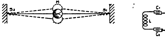
FIG. 136.— Model illustrating the action of an oscillating circuit with concentrated inductance L and capacity C_1, C_2 , which are analogous to the mass M , and the elasticity concentrated in the springs S_1, S_2 .
