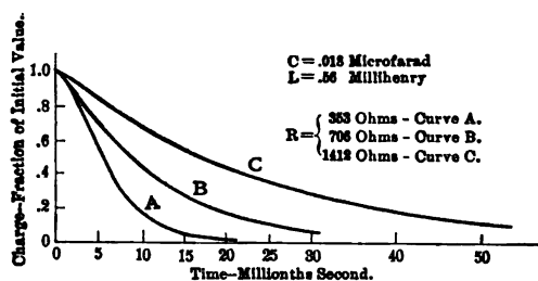
FIG. 19.—Undirectional discharge of a condenser. The conditions are the same as in FIG. 18, except for the increased resistance. Curve A is the critical case of quickest discharge. For smaller values of R the discharge becomes oscillatory. Curves B and C are for larger values of R .
