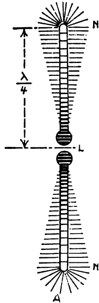
FIG. 81.—Vibration of a free oscillator. Radiating lines show distribution of potential; shading, the intensity of current. NN, nodes, L, loop, A, ground.
