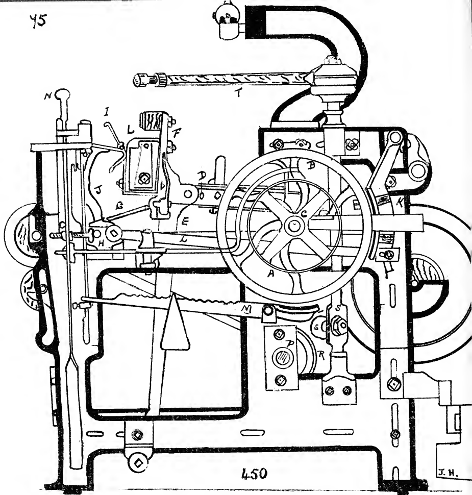
A Driving Pulley, B. Brake wheel, C crank, or Top shaft, D. crank arm E, slay wood, F, Box-end and slay, G, stop-rod tongue for a fast need, H, Frog, I, Weft fork, J, Weft fork hammer and lever K, Baer brake, L connection rod from frog to back brake, M, brake, connected with Weft fork, N, starting handle, P, Bottom shaft, on this shaft are fixed the Shedding tappets, Picking tappets R, S is the Picking bowl, on shaft to which the picking stick T is fixed.
