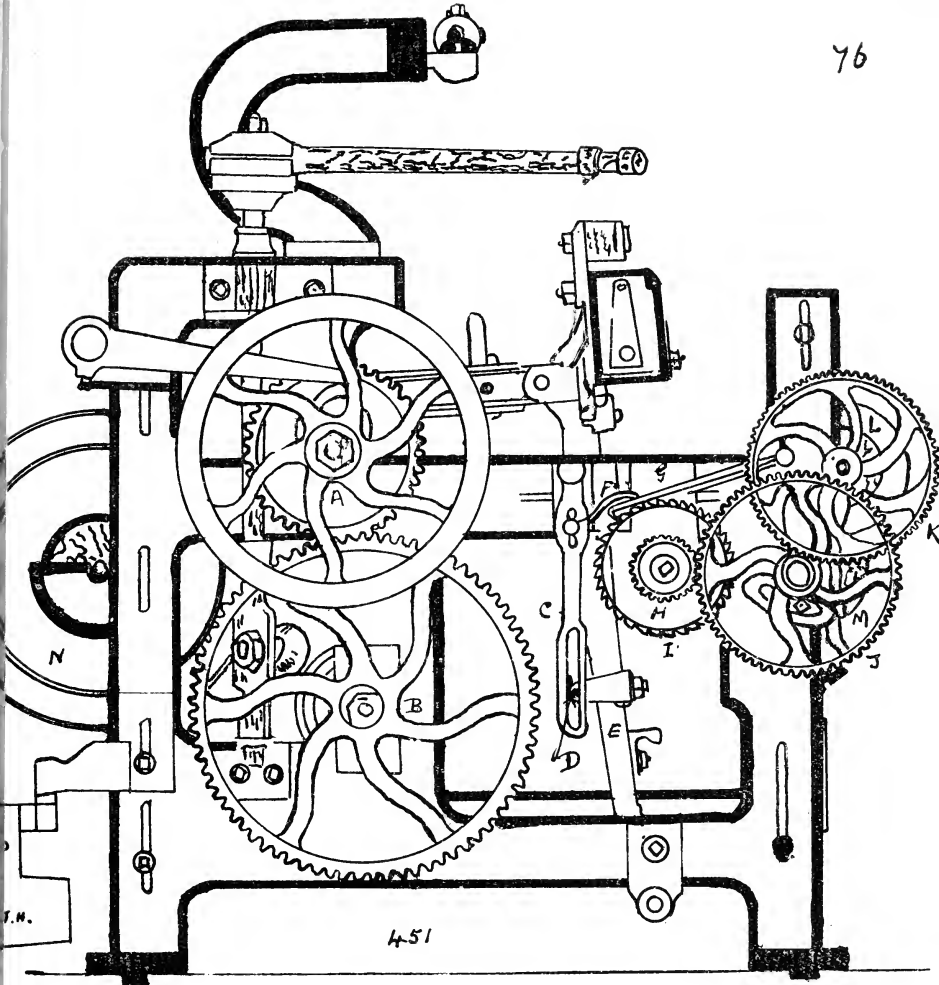
7, crank shaft on Driving wheel. B bottom shaft wheel. C, setting-up lever for taking-up motion, it receives its motions from a bracket and pin D fixed to the slay sword E on lathe arm. F, take-up lever catch. G, retaining catch. H, I, J, K, a train of wheels, the take-up motion, they are connected with the roller L, and L drives the cloth roller M by frictional contact. N Warp beam P Beam weight.
