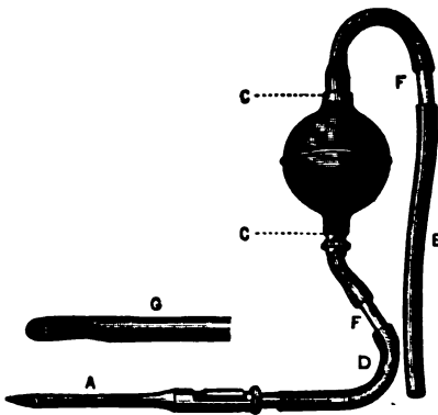
FIG. 581.—Fitch's aspirator.
