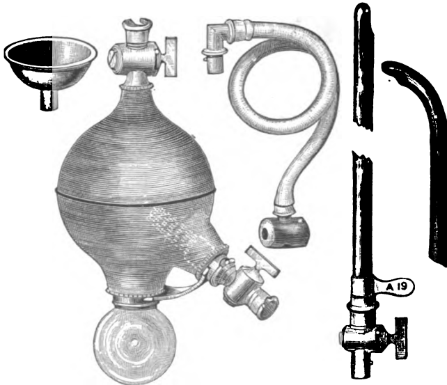
FIG. 670.—Bigelow's washer.
