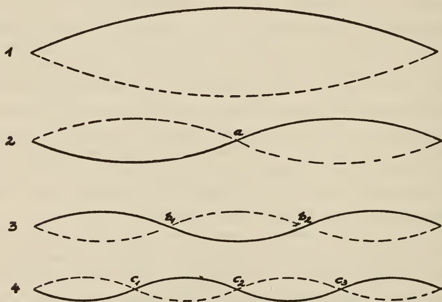
FIG. 9. Diagrams of transverse waves
