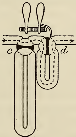
FIG. 7. Rotary valve of a wind instrument. In c the valve is in the resting position, in d it is activated
