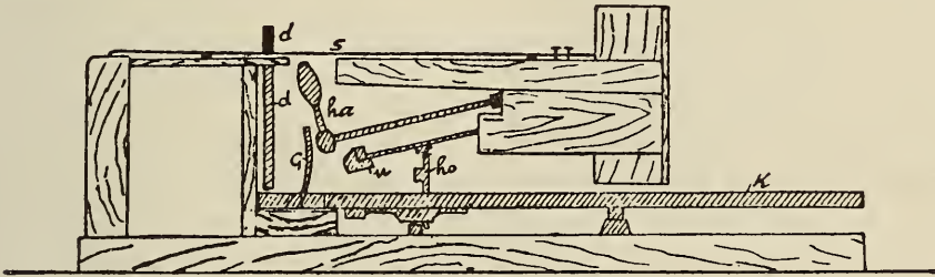
FIG. 4. Cristofori's action in a pianoforte of the Universitäts Museum, Leipzig
