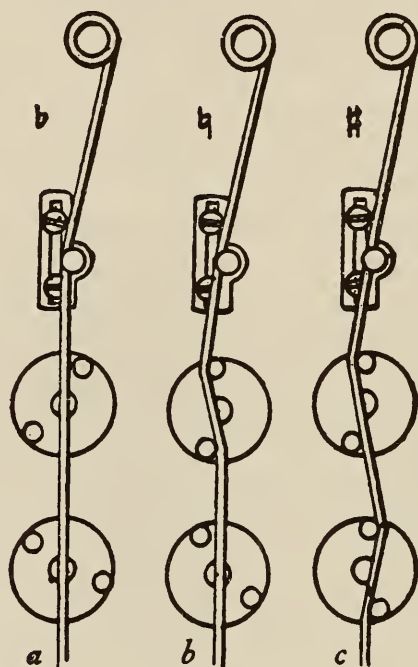
FIG. 5. Mechanism of a double-action pedal harp
