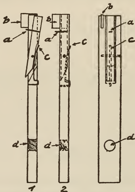
FIG. 2. Jack of the spinnet or harpsichord
