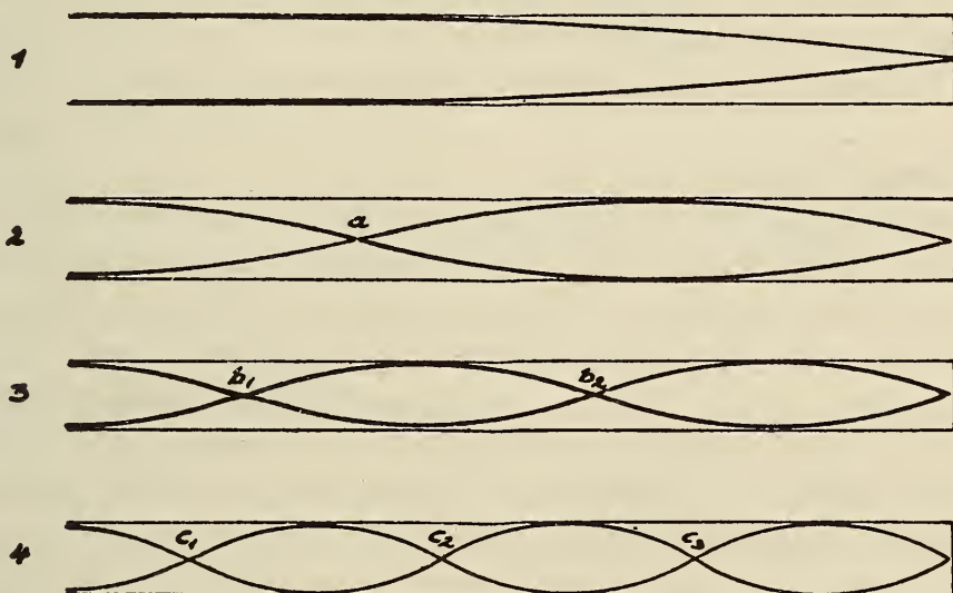
FIG. 11. Diagrams of sound waves inside a tube closed at one end (presented in the form of transverse waves)
