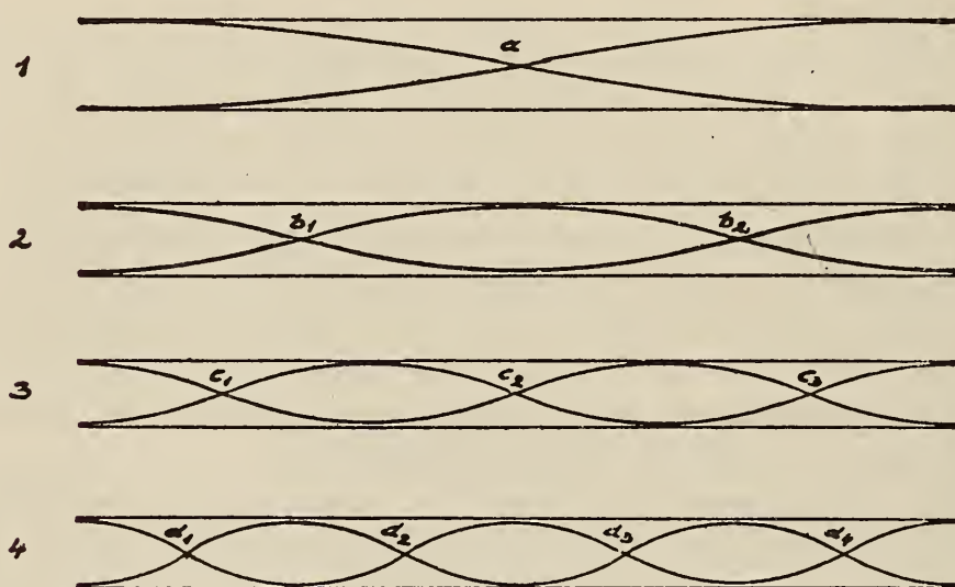
FIG. 10. Diagrams of sound waves inside a tube open at both ends (presented in the form of transverse waves)
