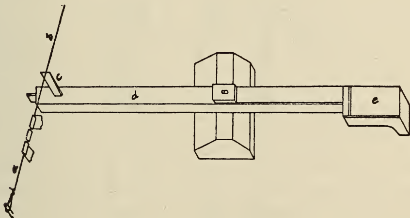
FIG. 1. Clavichord Key
