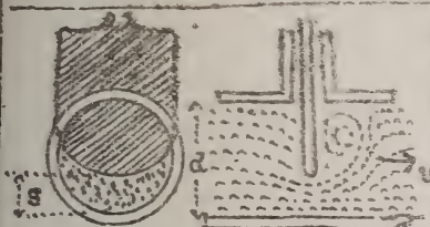
Fig. 574 Valve Gate.
