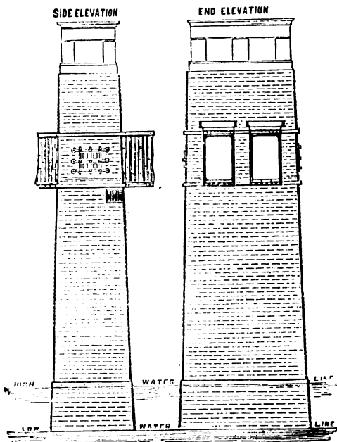
FIG. 98 a.—Land Tower.
