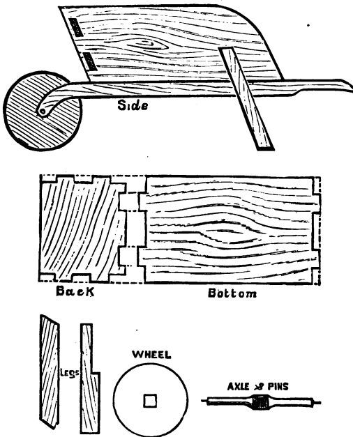
FIG. 69.—Wheelbarrow.
