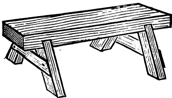
FIG. 63.—Carpenter's Stool.
