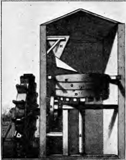
The Mill of Vitruvius.
