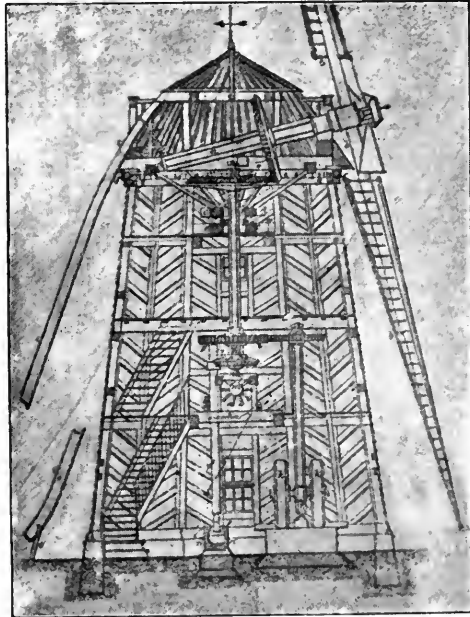
Modern Tower : Cap and Beam.
