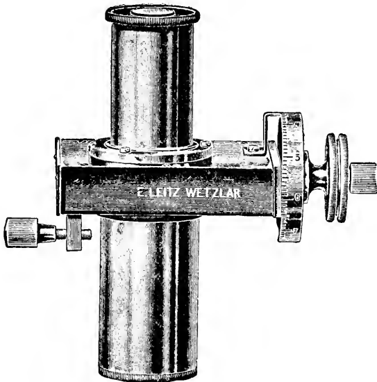
FIG. 24.—Micrometer Eye-Piece
