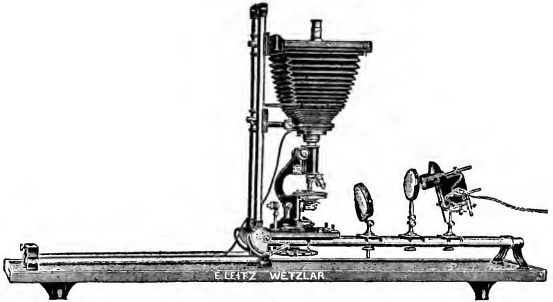
FIG. 29.—Microphotographic Apparatus
