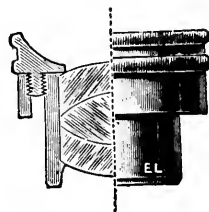
FIG. 9.—Abbé Condenser
