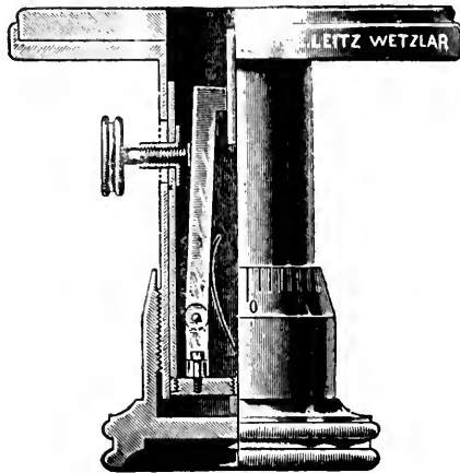
FIG. 34.—Hand Cylinder Microtome
