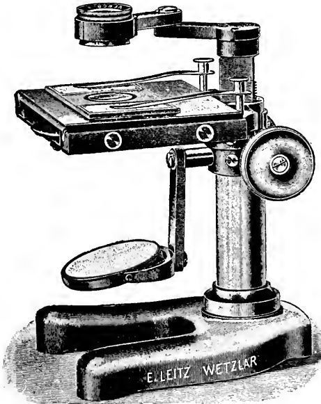
FIG. 6.—Dissecting Microscope
