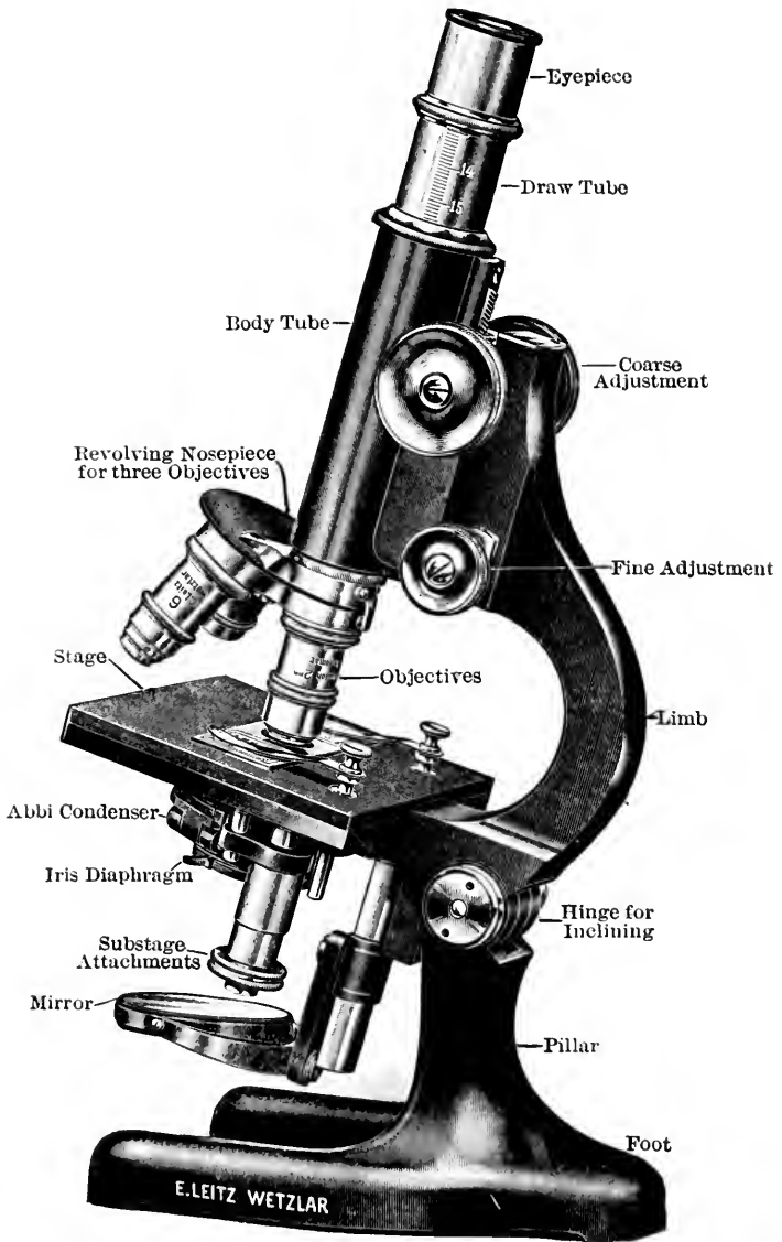
FIG. 8.—Compound Microscope
