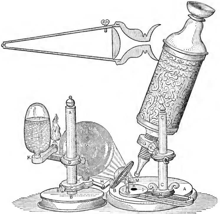
FIG. 7.—Compound Microscope of Robert Hooke
