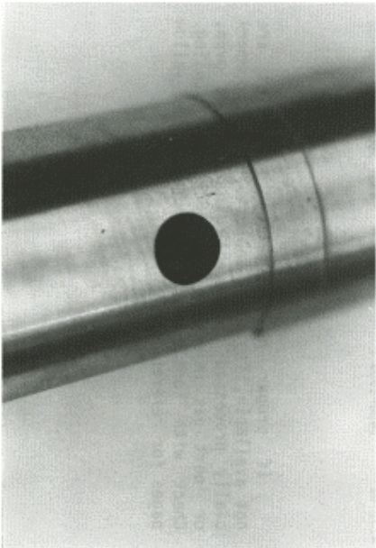
The bolt handle hole is drilled into the bolt body and grooved internally in two places to retain the bolt handle in "fire" and "safe" positions.
