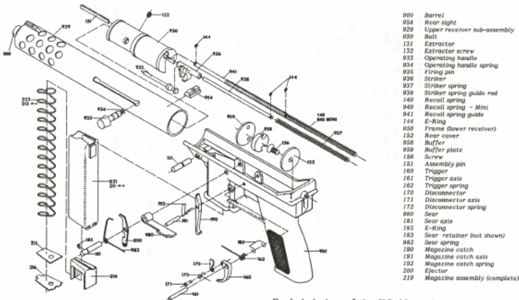
Exploded view of the KG-99 semi-automatic pistol.
