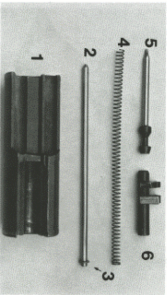
Semi-auto parts removed for the full auto conversion:
