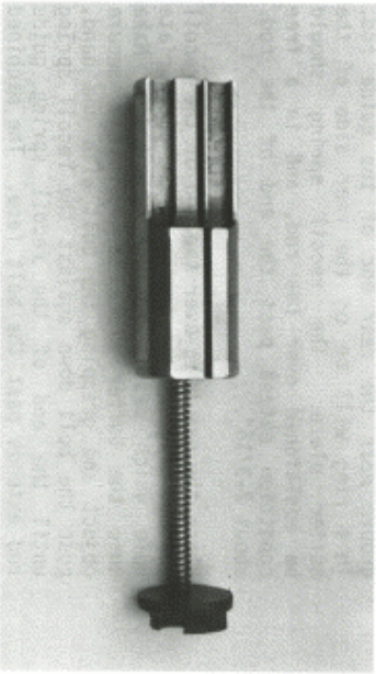
SMG Open-Bolt assembly ready for final assembly in upper receiver.
