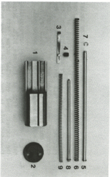
SMG Bolt Assembly field stripped: NOTE Items 8 & 9 are now deleted and not necessary for the SMG conversion.
