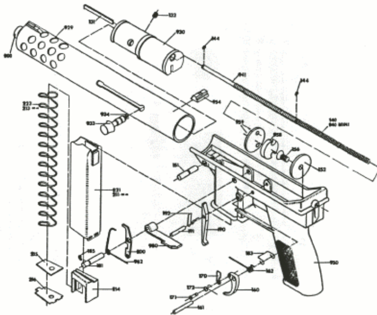
Exploded view of the KG-99 open-bolt SMG.
