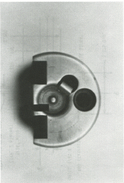
Close up view of front of SMG bolt. Note extractor, fixed firing pin, raised feed lip, recoil spring guide rod hole, and clearance notches for magazine feed lips and ejector.
