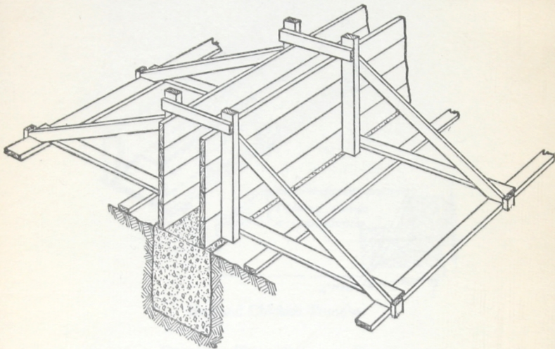
Wall Form on Top of Ground
