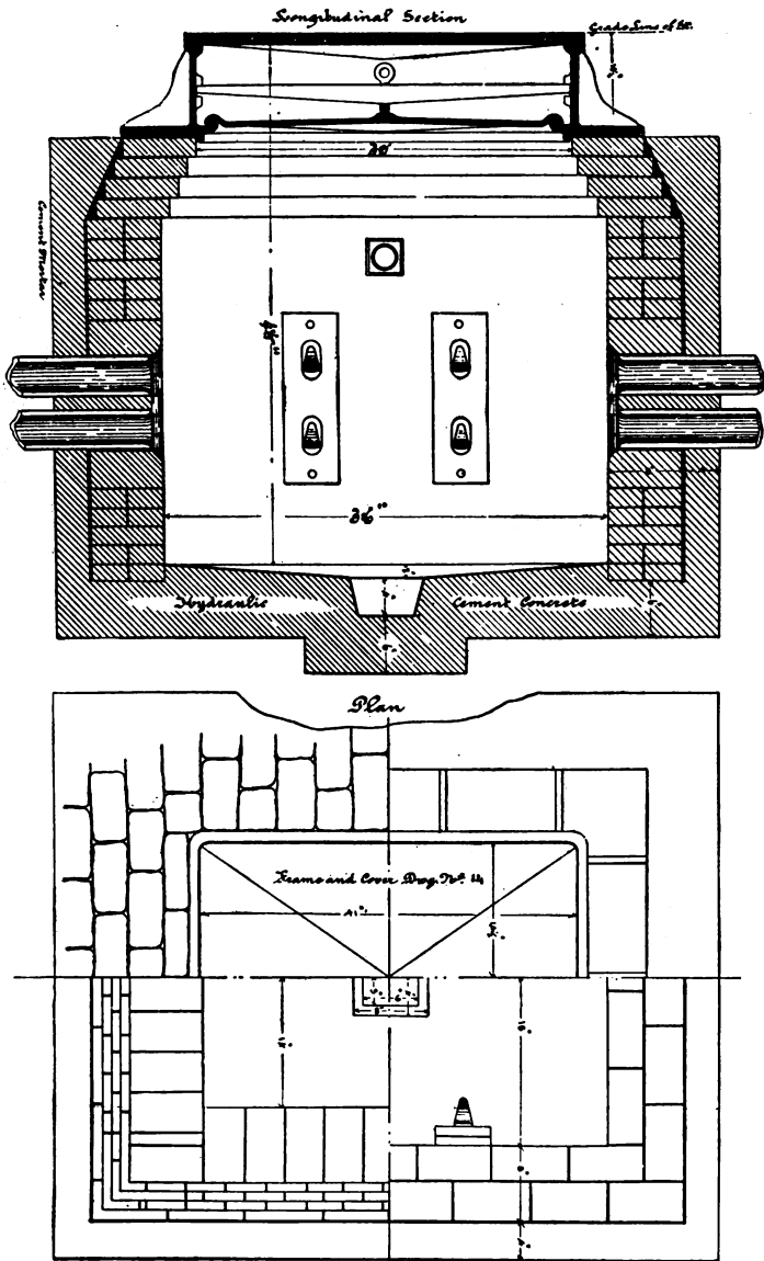
Fig. 30. Typical Brick Manhole.
