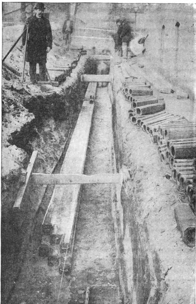
Fig. 13. Partially Complete Hollow-brick Conduit, Showing Mandrels.
