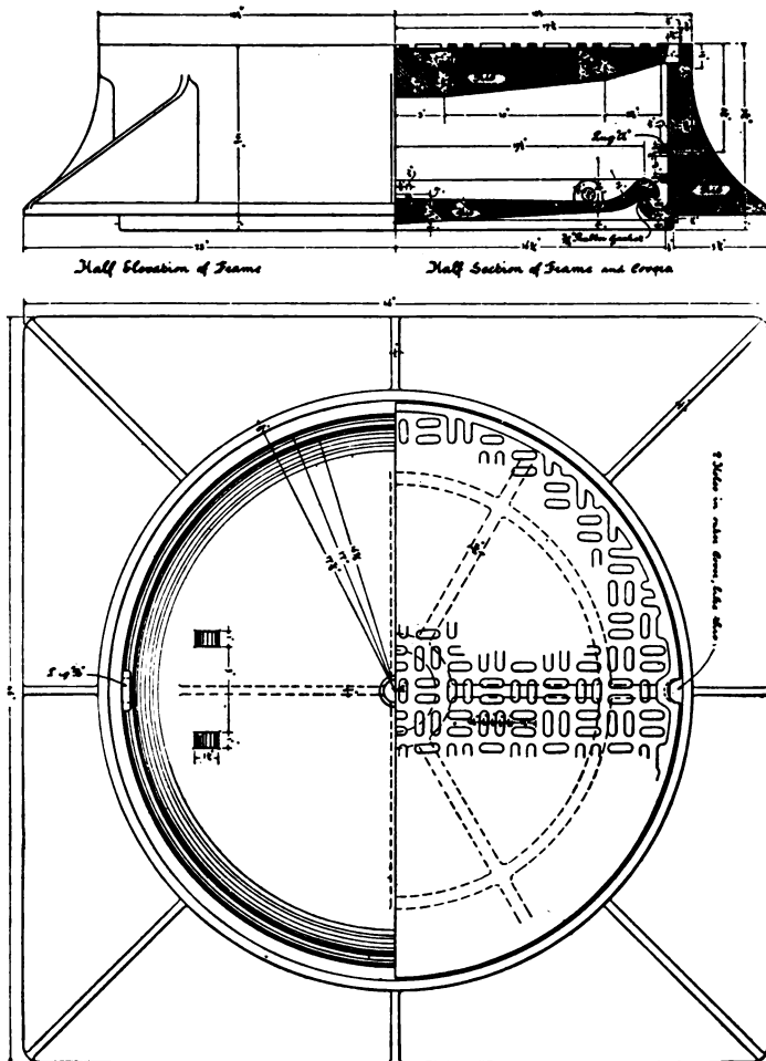
Fig. 34. Circular Tight Manhole Cover, Overhung Inner Cover.
