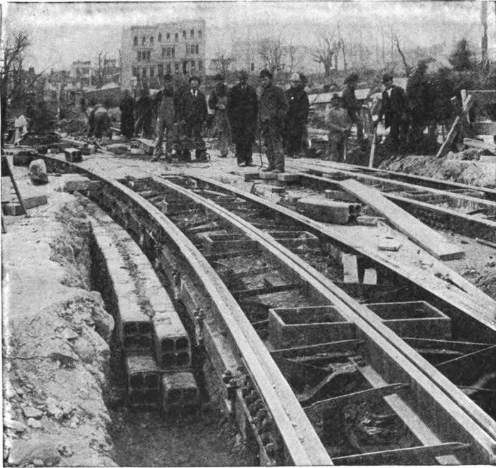
Fig. 20. Multiple Duct Curve.
