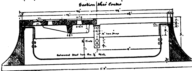
Fig. 37. Open Manhole Cover,
