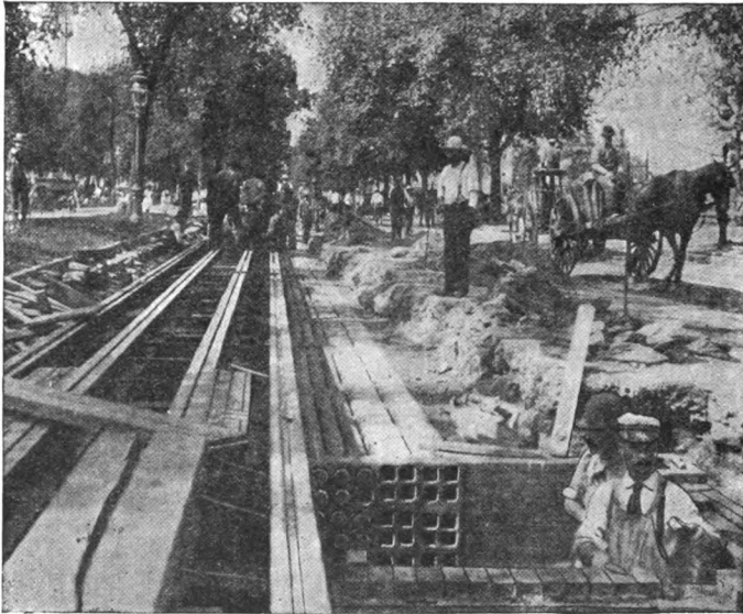
Fig. 19. Cement Pipe and Ducts.
