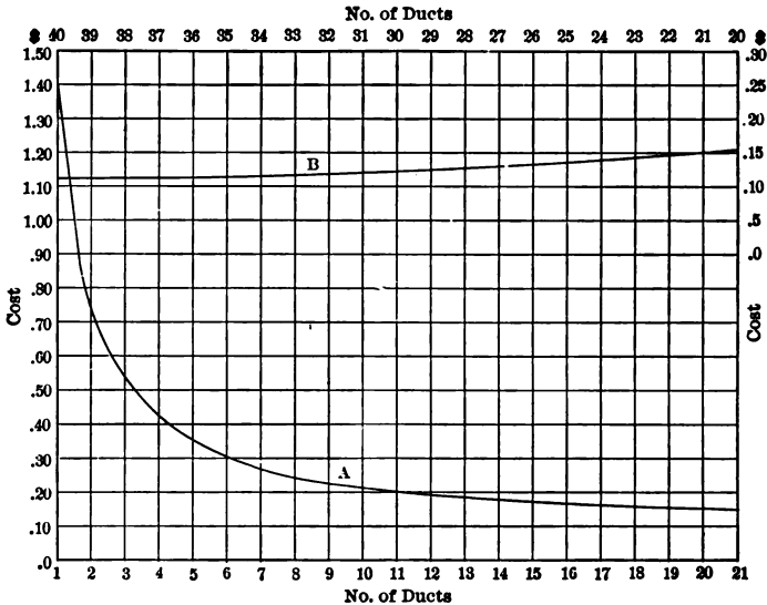
Fig. 56. Cost per Duct Foot; Average.
