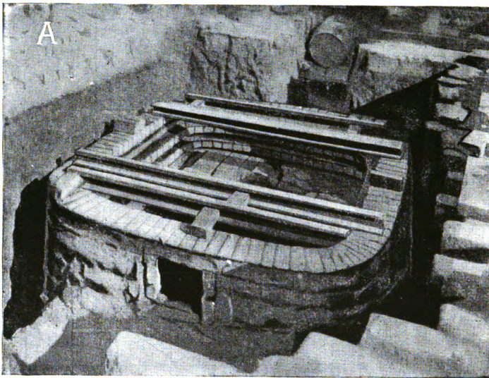
Fig. 31A. First Course for Rail Roof. Rails In Place.
