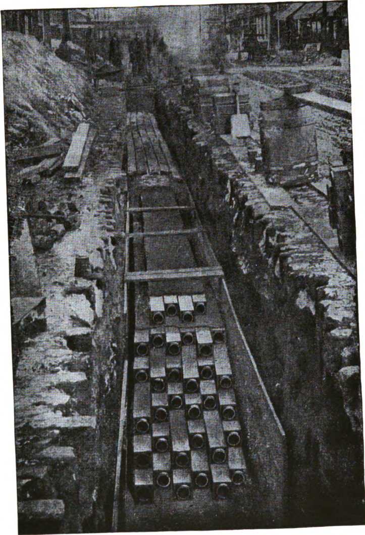
Fig. 25. Subway of 34-Single-ducts.
