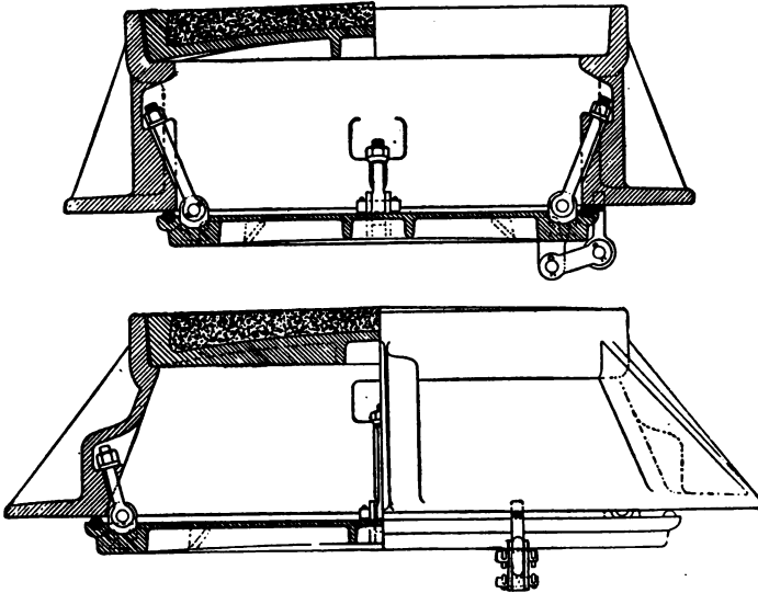
Fig. 36. Baltimore Manhole Frame and Cover.
