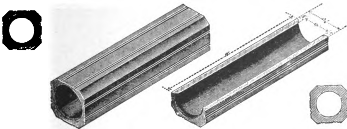
Fig. 10. Hollow-brick Ducts.
