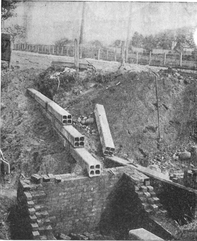
Fig. 15. Multiple Duct.
