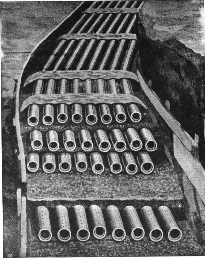
Fig. 6. Cement-lined Pipe Subway.
