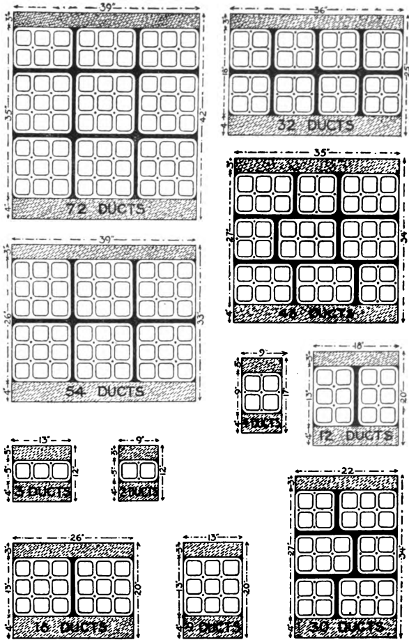
Fig. 24. Groupings of Multiple Ducts.
