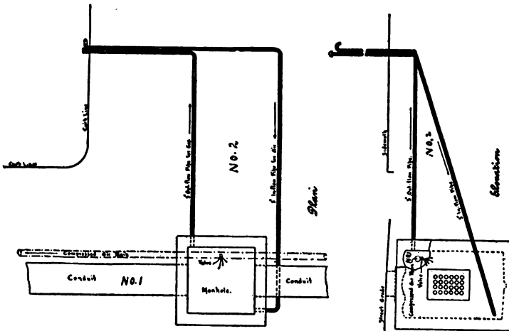
Fig. 53. Ventilating Systems.
