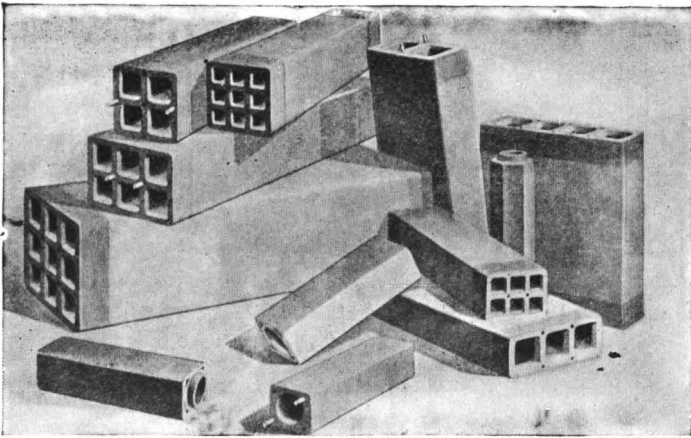
Fig. 22. Some Multiple Duct Forms.
