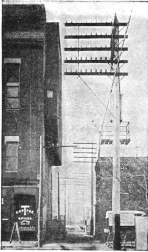
Fig. 41. Alley Line for Distribution.
