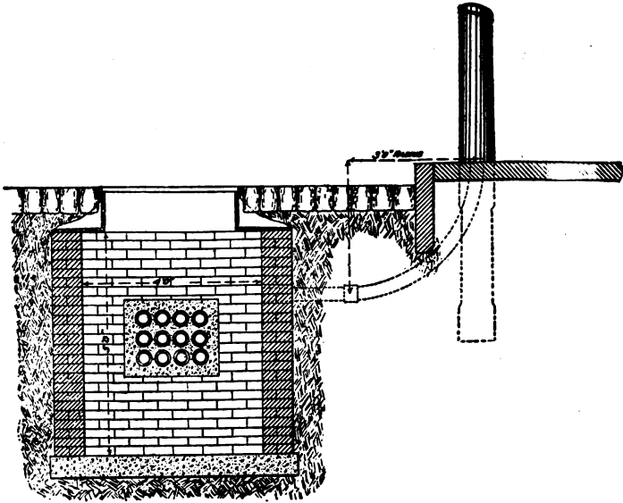
Fig. 40. Manhole with Lateral Connection.
