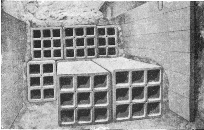
Fig. 26. Multiple Ducts.
