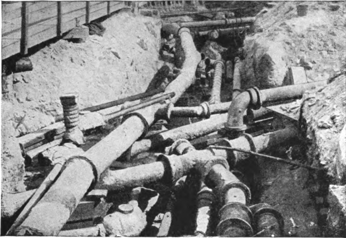
Fig. 51. A New York Street Corner, Showing Underground Pipe Construction.
