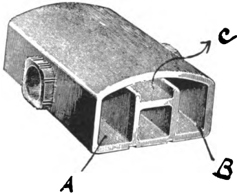
Fig. 47. Johnston Distributing Duct.
