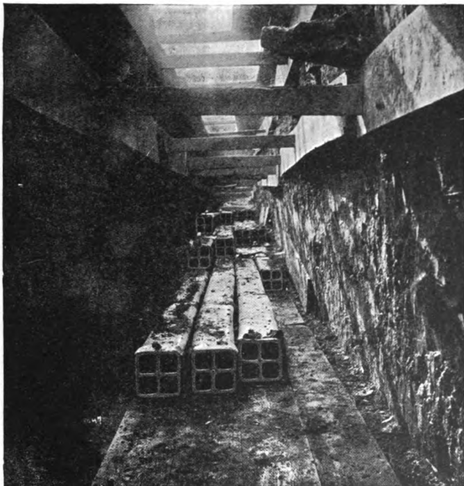
Fig. 18. Multiple Duct Conduit with Timber Foundation.
