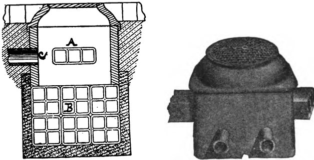
Figs. 43 and 44. Tile Service Distribution Box with Iron Surface Cover.
