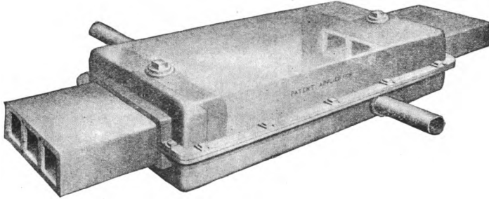
Fig. 45. Iron Service Box for Three-way Conduit, Two Services.
