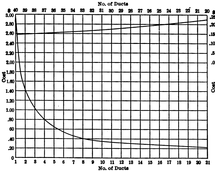
Fig. 57. Cost per Duct Foot; Maximum.
