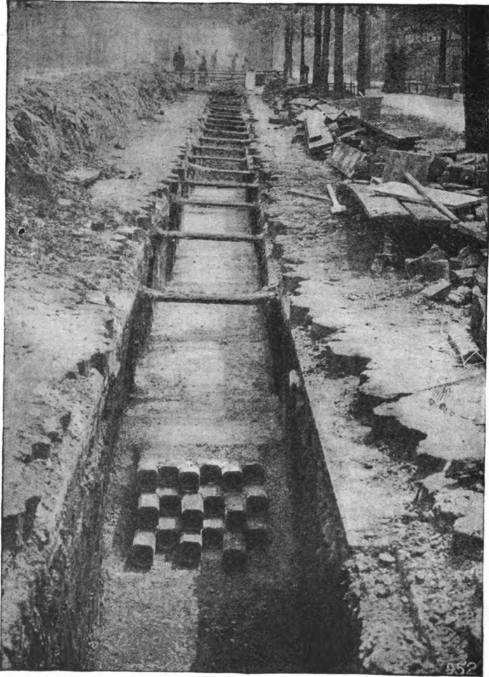
Fig. 14. Completed Conduit Trench Ready to Refill.
