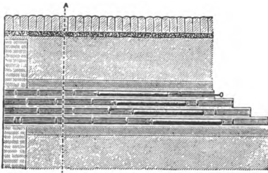
Fig. 12. Showing Use of Mandrel.
