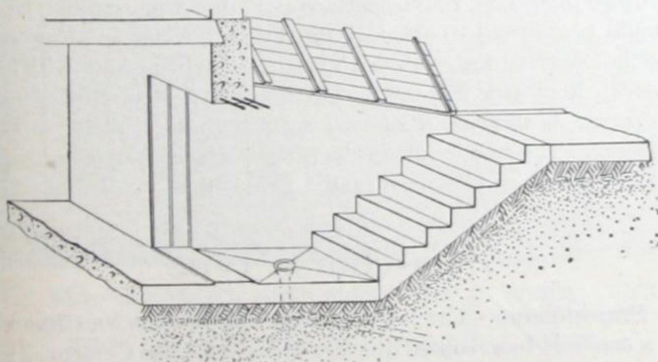
Fig. 43—Detail of hatchway steps.
