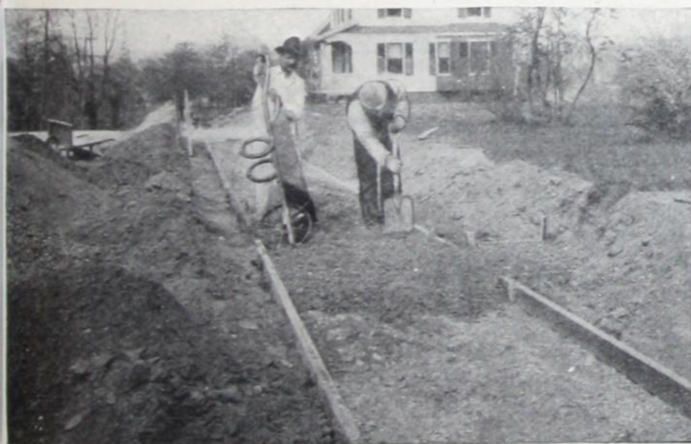
Fig. 48A—Building a small sidewalk in a country village. Two men at work—one wheeling and dumping, the other smoothing the concrete with a shovel.
