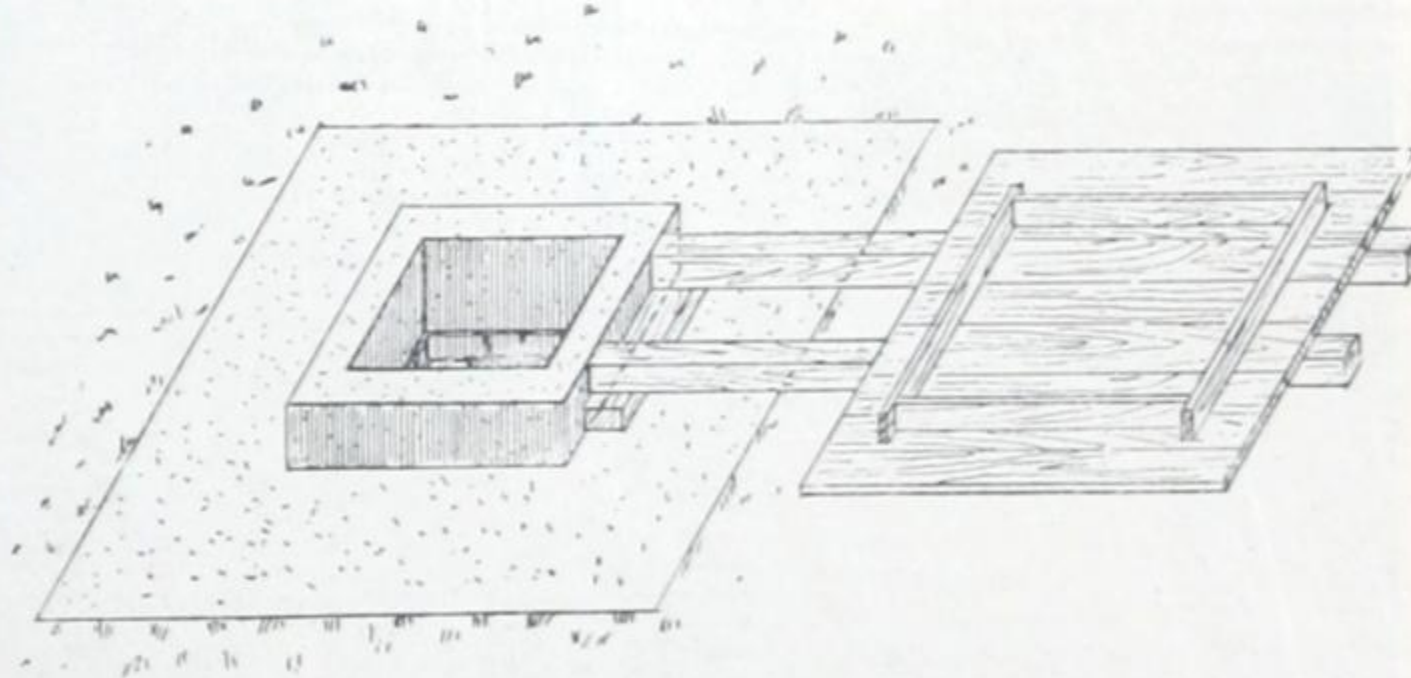
Fig. 126—Forms for well cover to be built at one side of the well and then skidded into its place over the top of the well.
