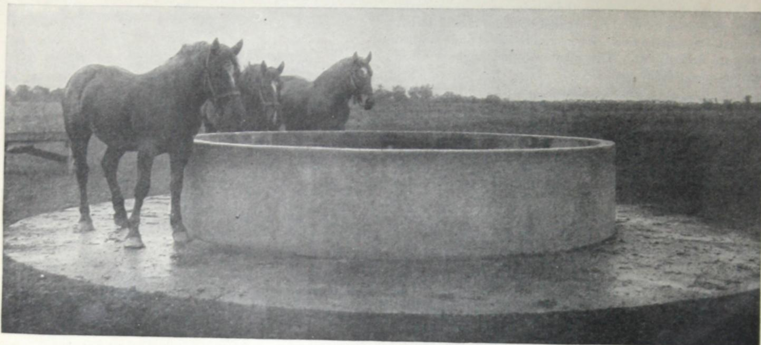
Fig. 114—Circular drinking trough of concrete, no corners to leak or bark legs of horses or cattle. The concrete pavement keeps the approach to the trough from getting muddy.
