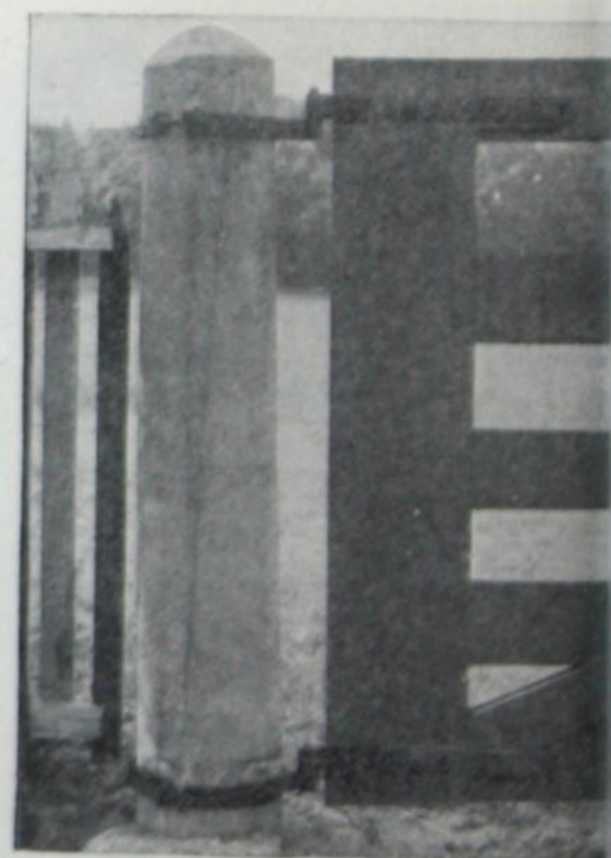
Fig. 146—A concrete gate post showing adjustable iron hoop hangers for hinges.
