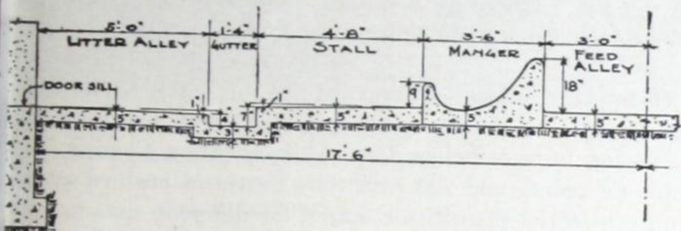
Fig. 61—Floor as in Fig. 60.
