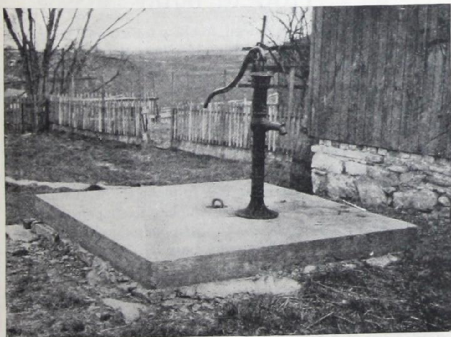
Fig. 125—A substantial, clean, sanitary well platform of concrete.
