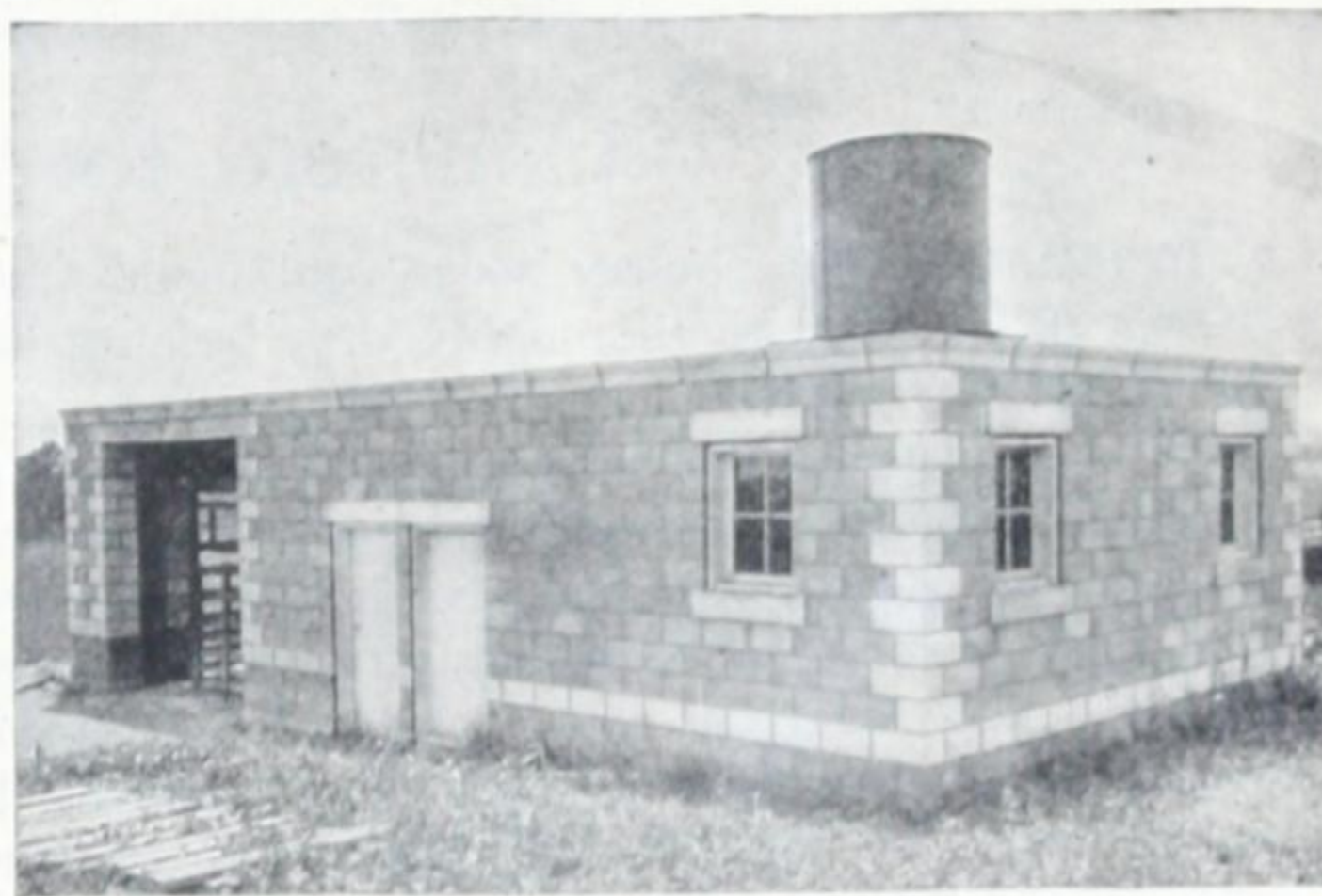
Fig. 84—Concrete block power house and farm scales.
