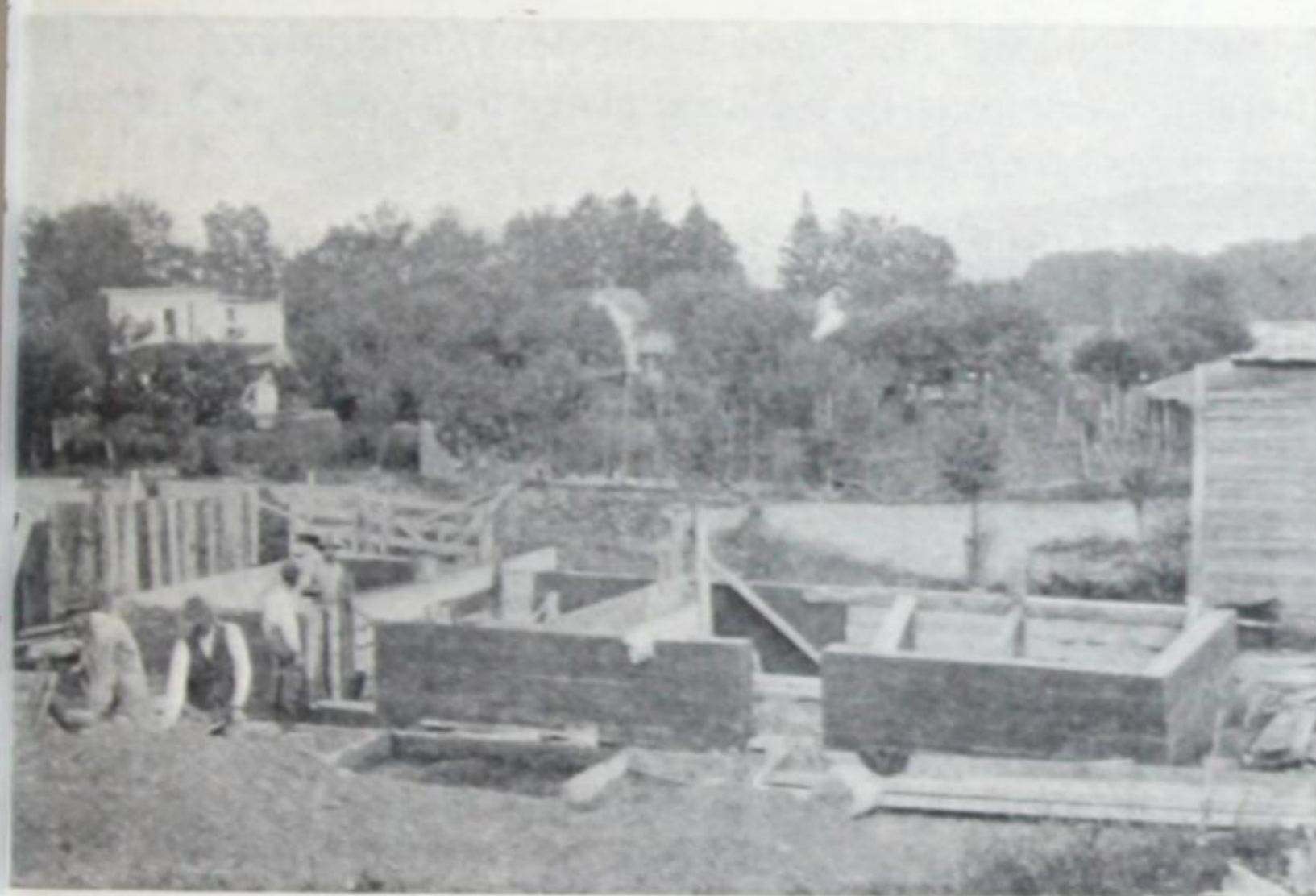
Fig. 23—Partly finished concrete walls showing spaces for doors and forms for partition walls.
