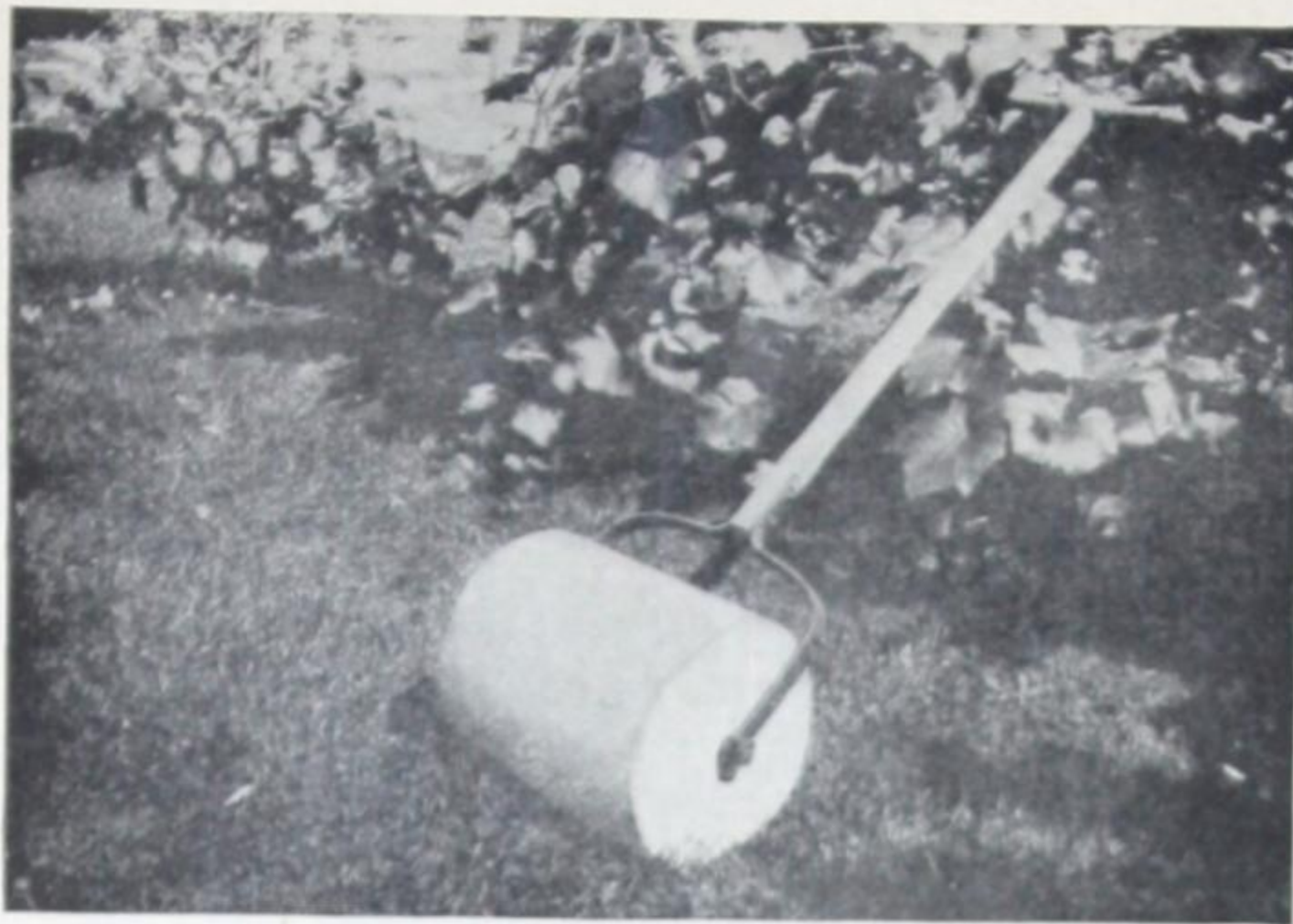
Fig. 170B—The complete roller ready for actual use.
