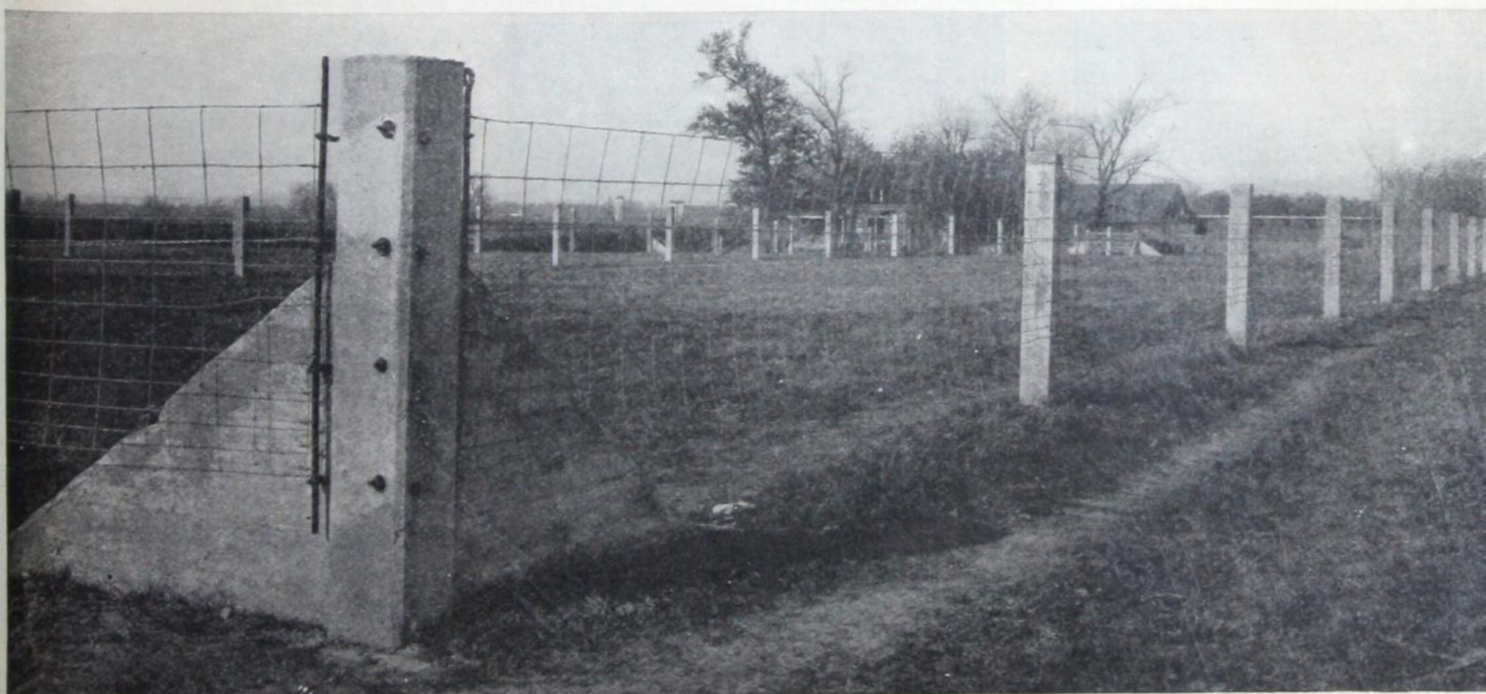
Fig. 143—Corner post double-braced. The eye bolts through the post hold rods to which the woven wire is attached; it may be tightened by screwing up the nuts on the opposite side of the post.
