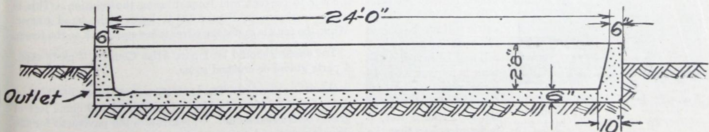
Fig. 130—Detail for manure pit. Simple, but efficient construction.
