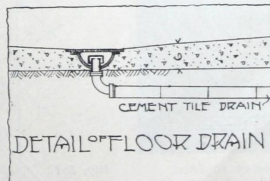
Fig. 184—Details for small garage.
