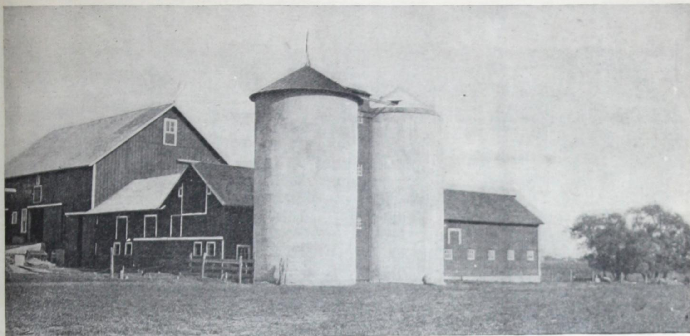
Fig. 104—Twin circular silos of monolithic concrete built against a frame barn.
