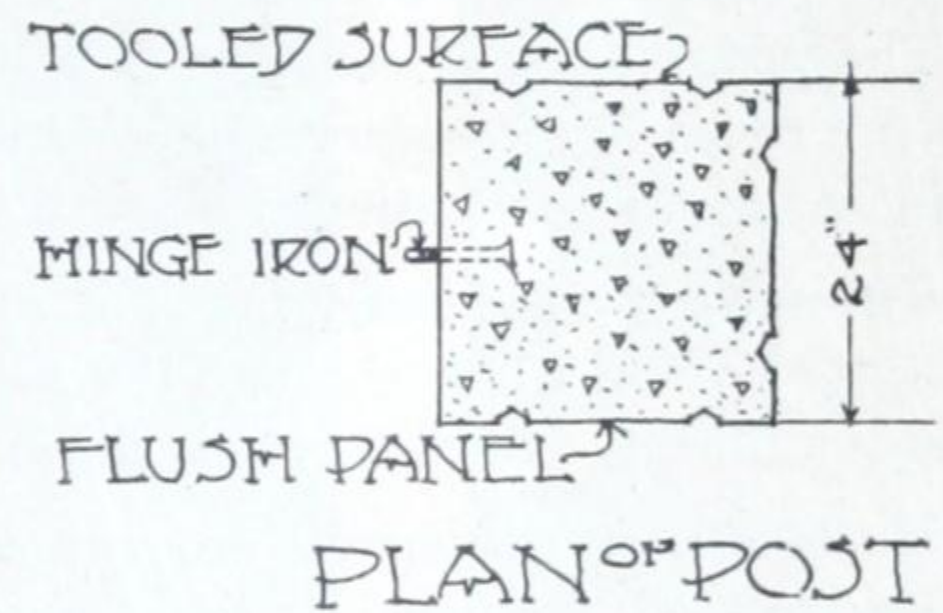
Fig. 147—At the top, general construction and reinforcement of gate posts. The bracing, as in Fig. 156 on page 73, and one way of anchoring a gate hinge—see also Fig. 146. In the center the form for the posts. To the right, the reinforcement and the dimensions of a concrete rail.
