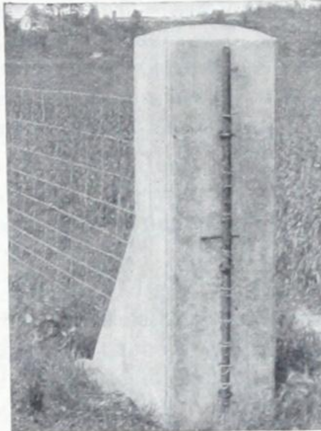
Fig. 155—Braced post pierced for wires and for eyebolts to hold rod on which wires are fastened.
