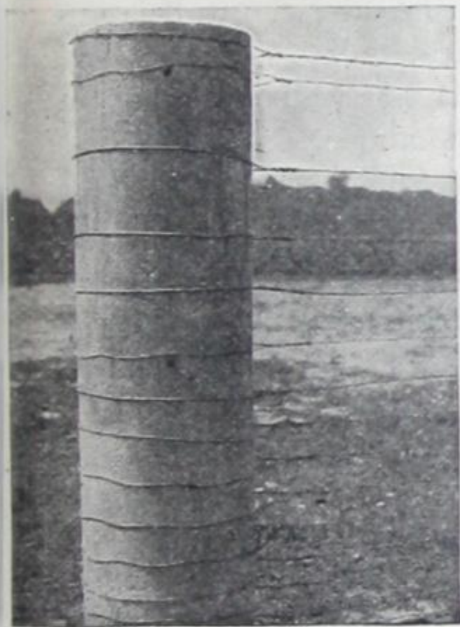
Fig. 153—Corner post in concrete—individual wires carried around and tied.
