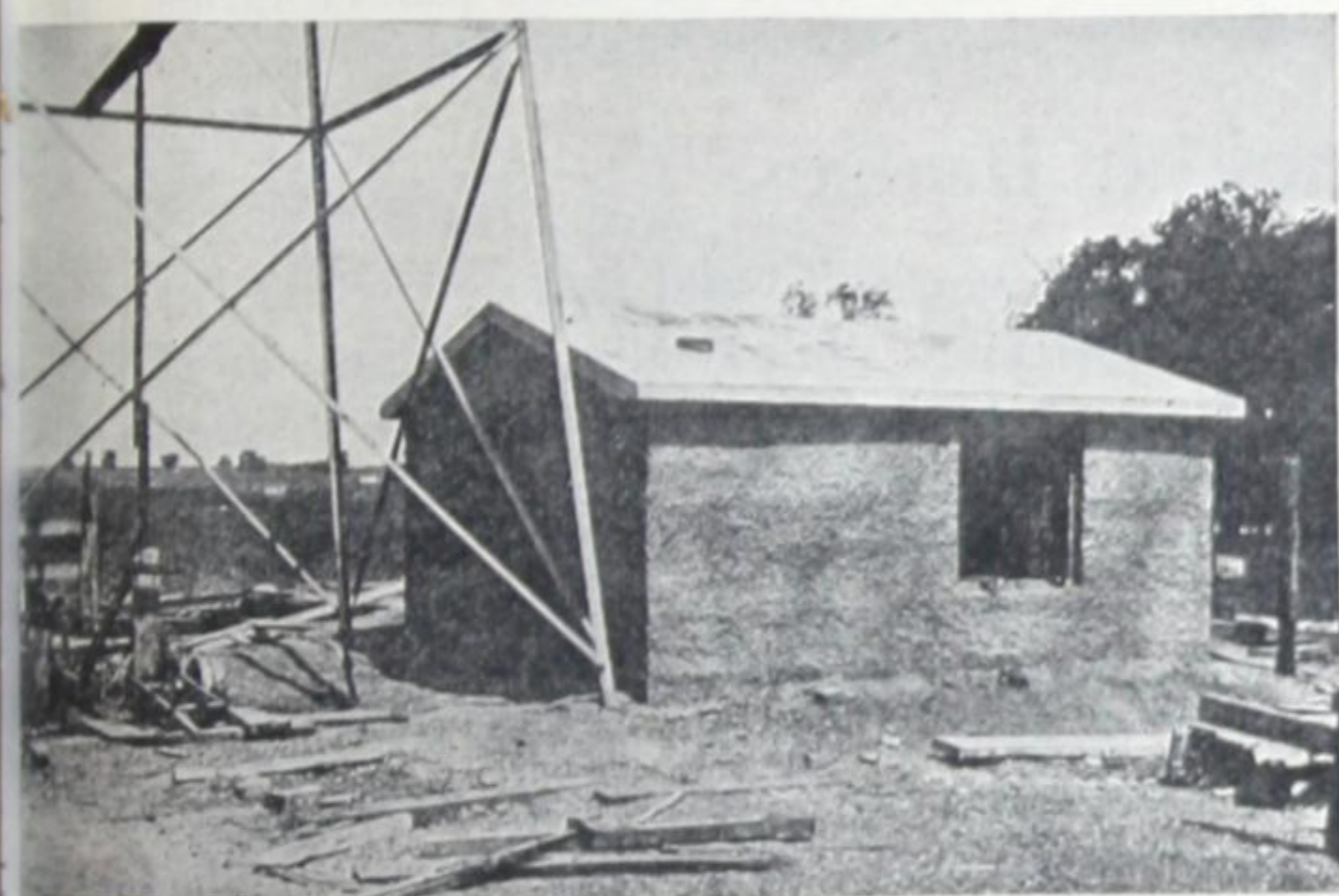
Fig. 83—Concrete engine house
