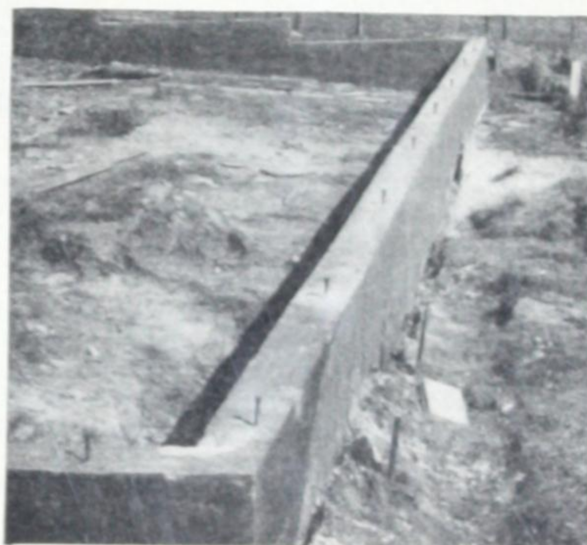
Fig. 24—Barn basement with projecting imbedded bolts for tying sills of superstructure to foundation.
