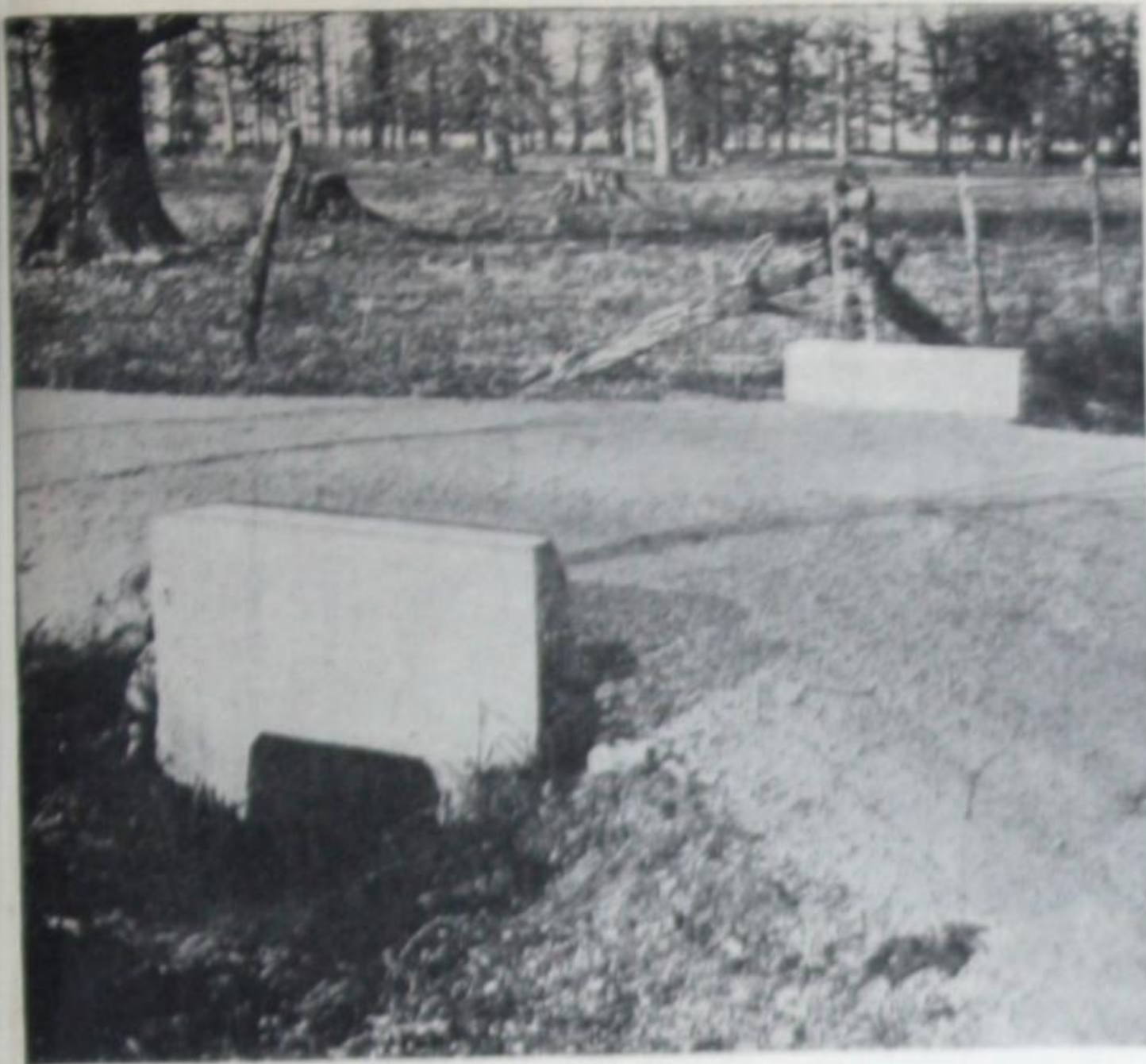
Fig. 188—Small concrete culvert of square type for a country road.
