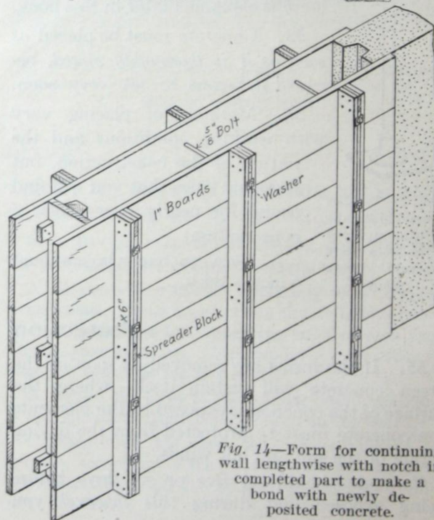
Fig. 13—Form for carrying wall up with use of least possible lumber.
