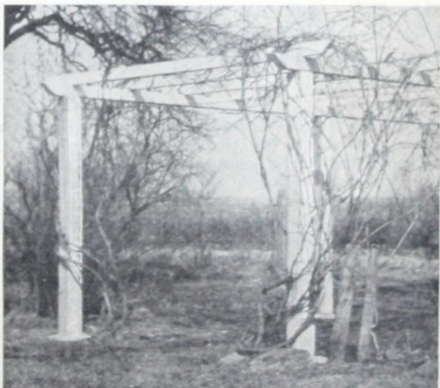
Fig. 174—Grape arbor with permanent and handsome pillars built of concrete
