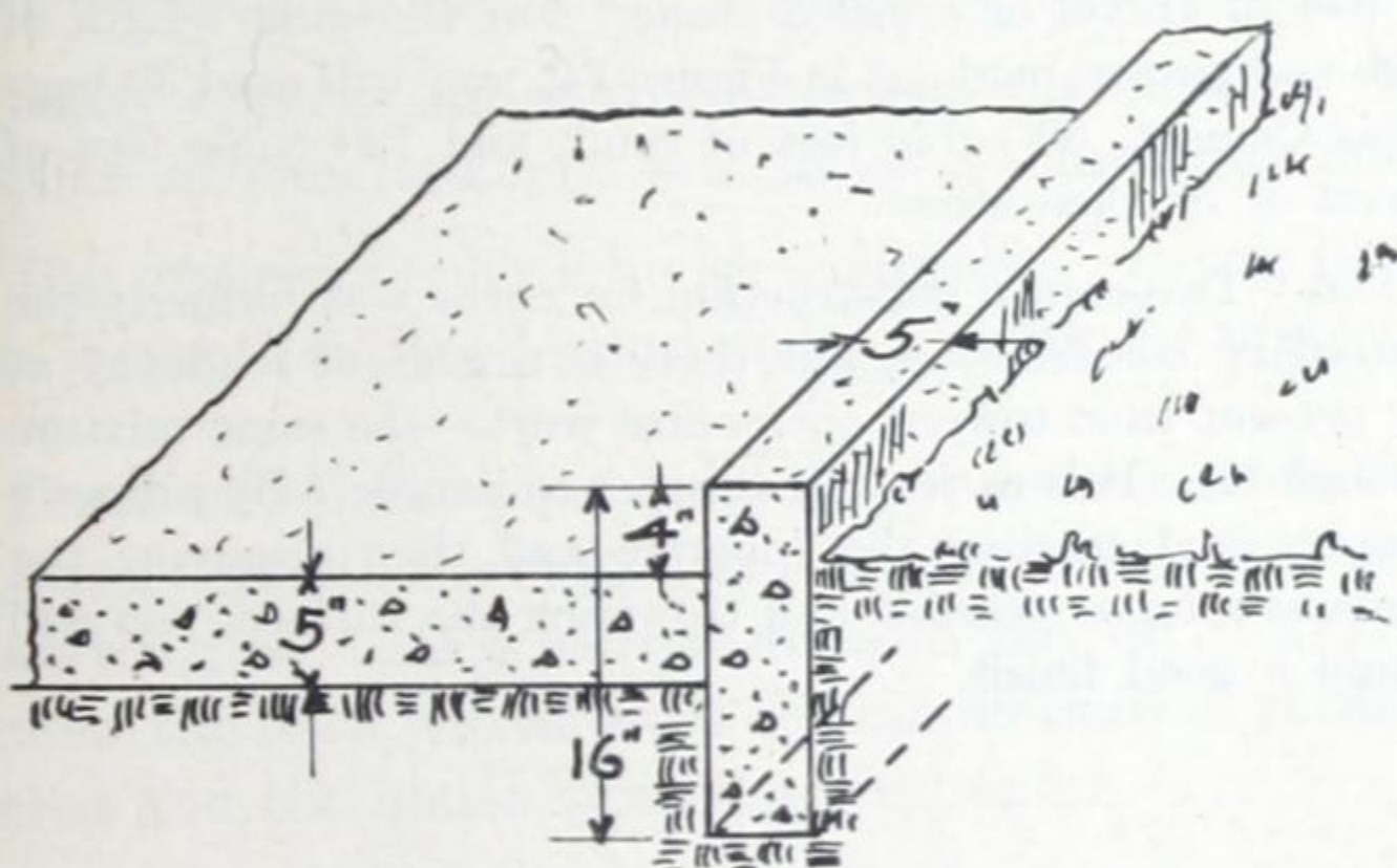
Fig. 69 —Diagrams showing construction of feeding floor. At the right the apron or turndown wall to prevent hogs from rooting up the floor.
