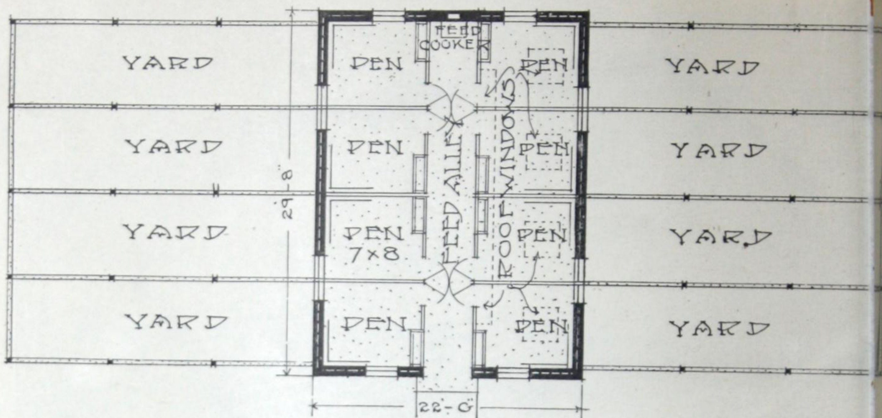
Fig. 110—Floor plan of model hog house.
