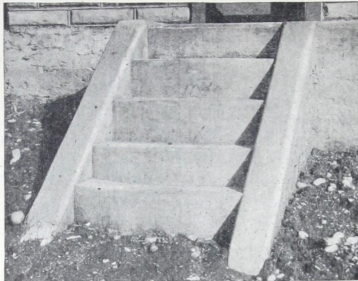
Fig. 44—Concrete steps with concrete side walls, as shown in Fig. 40. For description of walls, see pages 12 and 13 on forms and page 74 on construction in general.
