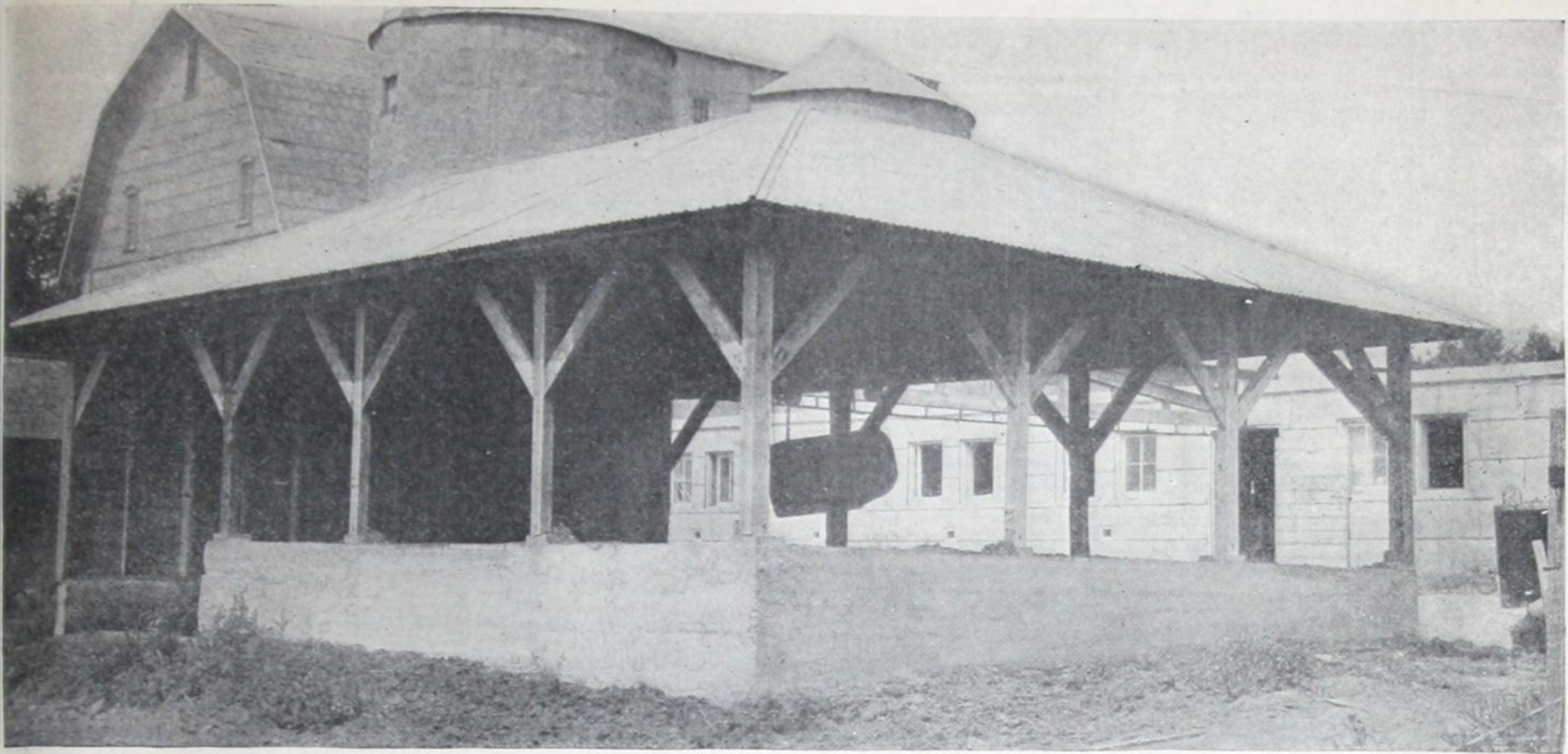
Fig. 129—Large concrete manure pit, roofed over, and provided with trolley carrier from barn.
