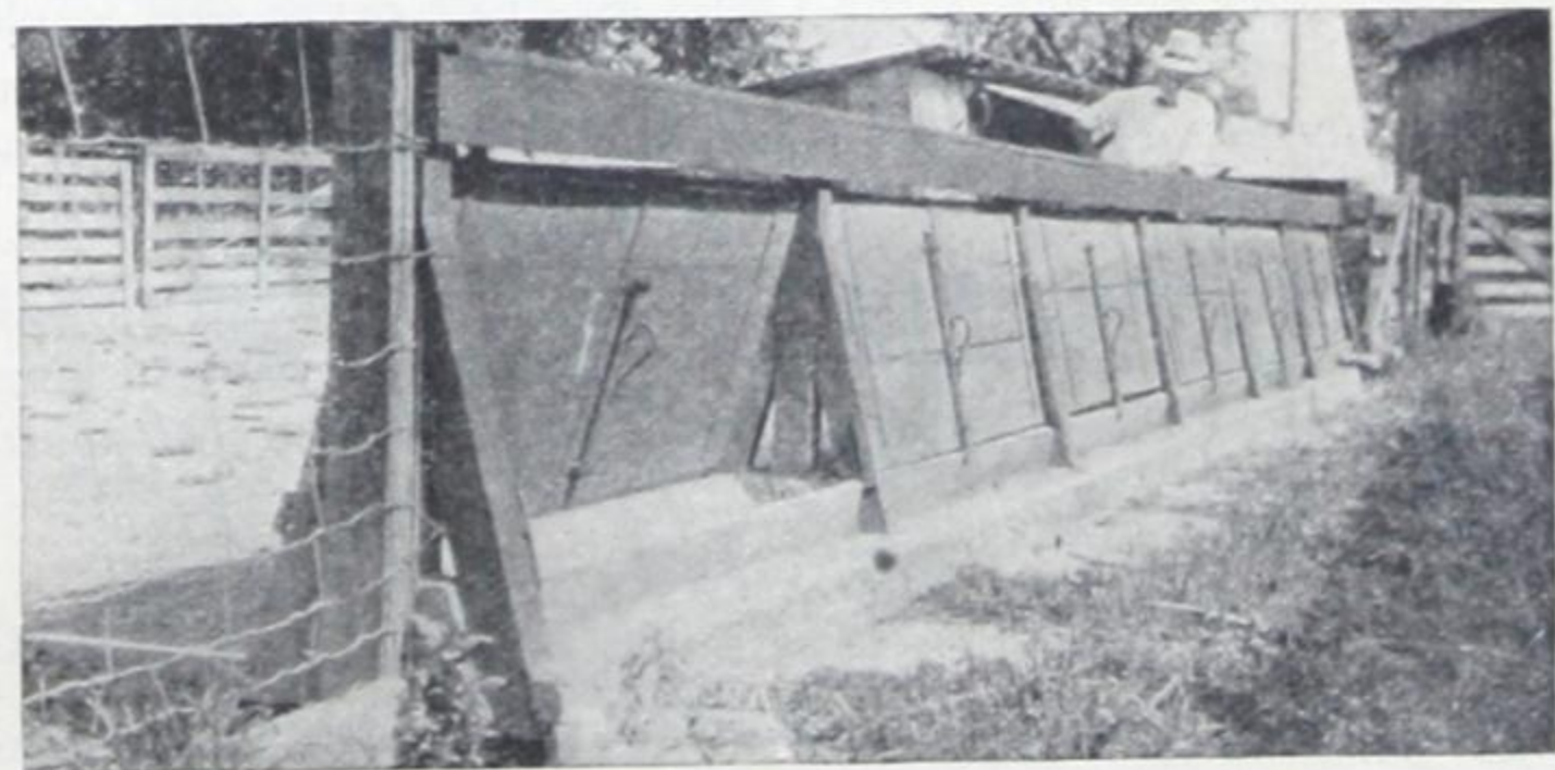
Fig. 159—Concrete feeding trough with flap corners.
