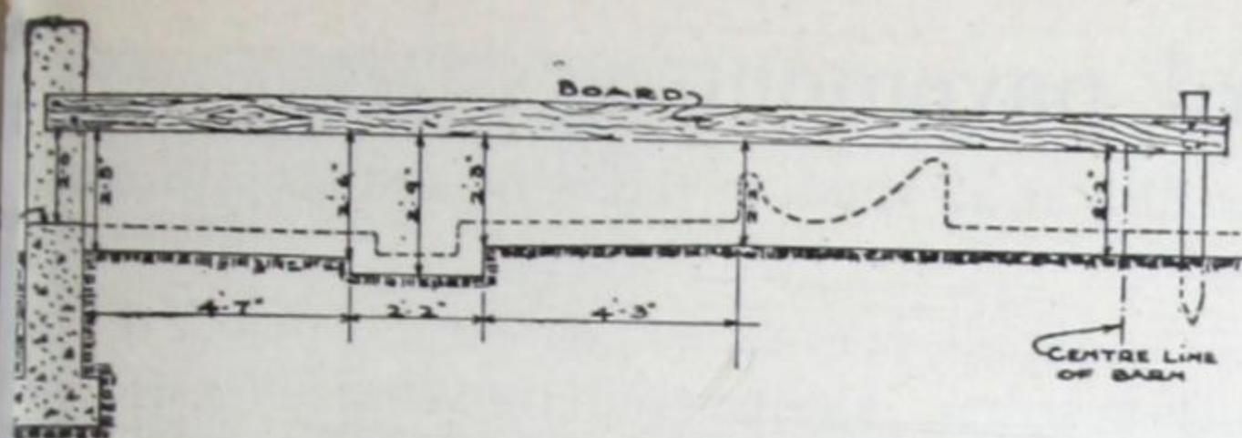
Fig. 60—Cow barn floor, cows facing in.
