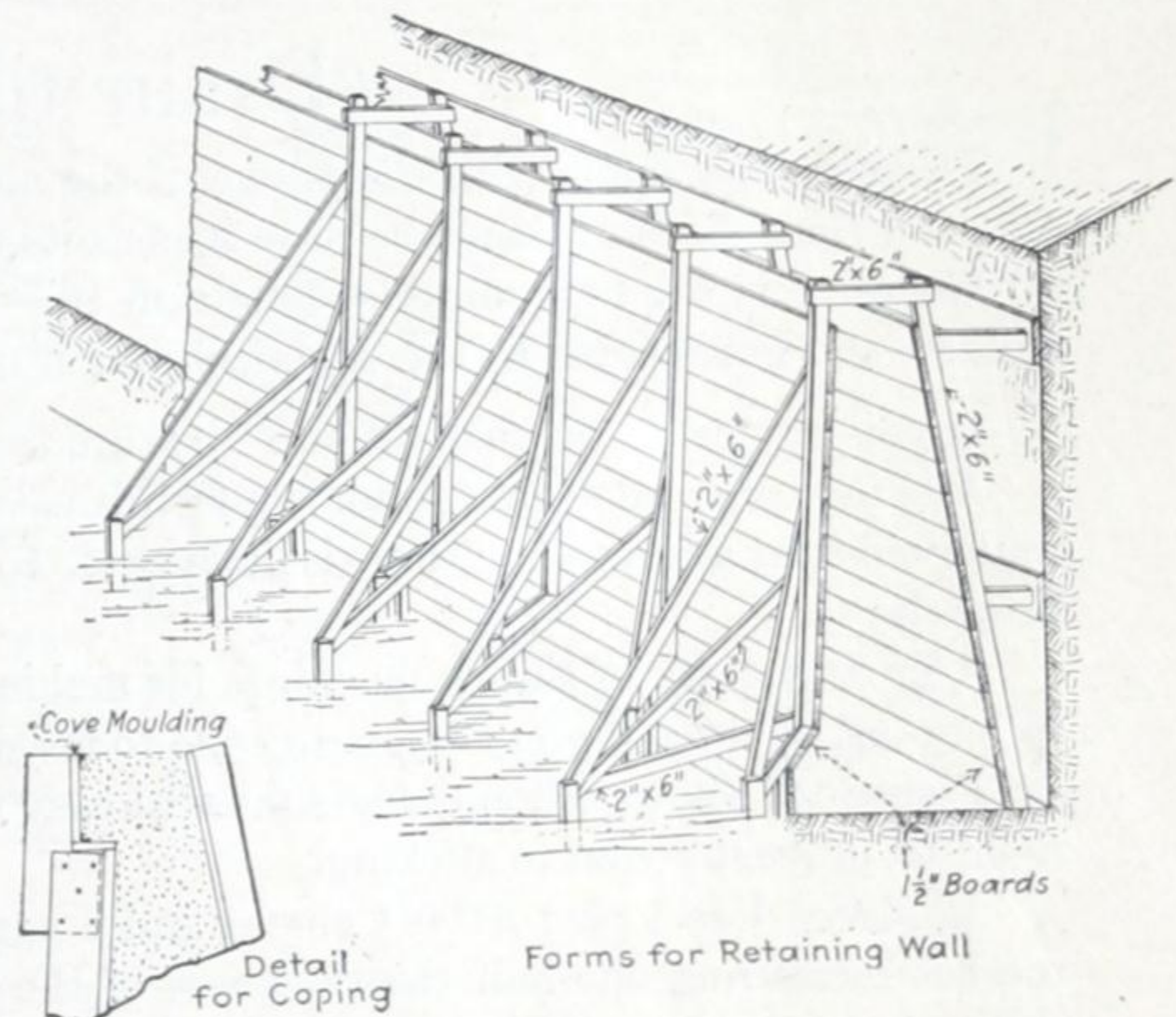
Fig. 163—Forms for retaining wall. Space back of the form (to the right) to be filled in after wall is completed. To the left, below, form for a top molding or coping.
