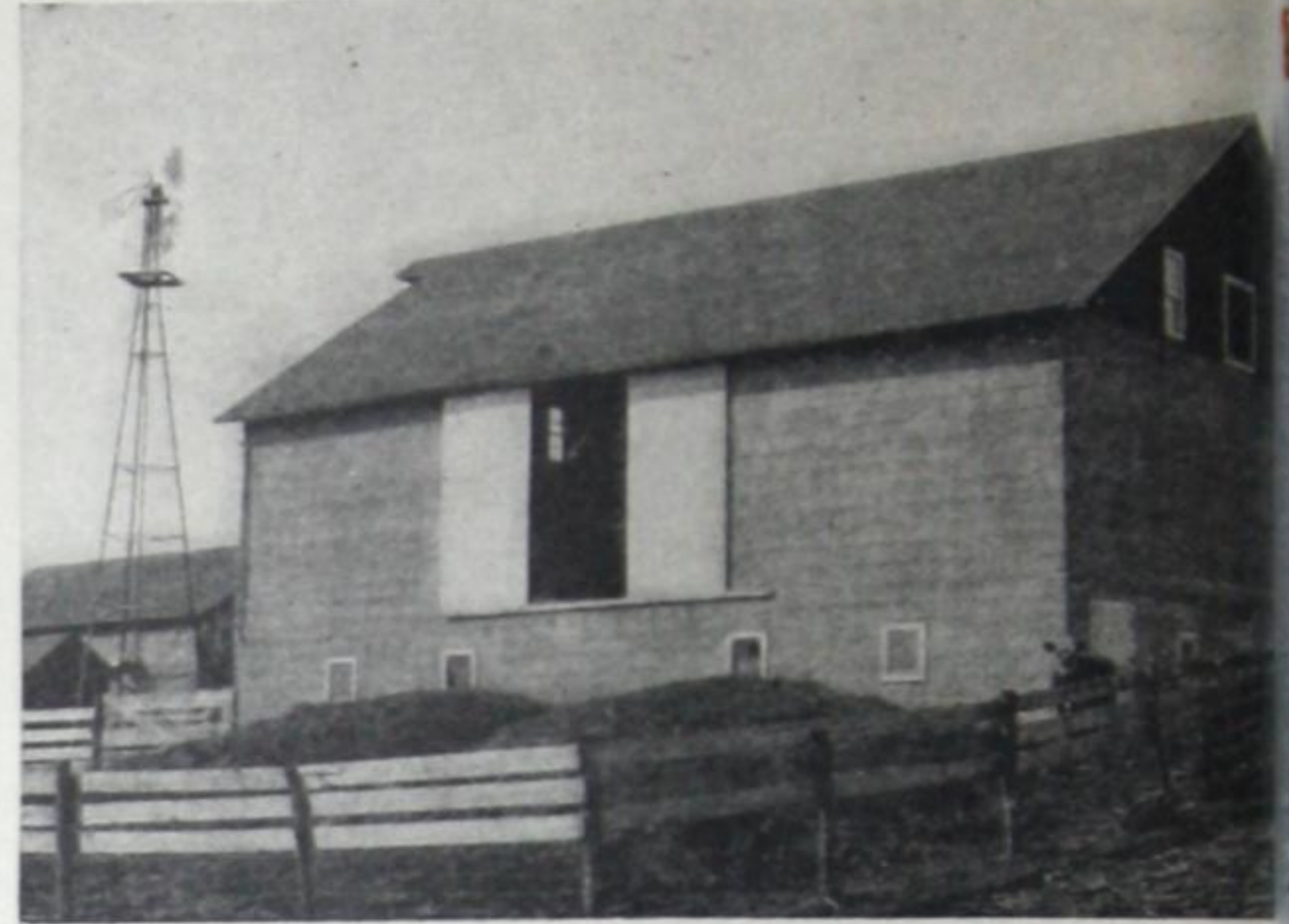
Fig. 96—A barn built of concrete to the eaves—a middle stage between Fig. 95 and the all-concrete barn. This gives the greatest possible safety in construction without a fire-proof roof.
