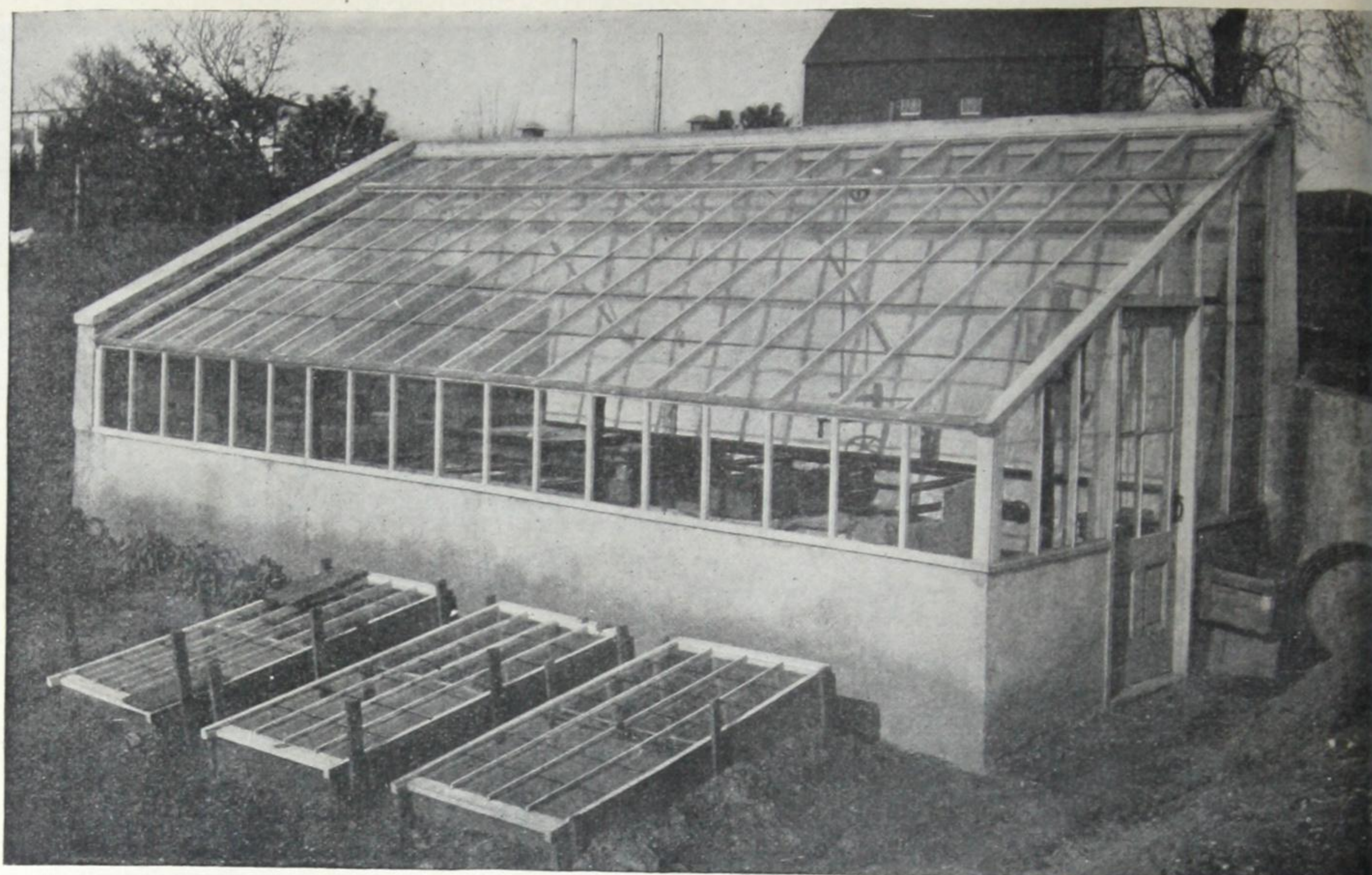
Fig. 92—A well constructed concrete greenhouse, with shed roof, built against a concrete retaining wall.
