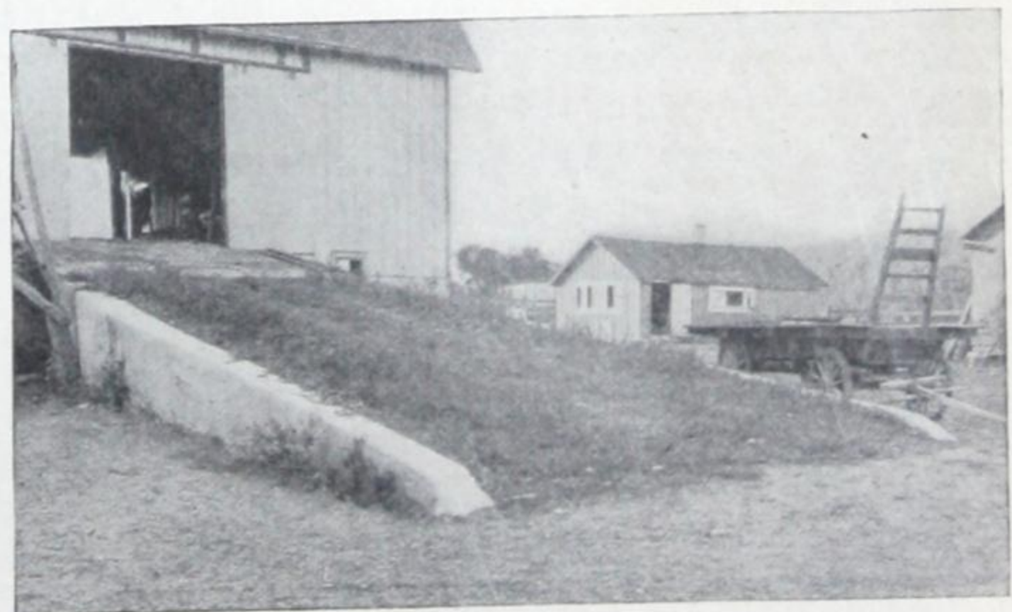
Fig. 164—Concrete approach to barn, with wooden platform for bridge over surface passageway.
