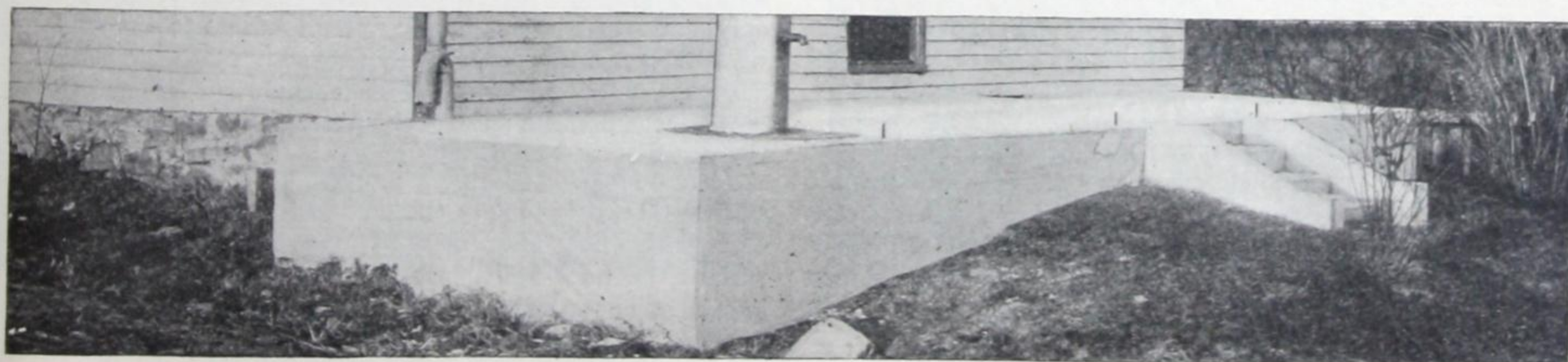
Fig. 59—Concrete porch floor and pump platform—showing spikes in floor to tie pillars to the floor.
