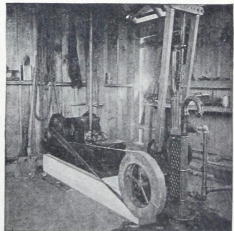
Fig. 33—Concrete engine base—saving wear and tear on engine, floor and whole building.
