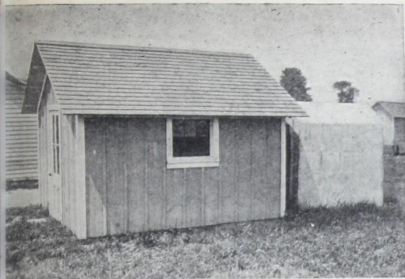
Fig. 81—Concrete milk cooler room with arch roof.
