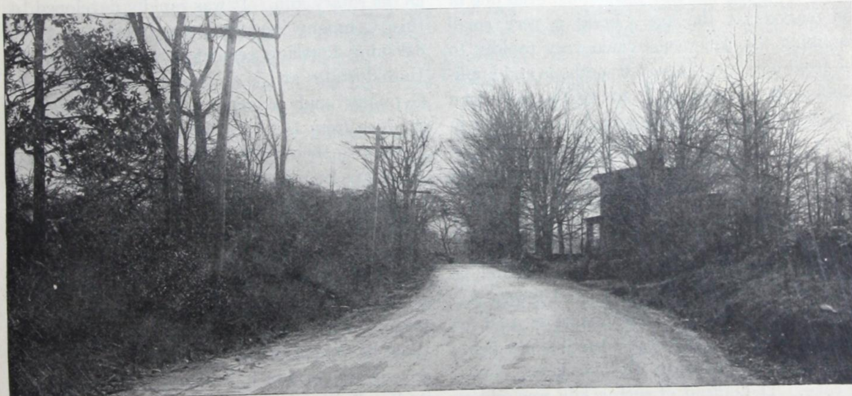
Fig. 201—A Greenwich, Conn., road built of Portland Cement concrete.
