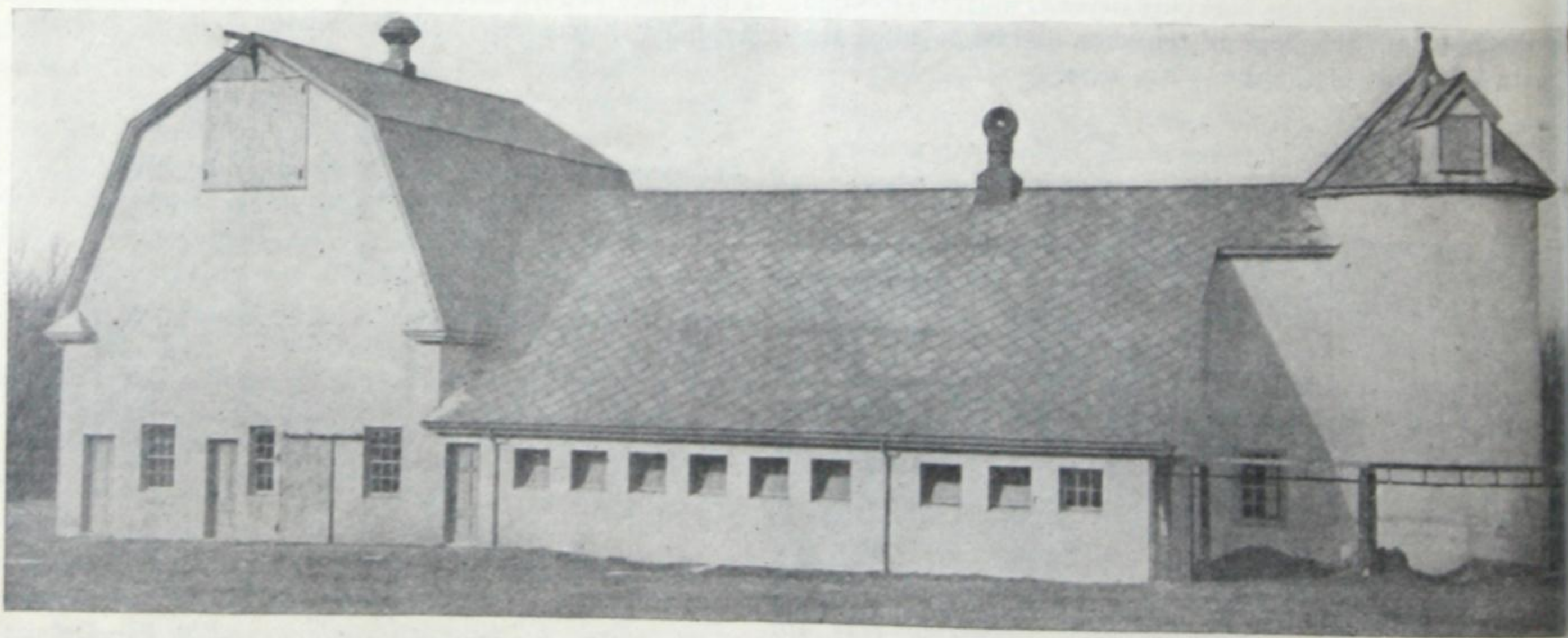
Fig. 97—Reinforced concrete barn, dairy and silo. Main building, 31 by 38 feet. Cow barn 50 by 38 feet.
