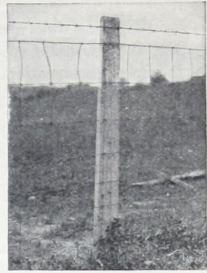
Fig. 152—Concrete line post with fencing held by wire rod through eyebolts.
