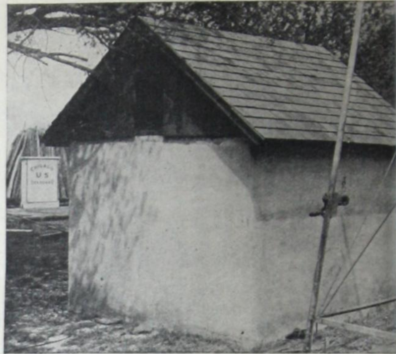
Fig. 118—Concrete water storage tank with wooden roof built beside windmill.
