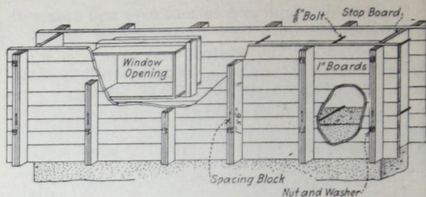
Fig. 12—Arrangement of form when window is to be inserted—Sectional form to be raised as wall is built up and used over and over.
