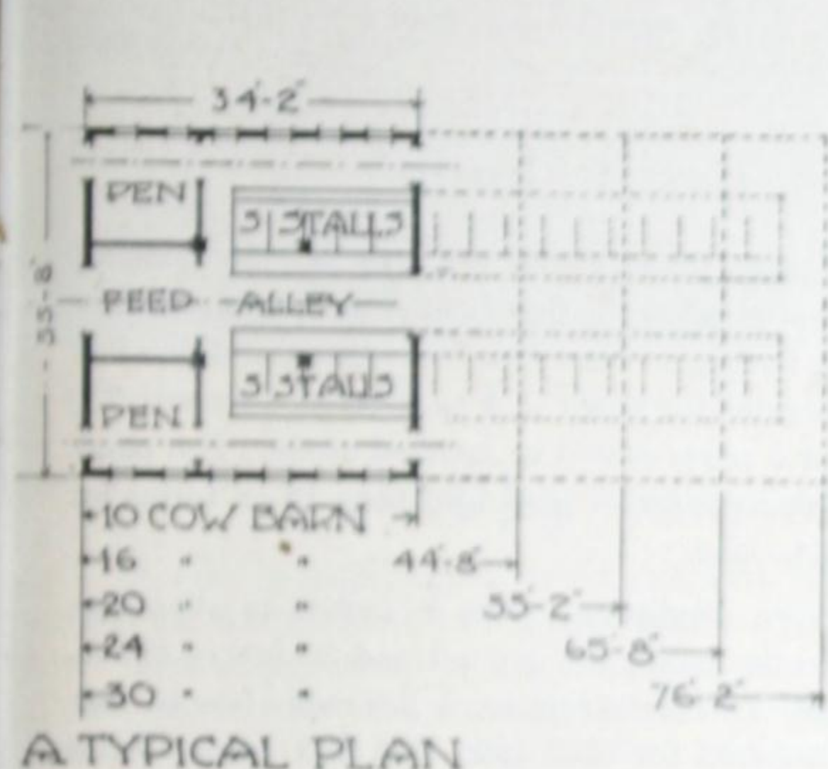
Fig. 100—Above and to the right model plans for layout of barn for different stock requirements. The drawing immediately above shows how this unit of construction can be made the basis for a growing barn to fit the growing needs of the farmer.
