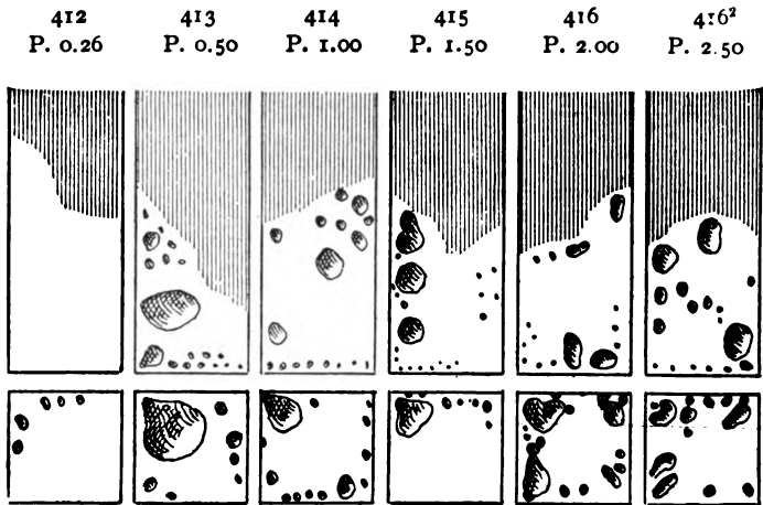
FIG. 31.—10.2% Iron Phosphide was added to White Iron, which diluted all elements same as Fig. 30, except P. The analysis of 412 was T. C. 3.00, Si. 0.25, P. 0.26. All other percentages are estimated.
