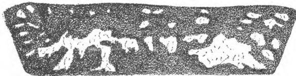
FIG. 46.—Fractures of Swedish Pig Irons.
