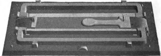
FIG. 85.—Keep's Test-bars \frac{1}{2} " \square \times 12".
