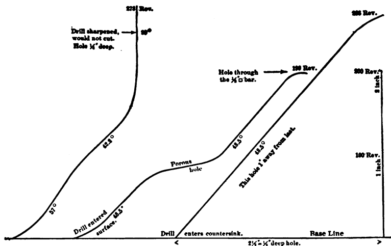
FIG. 84.—Hardness Diagram.
