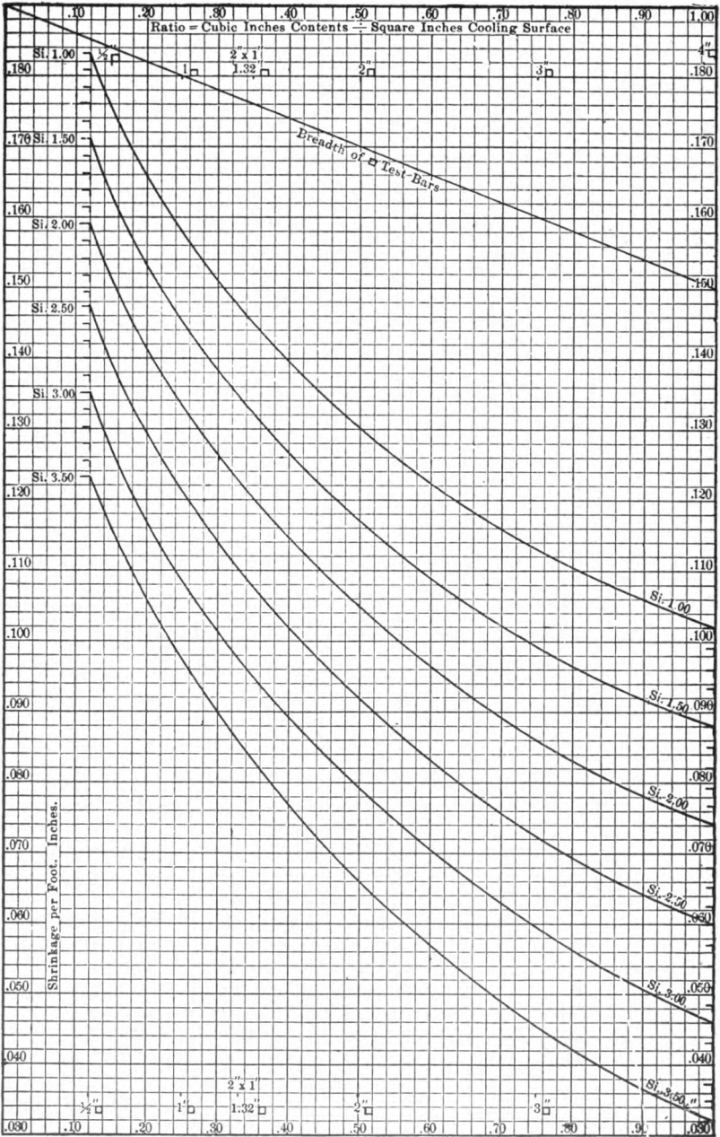
FIG. 81.—Keep's Shrinkage Chart. Approximate Relation of Shrinkage to Size and Percentage of Silicon.
