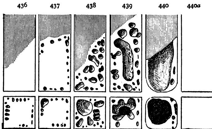
FIG. 30.—Steel Wire added to White Iron, remelted as in Fig. 29, and all elements diluted as in Fig. 31. Analysis of 436 same as 376. To 440 was added one per cent of aluminum, which made 440a, a solid casting.
