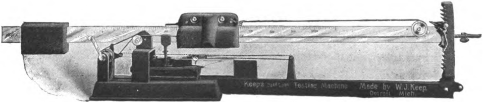
FIG. 90.—Keep's Dead-load Testing Machine, No. 10.
