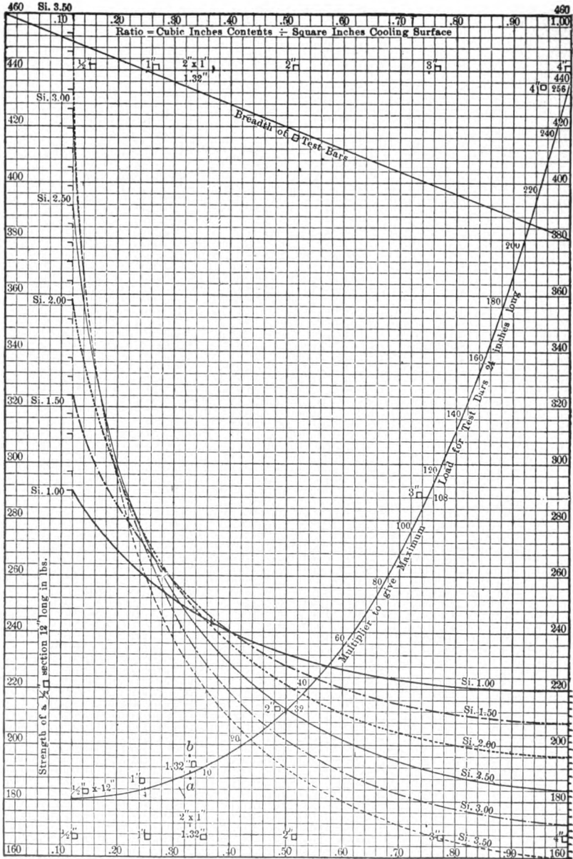
FIG. 82.—Keep's Strength Chart.—Approximate Relation of Strength to Size and Percentage of Silicon.
