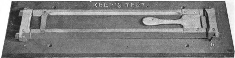
FIG. 91.—Keep's Test-bars 1" \square \times 24".
