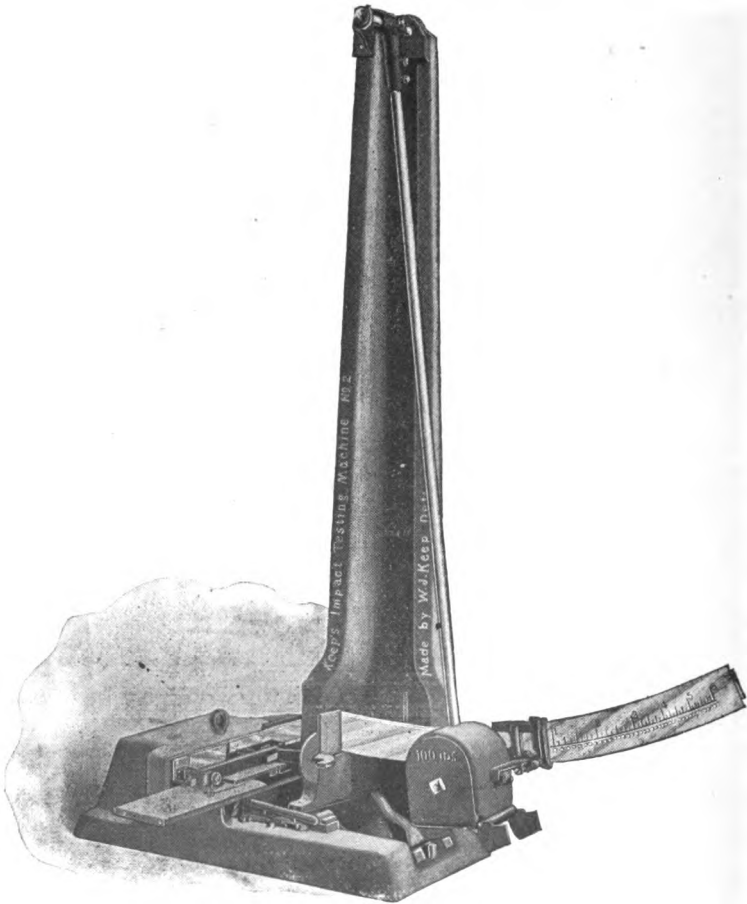
FIG. 98.—Keep's Impact-testing Machine, No. 2.
