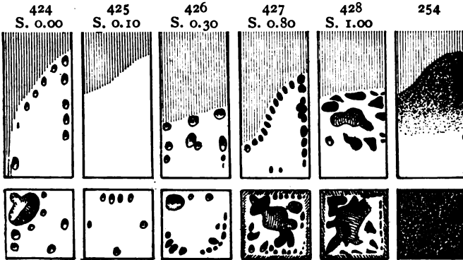
FIG. 40.—White Pig Iron + Iron Sulphide.
