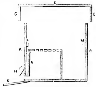
Fig. 4.—Longitudinal Section.
