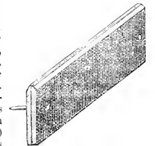
Fig. 12.—Side-board for inside lining: nail together so as to plane them up to true parallelograms.
