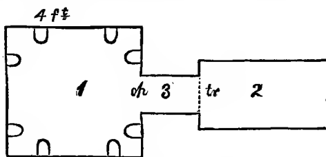
GROUND PLAN OF RABBIT-PIT.
