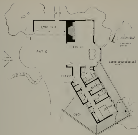
MICHAEL GOODMAN, ARCHITECT, BERKELEY—RESIDENCE FOR MR. AND MRS. THOMAS W. MOORE, RELIEZ VALLEY, LAFAYETTE
