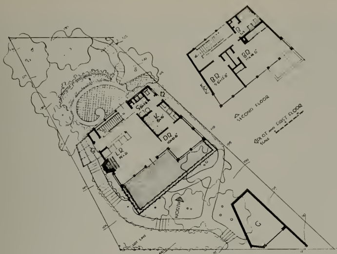
GARDNER A. DAILEY, ARCHITECT, SAN FRANCISCO—RESIDENCE FOR MR. AND MRS. L. D. OWENS Sausalito
