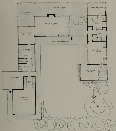
W. W. MAYHEW, ARCHITECT, SAN FRANCISCO—RESIDENCE FOR MR. AND MRS. J. MANOR, CONTRA COSTA COUNTY
