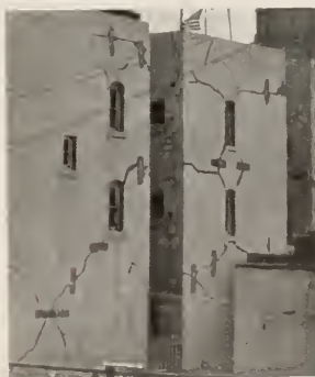
Horizontal and vertical ties may be used in repairing fractured walls.
