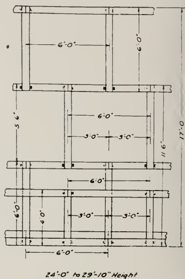
PLAN VIEW OF FOUNDATION COURSES.
