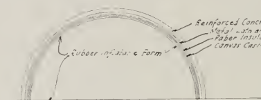
TYPICAL SECTION
