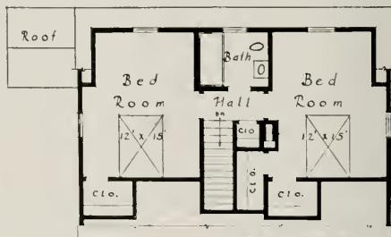
PLANS. HOUSE FOR MR. JOHN J. FARRELL Charles S. Keefe, Architect
