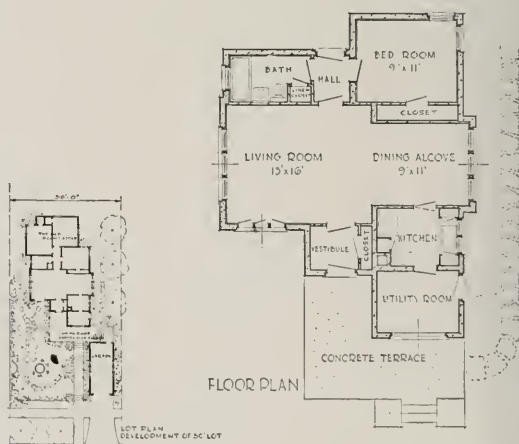
REINFORCED CONCRETE HOME OF MODERATE COST
