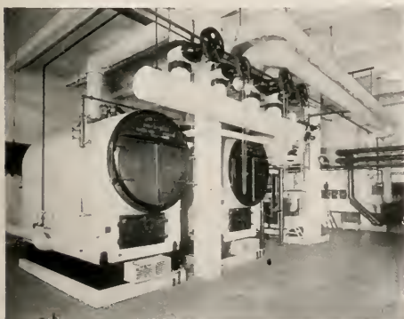
GAS FIRED BOILER INSTALLATION, HUNTINGTON LIBRARY, PASADENA
