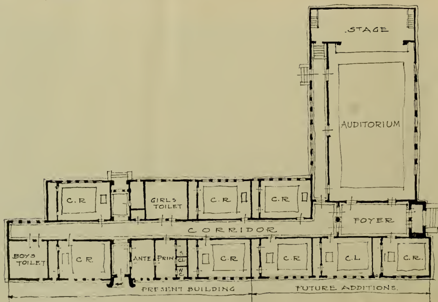
PLAN, LINDEN SCHOOL BUILDING, CHICO, CALIFORNIA Chester Cole, Architect; Louis L. Brouchoud
