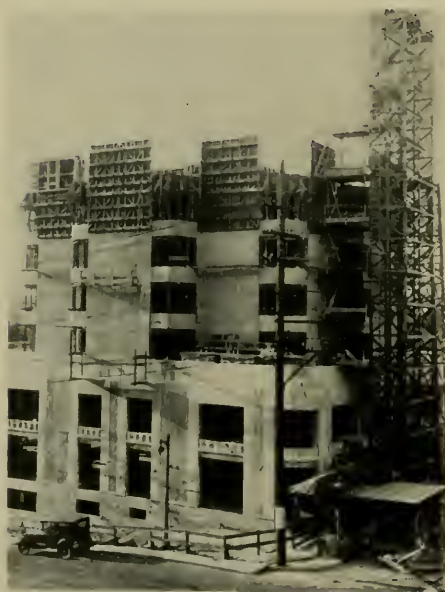
CONSTRUCTION VIEW, EDMOND MEANY HOTEL, SEATTLE R. C. Reamer, Architect
