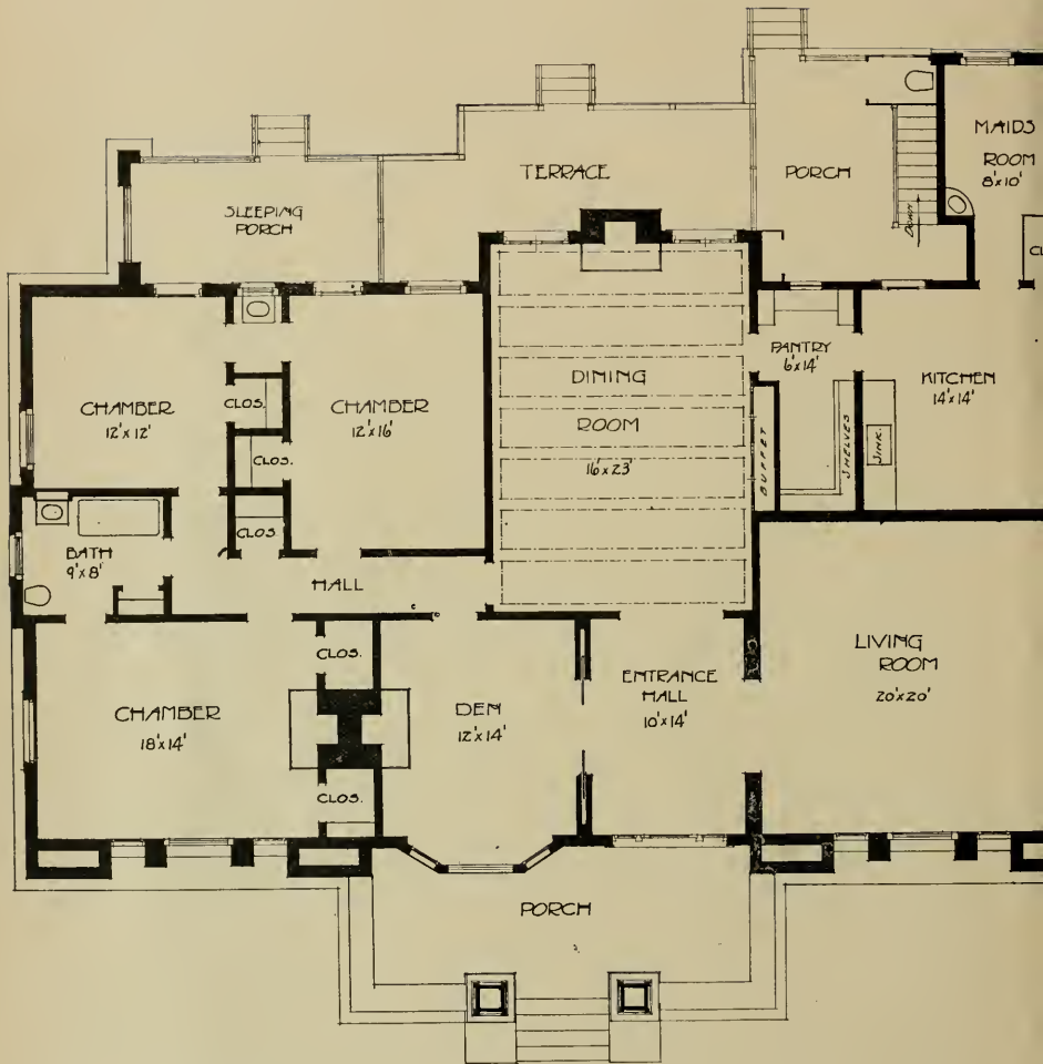
FLOOR PLAN, MISSION BUNGALOW TUCSON, ARIZONA
