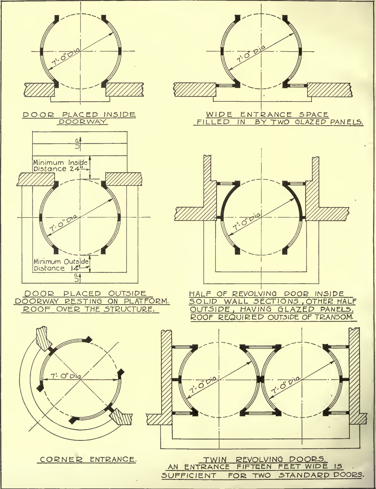
FIG. 2. VARIOUS ENTRANCE ARRANGEMENTS FOR REVOLVING DOOR INSTALLATIONS
