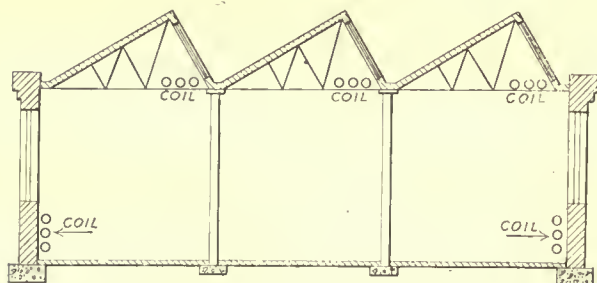
FIG. 3. OVERHEAD HEATING COILS
