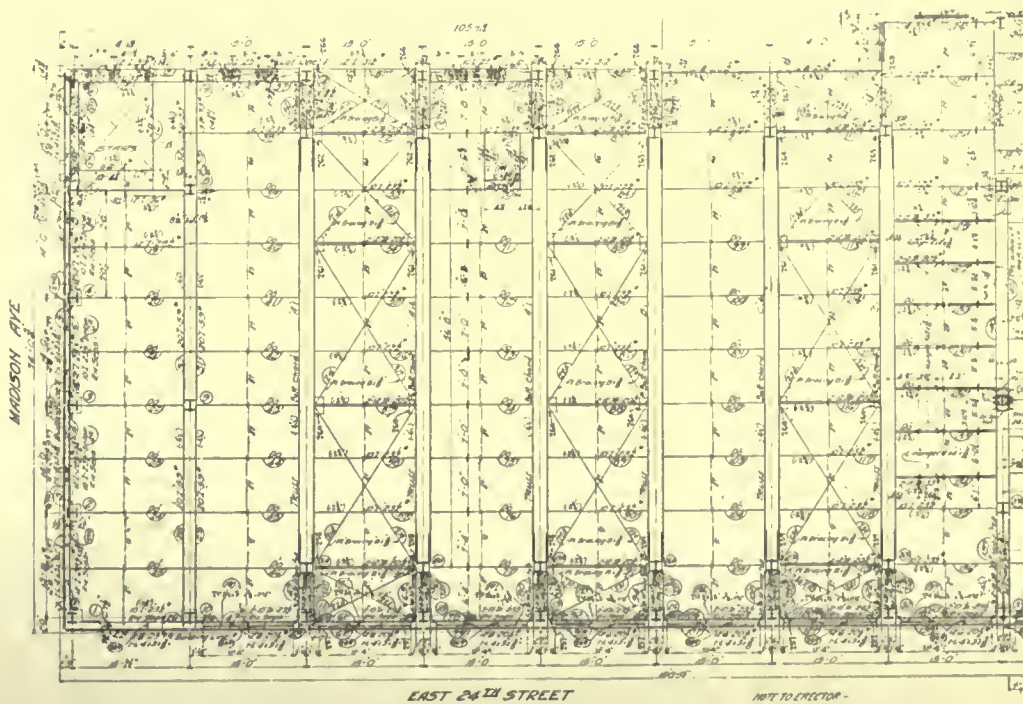
PORTION OF THIRD FLOOR FRAMING PLAN, SHOWING LOCATION OF TRUSSES AND DOUBLE-PLATE GIRDER
