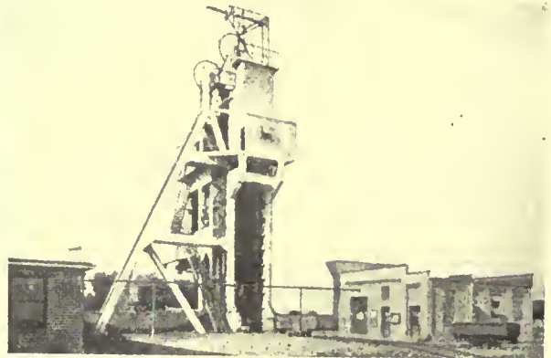
A TYPICAL CONCRETE HEAD-FRAME
