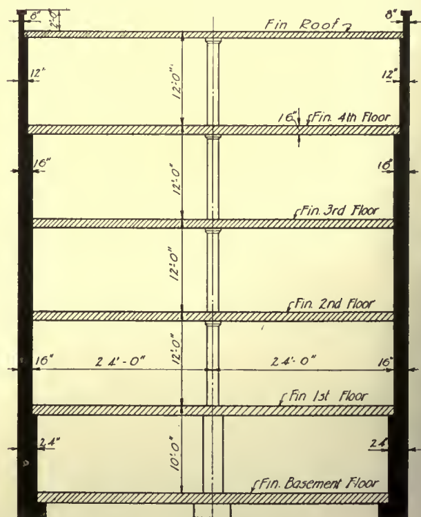
FIG. 2. CROSS-SECTION
