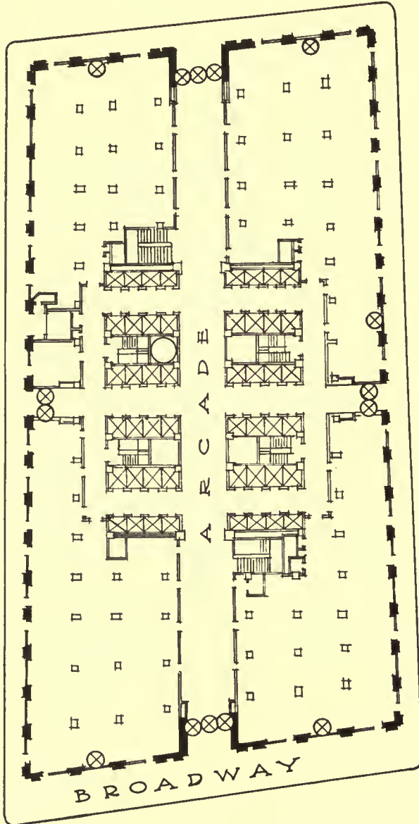
GROUND FLOOR PLAN, EQUITABLE BUILDING, NEW YORK CITY
