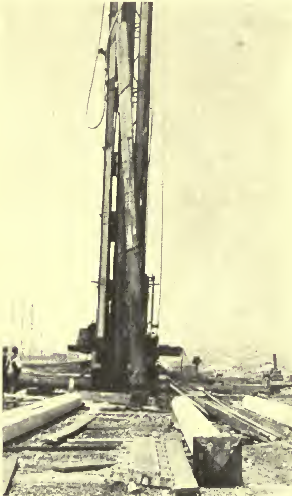
WITHDRAWING ONE OF THE TEST PILES
