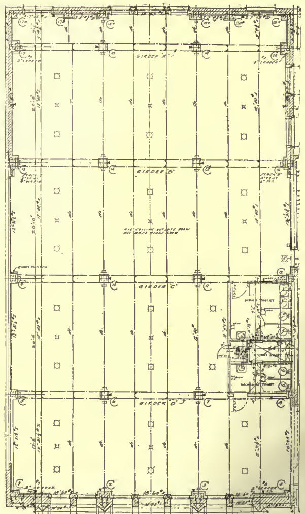
FOURTH FLOOR FRAMING PLAN Showing location of girders.
