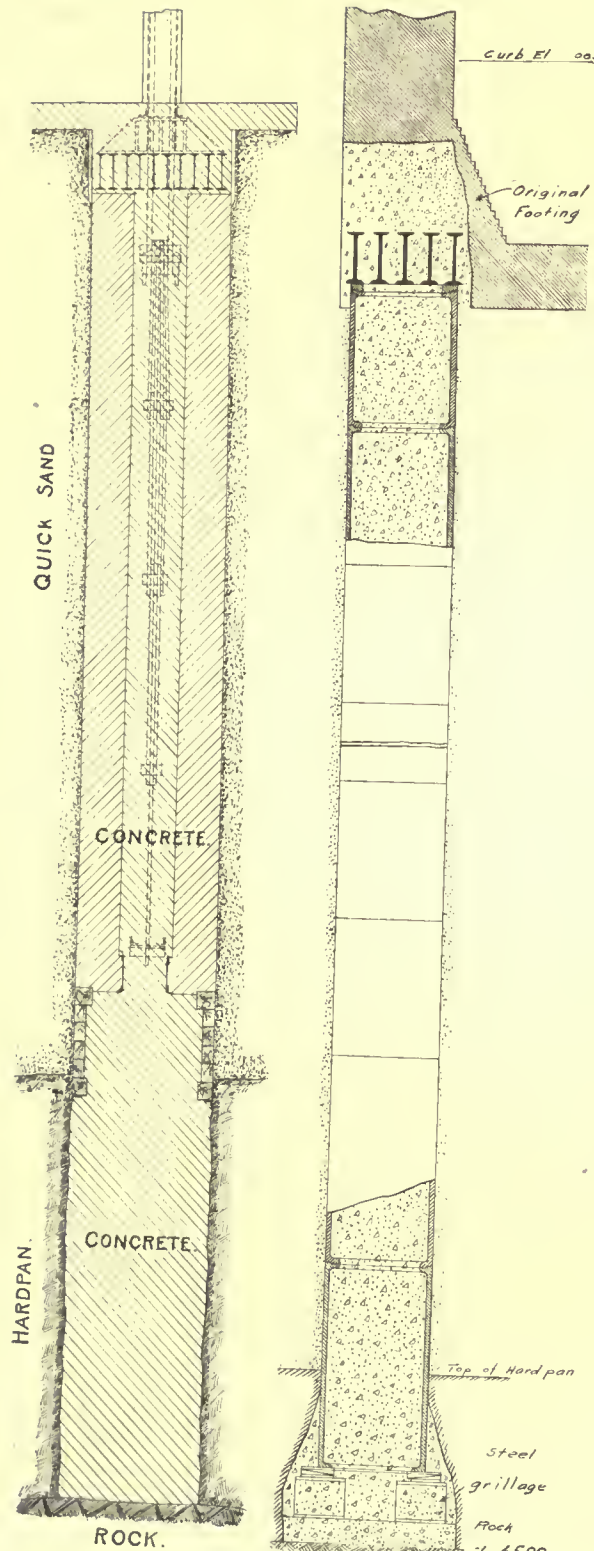
AT LEFT: METHOD USED IN ANCHORING COLUMNS TO CAISSONS, SINGER BLDG., N. Y. CITY At right: Caisson construction used in underpinning foundations of an existing building
