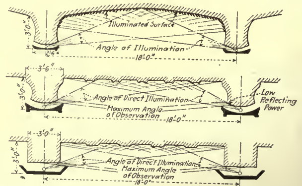
FIG. 5. THREE CROSS SECTIONS ILLUSTRATING SUGGESTED METHODS OF THEATRE ILLUMINATION
