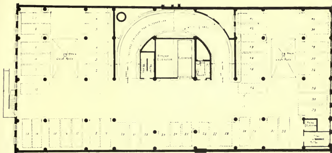
SECOND, THIRD AND FOURTH FLOOR PLANS HOTEL LA SALLE GARAGE, CHICAGO, ILLINOIS HOLABIRD & ROCHE, ARCHITECTS
