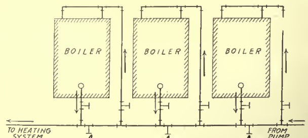
FIG. 2. BOILER CONNECTIONS
