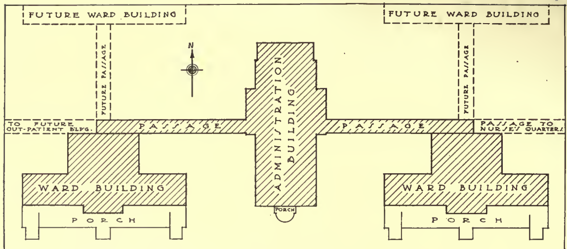
PLOT PLAN
