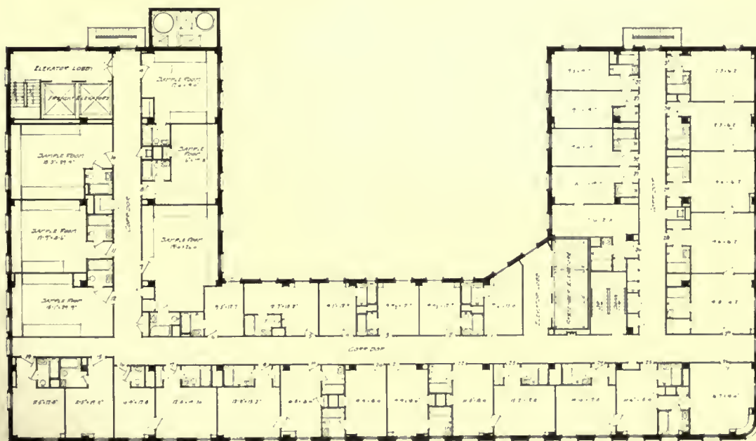
PLANS OF THE FOURTH FLOOR AND ABOVE
