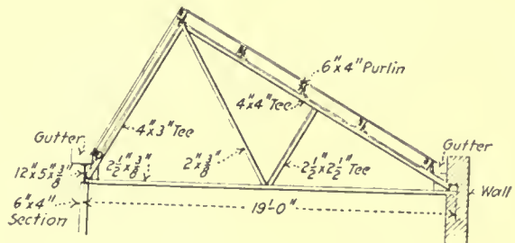
ARC WELDED ROOF TRUSS FOR SAWTOOTH CONSTRUCTION
