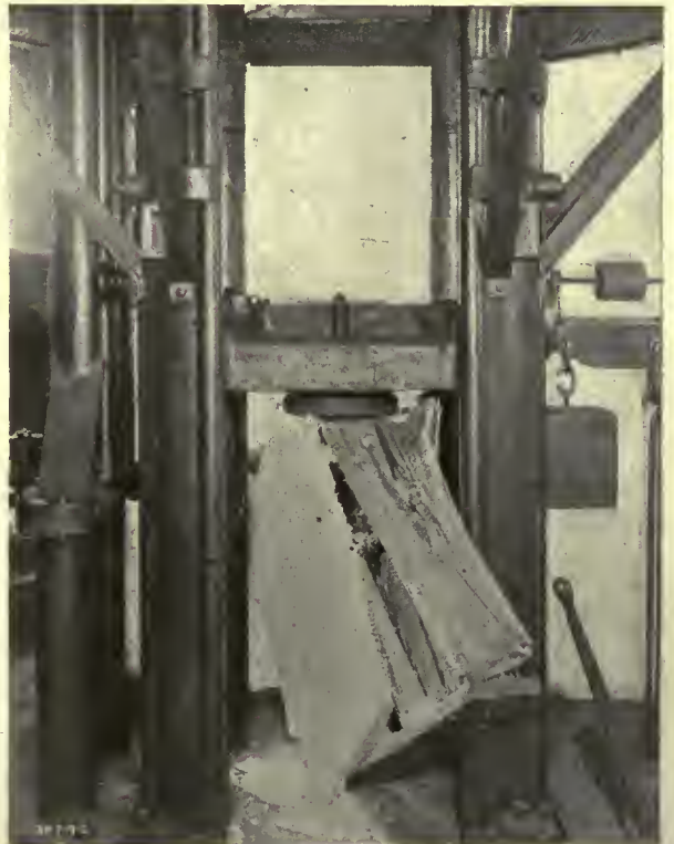
FAILURE OF WALL PANEL
