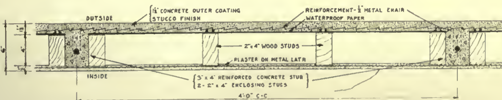
FIG. 2. TYPICAL CROSS-SECTION OF THE OUTSIDE WALL
