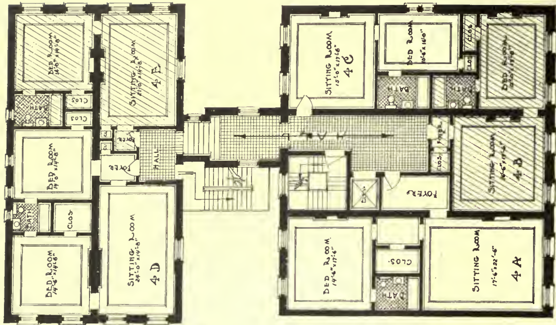
TYPICAL PLAN
