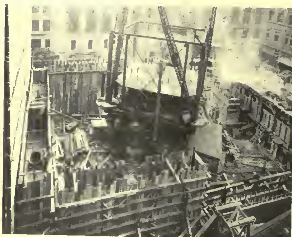
LATER VIEW, SEABOARD BANK BUILDING, ILLUSTRATING METHOD OF SINKING SERIES OF RECTANGULAR CAISSONS TO FORM ENCLOSING WALL
