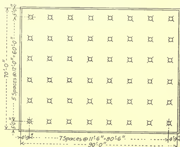
FIG. 2. FLOOR PLAN OF DRAFTING ROOM.
