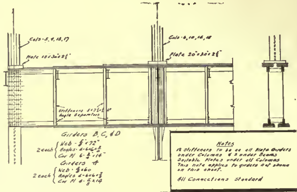
Detail of Girders A.C.C. & D
