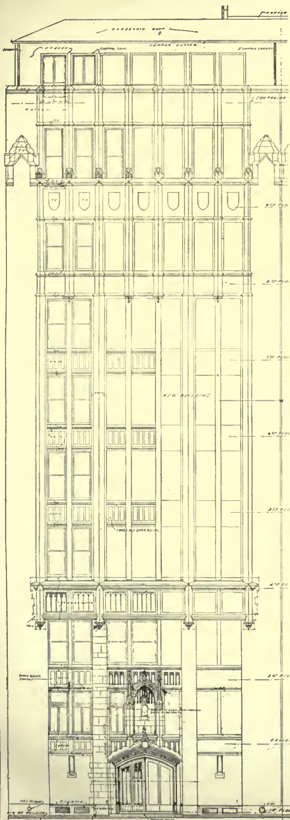
FRONT ELEVATION
