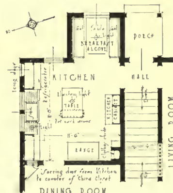
PLAN OF KITCHEN
