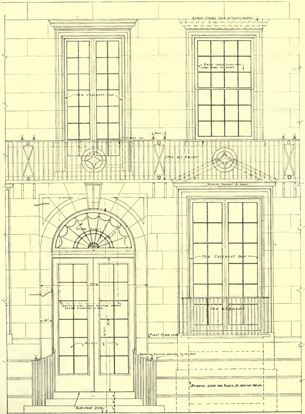
• 3/4-INCH SCALE • DETAIL • OF • ENTRANCE • MOTIVE •
