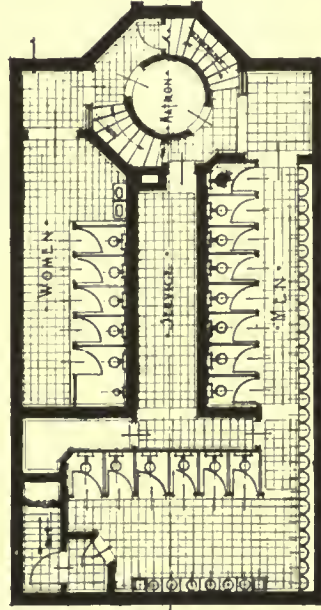
PLAN
