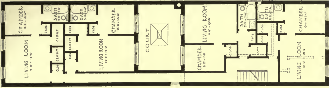
THIRD FLOOR PLAN ALTERATION TO HOUSE, H O U S E , NO. 128 WEST 49th STREET, NEW YORK HERBERT LUTTMAN, ARCHITECT
