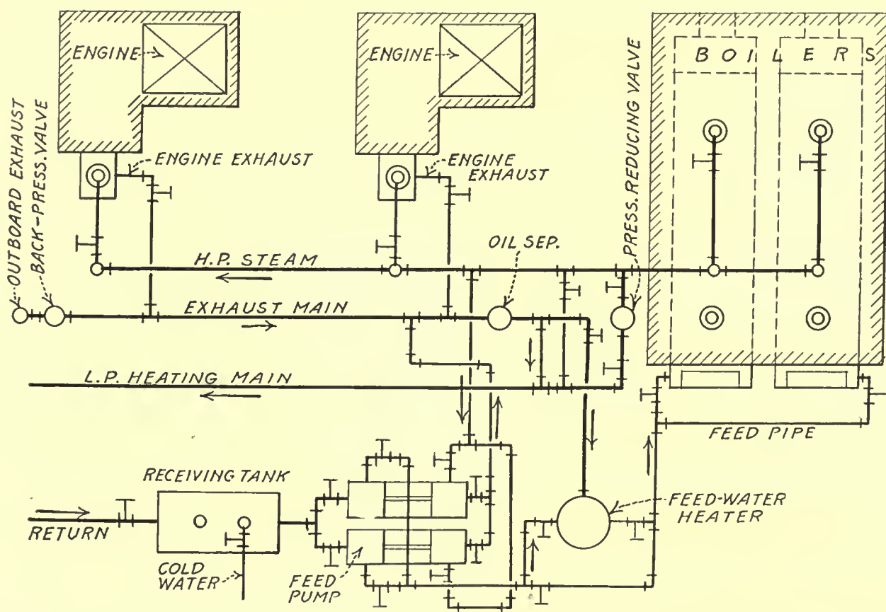
FIG. 7. PIPING LAYOUT WHERE EXHAUST STEAM IS UTILIZED FOR HEATING
