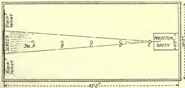
FIG. 2. PLAN OF EXPERIMENTAL ROOM
