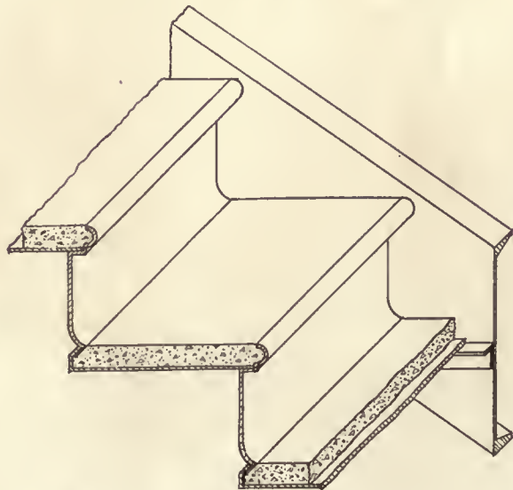
FIG. 8.—STEEL STAIRS WITH CONCRETE TREAD
