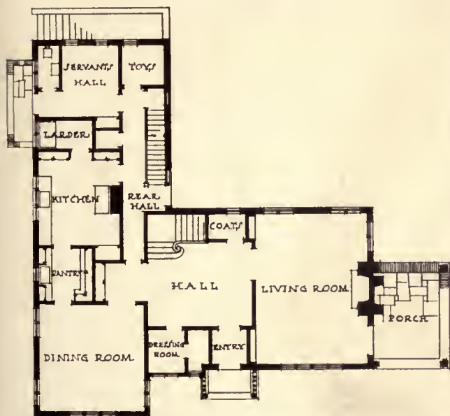
FIRST FLOOR PLAN SCALE 1/4" = 1' IN FEET
