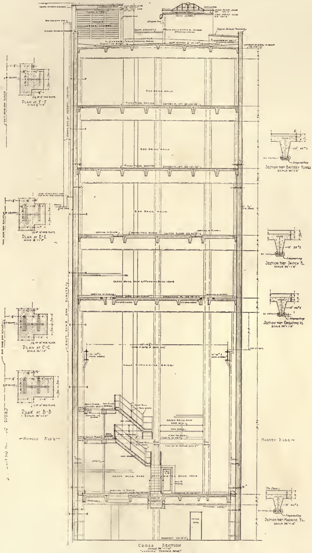
CHAUNCEY STREET STATION EDISON ELECTRIC ILLUMINATING CO., BOSTON, MASS. BIGELOW & WADSWORTH, ARCHITECTS
