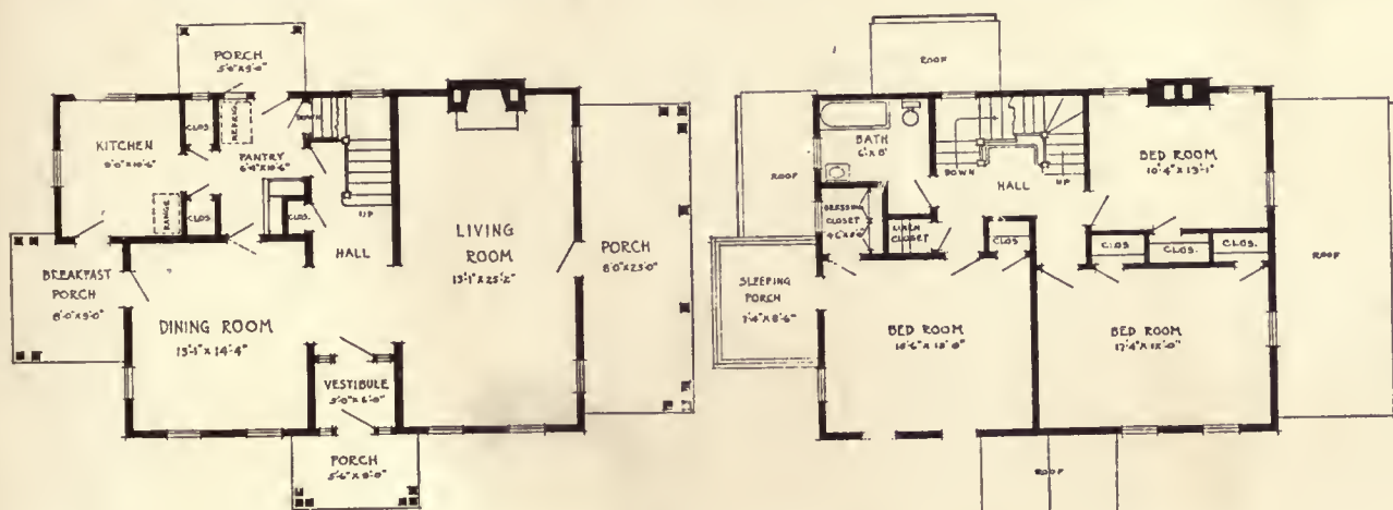
SIX-ROOM HOUSE—TYPE G GEORGE GILBERT, ARCHITECT
