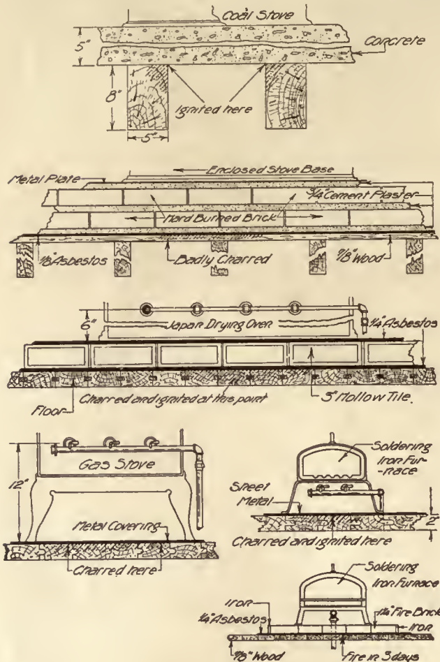
FIG. 1. FIRES DUE TO IMPROPER INSTALLATION OF HEATING DEVICES. TO MANY ANY OF THESE SIX INSTALLATIONS WOULD HAVE APPEARED PERFECTLY SAFE
