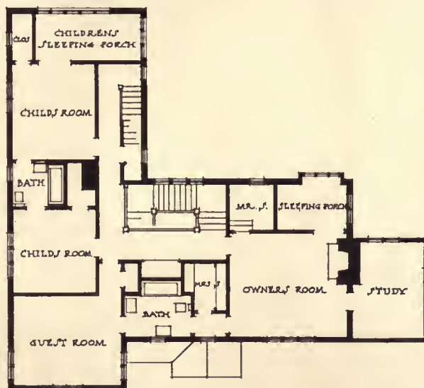
SECOND FLOOR PLAN SCALE 1/4" = 1' IN FEET
