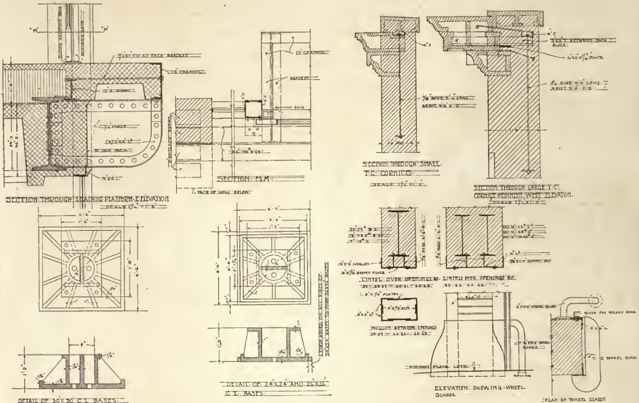
CONSTRUCTION DETAILS
