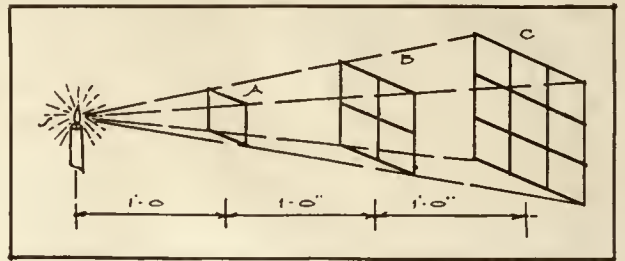
FIG. 2. THE ILLUMINATION ON A SURFACE VARIES INVERSELY AS THE SQUARE OF THE DISTANCE FROM THE SOURCE TO THE SURFACE
