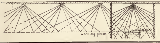
FIG. 6. WHERE RATIO OF ROOM WIDTH TO CEILING HEIGHT IS LARGE ALL RAYS REACH WORKING PLANE DIRECT, BUT WHERE THE RATIO IS SMALL THE RAYS MUST BE REFLECTED BY THE WALLS WITH CONSEQUENT LOSS
