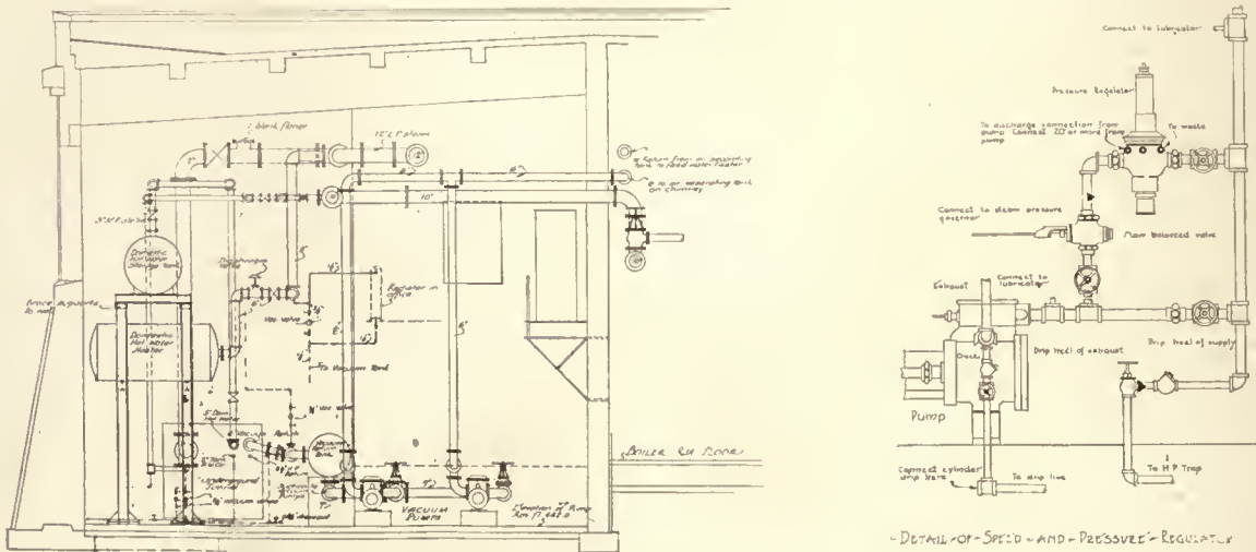
SECTION - TURV - PUMP - ROOM - SCALE - 1/4" = 1'-0"
