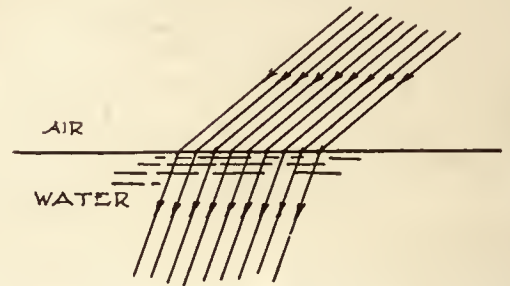
FIG. 5. REFRACTION. RAYS PASSING FROM ONE MEDIA TO ANOTHER OF DIFFERENT DENSITY ARE BENT
