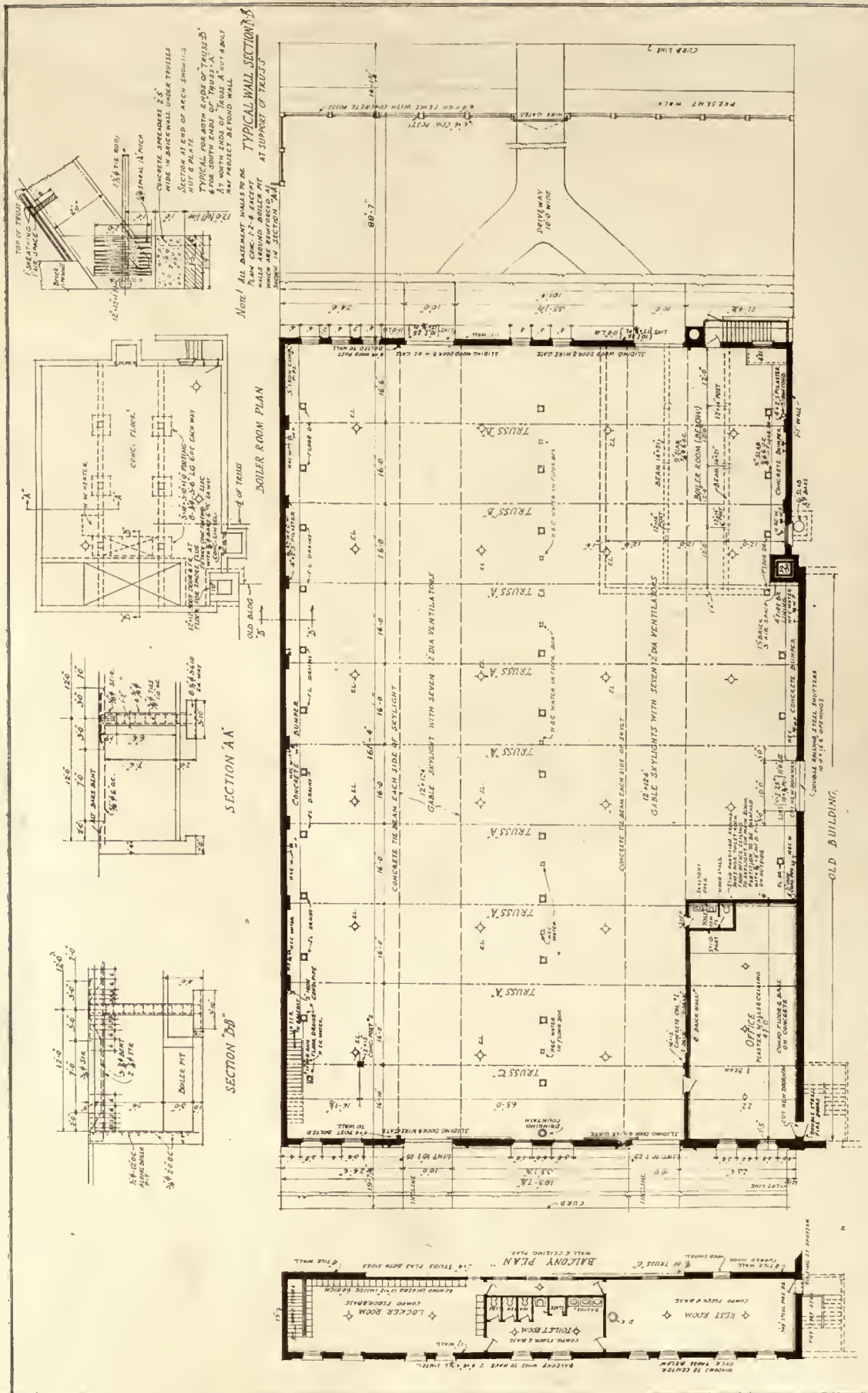
PLAN—GARAGE FOR MANDEL BROTHERS, CHICAGO I. S. STERN, ARCHITECT, L. J. MENSCH, ENGINEER
