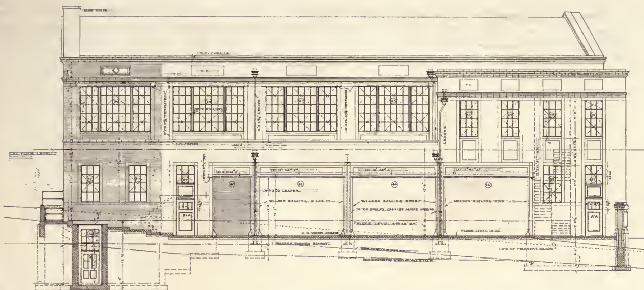
NORTH ELEVATION
