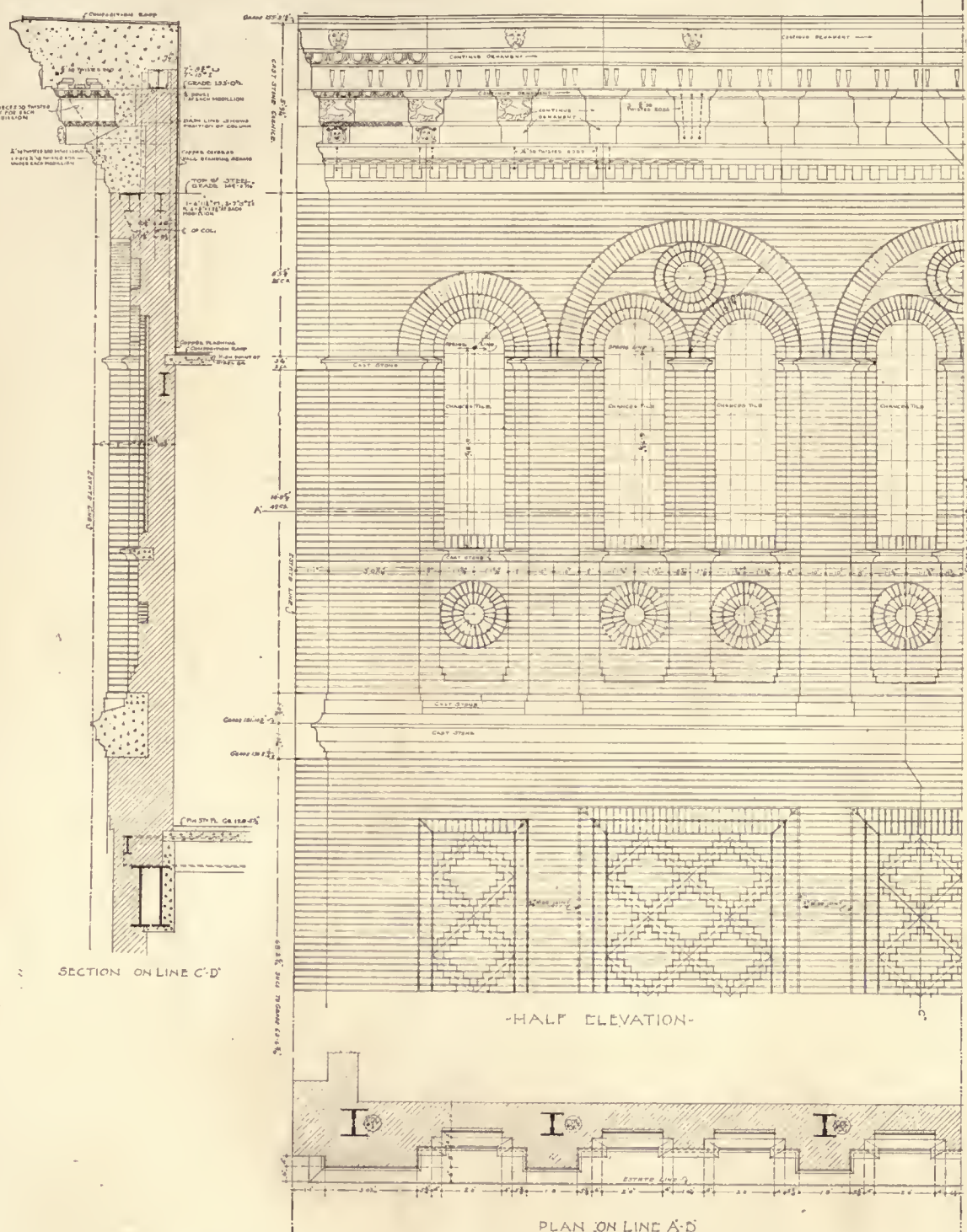
1/4 INCH SCALE DETAIL OF UPPER PART FRONT ELEVATION CHAUNCY STREET [21 ST ] STATION BOSTON FOR THE EDISON ELECTRIC ILLUMINATING COMPANY
