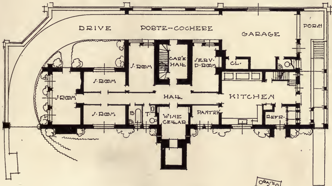
BASEMENT PLAN
