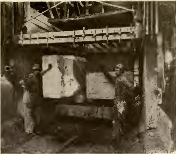
VIEW OF STONE GANG-SAW. ON THE GRATING ABOVE IS PLACED OTTAWA SAND, USED AS AN ABRASIVE, THE SAWS NOT BEING PROVIDED WITH TEETH
