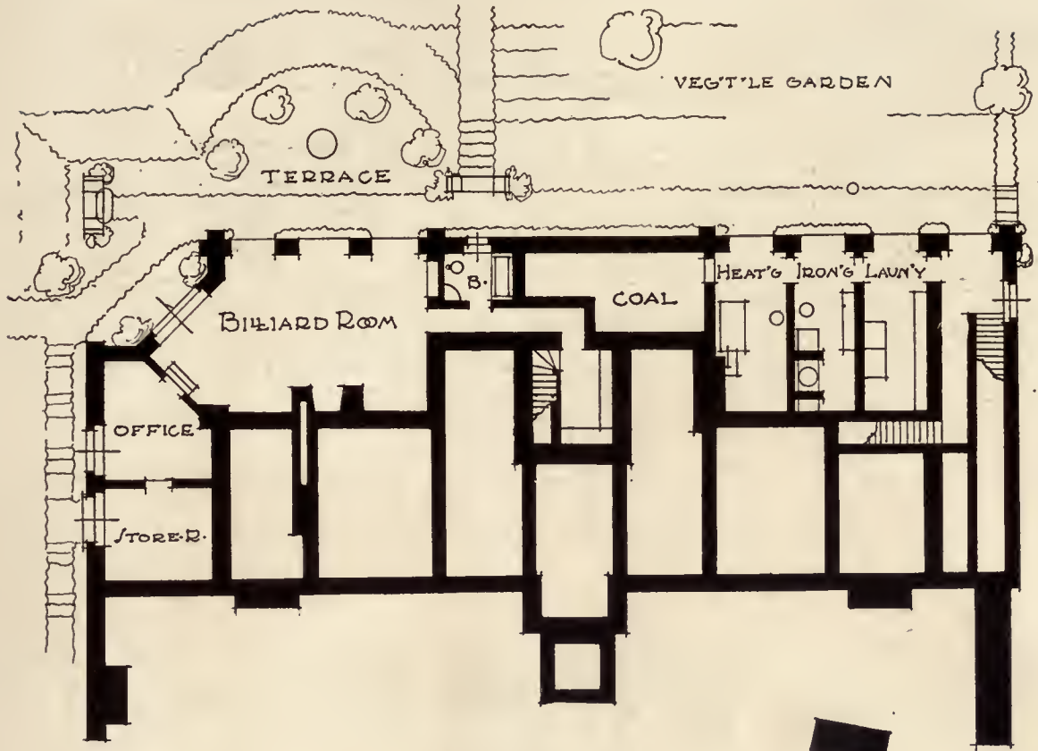
SUB-BASEMENT PLAN
