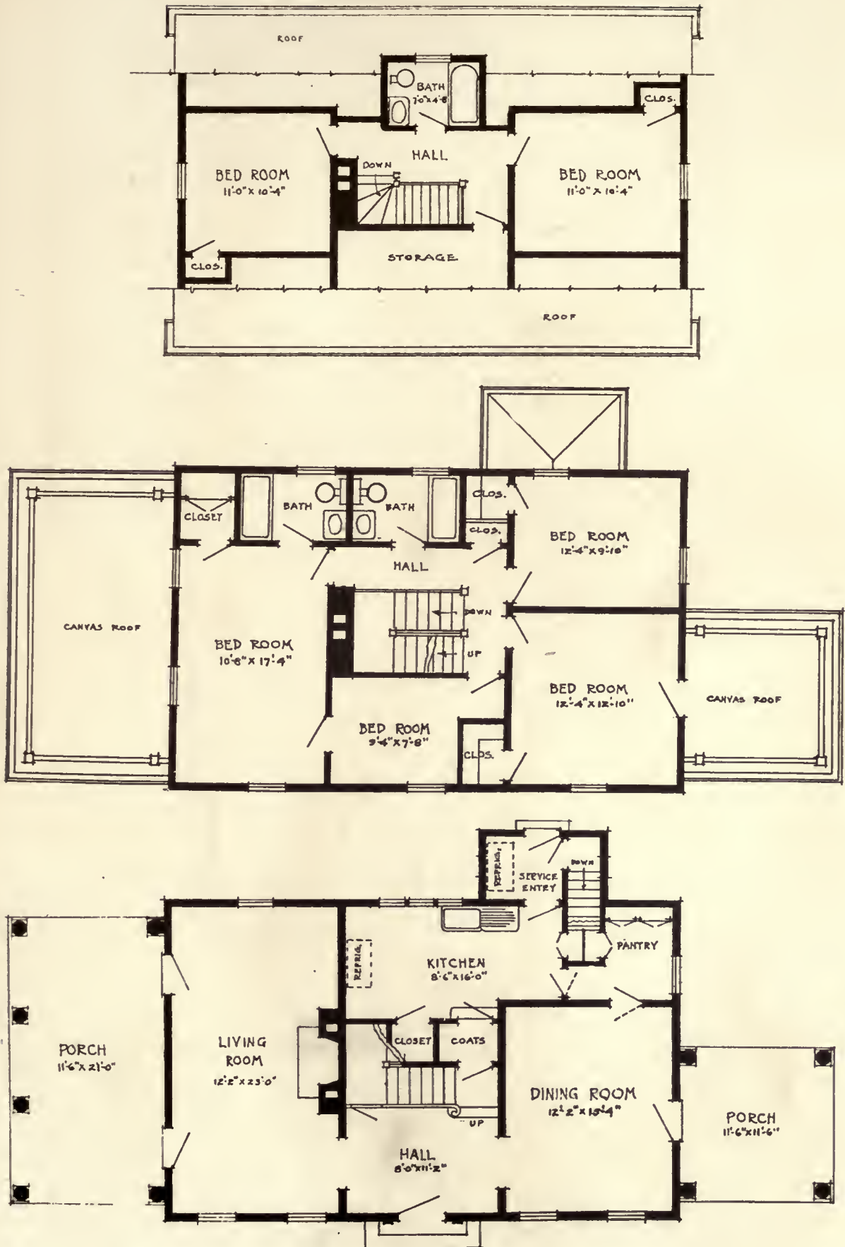
FLOOR PLANS, TYPES S 2 AND 3 MOTT B. SCHMIDT, ARCHITECT
