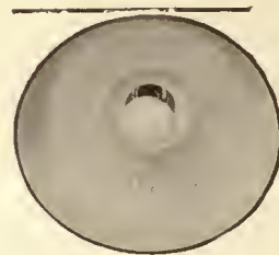
FIG. 5. PORCELAIN ENAMELED STEEL REFLECTOR AND ENAMELED-BOWL LAMP
