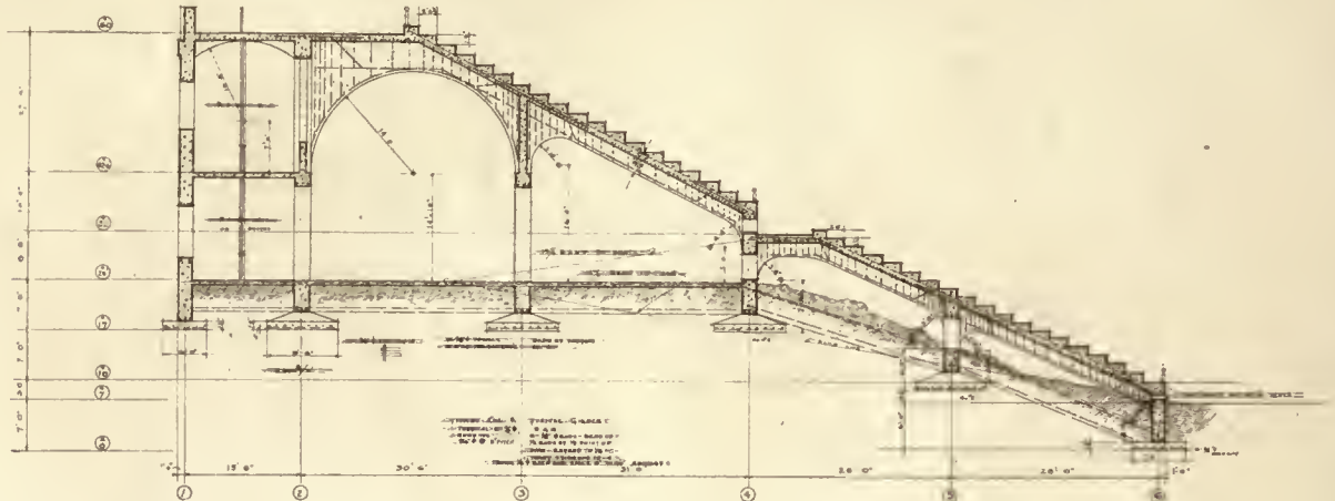
SECTION
