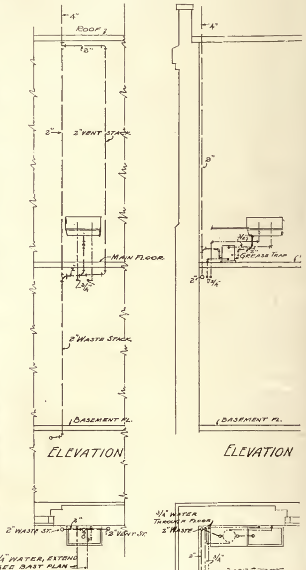
DETAILS KITCHEN SINKS
