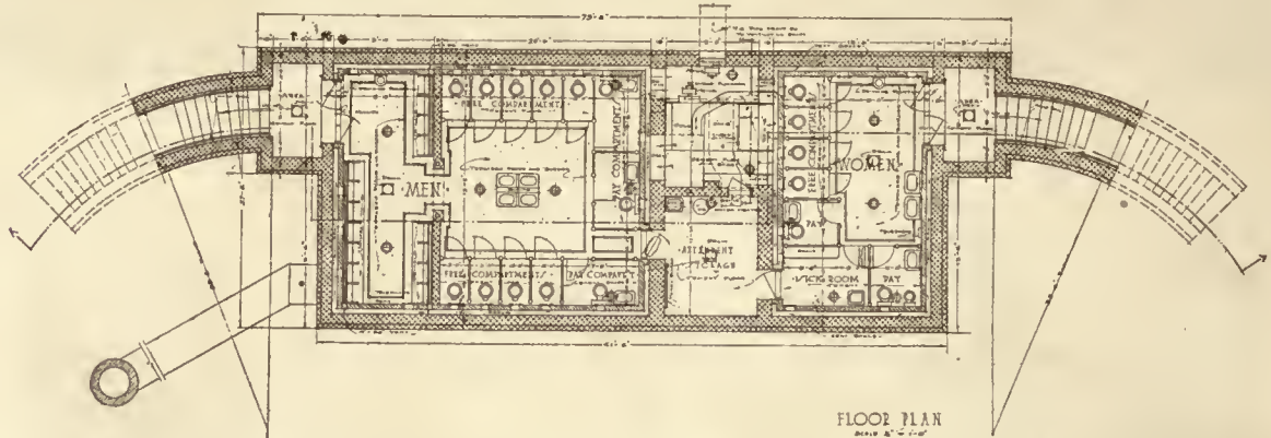
PLAN OF UNDERGROUND PUBLIC CONVENIENCE STATION, SCRANTON, PA. DUCKWORTH BROTHERS, ARCHITECTS
