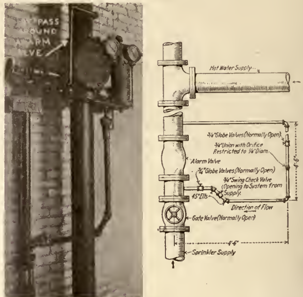
FIG 3. THE ARRANGEMENT OF VALVE HERE SHOWN IS IDENTICAL WITH REGULAR SYSTEM EXCEPT FOR THE BY-PASS.
