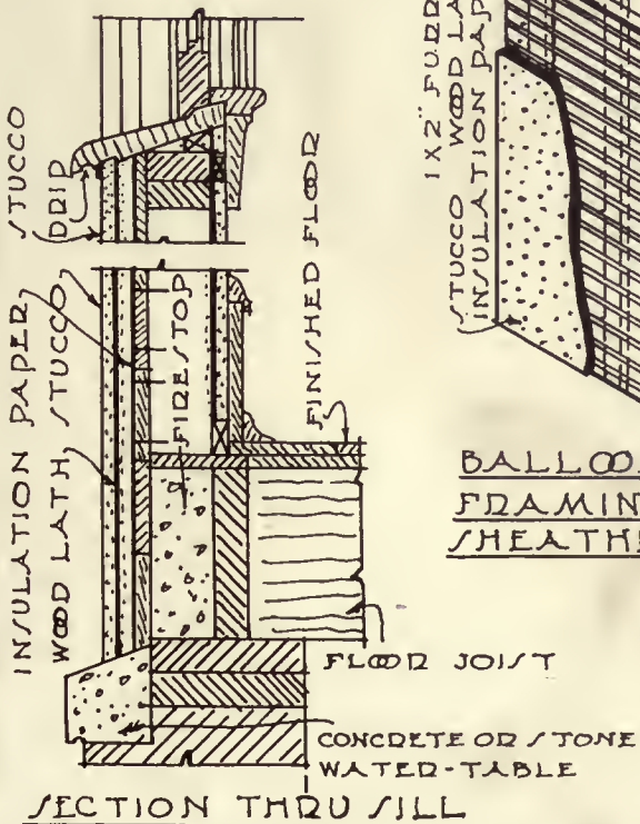
CONSTRUCTION DETAILS, STUCCO ON WOOD LATH
