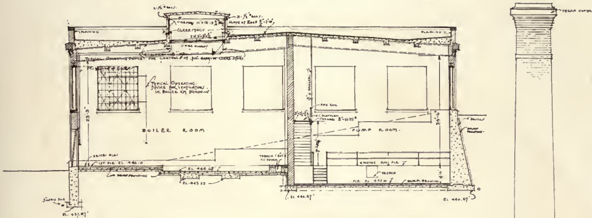
SECTION THRO. BOILER &amp; PUMP RMS. 4
