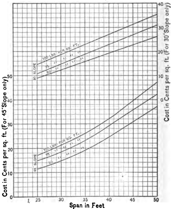
8 FT. BAY CURVES SHOWING THE RELATION OF COST TO SPAN (For Truss see Table 16)
