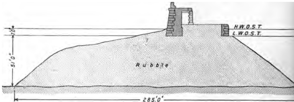
FIG. 92.—Section of Portland Breakwater.
