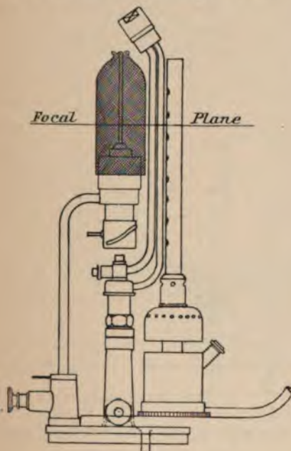
FIG. 231.—Pintsch Burner.
