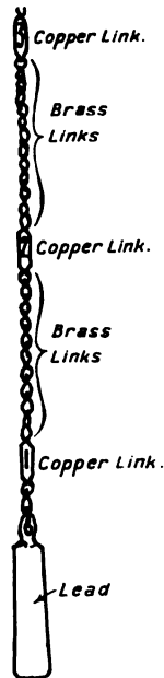
FIG. 41.—Chain Sounding-line.
