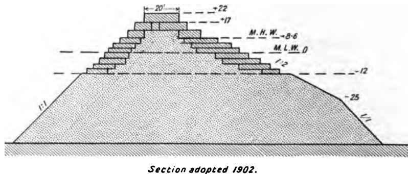
FIG. 121.—Section of Breakwater, Sandy Bay, U.S.A.
