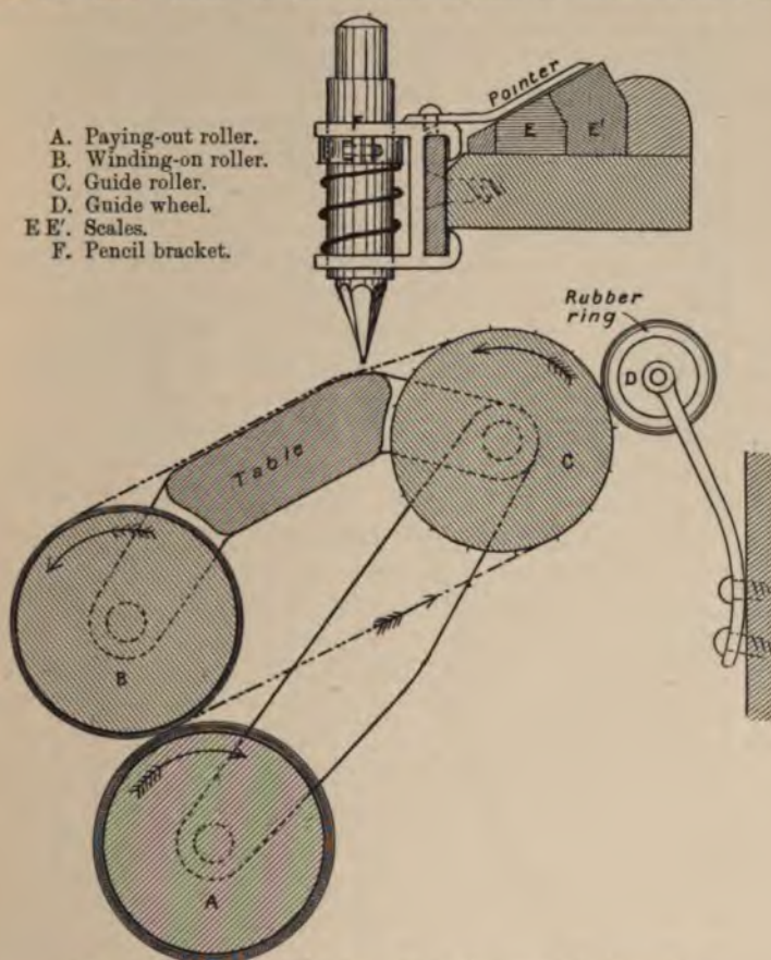
FIG. 43.—Mechanism of Section Plotter in Sutcliffe's Apparatus.
