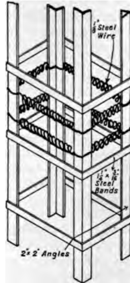
Figs. 68.—Johnston Pile.
