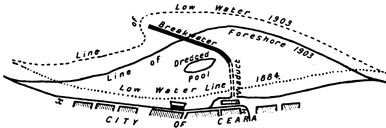
FIG. 19.—Harbour of Ceara. Effect of breakwater.
