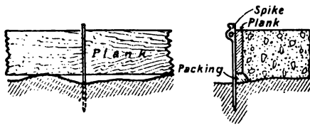
FIG. 133.—Moulds for Concrete Foundation.
