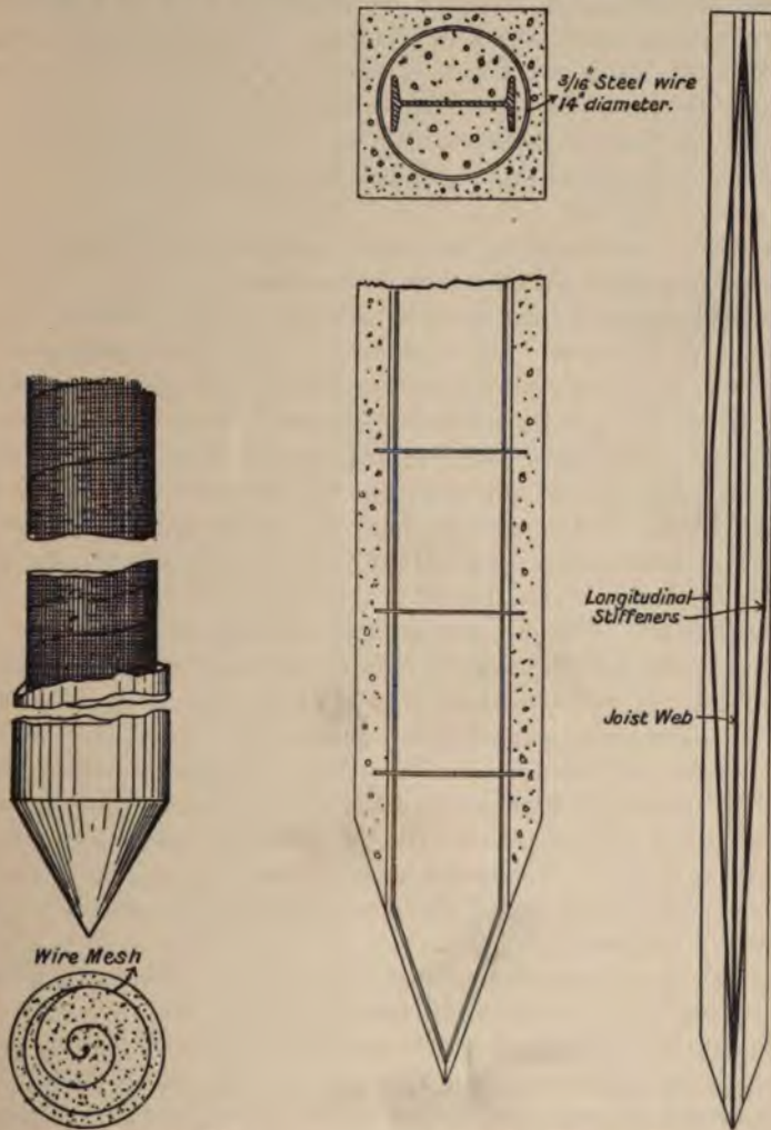
FIGS. 69.—Chenoweth Pile.
