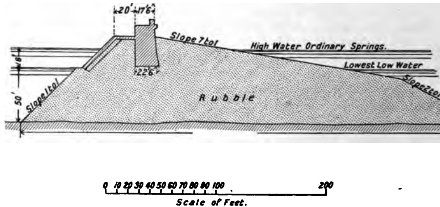
FIG. 97.—Section of Holyhead Breakwater.
