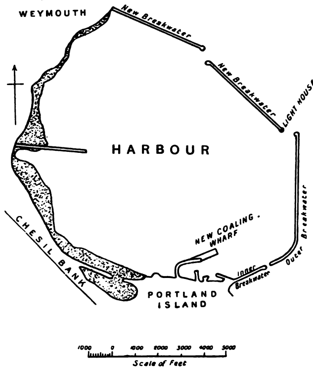
FIG. 5.—Portland Harbour.
