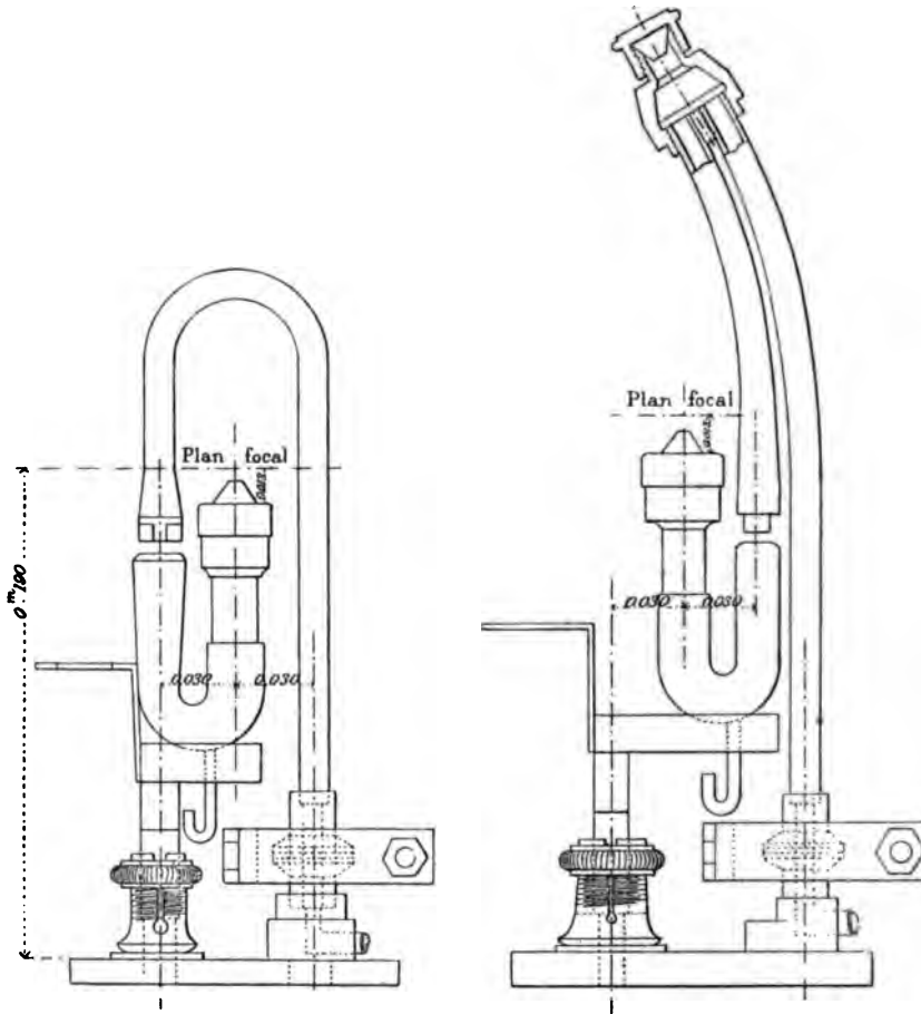
FIG. 233.—Luchaire Burner.
