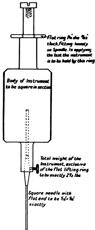
FIG. 90.—Needle for Cement Testing.
