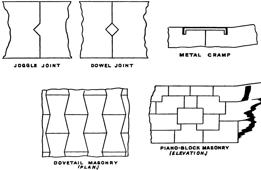
FIGS. 137-141.—Masonry Joints and Connections.
