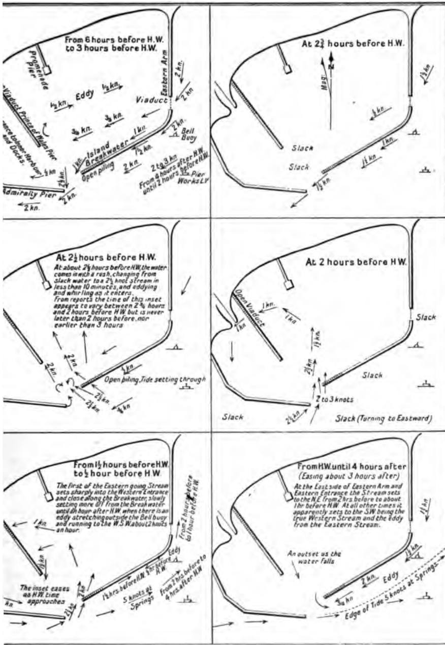
FIGS. 23-28. — Tidal Currents in and out of Dover Harbour.
