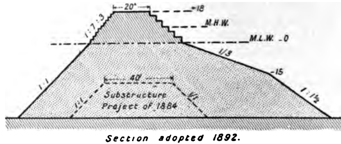
FIG. 120.—Section of Breakwater, Sandy Bay, U.S.A.
