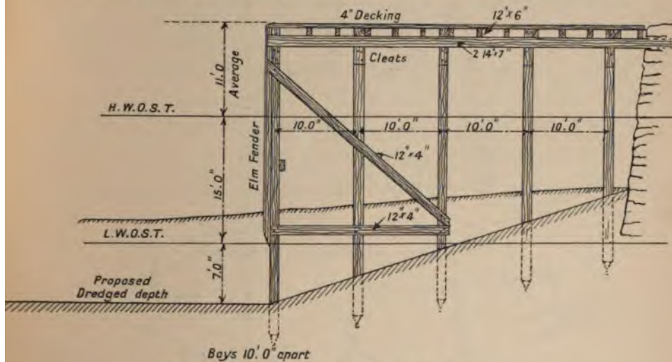
FIG. 34.—Whitby Harbour. Proposed fish quay.
