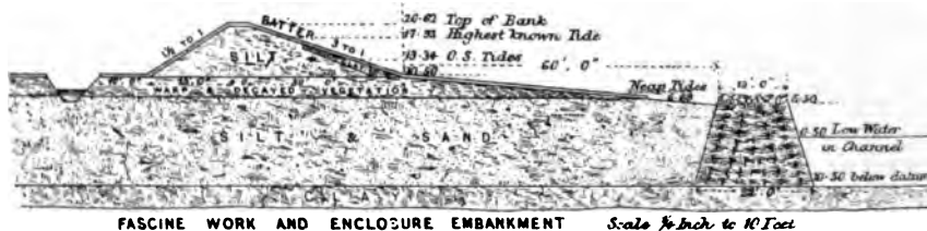
FIG. 212.—Fascine Work in the Wash. 1
