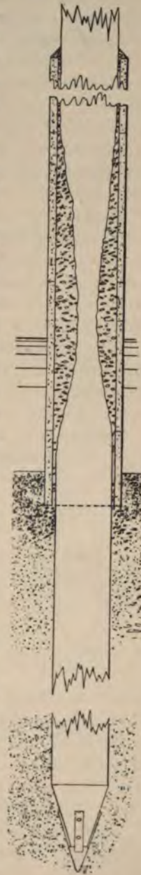
FIG. 61.—Application of Reinforced Concrete Slabs to Decayed Timber Pile.
