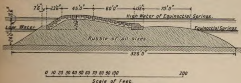
FIG. 93.—Section of Plymouth Breakwater.
