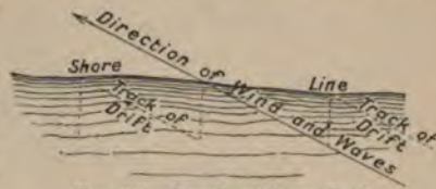
FIG. 14.—Track of Shore Drift.
