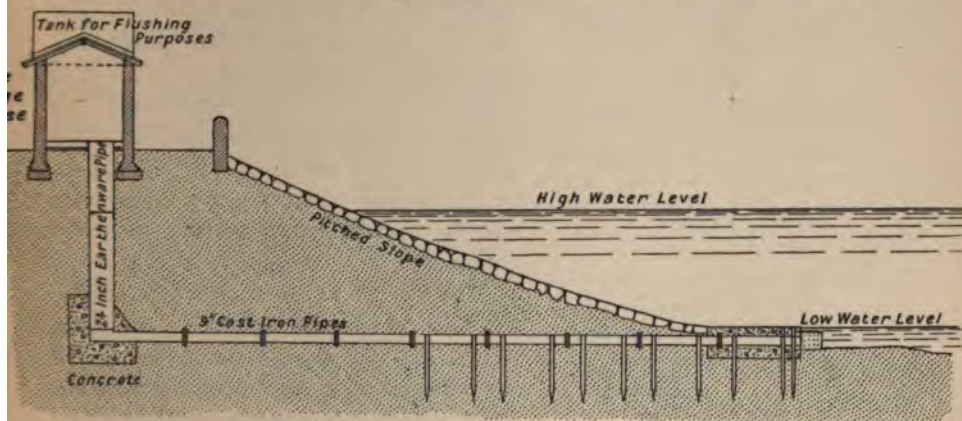
FIG. 48.—Tide-gauge House on River Bank.
