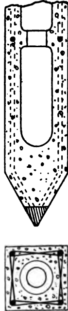
Figs. 67.—Mouchel Hollow Pile.
