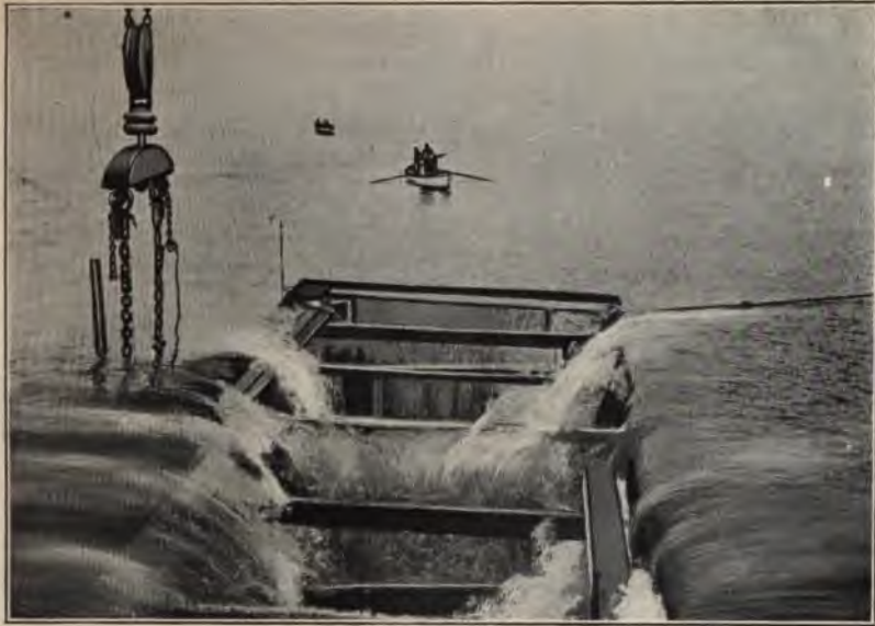
FIG. 151.—Sinking a Caisson at Zeebrugge Harbour Works.
