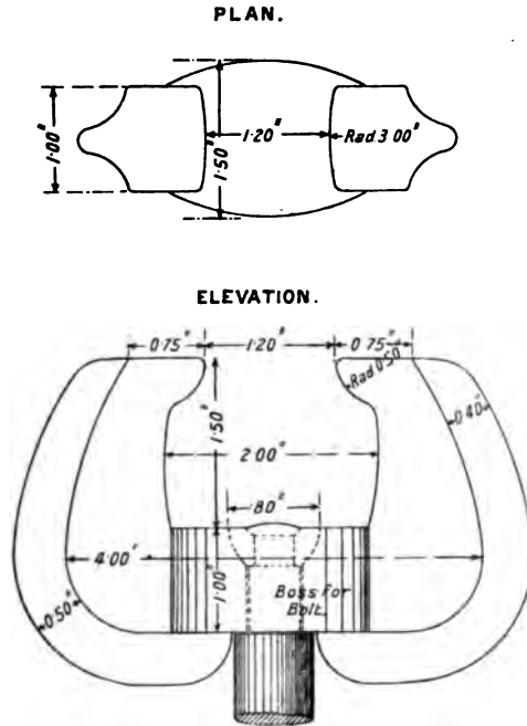
FIG. 89.—Standard Jaws for Briquette.
