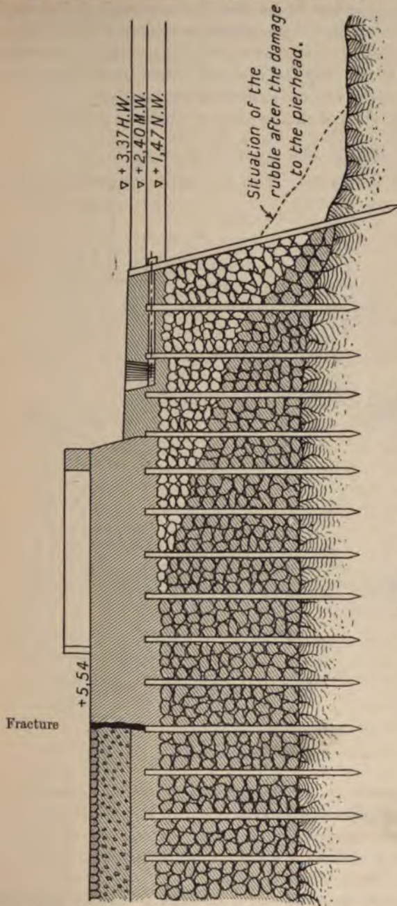
FIG. 162.—Longitudinal Section of South Pierhead at Pillau.
