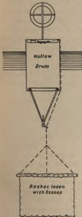
FIG. 53.—Float used on River Avon.
