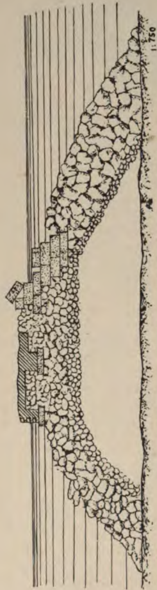
FIG. 112.—Section of Damaged Portion of Galliera Mole from C to D, fig. 109.
